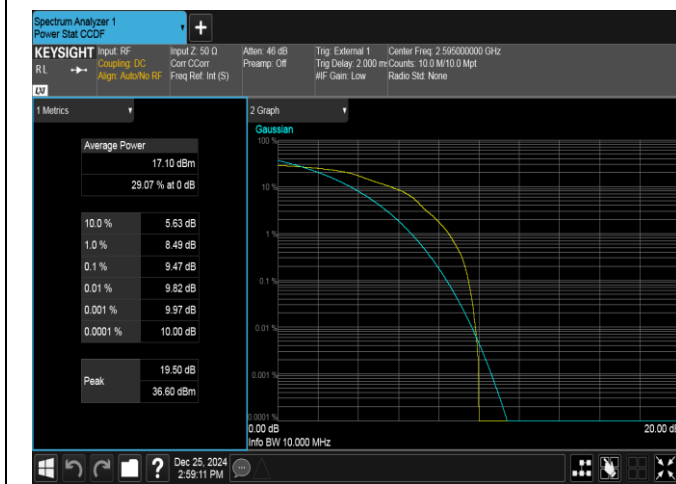
Band38-10MHz-16QAM-38000-1RB#0-PASS
