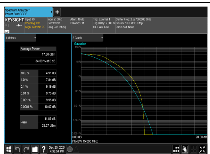
Band38-15MHz-QPSK-37825-75RB#0-PASS
