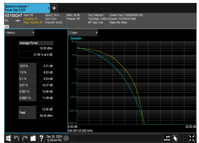
Band38-20MHz-16QAM-38000-100RB#0-PASS
