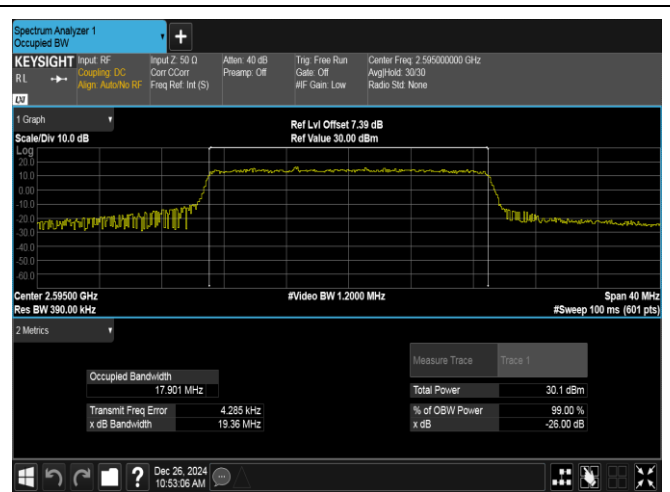
Band38-20MHz-QPSK-38000-100RB#0-PASS
