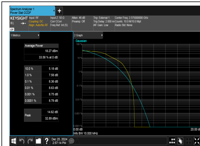
Band38-10MHz-QPSK-37800-1RB#0-PASS
