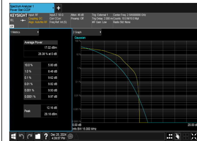
Band38-15MHz-16QAM-38000-1RB#0-PASS
