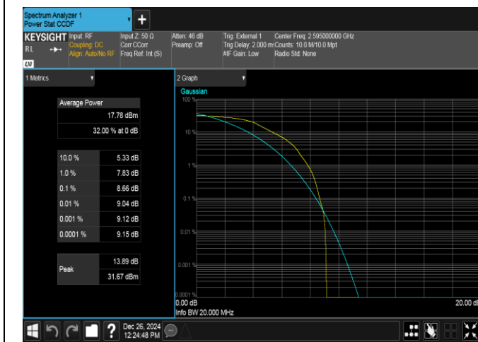
Band38-20MHz-QPSK-38000-1RB#0-PASS
