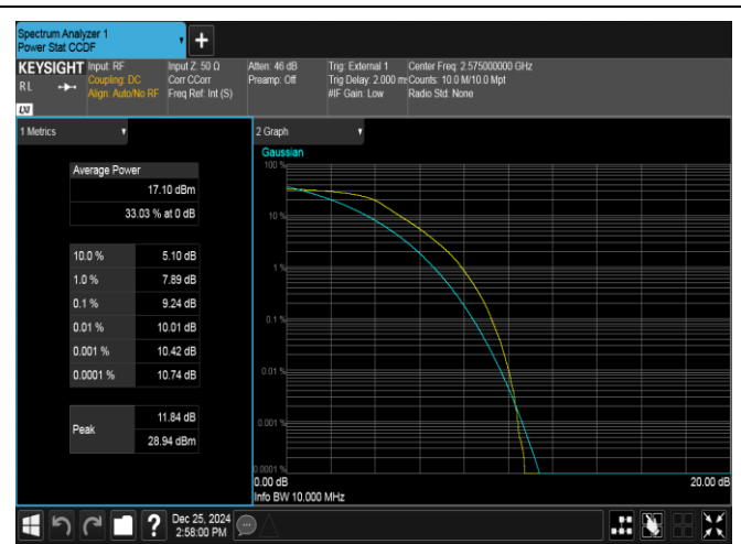
Band38-10MHz-QPSK-37800-50RB#0-PASS
