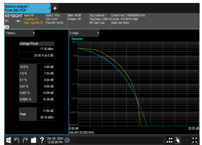
Band38-20MHz-QPSK-38000-100RB#0-PASS
