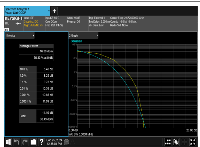
Band38-5MHz-16QAM-37775-25RB#0-PASS
