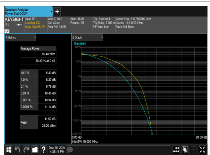
Band38-15MHz-16QAM-37825-75RB#0-PASS
