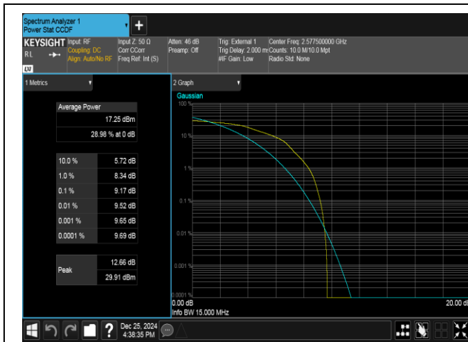
Band38-15MHz-16QAM-37825-1RB#0-PASS
