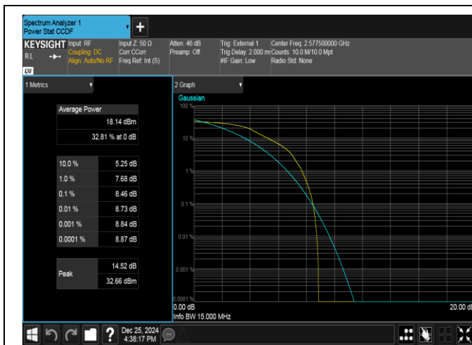
Band38-15MHz-QPSK-37825-1RB#0-PASS
