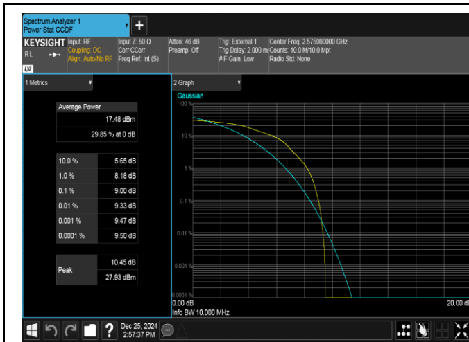
Band38-10MHz-16QAM-37800-1RB#0-PASS
