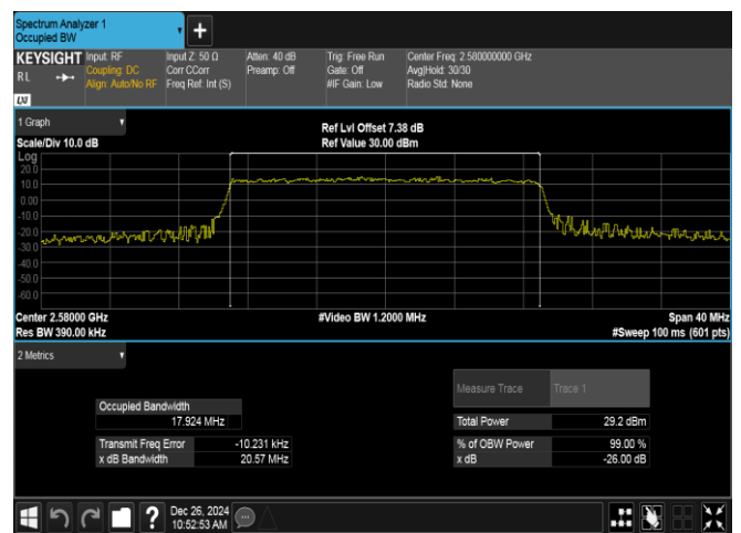
Band38-20MHz-16QAM-37850-100RB#0-PASS
