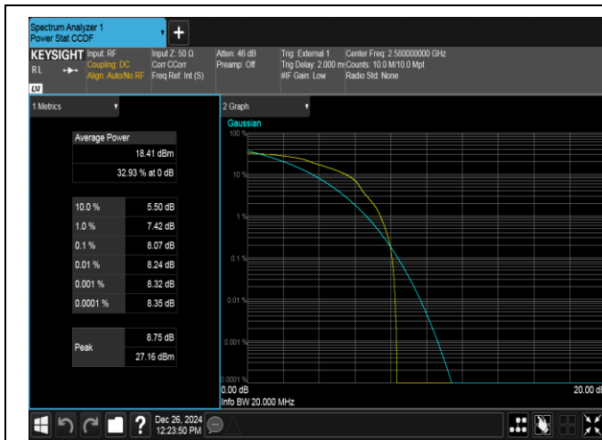
Band38-20MHz-16QAM-37850-1RB#0-PASS
