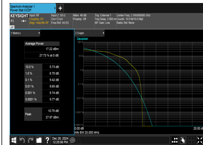
Band38-20MHz-16QAM-38000-1RB#0-PASS
