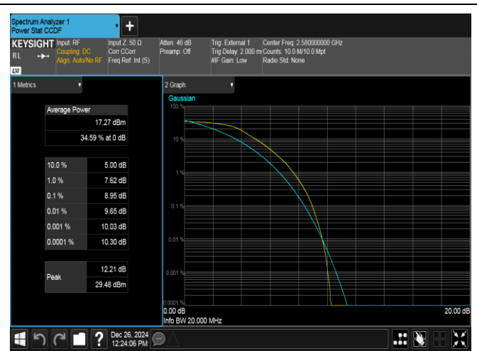
Band38-20MHz-QPSK-37850-100RB#0-PASS
