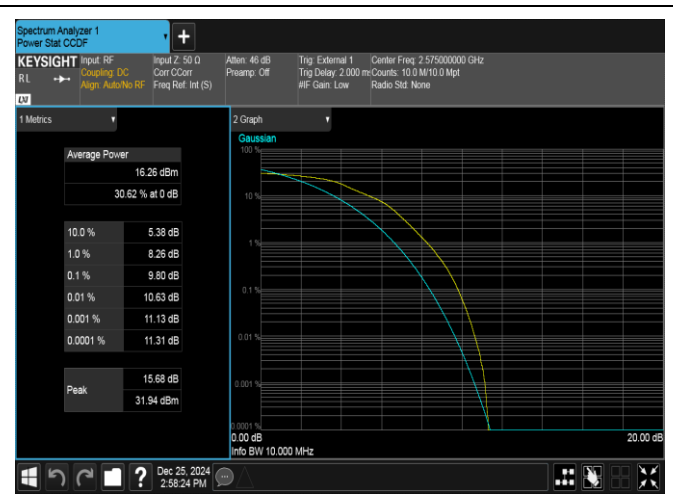
Band38-10MHz-16QAM-37800-50RB#0-PASS
