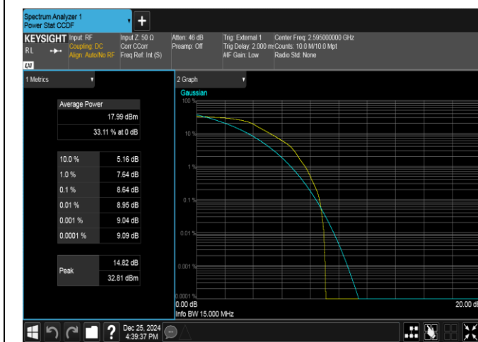
Band38-15MHz-QPSK-38000-1RB#0-PASS
