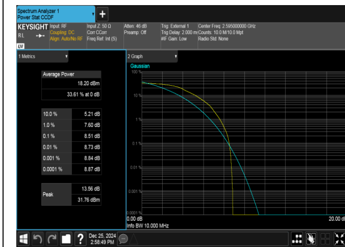
Band38-10MHz-QPSK-38000-1RB#0-PASS
