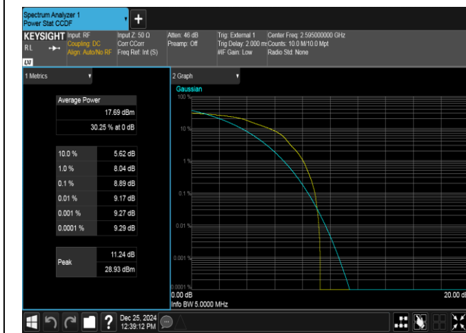
Band38-5MHz-16QAM-38000-1RB#0-PASS
