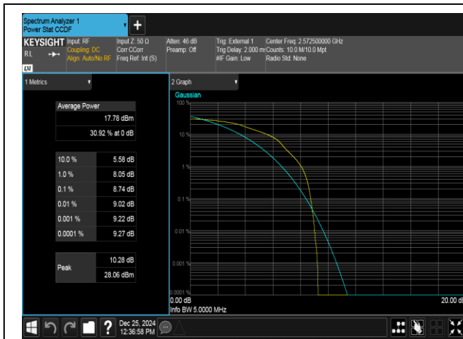
Band38-5MHz-16QAM-37775-1RB#0-PASS
