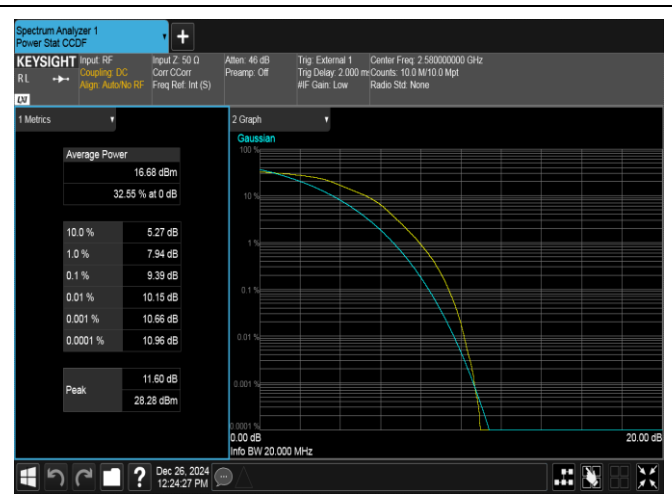
Band38-20MHz-16QAM-37850-100RB#0-PASS
