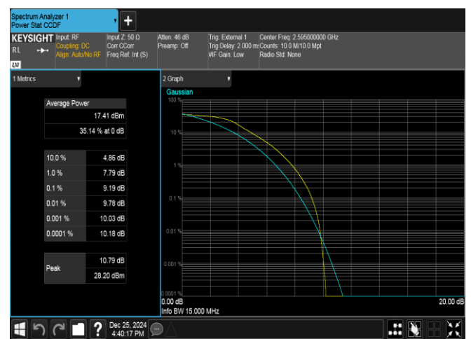
Band38-15MHz-QPSK-38000-75RB#0-PASS
