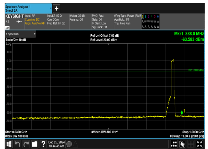
Band26(824-849)-15MHz-16QAM-26965-75RB#0-30~1000-PASS
