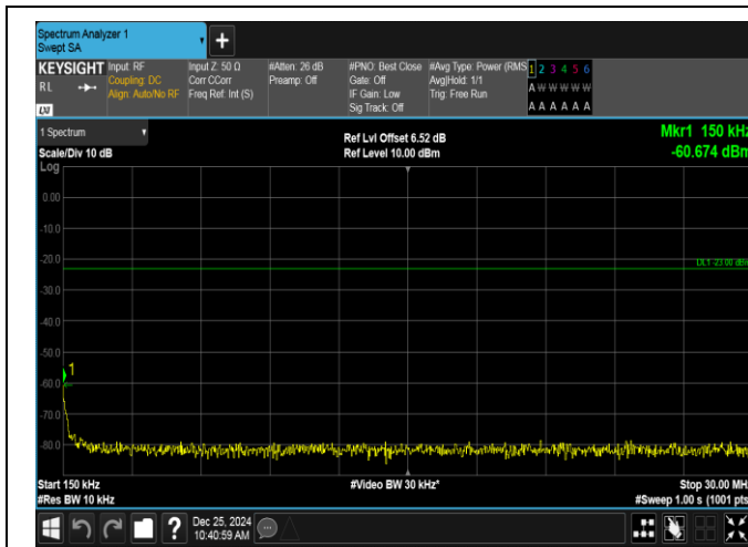
Band26(824-849)-15MHz-QPSK-26965-1RB#74-0.15~30-PASS
