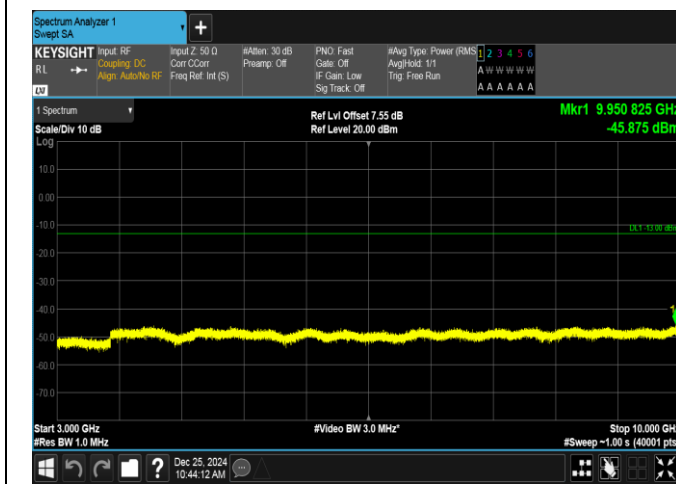
Band26(824-849)-15MHz-QPSK-26965-75RB#0-3000~10000-PASS
