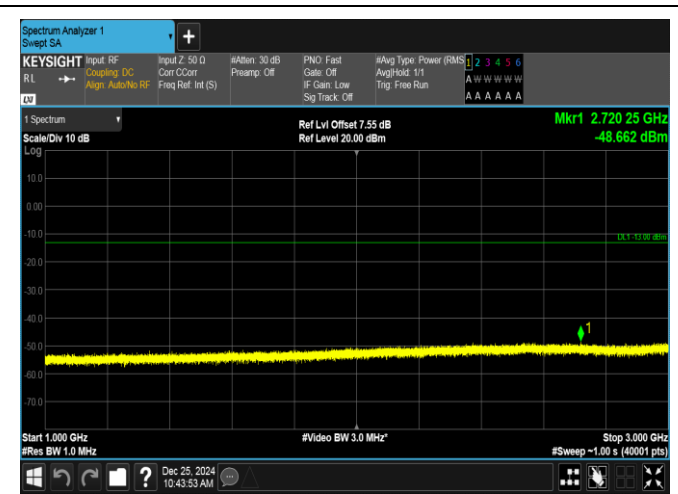
Band26(824-849)-15MHz-QPSK-26965-75RB#0-1000~3000-PASS
