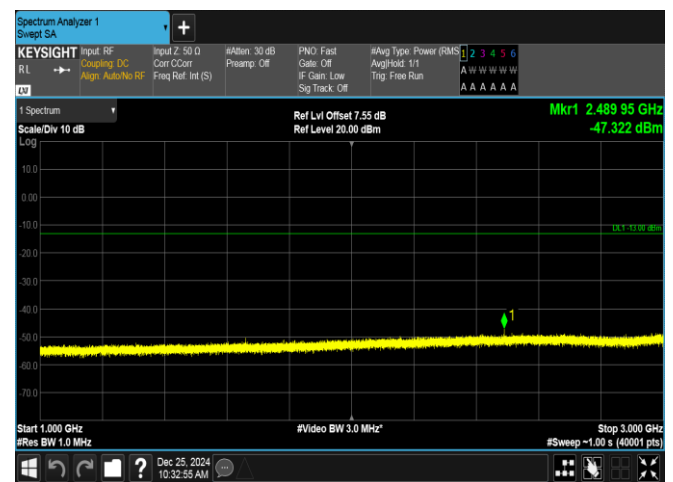
Band26(824-849)-15MHz-16QAM-26915-1RB#0-1000~3000-PASS
