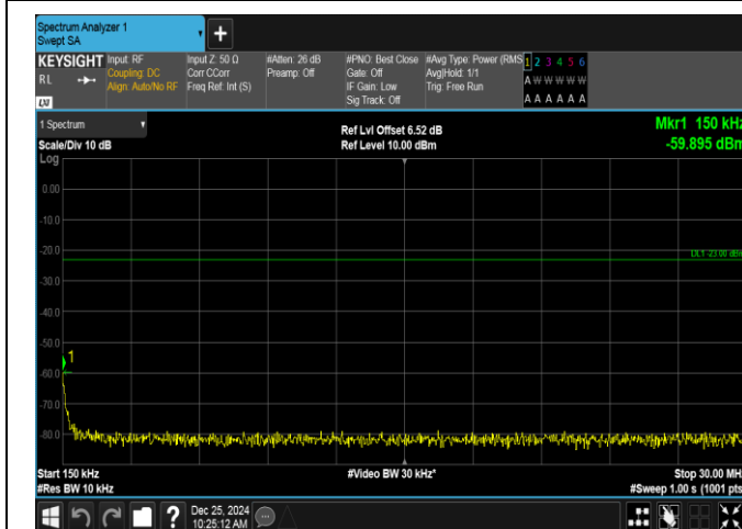
Band26(824-849)-15MHz-16QAM-26865-1RB#0-0.15~30-PASS
