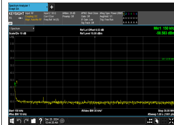
Band26(824-849)-15MHz-16QAM-26965-75RB#0-0.15~30-PASS
