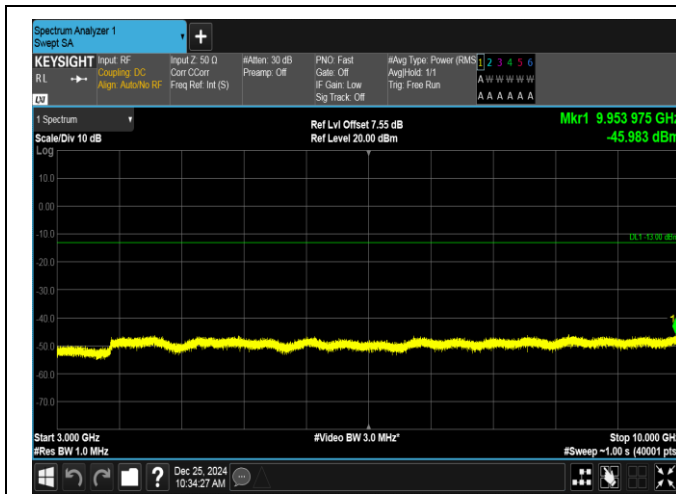
Band26(824-849)-15MHz-QPSK-26915-1RB#74-3000~10000-PASS
