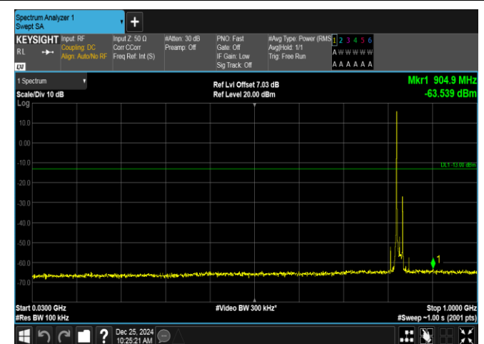
Band26(824-849)-15MHz-16QAM-26865-1RB#0-30~1000-PASS
