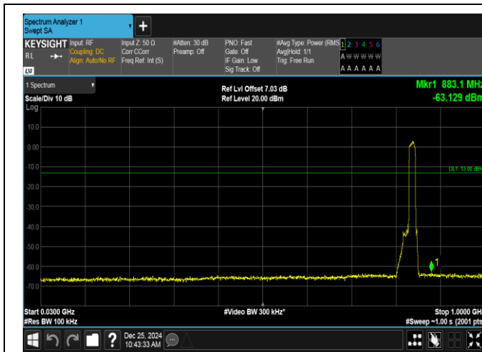
Band26(824-849)-15MHz-QPSK-26965-75RB#0-30~1000-PASS
