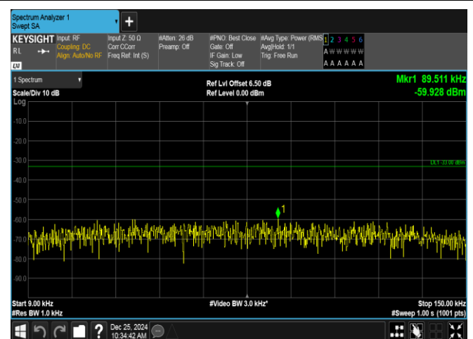
Band26(824-849)-15MHz-16QAM-26915-1RB#74-0.009~0.15-PASS
