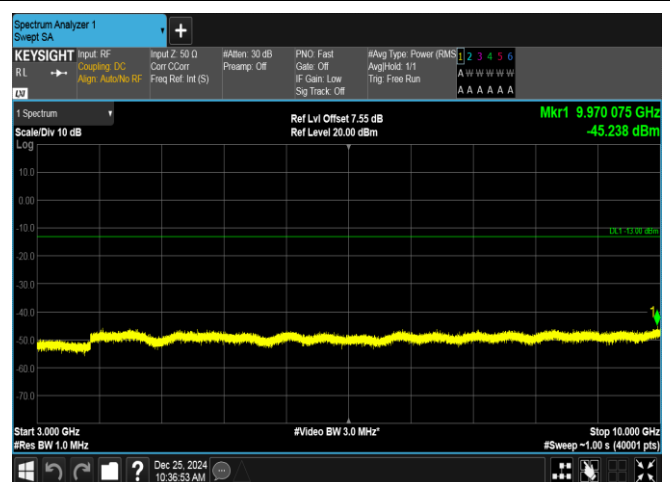
Band26(824-849)-15MHz-QPSK-26915-75RB#0-3000~10000-PASS
