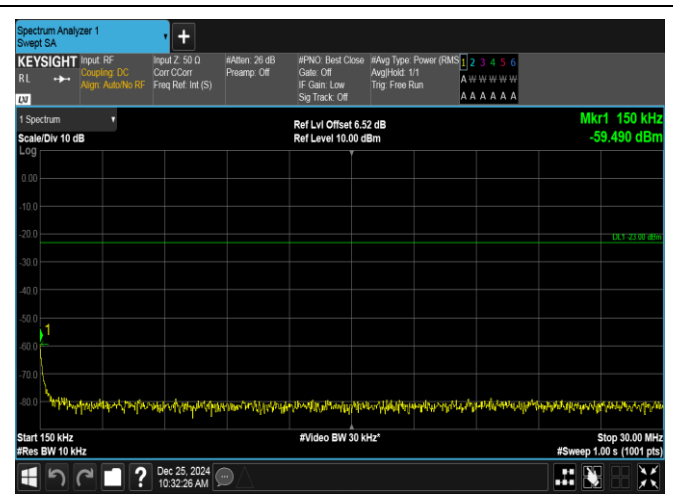
Band26(824-849)-15MHz-16QAM-26915-1RB#0-0.15~30-PASS
