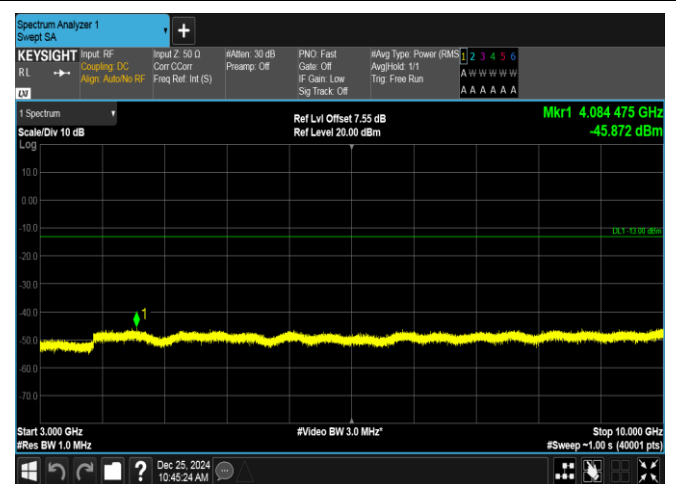
Band26(824-849)-15MHz-16QAM-26965-75RB#0-3000~10000-PASS
