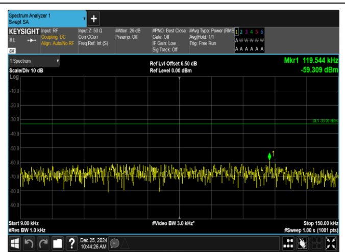
Band26(824-849)-15MHz-16QAM-26965-75RB#0-0.009~0.15-PASS
