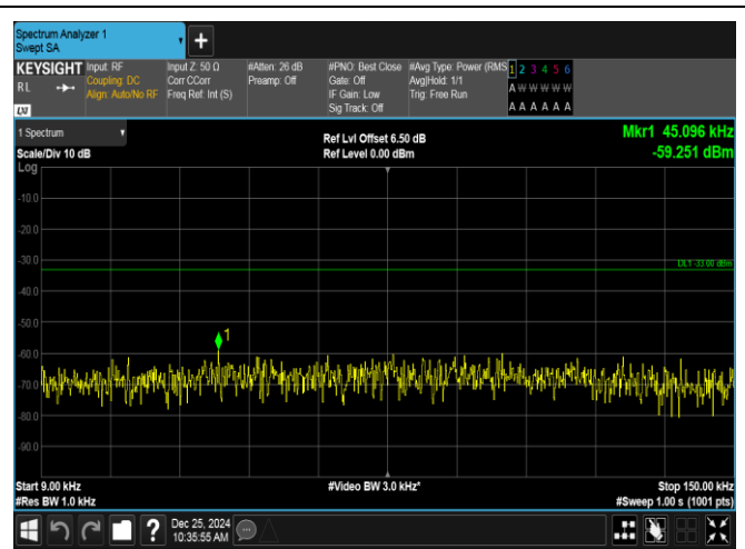
Band26(824-849)-15MHz-QPSK-26915-75RB#0-0.009~0.15-PASS
