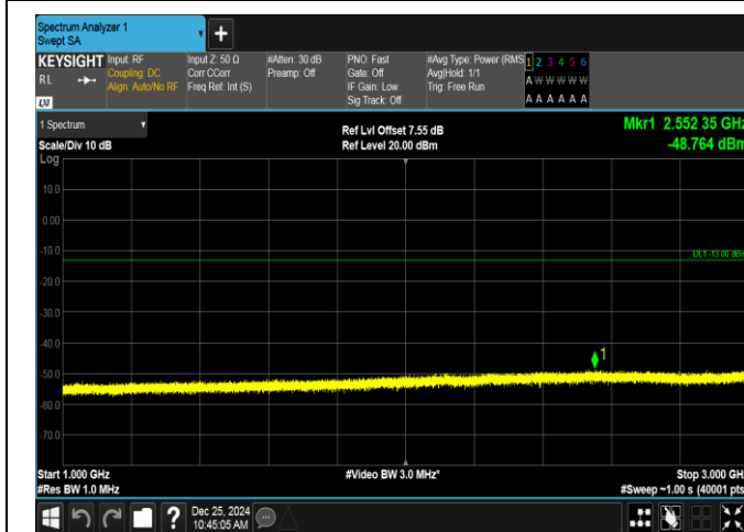
Band26(824-849)-15MHz-16QAM-26965-75RB#0-1000~3000-PASS
