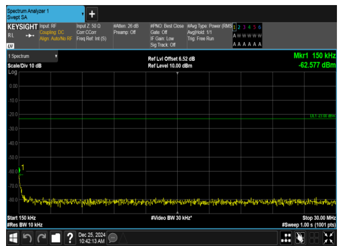
Band26(824-849)-15MHz-16QAM-26965-1RB#74-0.15~30-PASS
