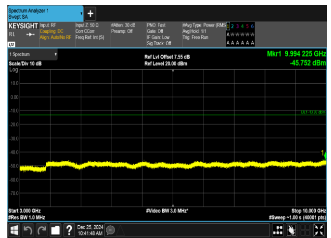
Band26(824-849)-15MHz-QPSK-26965-1RB#74-3000~10000-PASS
