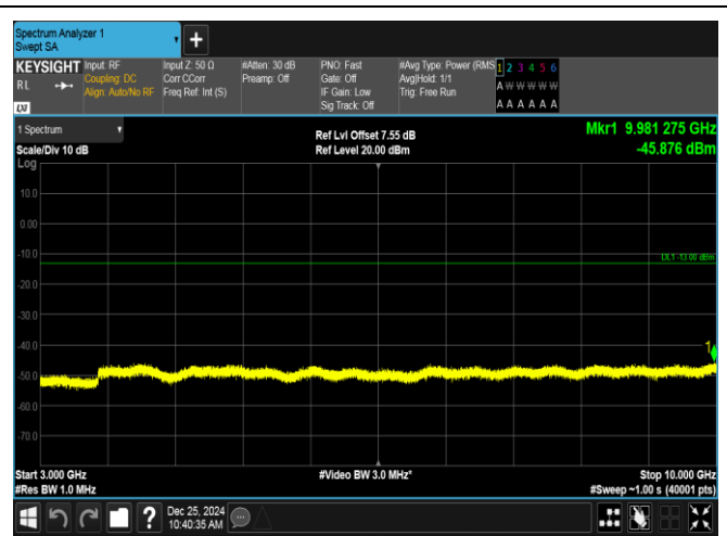
Band26(824-849)-15MHz-16QAM-26965-1RB#0-3000~10000-PASS
