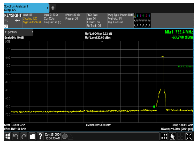
Band26(824-849)-15MHz-QPSK-26915-75RB#0-30~1000-PASS
