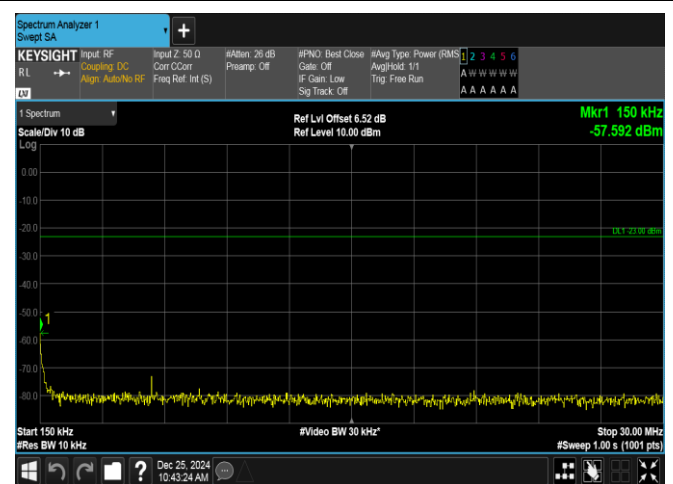
Band26(824-849)-15MHz-QPSK-26965-75RB#0-0.15~30-PASS
