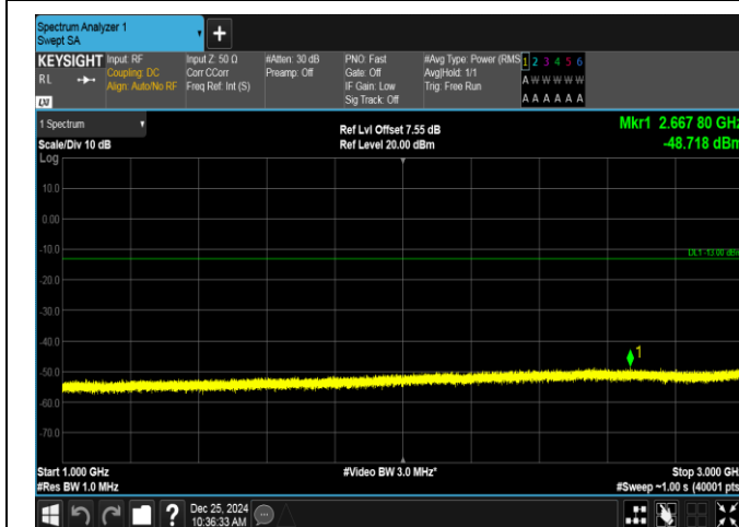
Band26(824-849)-15MHz-QPSK-26915-75RB#0-1000~3000-PASS
