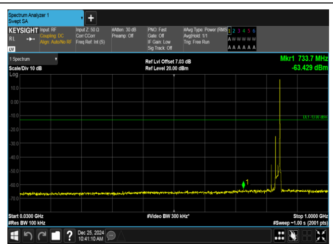
Band26(824-849)-15MHz-QPSK-26965-1RB#74-30~1000-PASS
