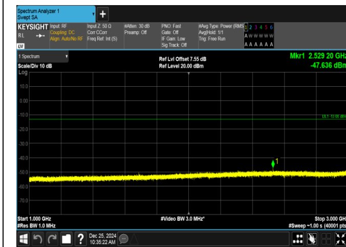
Band26(824-849)-15MHz-16QAM-26915-1RB#74-1000~3000-PASS
