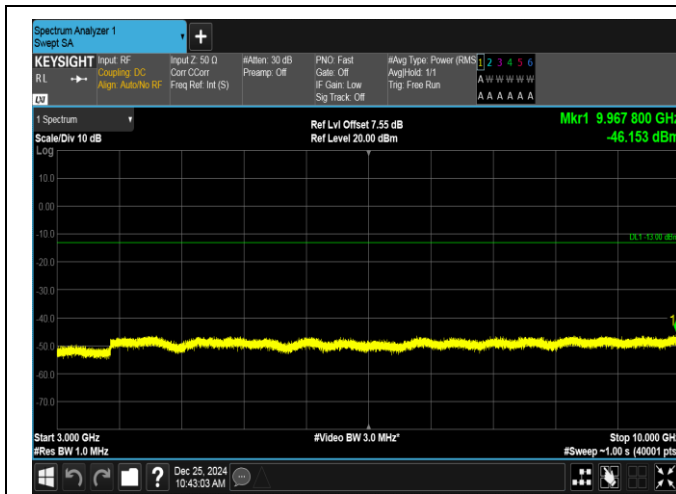
Band26(824-849)-15MHz-16QAM-26965-1RB#74-3000~10000-PASS
