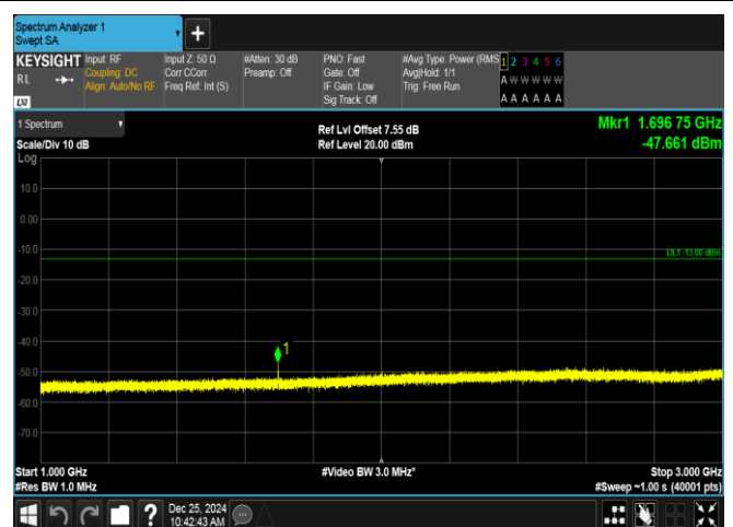
Band26(824-849)-15MHz-16QAM-26965-1RB#74-1000~3000-PASS
