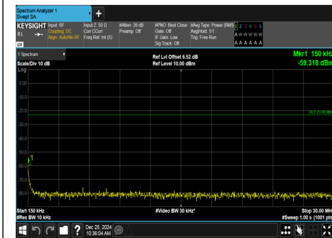
Band26(824-849)-15MHz-QPSK-26915-75RB#0-0.15~30-PASS
