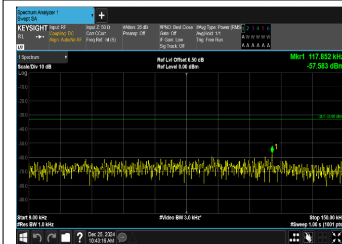
Band26(824-849)-15MHz-QPSK-26965-75RB#0-0.009~0.15-PASS
