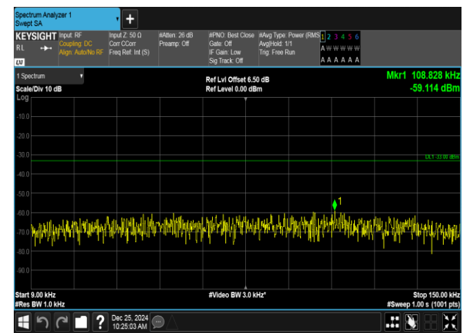
Band26(824-849)-15MHz-16QAM-26865-1RB#0-0.009~0.15-PASS
