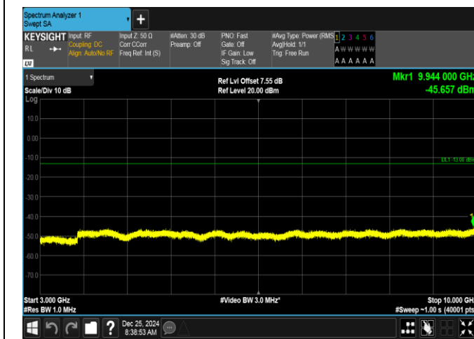
Band26(824-849)-3MHz-16QAM-26915-15RB#0-3000~10000-PASS
