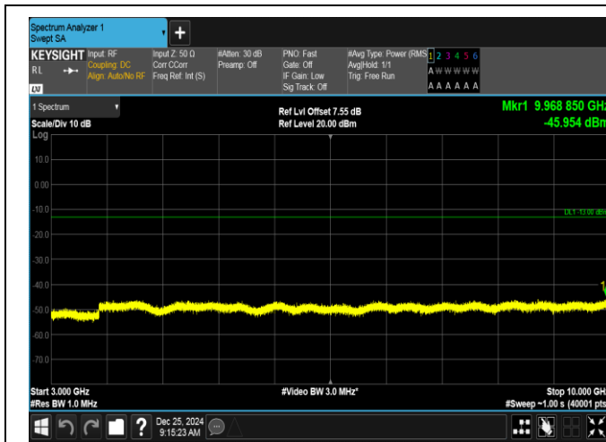
Band26(824-849)-5MHz-QPSK-26915-1RB#24-3000~10000-PASS
