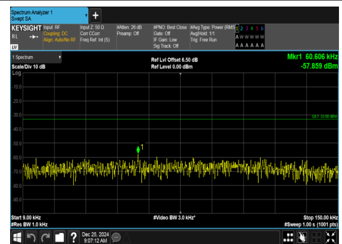
Band26(824-849)-5MHz-QPSK-26815-1RB#24-0.009~0.15-PASS
