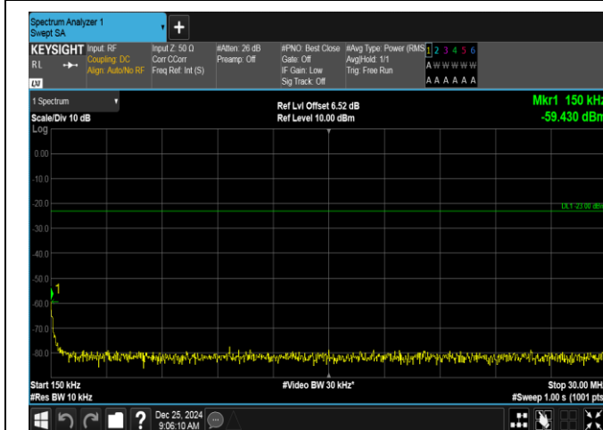
Band26(824-849)-5MHz-16QAM-26815-1RB#0-0.15~30-PASS
