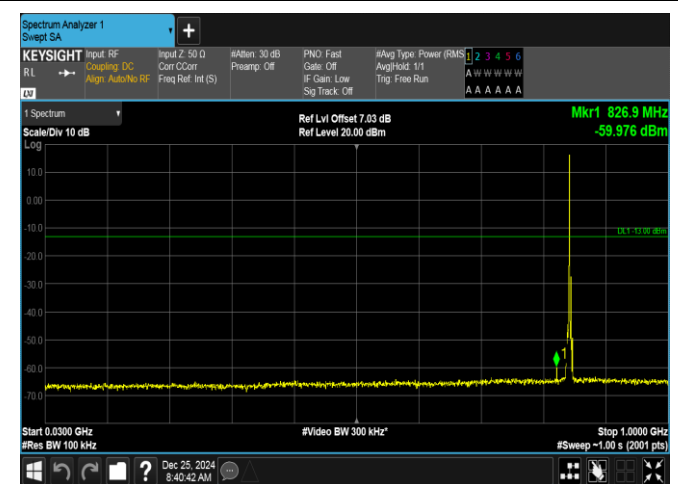
Band26(824-849)-3MHz-16QAM-27025-1RB#0-30~1000-PASS
