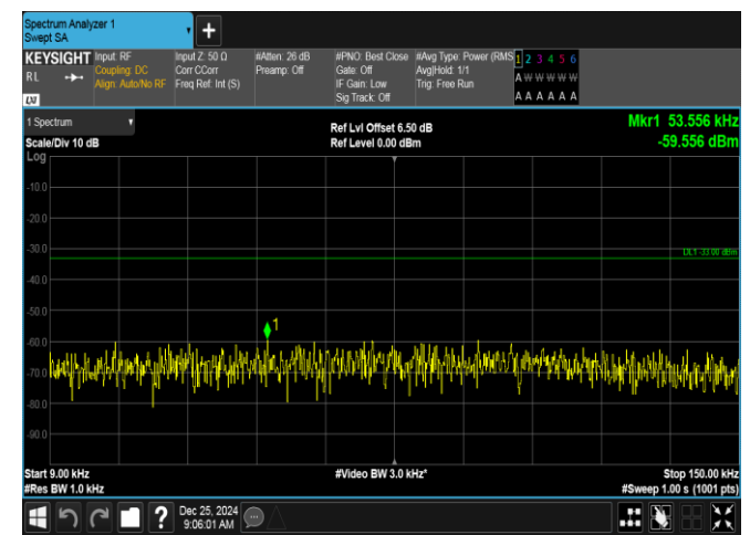
Band26(824-849)-5MHz-16QAM-26815-1RB#0-0.009~0.15-PASS
