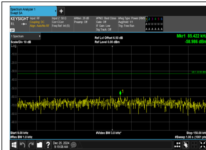
Band26(824-849)-5MHz-QPSK-27015-1RB#0-0.009~0.15-PASS
