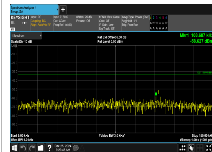
Band26(824-849)-5MHz-QPSK-27015-25RB#0-0.009~0.15-PASS
