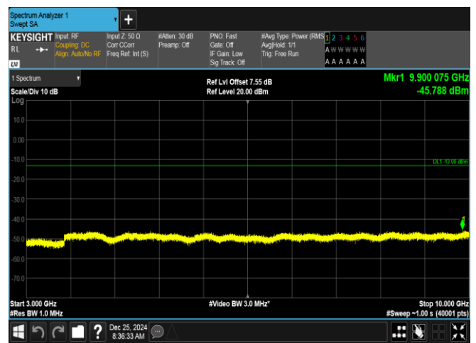
Band26(824-849)-3MHz-16QAM-26915-1RB#14-3000~10000-PASS
