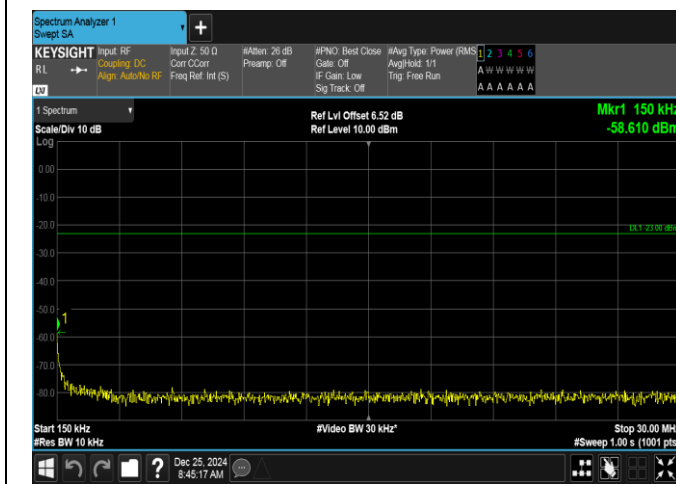
Band26(824-849)-3MHz-16QAM-27025-15RB#0-0.15~30-PASS
