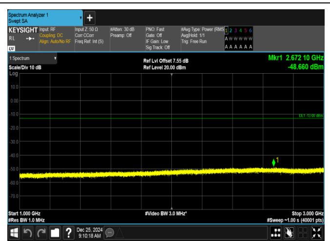
Band26(824-849)-5MHz-QPSK-26815-25RB#0-1000~3000-PASS
