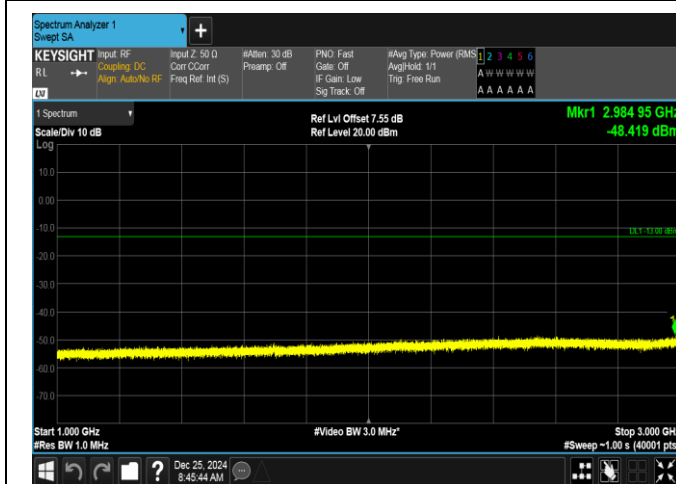
Band26(824-849)-3MHz-16QAM-27025-15RB#0-1000~3000-PASS
