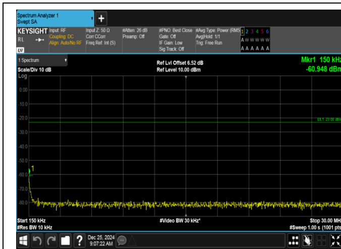
Band26(824-849)-5MHz-QPSK-26815-1RB#24-0.15~30-PASS
