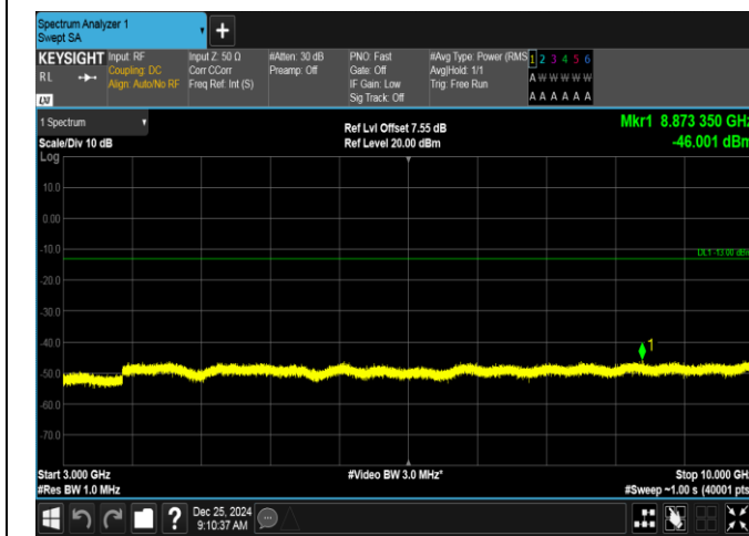
Band26(824-849)-5MHz-QPSK-26815-25RB#0-3000~10000-PASS
