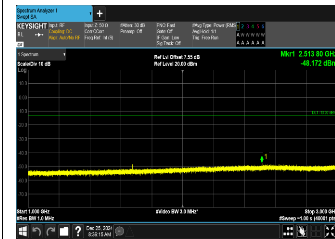
Band26(824-849)-3MHz-16QAM-26915-1RB#14-1000~3000-PASS
