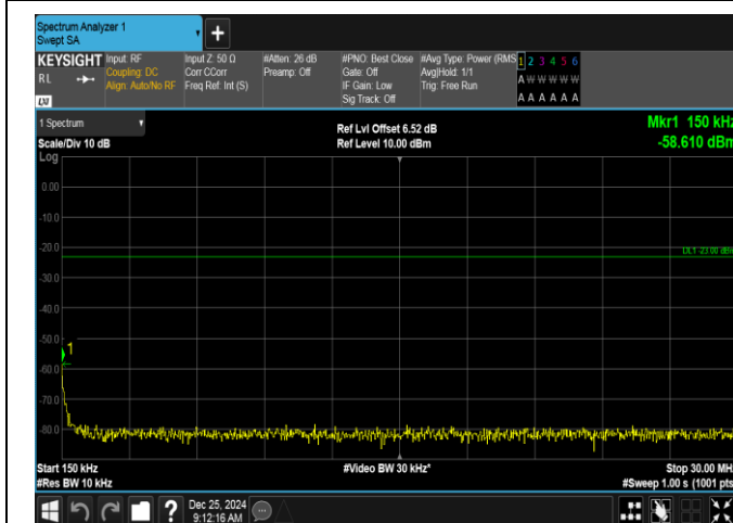
Band26(824-849)-5MHz-QPSK-26915-1RB#0-0.15~30-PASS
