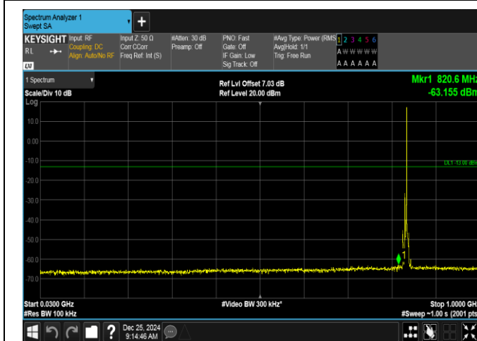
Band26(824-849)-5MHz-QPSK-26915-1RB#24-30~1000-PASS
