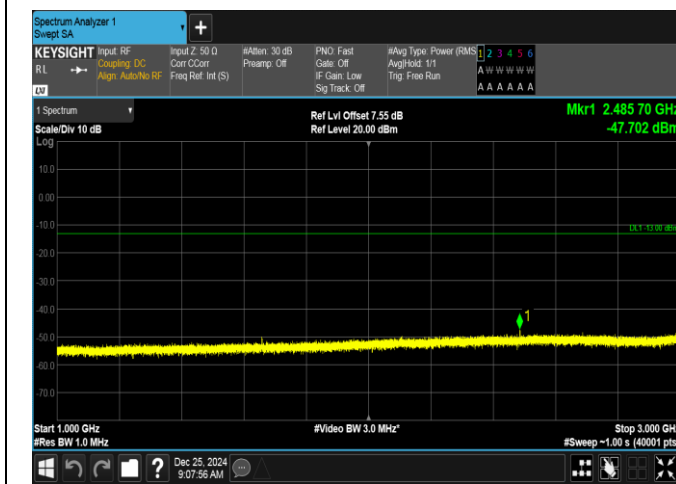
Band26(824-849)-5MHz-QPSK-26815-1RB#24-1000~3000-PASS
