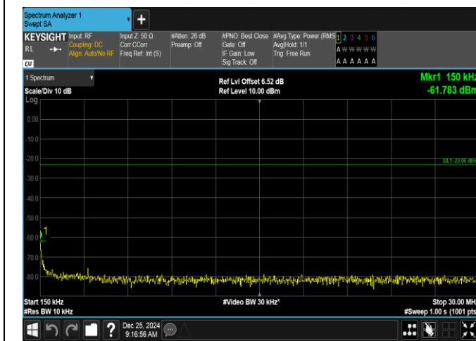
Band26(824-849)-5MHz-QPSK-26915-25RB#0-0.15~30-PASS
