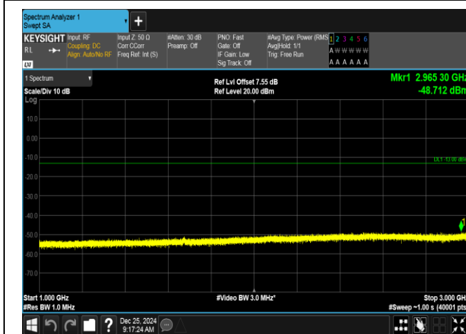
Band26(824-849)-5MHz-QPSK-26915-25RB#0-1000~3000-PASS
