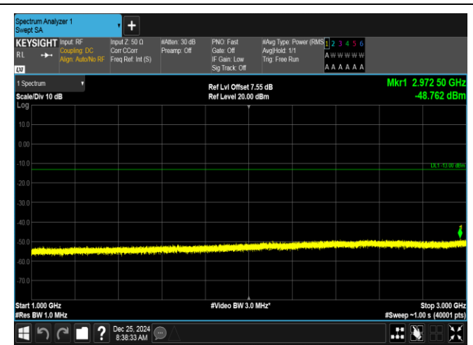
Band26(824-849)-3MHz-16QAM-26915-15RB#0-1000~3000-PASS
