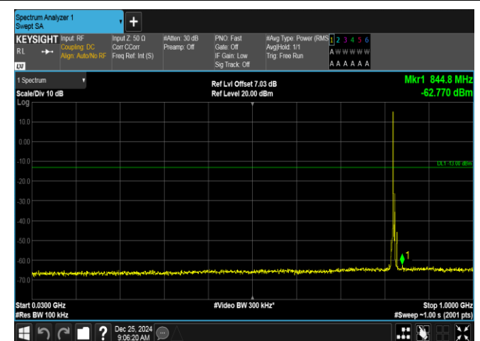
Band26(824-849)-5MHz-16QAM-26815-1RB#0-30~1000-PASS
