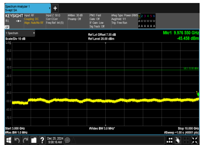
Band26(824-849)-5MHz-QPSK-26815-1RB#24-3000~10000-PASS
