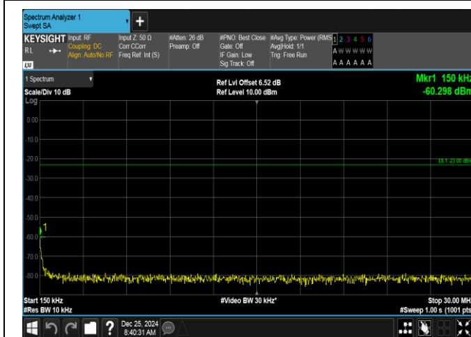
Band26(824-849)-3MHz-16QAM-27025-1RB#0-0.15~30-PASS
