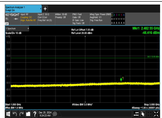
Band26(824-849)-5MHz-QPSK-27015-25RB#0-1000~3000-PASS
