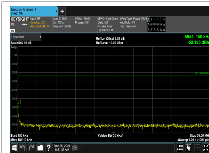
Band26(824-849)-5MHz-QPSK-27015-1RB#24-0.15~30-PASS
