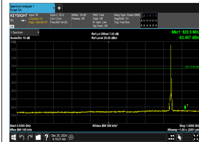
Band26(824-849)-5MHz-QPSK-27015-1RB#0-30~1000-PASS
