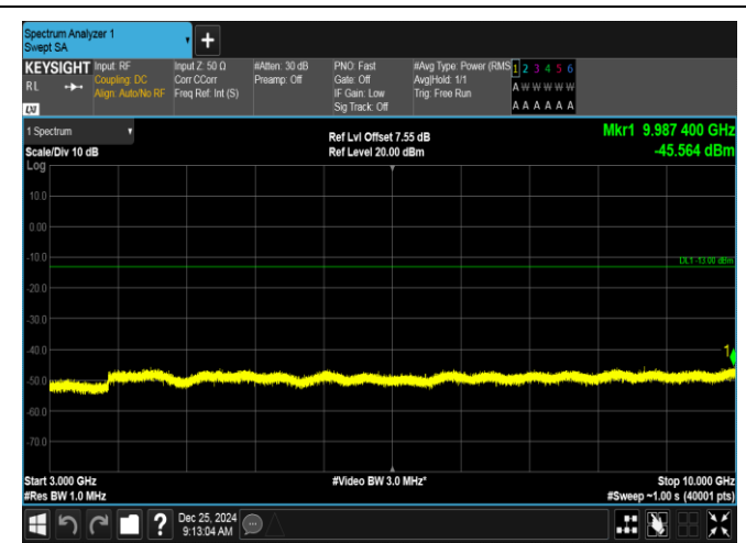
Band26(824-849)-5MHz-QPSK-26915-1RB#0-3000~10000-PASS
