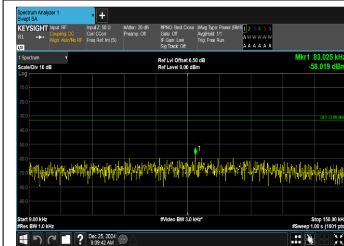
Band26(824-849)-5MHz-QPSK-26815-25RB#0-0.009~0.15-PASS
