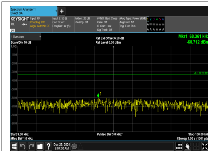
Band26(824-849)-5MHz-QPSK-26815-1RB#0-0.009~0.15-PASS
