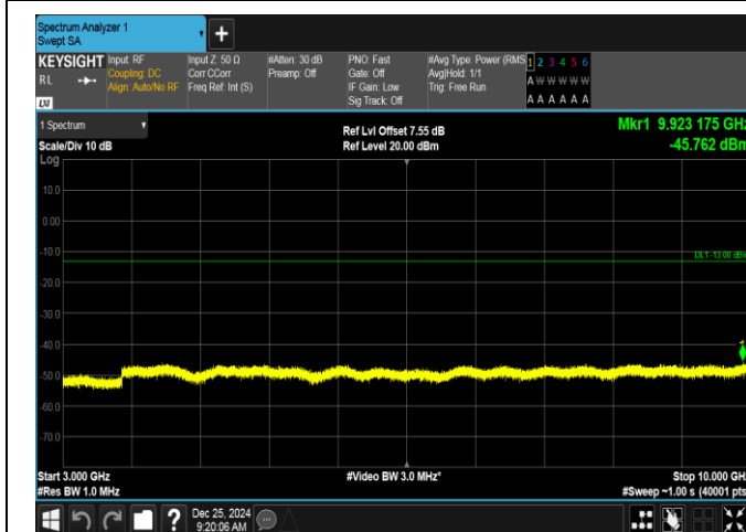
Band26(824-849)-5MHz-QPSK-27015-1RB#0-3000~10000-PASS
