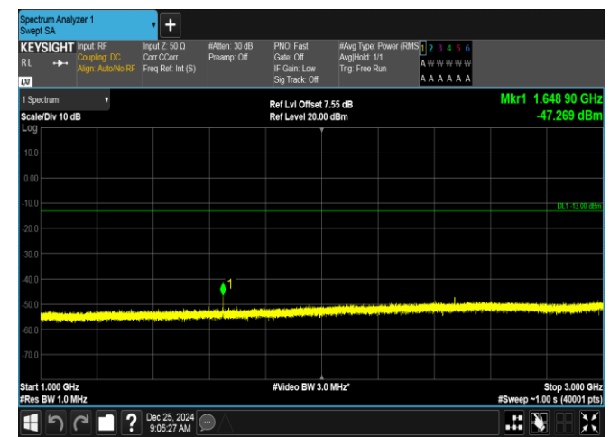
Band26(824-849)-5MHz-QPSK-26815-1RB#0-1000~3000-PASS
