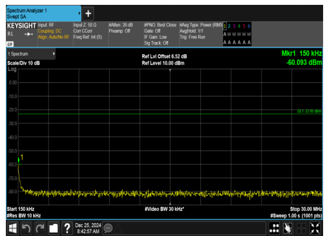
Band26(824-849)-3MHz-16QAM-27025-1RB#14-0.15~30-PASS
