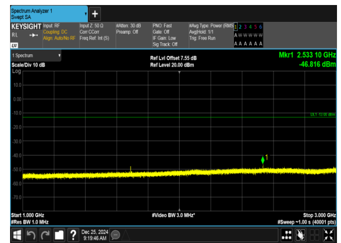
Band26(824-849)-5MHz-QPSK-27015-1RB#0-1000~3000-PASS
