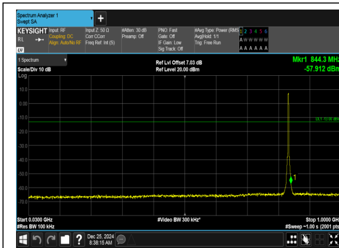
Band26(824-849)-3MHz-16QAM-26915-15RB#0-30~1000-PASS
