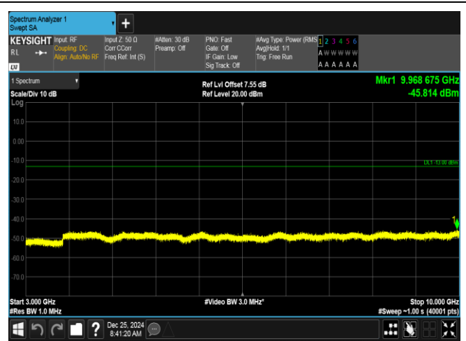
Band26(824-849)-3MHz-16QAM-27025-1RB#0-3000~10000-PASS
