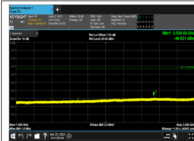
Band26(824-849)-3MHz-16QAM-27025-1RB#0-1000~3000-PASS
