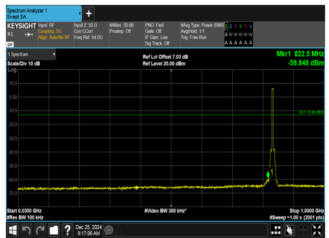
Band26(824-849)-5MHz-QPSK-26915-25RB#0-30~1000-PASS
