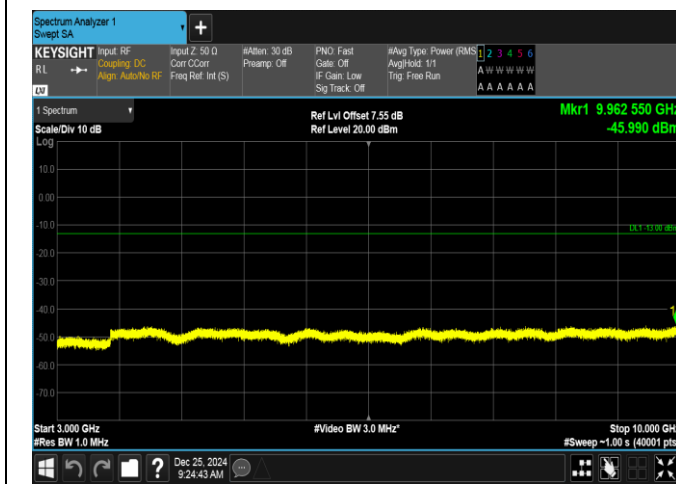
Band26(824-849)-5MHz-QPSK-27015-25RB#0-3000~10000-PASS
