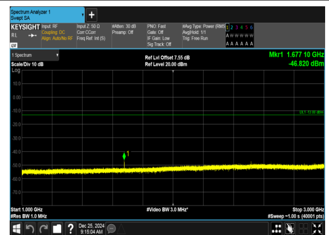
Band26(824-849)-5MHz-QPSK-26915-1RB#24-1000~3000-PASS
