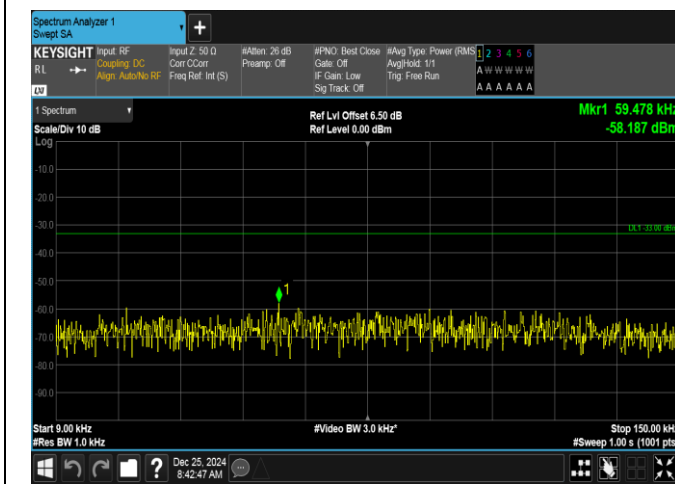
Band26(824-849)-3MHz-16QAM-27025-1RB#14-0.009~0.15-PASS
