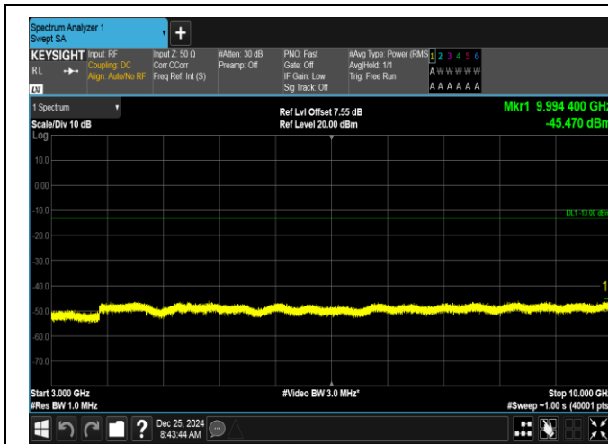
Band26(824-849)-3MHz-16QAM-27025-1RB#14-3000~10000-PASS
