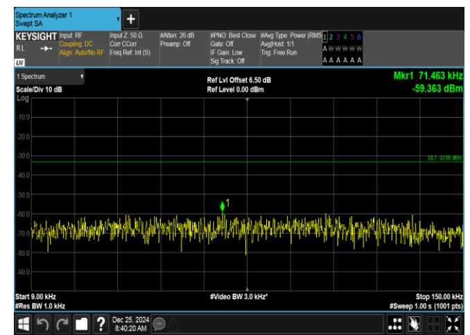
Band26(824-849)-3MHz-16QAM-27025-1RB#0-0.009~0.15-PASS
