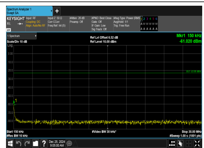
Band26(824-849)-5MHz-QPSK-26815-1RB#0-0.15~30-PASS
