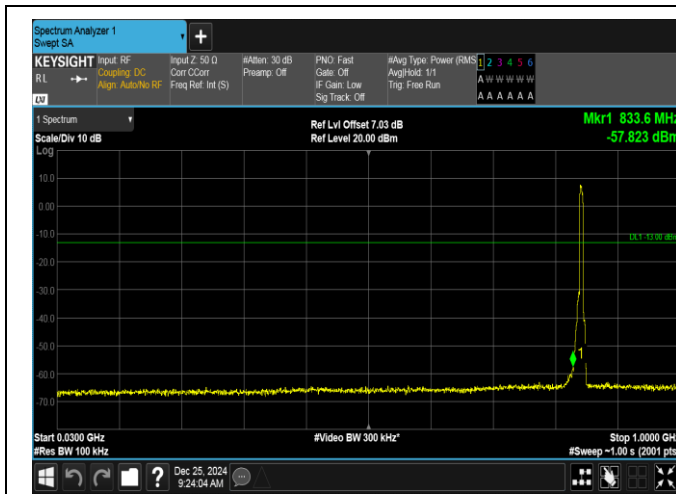
Band26(824-849)-5MHz-QPSK-27015-25RB#0-30~1000-PASS
