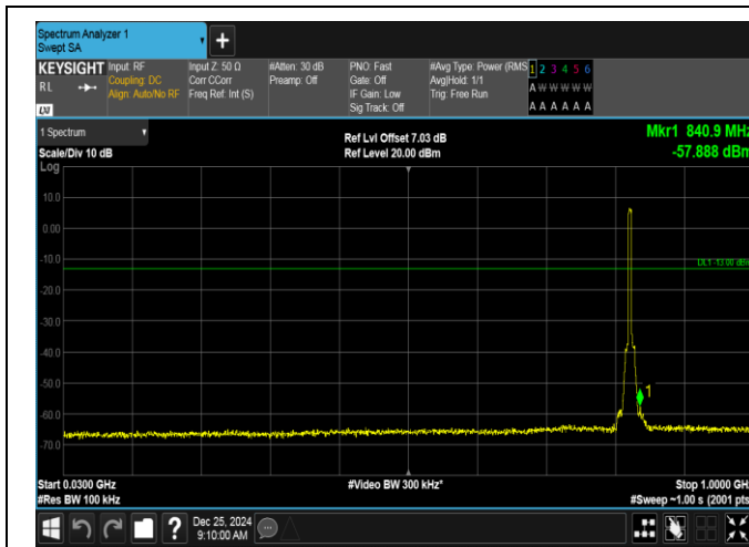
Band26(824-849)-5MHz-QPSK-26815-25RB#0-30~1000-PASS
