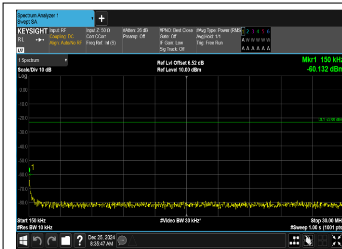
Band26(824-849)-3MHz-16QAM-26915-1RB#14-0.15~30-PASS
