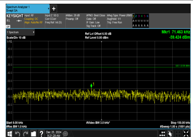
Band26(824-849)-5MHz-QPSK-27015-1RB#24-0.009~0.15-PASS
