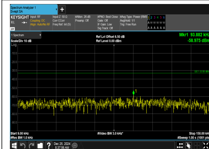
Band26(824-849)-3MHz-16QAM-26915-15RB#0-0.009~0.15-PASS
