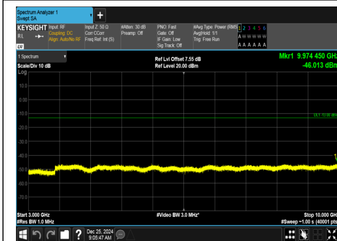
Band26(824-849)-5MHz-QPSK-26815-1RB#0-3000~10000-PASS
