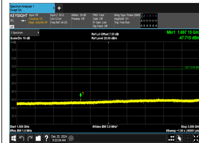
Band26(824-849)-5MHz-QPSK-27015-1RB#24-1000~3000-PASS
