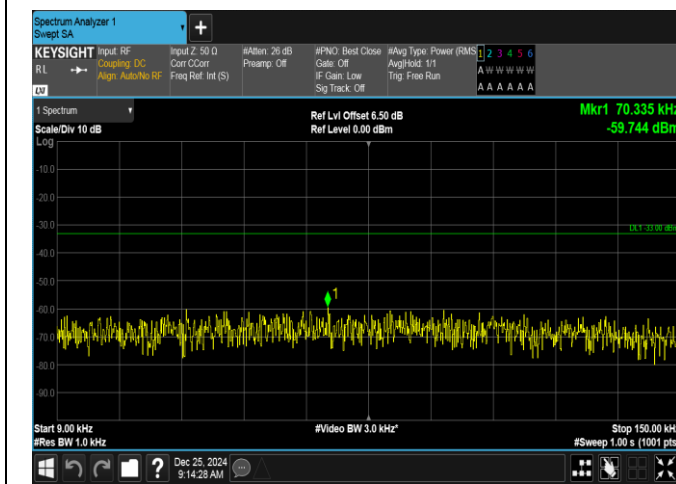
Band26(824-849)-5MHz-QPSK-26915-1RB#24-0.009~0.15-PASS
