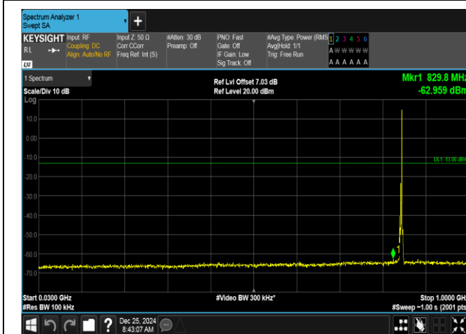
Band26(824-849)-3MHz-16QAM-27025-1RB#14-30~1000-PASS
