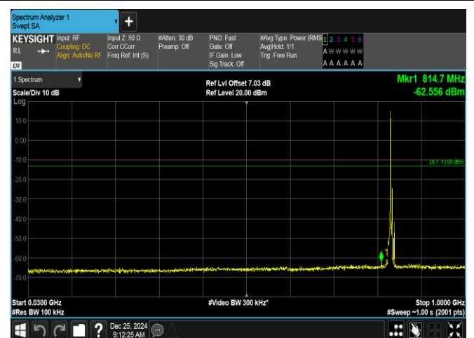
Band26(824-849)-5MHz-QPSK-26915-1RB#0-30~1000-PASS
