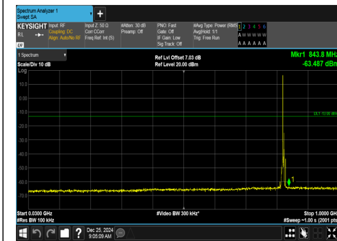
Band26(824-849)-5MHz-QPSK-26815-1RB#0-30~1000-PASS
