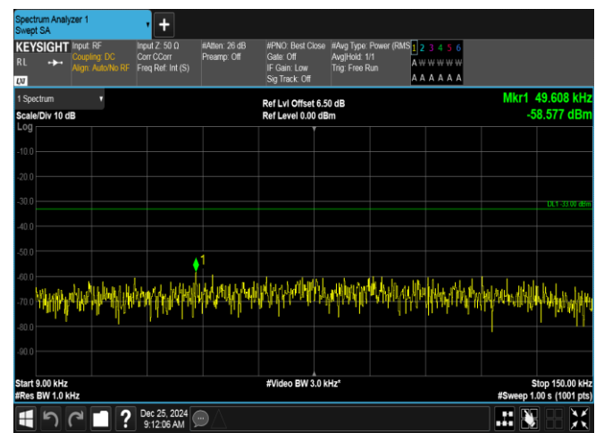
Band26(824-849)-5MHz-QPSK-26915-1RB#0-0.009~0.15-PASS
