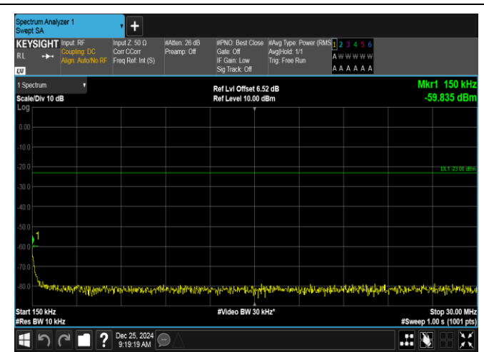
Band26(824-849)-5MHz-QPSK-27015-1RB#0-0.15~30-PASS
