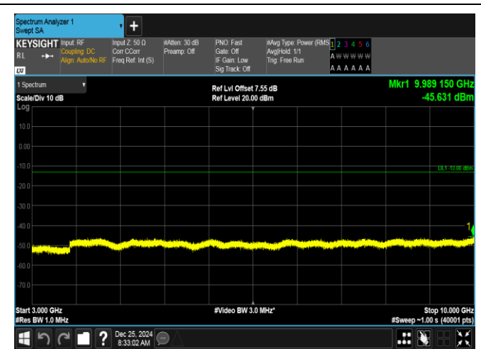
Band26(824-849)-3MHz-QPSK-26915-1RB#0-3000~10000-PASS
