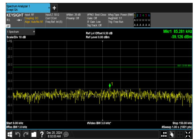
Band26(824-849)-3MHz-QPSK-26915-1RB#0-0.009~0.15-PASS
