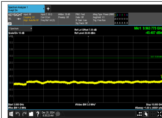
Band26(824-849)-3MHz-QPSK-26915-1RB#14-3000~10000-PASS
