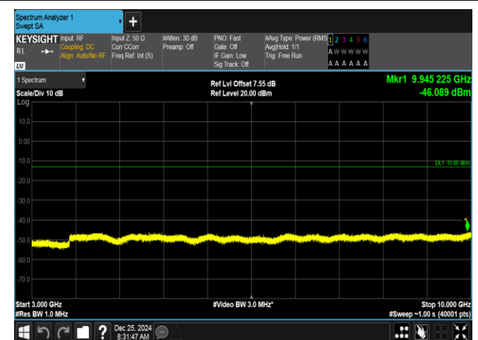
Band26(824-849)-3MHz-16QAM-26805-15RB#0-3000~10000-PASS
