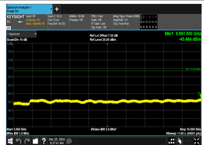
Band26(824-849)-3MHz-QPSK-26915-15RB#0-3000~10000-PASS
