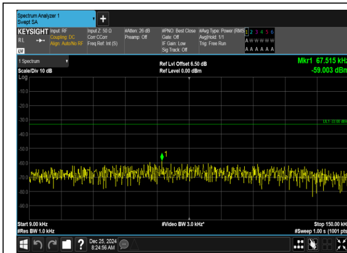
Band26(824-849)-3MHz-QPSK-26805-1RB#0-0.009~0.15-PASS
