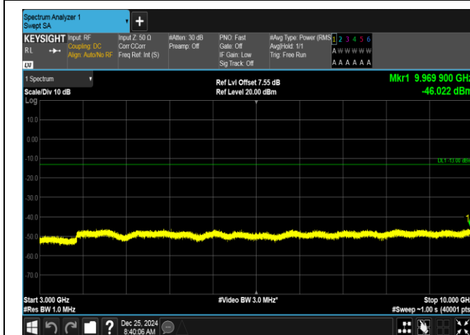
Band26(824-849)-3MHz-QPSK-27025-1RB#0-3000~10000-PASS
