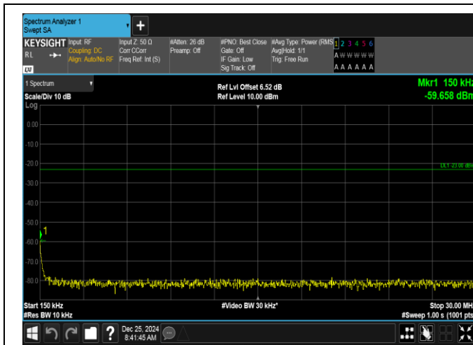
Band26(824-849)-3MHz-QPSK-27025-1RB#14-0.15~30-PASS
