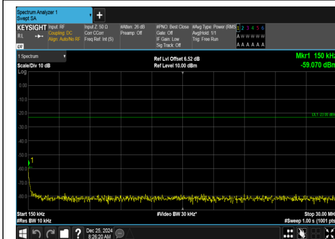
Band26(824-849)-3MHz-16QAM-26805-1RB#0-0.15~30-PASS
