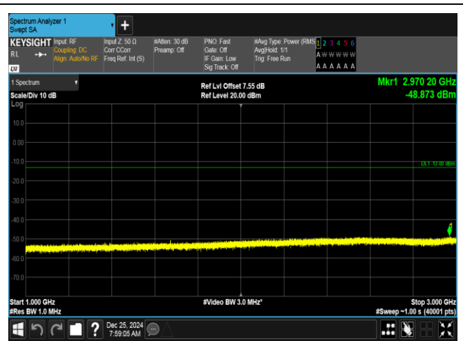
Band26(824-849)-1.4MHz-16QAM-26915-6RB#0-1000~3000-PASS
