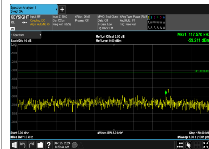
Band26(824-849)-3MHz-QPSK-26805-15RB#0-0.009~0.15-PASS
