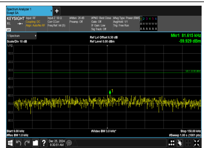
Band26(824-849)-3MHz-16QAM-26805-15RB#0-0.009~0.15-PASS
