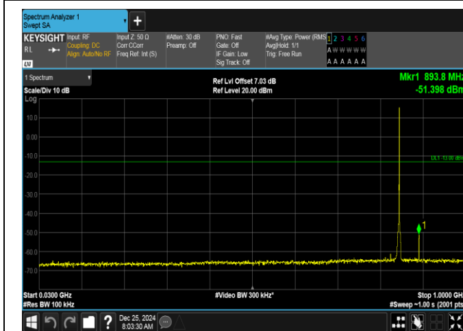
Band26(824-849)-1.4MHz-16QAM-27033-1RB#5-30~1000-PASS
