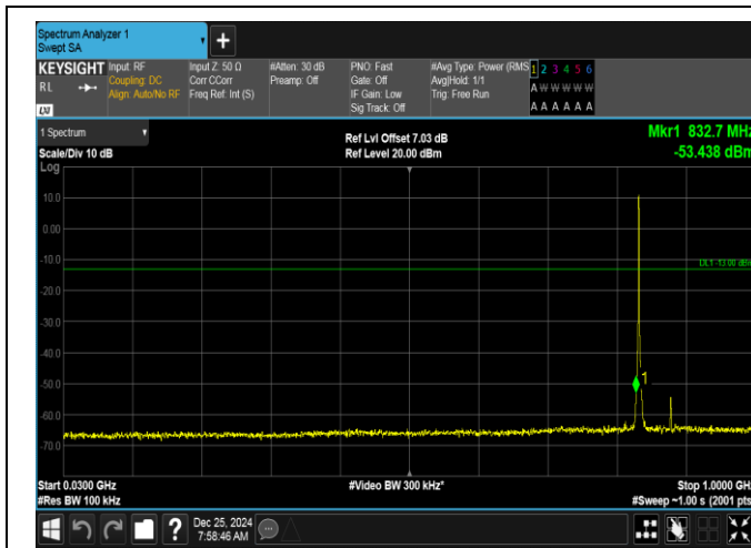
Band26(824-849)-1.4MHz-16QAM-26915-6RB#0-30~1000-PASS
