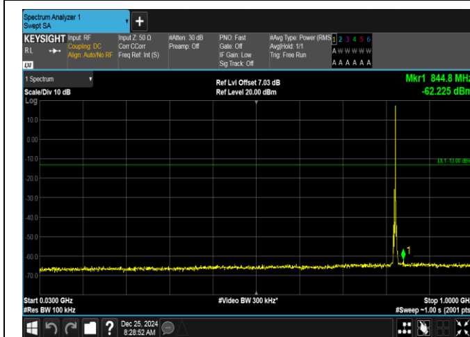
Band26(824-849)-3MHz-16QAM-26805-1RB#14-30~1000-PASS
