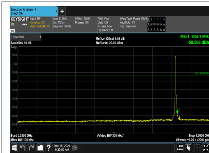
Band26(824-849)-3MHz-QPSK-26805-15RB#0-30~1000-PASS
