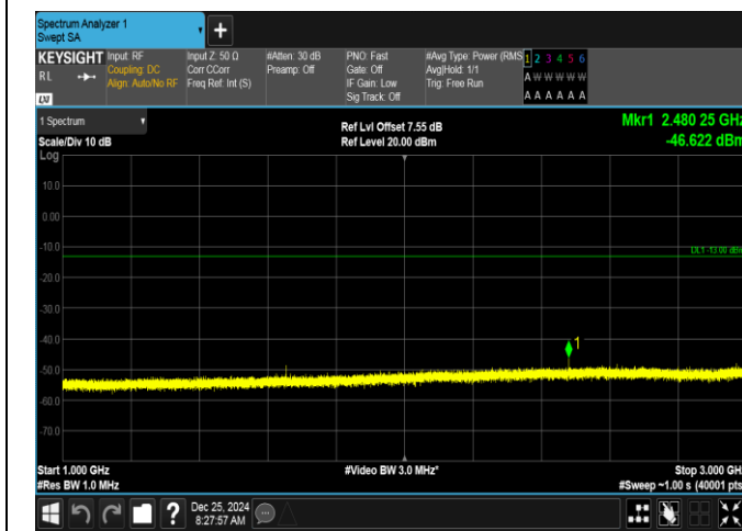
Band26(824-849)-3MHz-QPSK-26805-1RB#14-1000~3000-PASS
