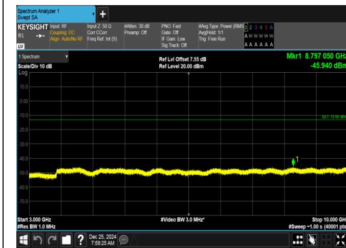
Band26(824-849)-1.4MHz-16QAM-26915-6RB#0-3000~10000-PASS
