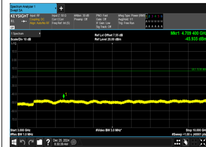
Band26(824-849)-3MHz-QPSK-26805-15RB#0-3000~10000-PASS
