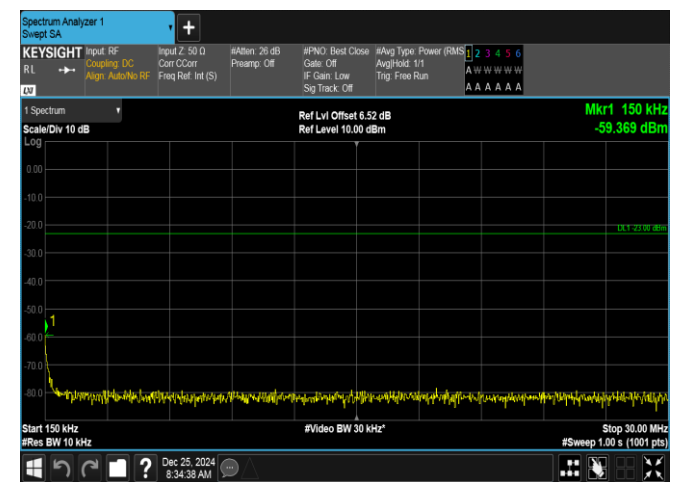
Band26(824-849)-3MHz-QPSK-26915-1RB#14-0.15~30-PASS
