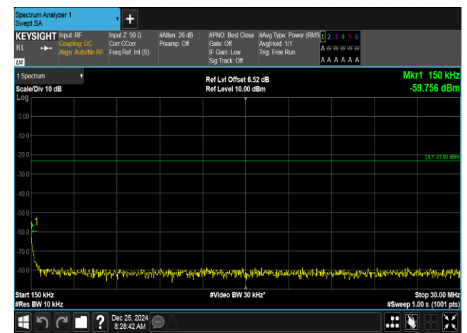
Band26(824-849)-3MHz-16QAM-26805-1RB#14-0.15~30-PASS
