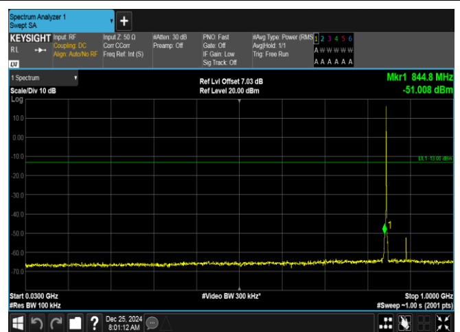
Band26(824-849)-1.4MHz-16QAM-27033-1RB#0-30~1000-PASS
