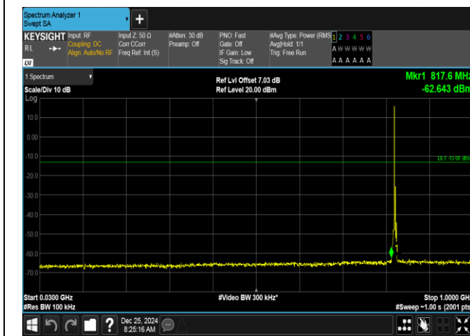
Band26(824-849)-3MHz-QPSK-26805-1RB#0-30~1000-PASS
