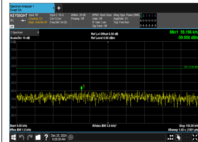
Band26(824-849)-3MHz-16QAM-26805-1RB#14-0.009~0.15-PASS
