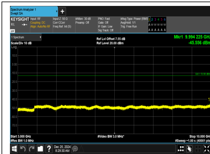
Band26(824-849)-3MHz-16QAM-26805-1RB#14-3000~10000-PASS
