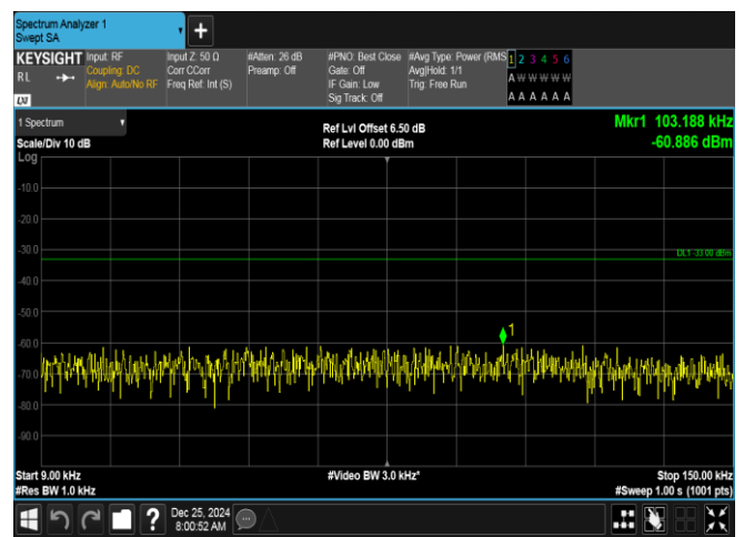
Band26(824-849)-1.4MHz-16QAM-27033-1RB#0-0.009~0.15-PASS
