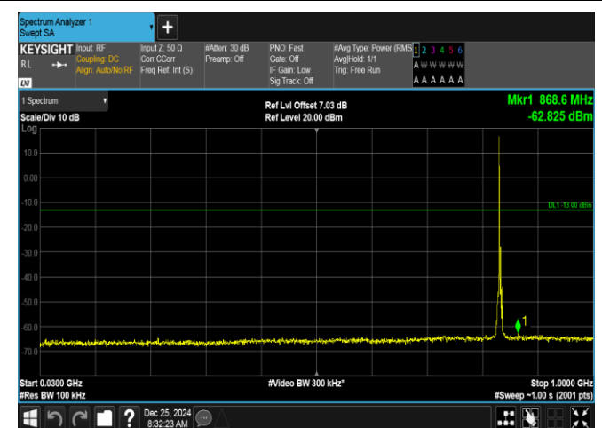
Band26(824-849)-3MHz-QPSK-26915-1RB#0-30~1000-PASS
