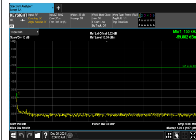
Band26(824-849)-3MHz-QPSK-26915-15RB#0-0.15~30-PASS
