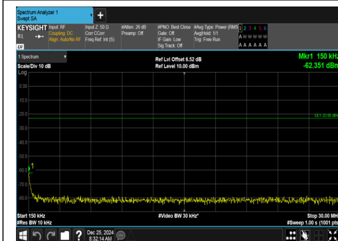
Band26(824-849)-3MHz-QPSK-26915-1RB#0-0.15~30-PASS
