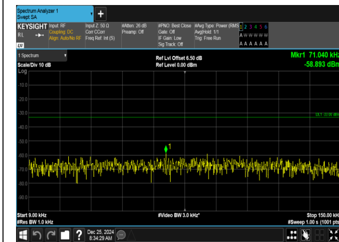
Band26(824-849)-3MHz-QPSK-26915-1RB#14-0.009~0.15-PASS
