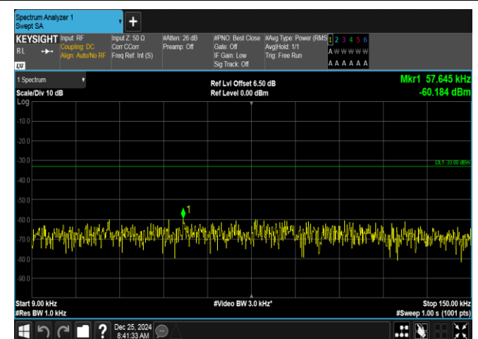
Band26(824-849)-3MHz-QPSK-27025-1RB#14-0.009~0.15-PASS
