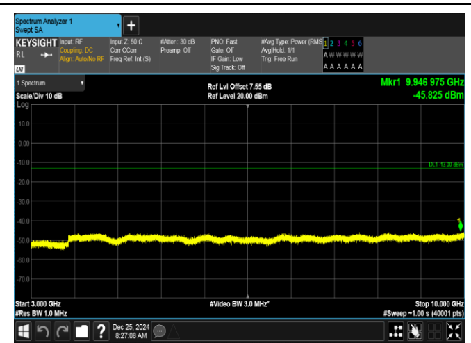
Band26(824-849)-3MHz-16QAM-26805-1RB#0-3000~10000-PASS
