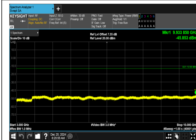
Band26(824-849)-3MHz-QPSK-26805-1RB#0-3000~10000-PASS
