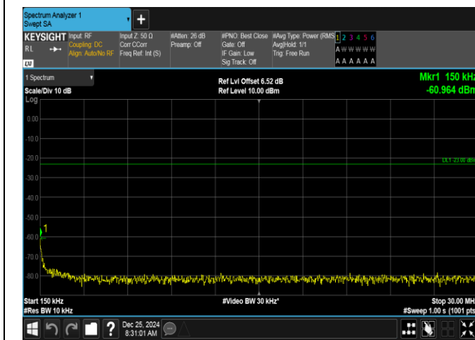
Band26(824-849)-3MHz-16QAM-26805-15RB#0-0.15~30-PASS
