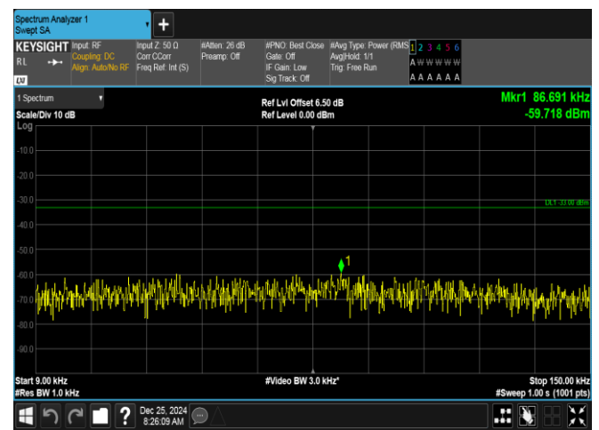
Band26(824-849)-3MHz-16QAM-26805-1RB#0-0.009~0.15-PASS
