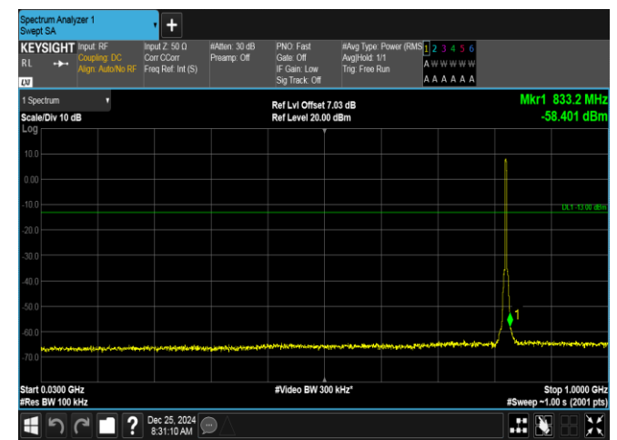
Band26(824-849)-3MHz-16QAM-26805-15RB#0-30~1000-PASS
