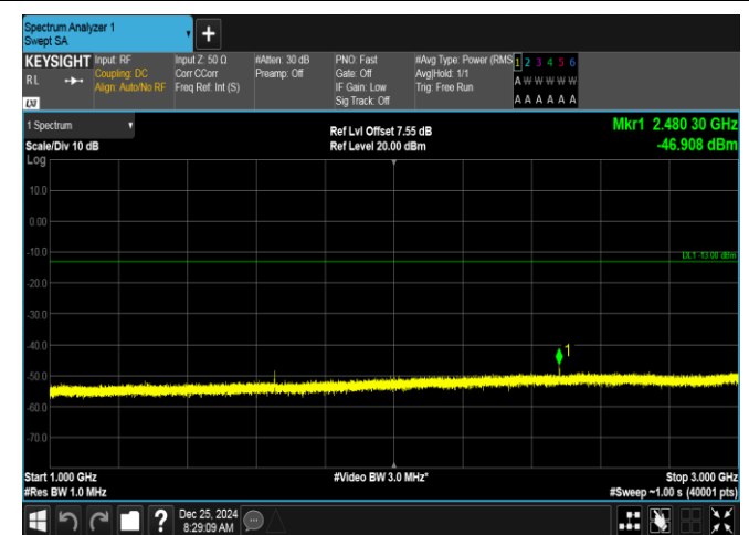
Band26(824-849)-3MHz-16QAM-26805-1RB#14-1000~3000-PASS
