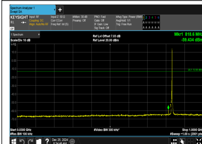
Band26(824-849)-3MHz-QPSK-26915-1RB#14-30~1000-PASS
