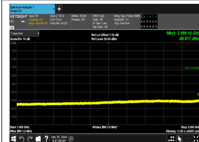
Band26(824-849)-3MHz-16QAM-26805-15RB#0-1000~3000-PASS
