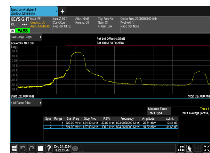
Band26(824-849)-3MHz-16QAM-26805-1RB#0-PASS
