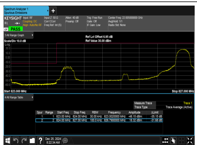
Band26(824-849)-3MHz-16QAM-26805-1RB#14-PASS
