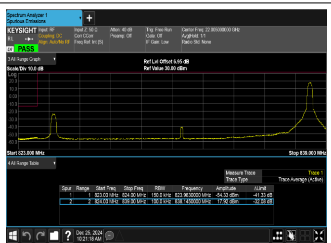
Band26(824-849)-15MHz-16QAM-26865-1RB#74-PASS
