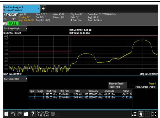
Band26(824-849)-1.4MHz-16QAM-26797-1RB#5-PASS
