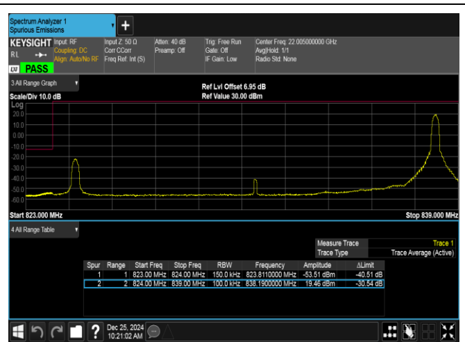
Band26(824-849)-15MHz-QPSK-26865-1RB#74-PASS
