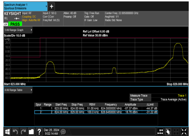
Band26(824-849)-5MHz-QPSK-26815-1RB#24-PASS
