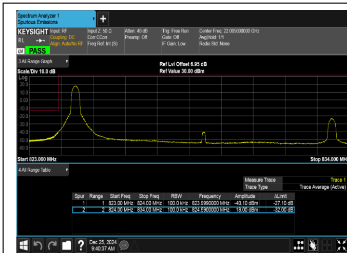
Band26(824-849)-10MHz-16QAM-26840-1RB#0-PASS
