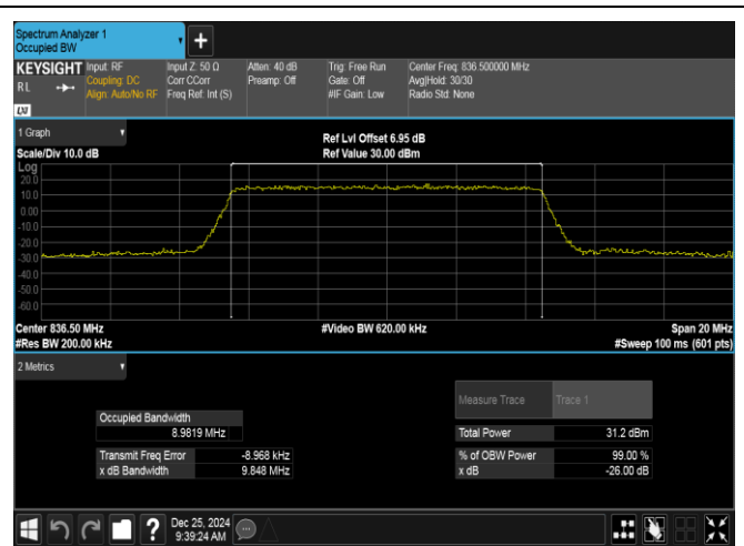
Band26(824-849)-10MHz-QPSK-26915-50RB#0-PASS
