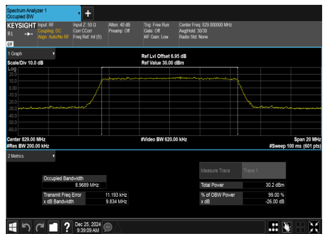
Band26(824-849)-10MHz-16QAM-26840-50RB#0-PASS
