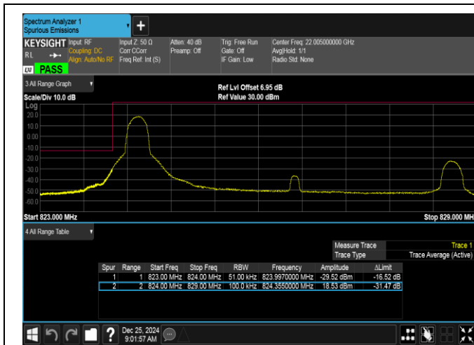
Band26(824-849)-5MHz-16QAM-26815-1RB#0-PASS
