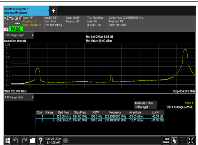
Band26(824-849)-10MHz-16QAM-26840-1RB#49-PASS
