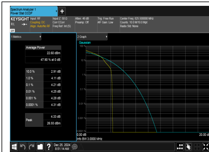
Band26(824-849)-3MHz-16QAM-26805-1RB#0-PASS
