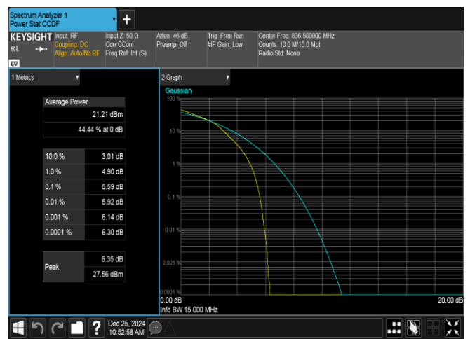
Band26(824-849)-15MHz-16QAM-26915-75RB#0-PASS
