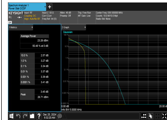
Band26(824-849)-5MHz-QPSK-26915-1RB#0-PASS
