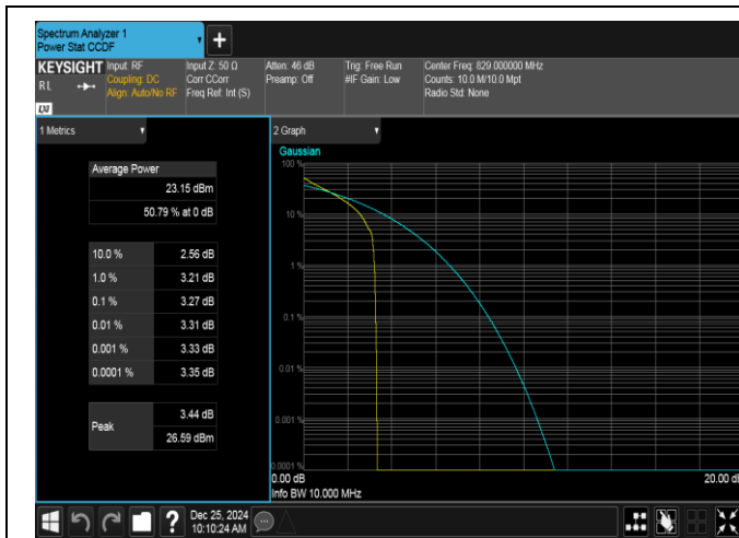
Band26(824-849)-10MHz-QPSK-26840-1RB#0-PASS
