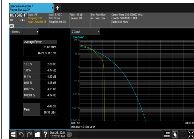
Band26(824-849)-15MHz-16QAM-26915-1RB#0-PASS
