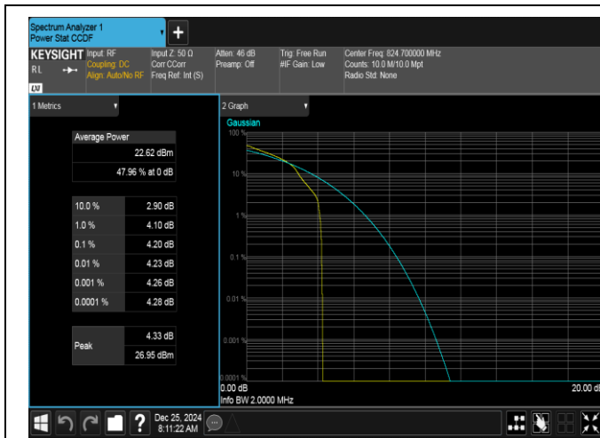
Band26(824-849)-1.4MHz-16QAM-26797-1RB#0-PASS
