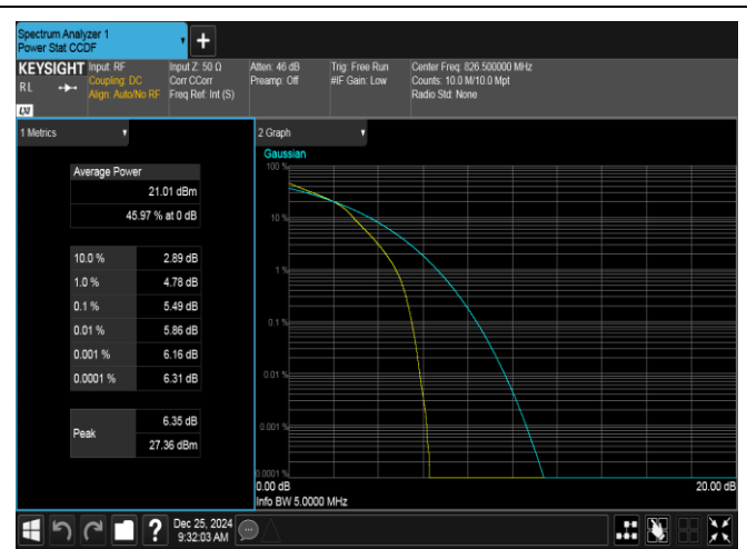
Band26(824-849)-5MHz-16QAM-26815-25RB#0-PASS
