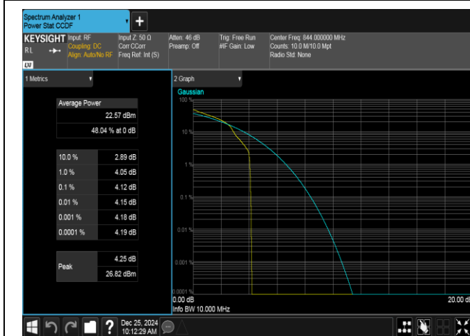
Band26(824-849)-10MHz-16QAM-26990-1RB#0-PASS
