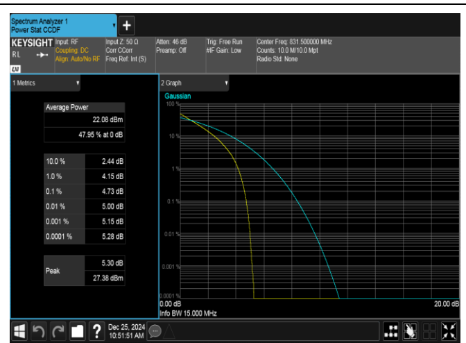
Band26(824-849)-15MHz-QPSK-26865-75RB#0-PASS
