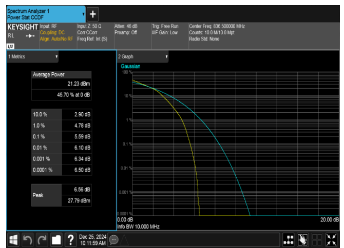
Band26(824-849)-10MHz-16QAM-26915-50RB#0-PASS
