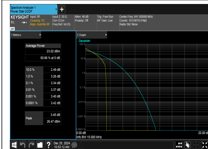
Band26(824-849)-15MHz-QPSK-26965-1RB#0-PASS
