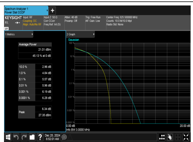
Band26(824-849)-3MHz-16QAM-26805-15RB#0-PASS
