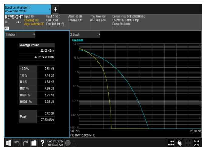
Band26(824-849)-15MHz-QPSK-26965-75RB#0-PASS
