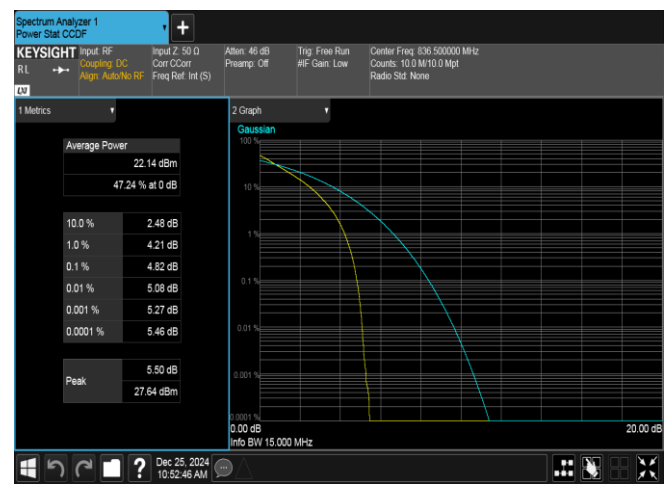
Band26(824-849)-15MHz-QPSK-26915-75RB#0-PASS
