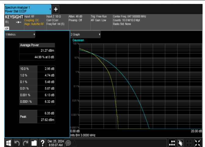
Band26(824-849)-3MHz-16QAM-27025-15RB#0-PASS
