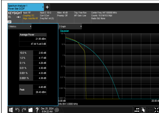
Band26(824-849)-3MHz-16QAM-27025-1RB#0-PASS
