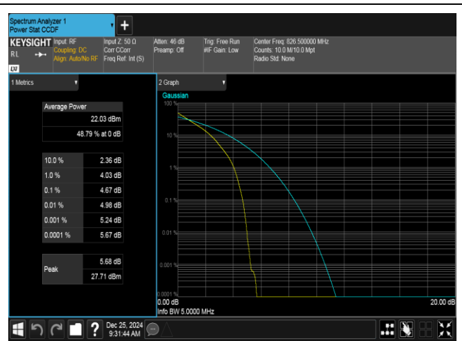
Band26(824-849)-5MHz-QPSK-26815-25RB#0-PASS
