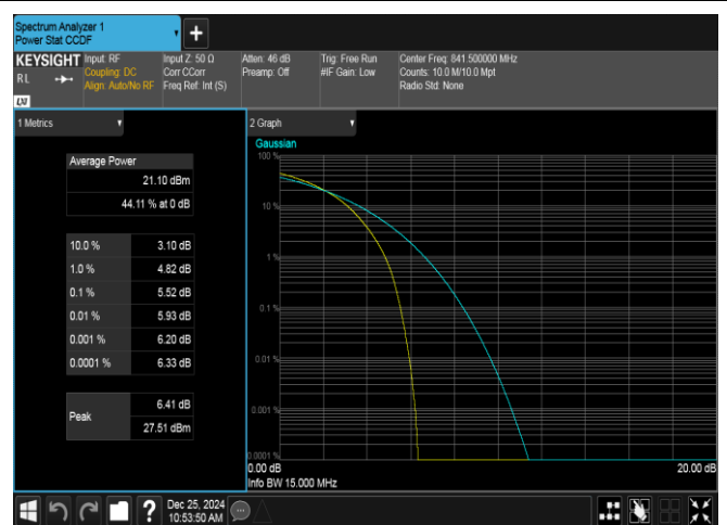
Band26(824-849)-15MHz-16QAM-26965-75RB#0-PASS
