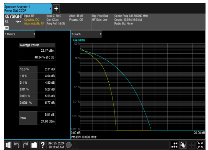
Band26(824-849)-10MHz-QPSK-26915-50RB#0-PASS
