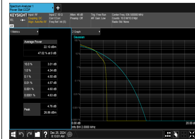
Band26(824-849)-1.4MHz-16QAM-26915-1RB#0-PASS
