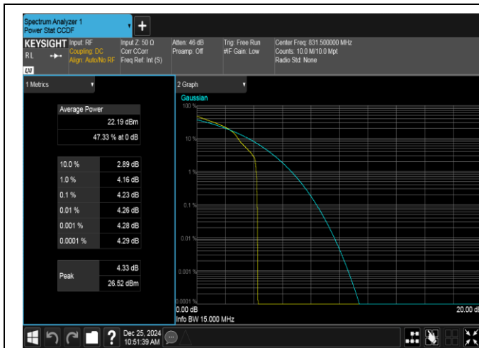
Band26(824-849)-15MHz-16QAM-26865-1RB#0-PASS
