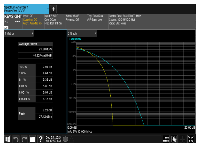
Band26(824-849)-10MHz-16QAM-26990-50RB#0-PASS
