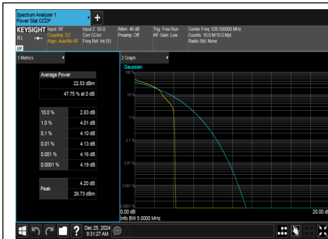
Band26(824-849)-5MHz-16QAM-26815-1RB#0-PASS
