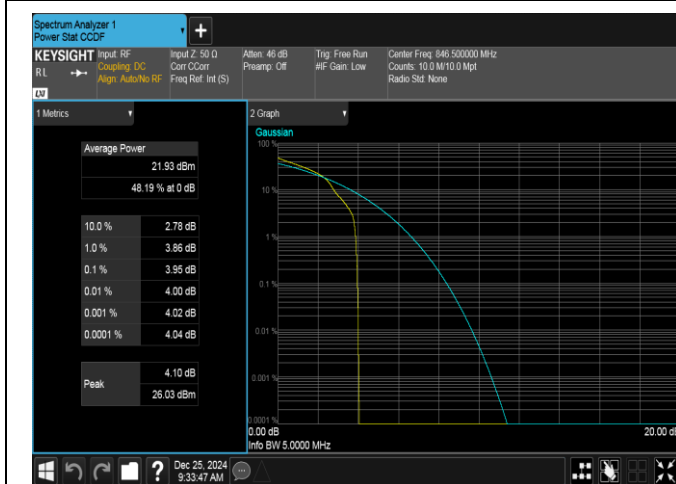
Band26(824-849)-5MHz-16QAM-27015-1RB#0-PASS
