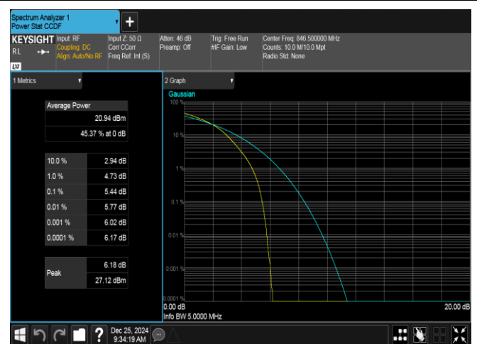
Band26(824-849)-5MHz-16QAM-27015-25RB#0-PASS
