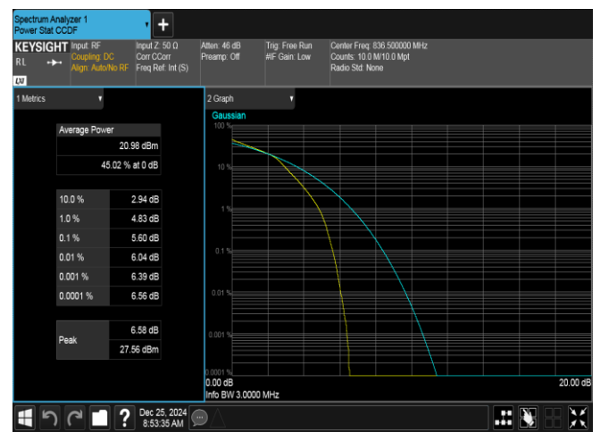
Band26(824-849)-3MHz-16QAM-26915-15RB#0-PASS
