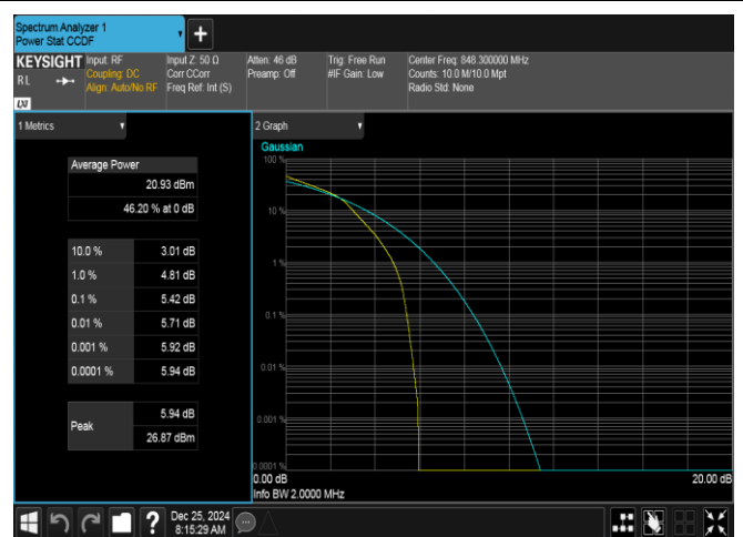
Band26(824-849)-1.4MHz-16QAM-27033-6RB#0-PASS
