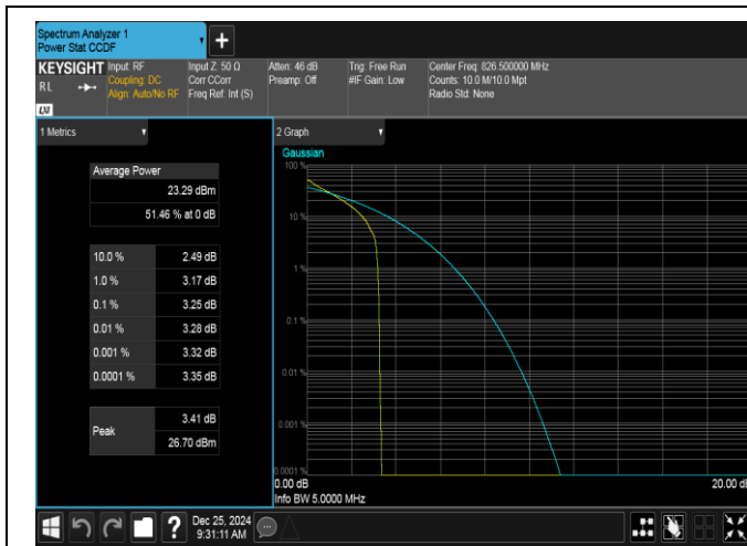
Band26(824-849)-5MHz-QPSK-26815-1RB#0-PASS
