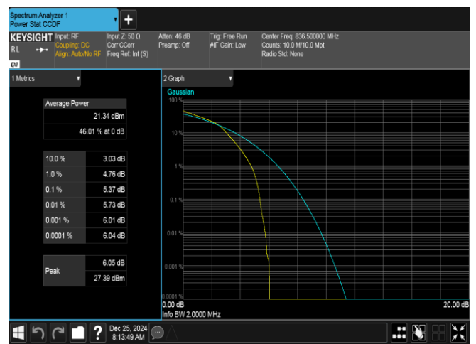
Band26(824-849)-1.4MHz-16QAM-26915-6RB#0-PASS
