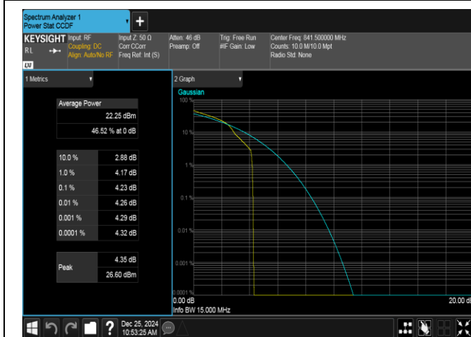
Band26(824-849)-15MHz-16QAM-26965-1RB#0-PASS
