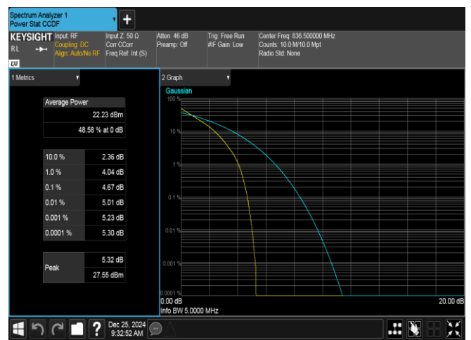
Band26(824-849)-5MHz-QPSK-26915-25RB#0-PASS
