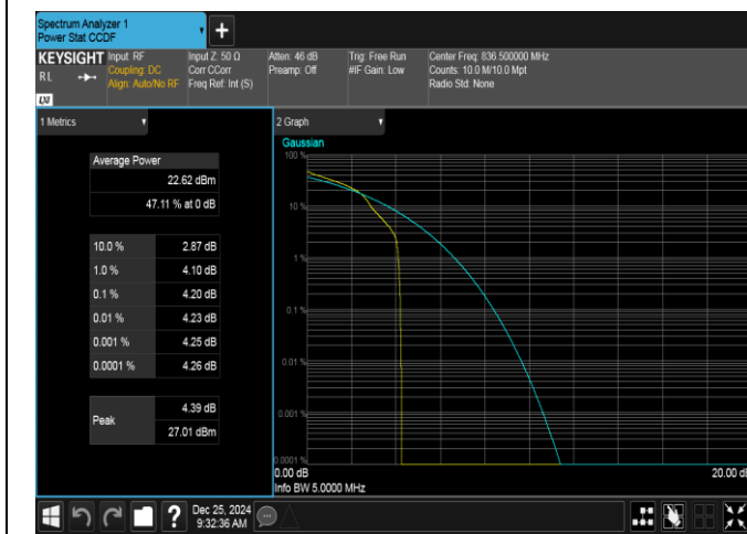
Band26(824-849)-5MHz-16QAM-26915-1RB#0-PASS
