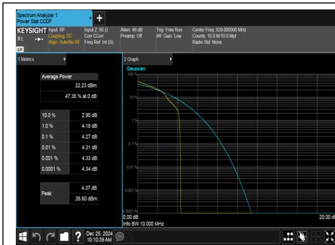
Band26(824-849)-10MHz-16QAM-26840-1RB#0-PASS
