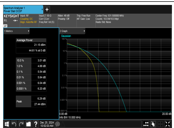
Band26(824-849)-15MHz-16QAM-26865-75RB#0-PASS
