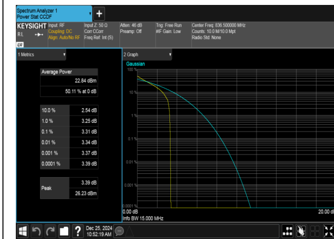
Band26(824-849)-15MHz-QPSK-26915-1RB#0-PASS
