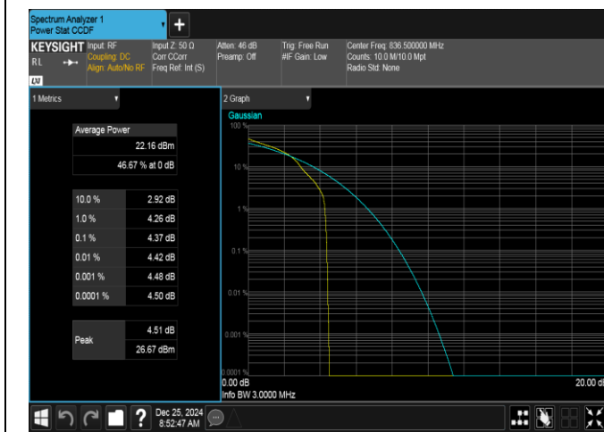
Band26(824-849)-3MHz-16QAM-26915-1RB#0-PASS
