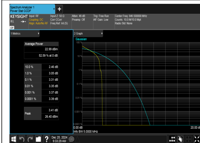
Band26(824-849)-5MHz-QPSK-27015-1RB#0-PASS
