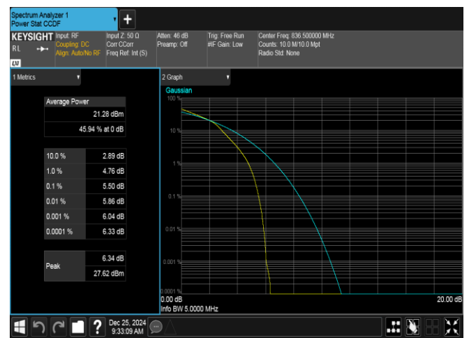
Band26(824-849)-5MHz-16QAM-26915-25RB#0-PASS
