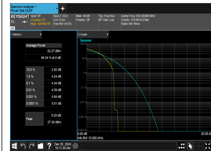
Band26(824-849)-10MHz-16QAM-26915-1RB#0-PASS
