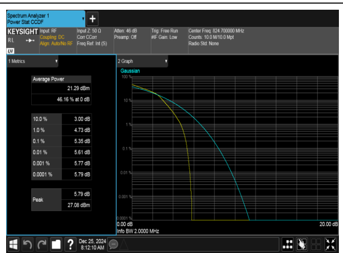
Band26(824-849)-1.4MHz-16QAM-26797-6RB#0-PASS
