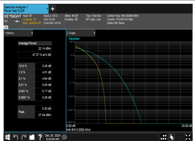
Band26(824-849)-5MHz-QPSK-27015-25RB#0-PASS
