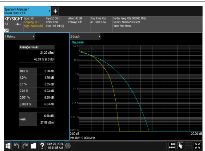
Band26(824-849)-10MHz-16QAM-26840-50RB#0-PASS
