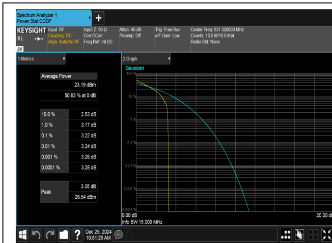
Band26(824-849)-15MHz-QPSK-26865-1RB#0-PASS
