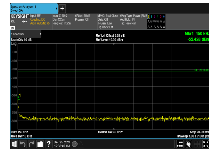
Band26(814-824)-3MHz-16QAM-26705-15RB#0-0.15~30-PASS
