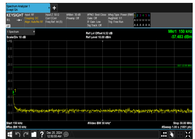
Band26(814-824)-3MHz-16QAM-26775-1RB#14-0.15-30-PASS
