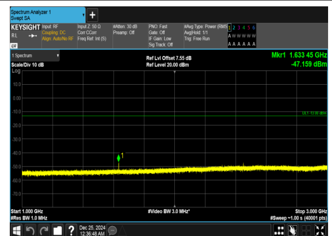
Band26(814-824)-3MHz-16QAM-26705-1RB#14-1000-3000-PASS
