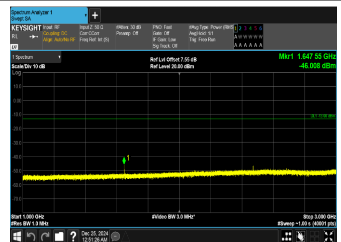
Band26(814-824)-3MHz-16QAM-26775-1RB#14-1000-3000-PASS
