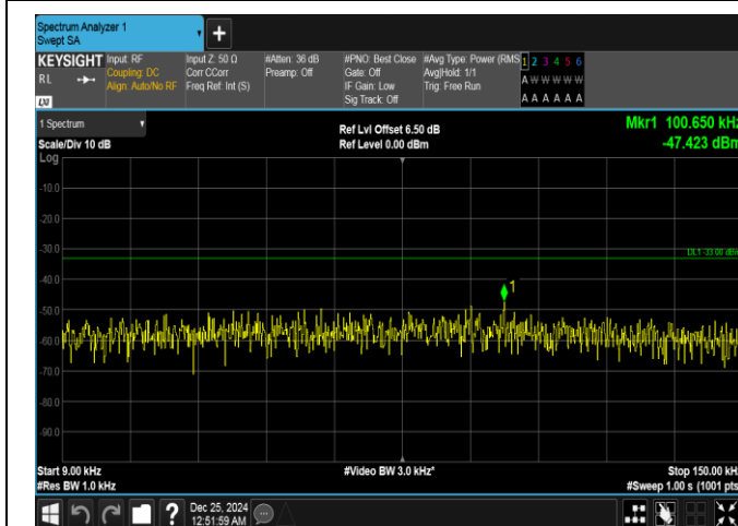
Band26(814-824)-3MHz-QPSK-26775-15RB#0-0.009~0.15-PASS
