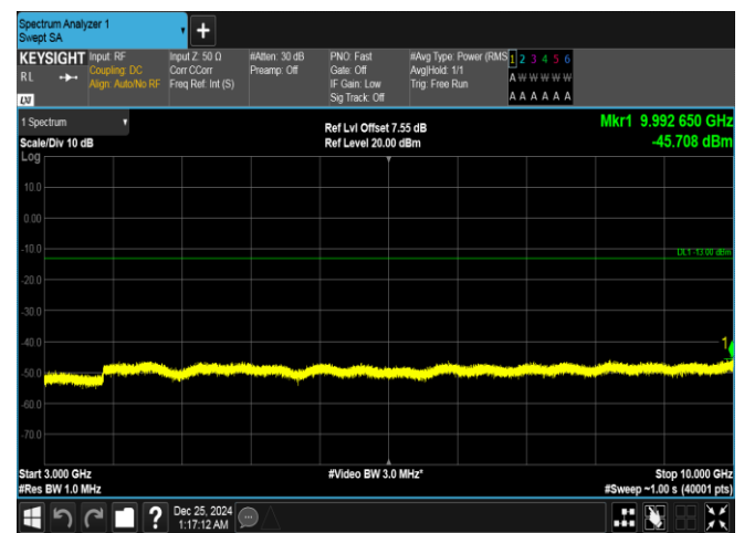
Band26(814-824)-5MHz-QPSK-26715-1RB#24-3000~10000-PASS
