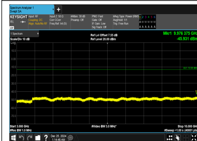
Band26(814-824)-5MHz-QPSK-26715-1RB#0-3000~10000-PASS
