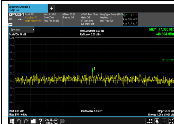
Band26(814-824)-5MHz-QPSK-26715-25RB#0-0.009~0.15-PASS
