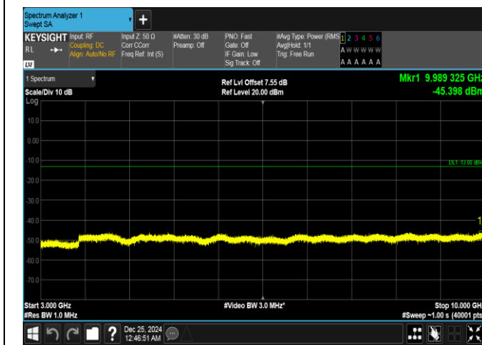
Band26(814-824)-3MHz-16QAM-26740-15RB#0-3000~10000-PASS
