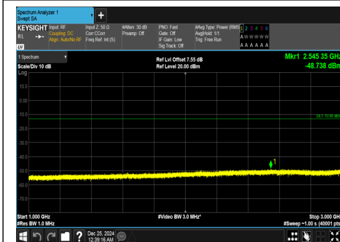
Band26(814-824)-3MHz-16QAM-26705-15RB#0-1000~3000-PASS
