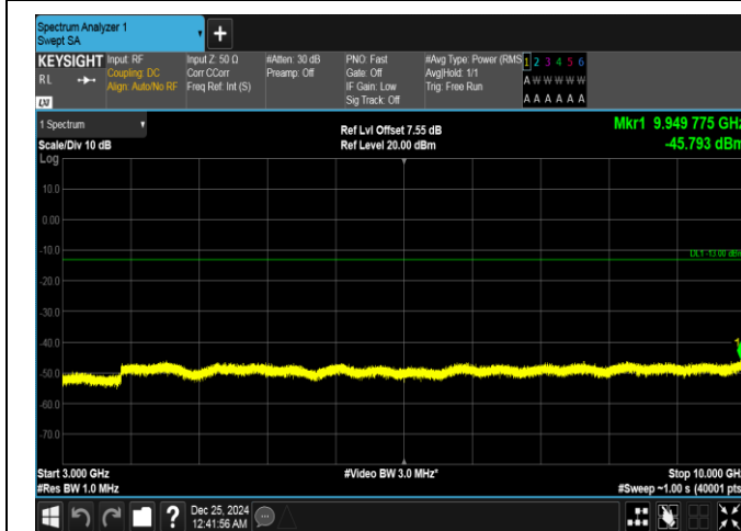
Band26(814-824)-3MHz-16QAM-26740-1RB#0-3000~10000-PASS
