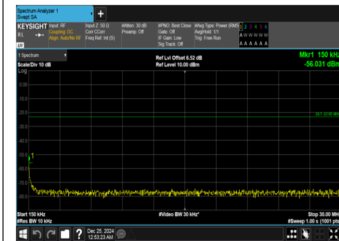
Band26(814-824)-3MHz-16QAM-26775-15RB#0-0.15~30-PASS
