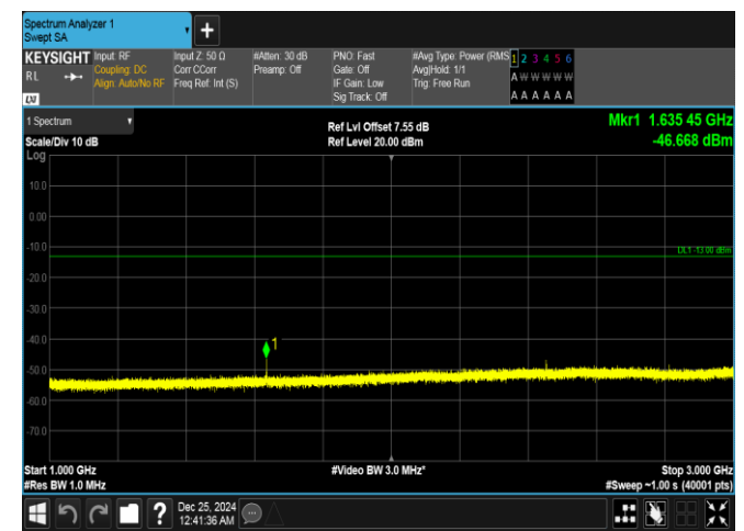
Band26(814-824)-3MHz-16QAM-26740-1RB#0-1000~3000-PASS
