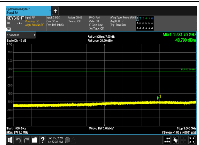
Band26(814-824)-3MHz-QPSK-26775-15RB#0-1000~3000-PASS
