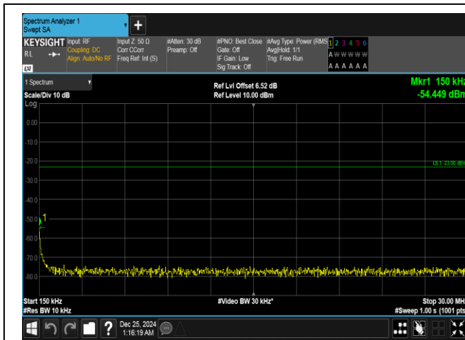
Band26(814-824)-5MHz-QPSK-26715-1RB#24-0.15~30-PASS
