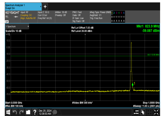
Band26(814-824)-3MHz-16QAM-26705-15RB#0-30~1000-PASS
