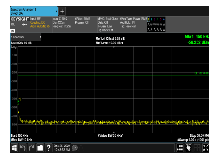
Band26(814-824)-3MHz-16QAM-26740-1RB#14-0.15~30-PASS
