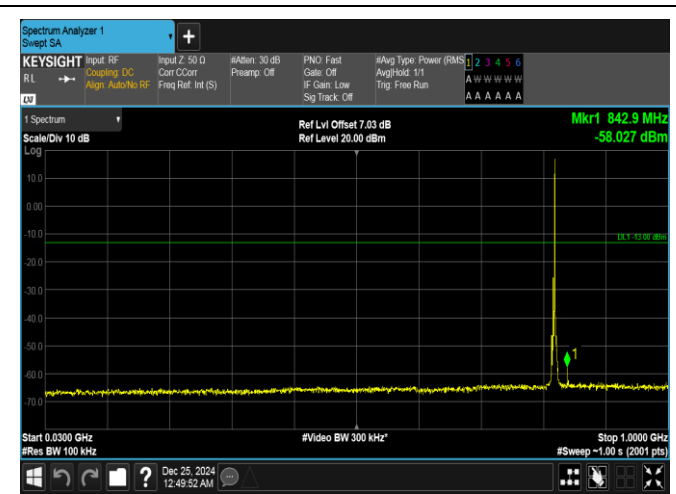
Band26(814-824)-3MHz-QPSK-26775-1RB#14-30~1000-PASS
