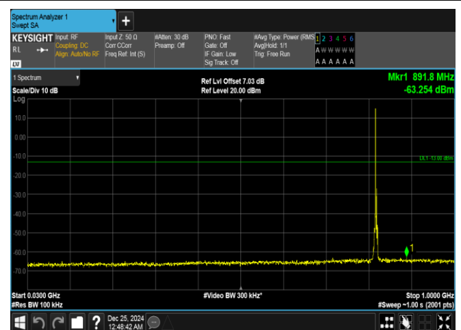
Band26(814-824)-3MHz-16QAM-26775-1RB#0-30~1000-PASS
