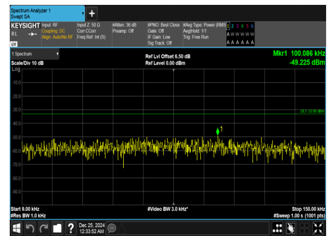
Band26(814-824)-3MHz-16QAM-26705-1RB#0-0.009~0.15-PASS
