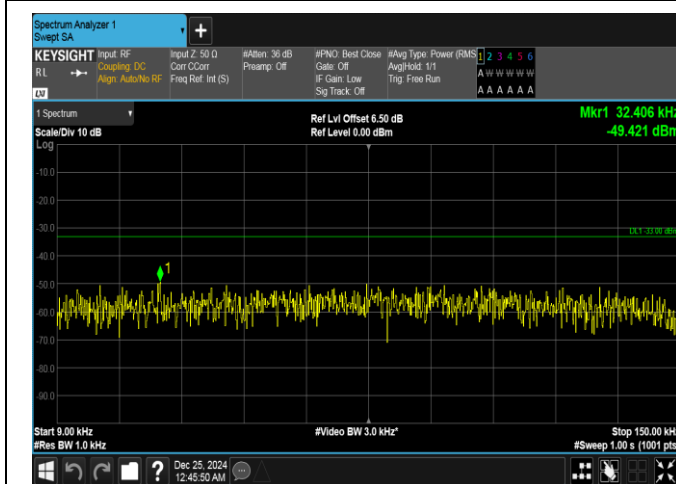
Band26(814-824)-3MHz-16QAM-26740-15RB#0-0.009~0.15-PASS
