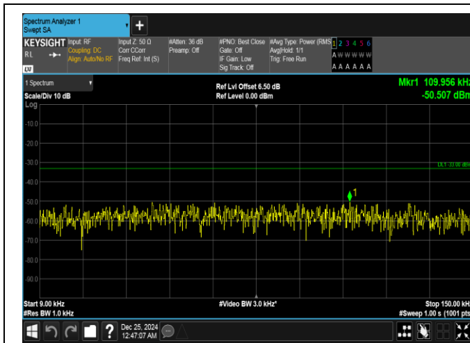
Band26(814-824)-3MHz-QPSK-26775-1RB#0-0.009~0.15-PASS
