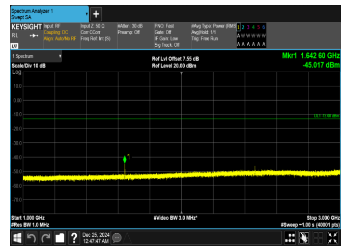
Band26(814-824)-3MHz-QPSK-26775-1RB#0-1000~3000-PASS
