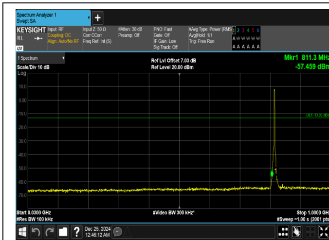
Band26(814-824)-3MHz-16QAM-26740-15RB#0-30~1000-PASS
