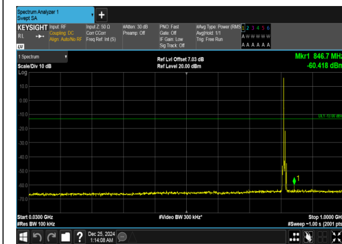
Band26(814-824)-5MHz-QPSK-26715-1RB#0-30~1000-PASS
