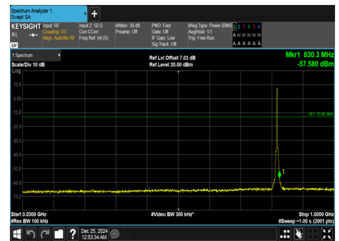
Band26(814-824)-3MHz-16QAM-26775-15RB#0-30~1000-PASS
