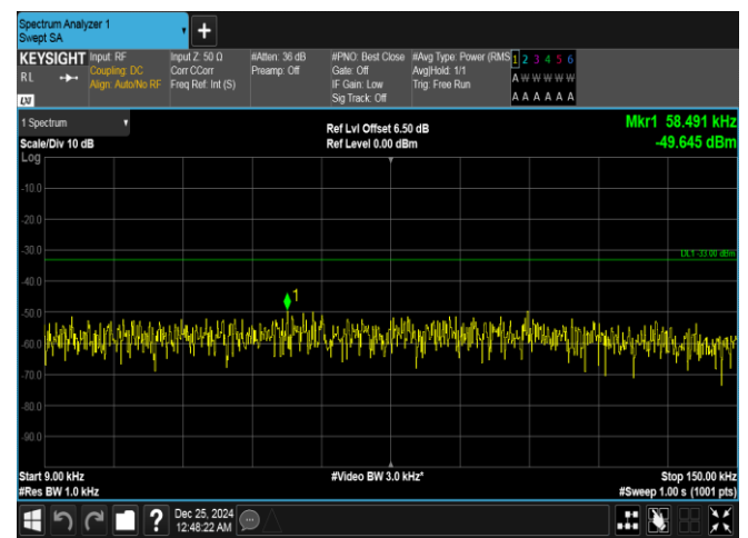
Band26(814-824)-3MHz-16QAM-26775-1RB#0-0.009~0.15-PASS
