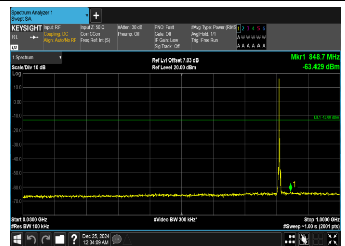
Band26(814-824)-3MHz-16QAM-26705-1RB#0-30~1000-PASS
