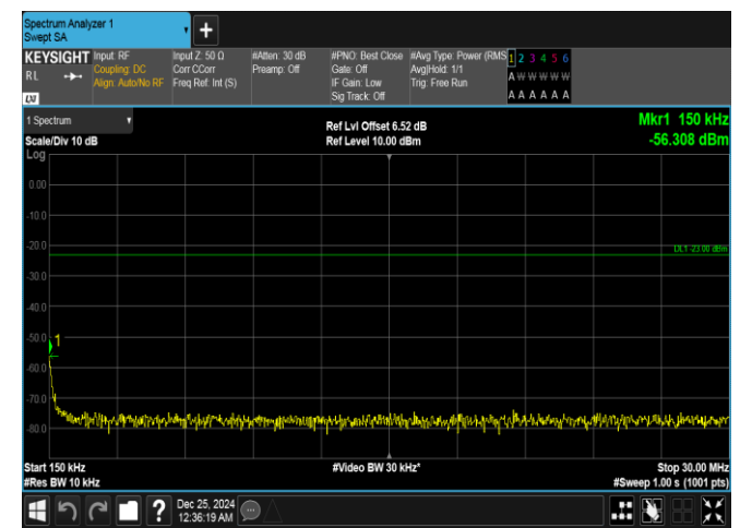
Band26(814-824)-3MHz-16QAM-26705-1RB#14-0.15-30-PASS
