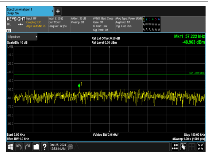
Band26(814-824)-3MHz-16QAM-26775-15RB#0-0.009~0.15-PASS
