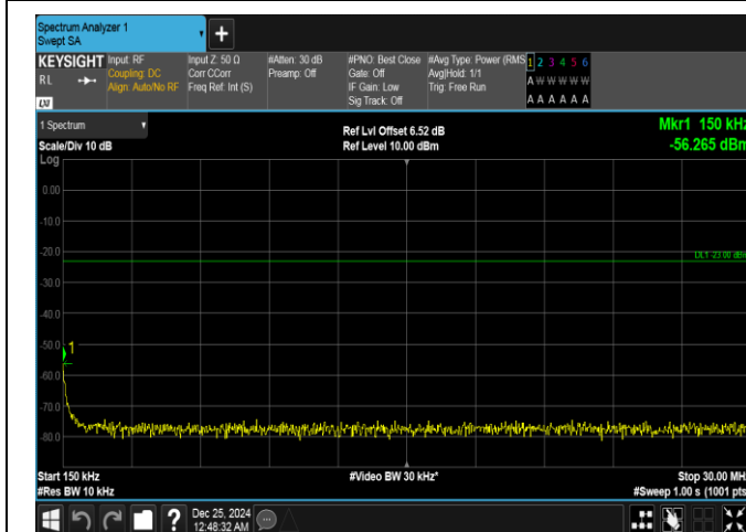
Band26(814-824)-3MHz-16QAM-26775-1RB#0-0.15~30-PASS
