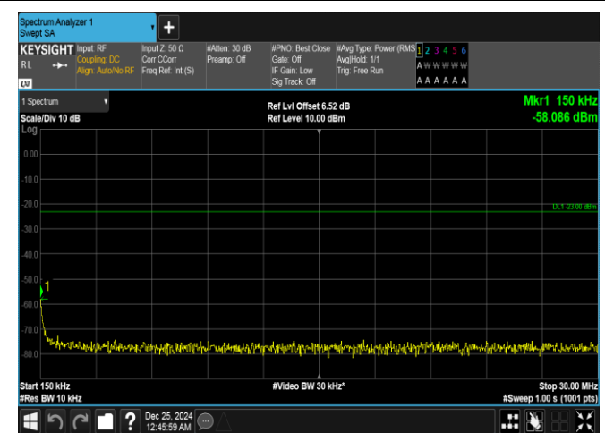
Band26(814-824)-3MHz-16QAM-26740-15RB#0-0.15~30-PASS
