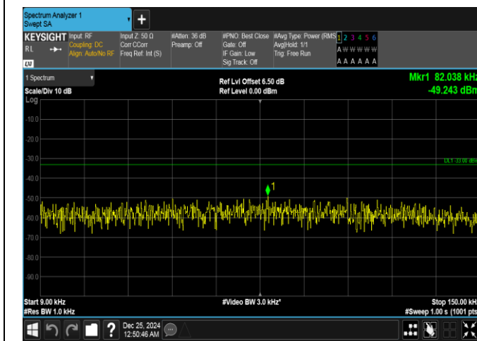
Band26(814-824)-3MHz-16QAM-26775-1RB#14-0.009-0.15-PASS
