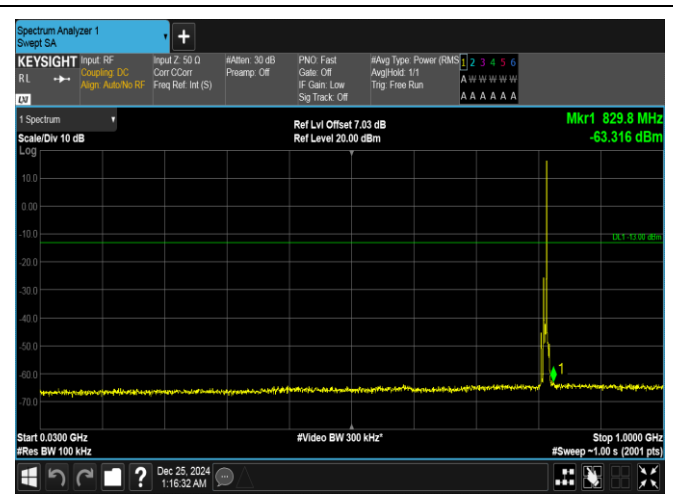
Band26(814-824)-5MHz-QPSK-26715-1RB#24-30~1000-PASS
