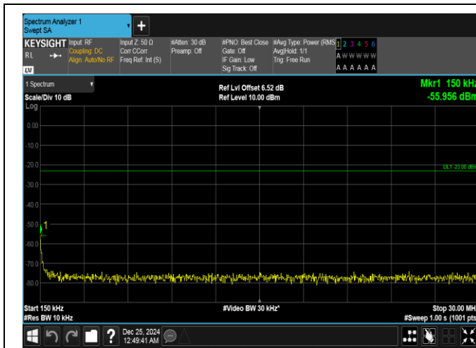
Band26(814-824)-3MHz-QPSK-26775-1RB#14-0.15~30-PASS
