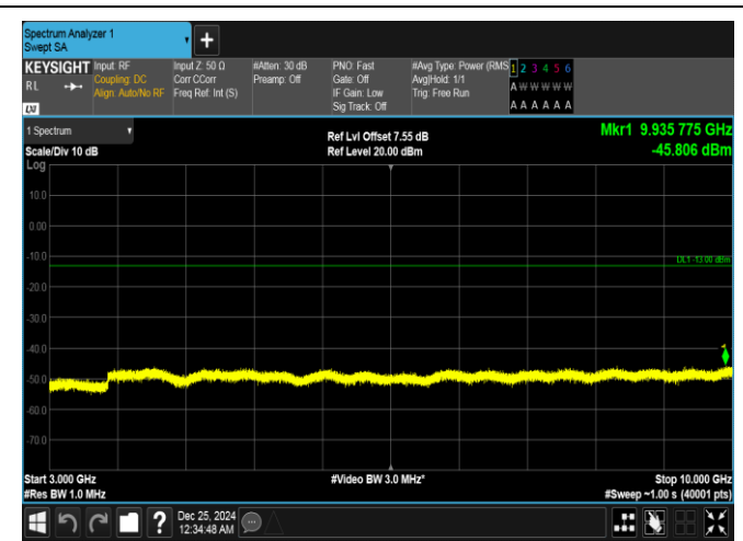
Band26(814-824)-3MHz-16QAM-26705-1RB#0-3000-10000-PASS
