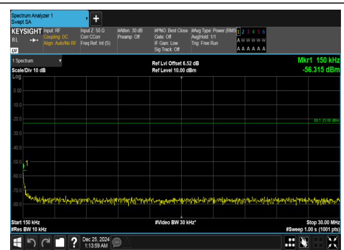
Band26(814-824)-5MHz-QPSK-26715-1RB#0-0.15~30-PASS
