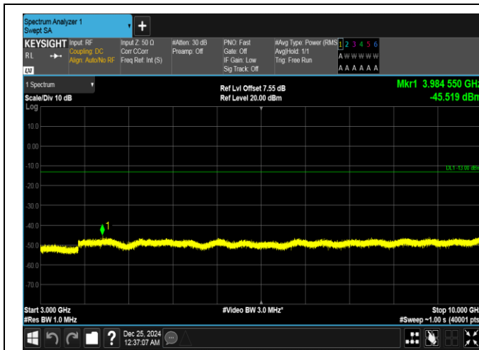
Band26(814-824)-3MHz-16QAM-26705-1RB#14-3000~10000-PASS
