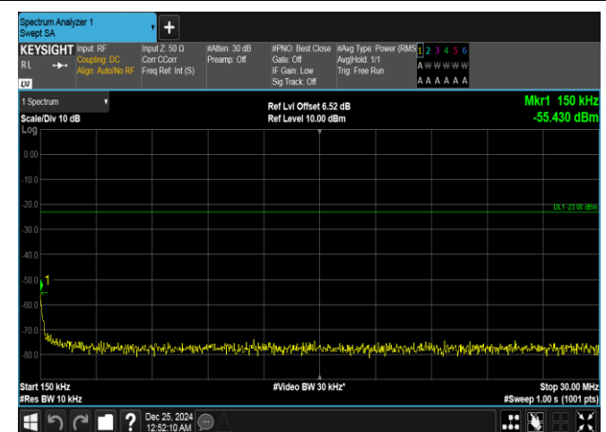
Band26(814-824)-3MHz-QPSK-26775-15RB#0-0.15~30-PASS
