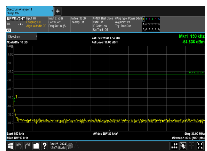
Band26(814-824)-3MHz-QPSK-26775-1RB#0-0.15~30-PASS
