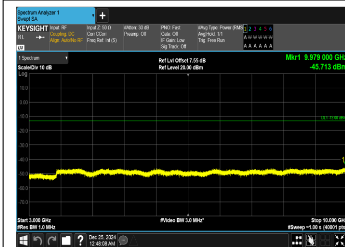
Band26(814-824)-3MHz-QPSK-26775-1RB#0-3000~10000-PASS
