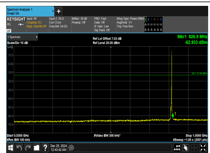
Band26(814-824)-3MHz-16QAM-26740-1RB#14-30~1000-PASS
