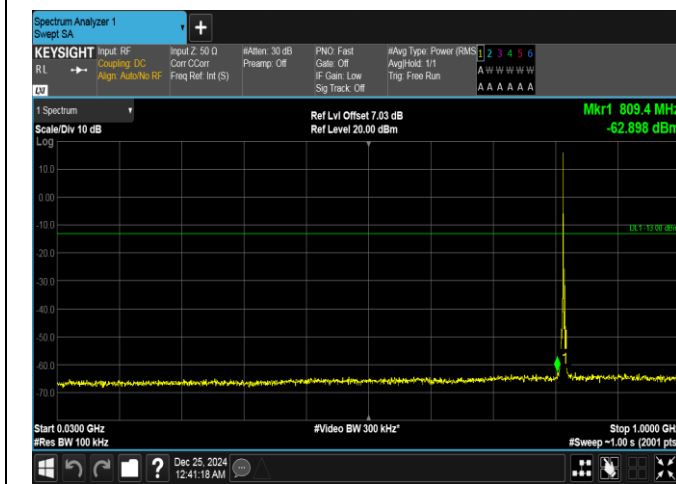
Band26(814-824)-3MHz-16QAM-26740-1RB#0-30~1000-PASS
