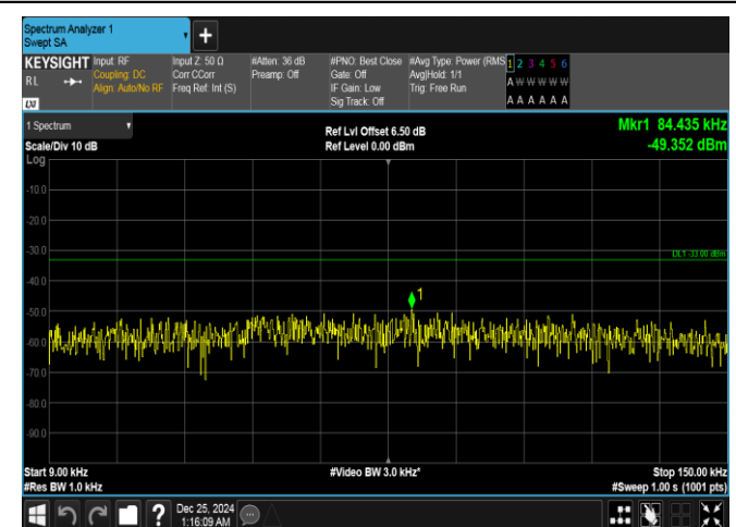
Band26(814-824)-5MHz-QPSK-26715-1RB#24-0.009~0.15-PASS
