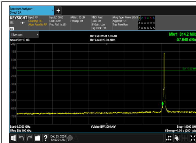
Band26(814-824)-3MHz-QPSK-26775-15RB#0-30~1000-PASS
