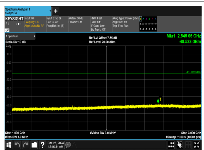
Band26(814-824)-3MHz-16QAM-26740-15RB#0-1000~3000-PASS
