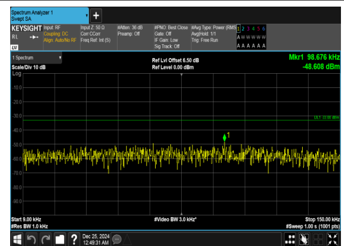
Band26(814-824)-3MHz-QPSK-26775-1RB#14-0.009~0.15-PASS
