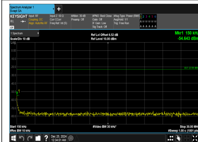
Band26(814-824)-3MHz-16QAM-26705-1RB#0-0.15~30-PASS
