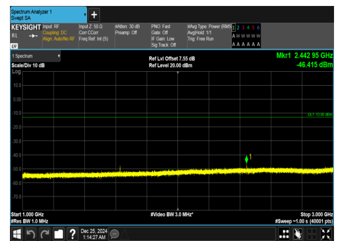
Band26(814-824)-5MHz-QPSK-26715-1RB#0-1000~3000-PASS
