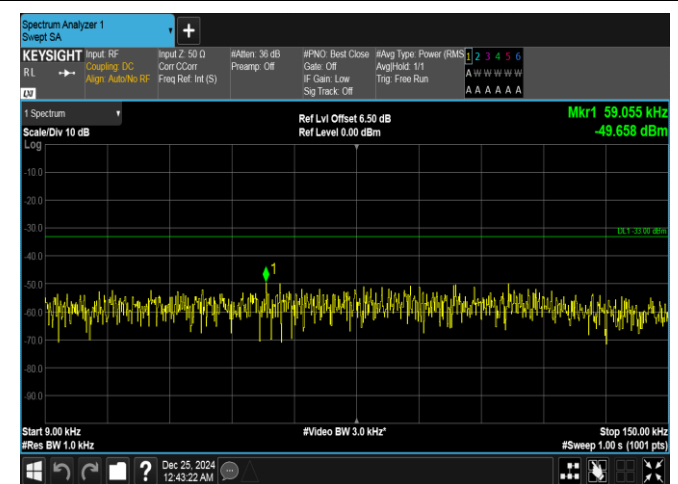
Band26(814-824)-3MHz-16QAM-26740-1RB#14-0.009~0.15-PASS
