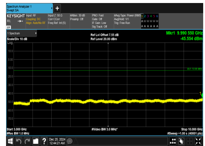
Band26(814-824)-3MHz-16QAM-26740-1RB#14-3000~10000-PASS
