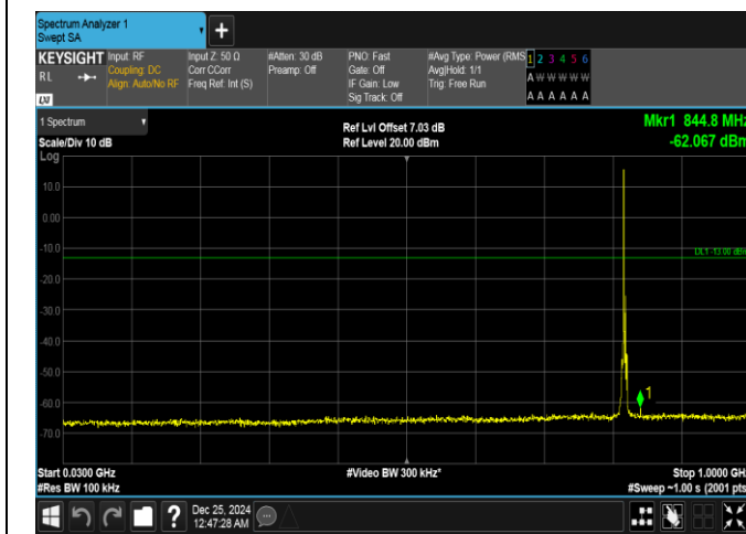
Band26(814-824)-3MHz-QPSK-26775-1RB#0-30~1000-PASS
