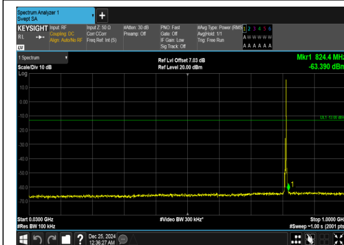
Band26(814-824)-3MHz-16QAM-26705-1RB#14-30-1000-PASS
