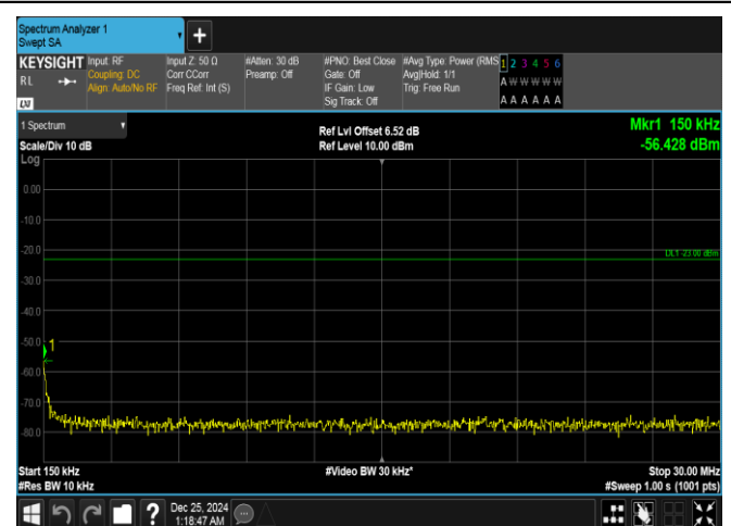
Band26(814-824)-5MHz-QPSK-26715-25RB#0-0.15~30-PASS
