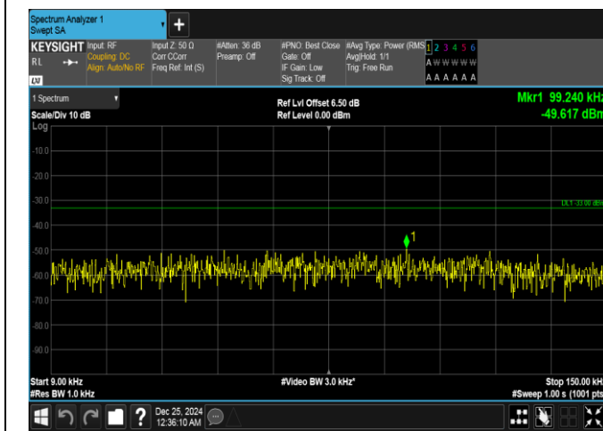
Band26(814-824)-3MHz-16QAM-26705-1RB#14-0.009-0.15-PASS
