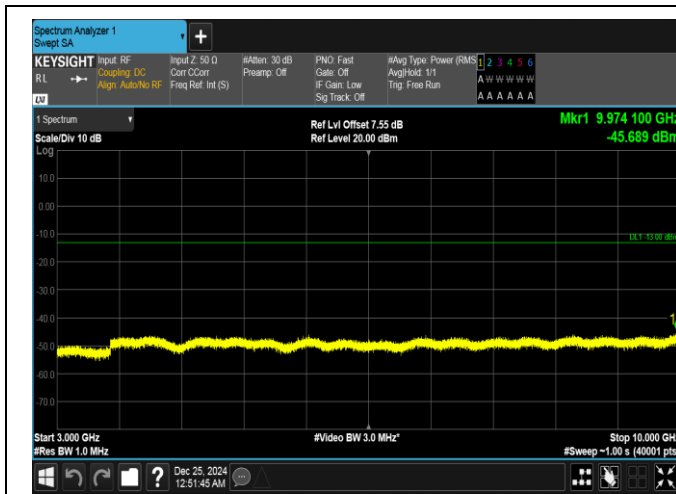
Band26(814-824)-3MHz-16QAM-26775-1RB#14-3000~10000-PASS
