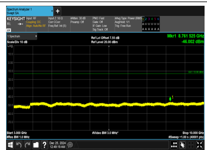
Band26(814-824)-3MHz-16QAM-26775-1RB#0-3000-10000-PASS
