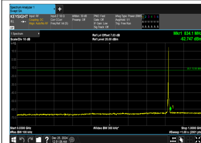
Band26(814-824)-3MHz-16QAM-26775-1RB#14-30-1000-PASS
