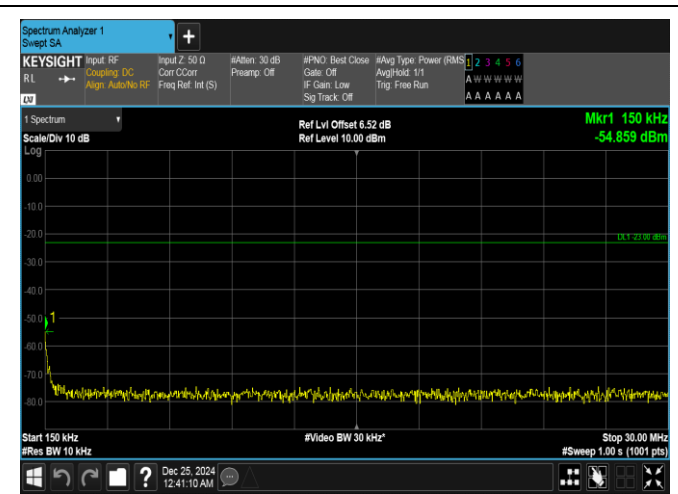
Band26(814-824)-3MHz-16QAM-26740-1RB#0-0.15~30-PASS
