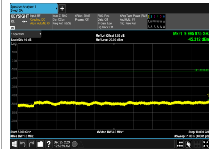
Band26(814-824)-3MHz-QPSK-26775-15RB#0-3000~10000-PASS
