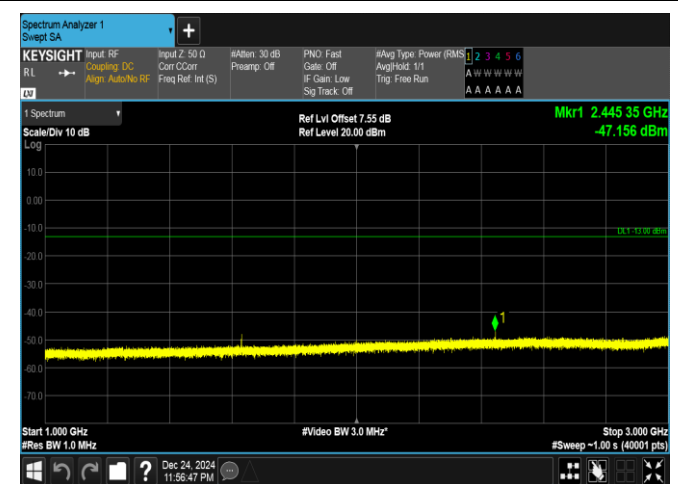
Band26(814-824)-1.4MHz-16QAM-26697-1RB#5-1000~3000-PASS
