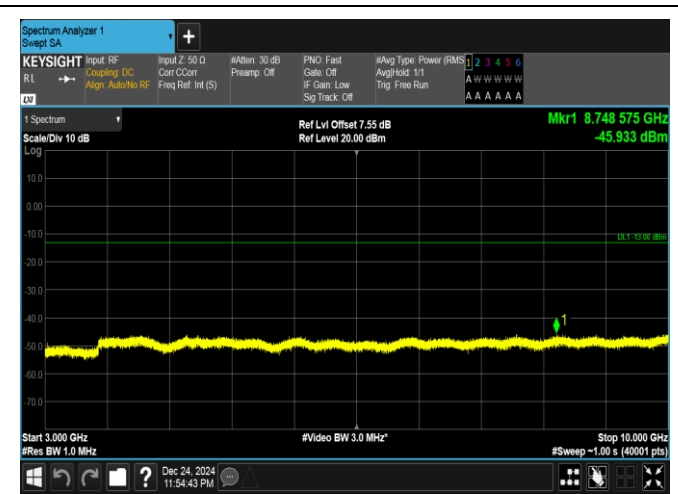
Band26(814-824)-1.4MHz-16QAM-26697-1RB#0-3000~10000-PASS
