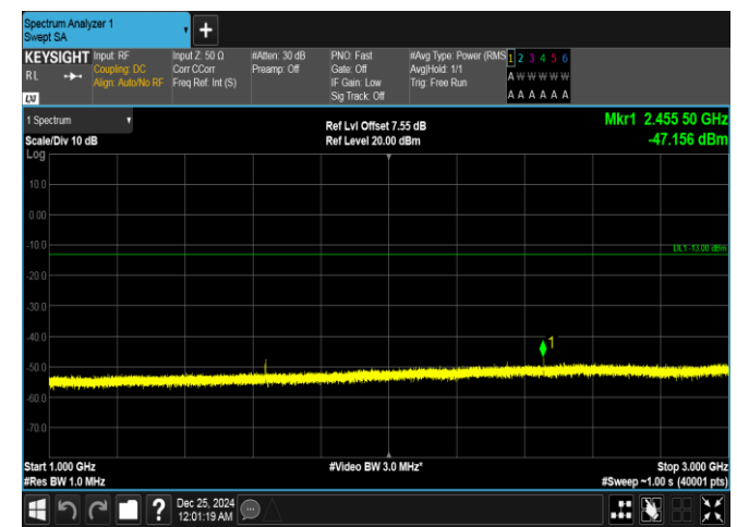
Band26(814-824)-1.4MHz-16QAM-26740-1RB#0-1000~3000-PASS
