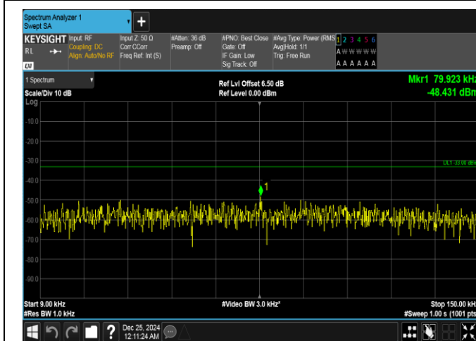
Band26(814-824)-1.4MHz-QPSK-26783-6RB#0-0.009~0.15-PASS
