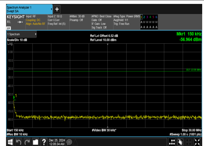
Band26(814-824)-1.4MHz-16QAM-26740-6RB#0-0.15~30-PASS
