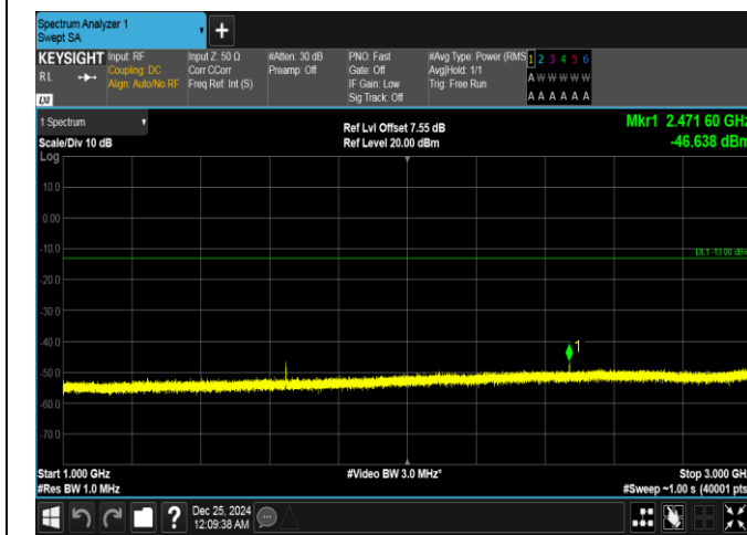
Band26(814-824)-1.4MHz-QPSK-26783-1RB#5-1000~3000-PASS
