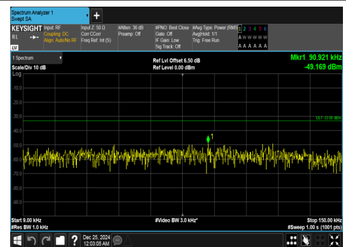
Band26(814-824)-1.4MHz-16QAM-26740-1RB#5-0.009~0.15-PASS
