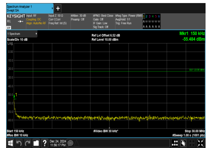
Band26(814-824)-1.4MHz-16QAM-26697-1RB#5-0.15~30-PASS
