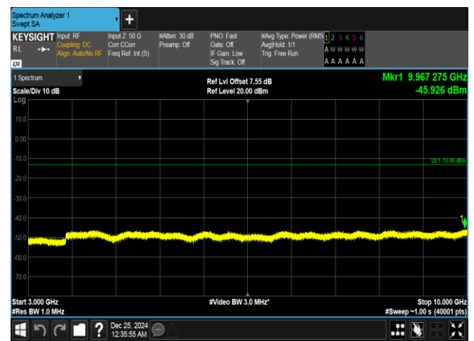
Band26(814-824)-3MHz-QPSK-26705-1RB#14-3000~10000-PASS
