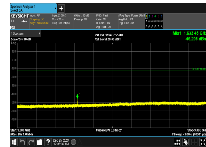
Band26(814-824)-3MHz-QPSK-26705-1RB#14-1000~3000-PASS
