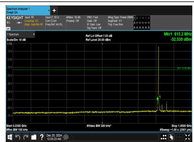
Band26(814-824)-1.4MHz-16QAM-26740-1RB#5-30~1000-PASS
