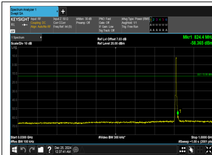
Band26(814-824)-3MHz-QPSK-26705-15RB#0-30~1000-PASS
