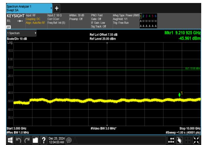
Band26(814-824)-1.4MHz-16QAM-26740-1RB#5-3000~10000-PASS
