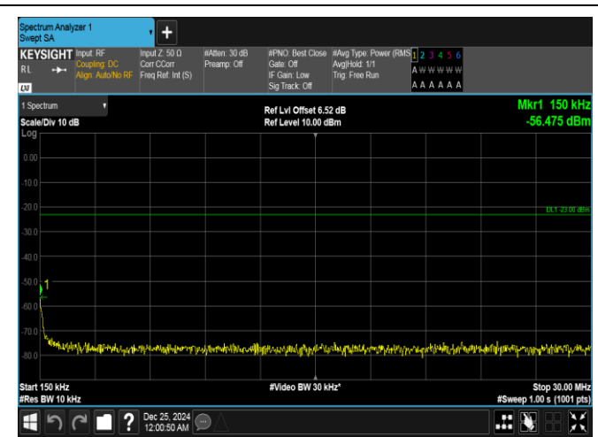
Band26(814-824)-1.4MHz-16QAM-26740-1RB#0-0.15~30-PASS
