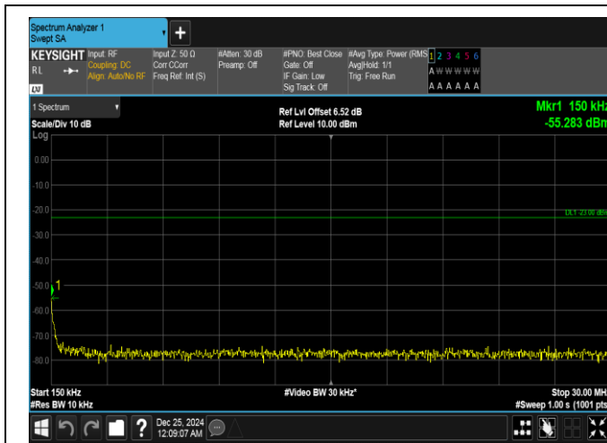
Band26(814-824)-1.4MHz-QPSK-26783-1RB#5-0.15~30-PASS
