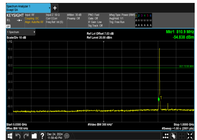
Band26(814-824)-1.4MHz-16QAM-26697-6RB#0-30~1000-PASS
