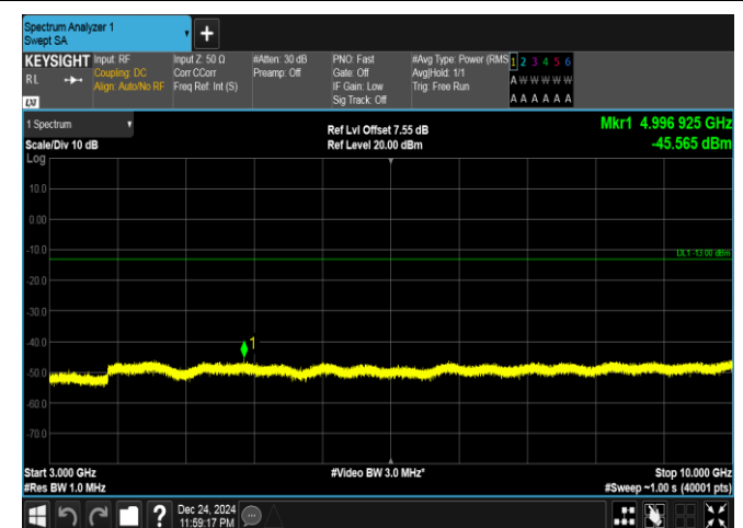
Band26(814-824)-1.4MHz-16QAM-26697-6RB#0-3000~10000-PASS
