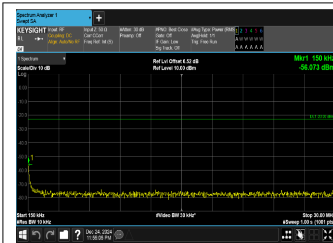
Band26(814-824)-1.4MHz-QPSK-26697-1RB#5-0.15~30-PASS
