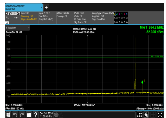
Band26(814-824)-1.4MHz-QPSK-26740-1RB#0-30~1000-PASS
