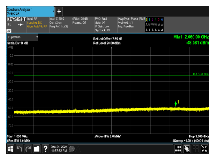
Band26(814-824)-1.4MHz-QPSK-26697-6RB#0-1000~3000-PASS
