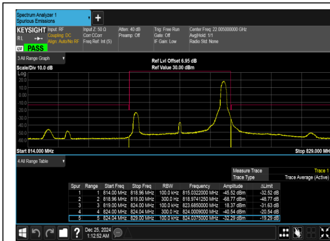
Band26(814-824)-5MHz-16QAM-26765-1RB#24-PASS
