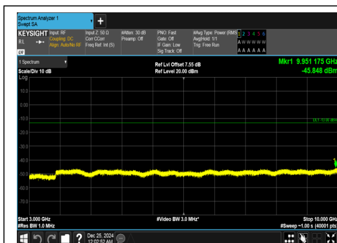
Band26(814-824)-1.4MHz-OPSK-26740-1RB#5-3000~10000-PASS
