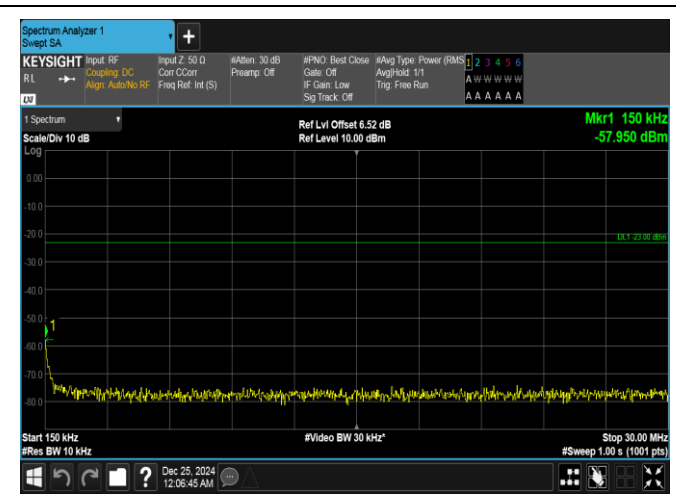
Band26(814-824)-1.4MHz-QPSK-26783-1RB#0-0.15~30-PASS
