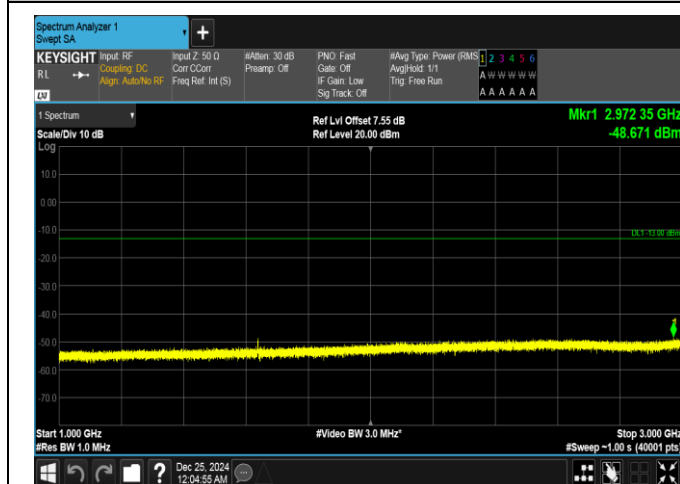
Band26(814-824)-1.4MHz-QPSK-26740-6RB#0-1000~3000-PASS
