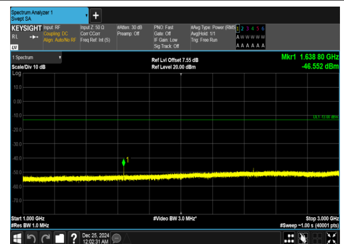
Band26(814-824)-1.4MHz-QPSK-26740-1RB#5-1000~3000-PASS
