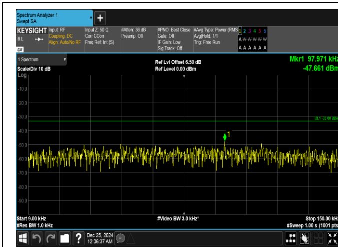
Band26(814-824)-1.4MHz-QPSK-26783-1RB#0-0.009~0.15-PASS
