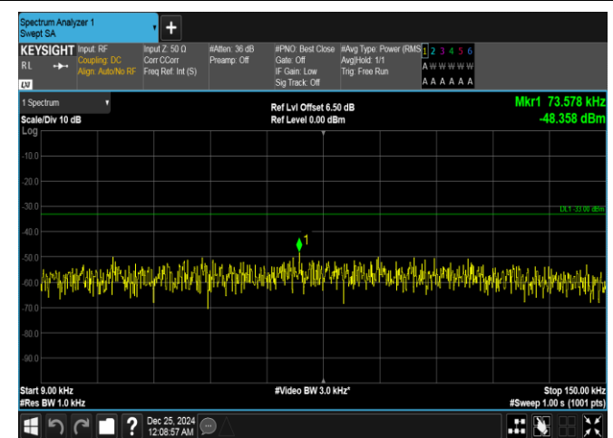
Band26(814-824)-1.4MHz-QPSK-26783-1RB#5-0.009~0.15-PASS
