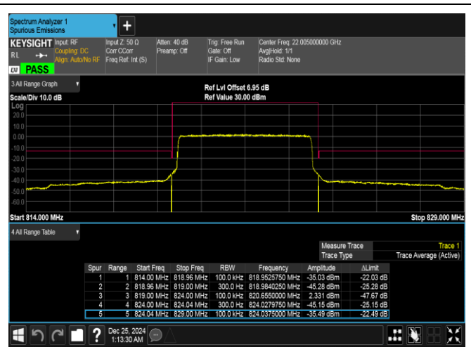
Band26(814-824)-5MHz-16QAM-26765-25RB#0-PASS
