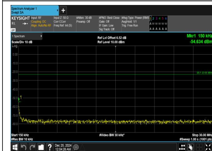
Band26(814-824)-1.4MHz-QPSK-26740-6RB#0-0.15~30-PASS
