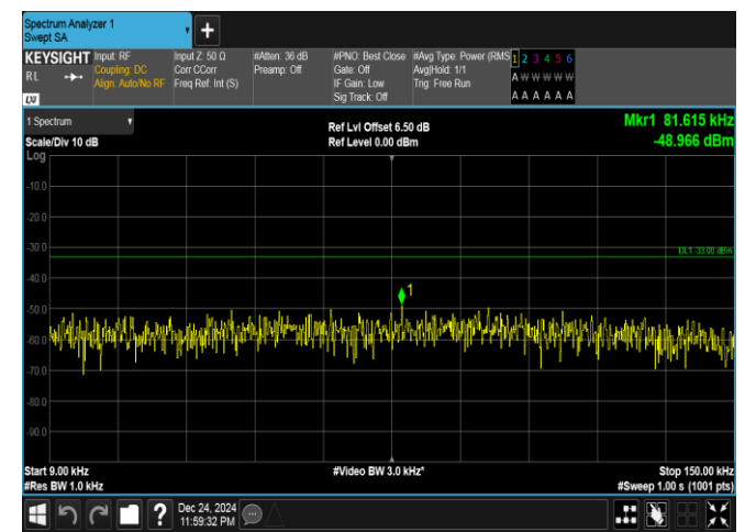
Band26(814-824)-1.4MHz-QPSK-26740-1RB#0-0.009~0.15-PASS
