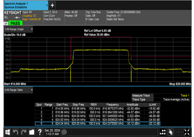
Band26(814-824)-5MHz-QPSK-26765-25RB#0-PASS
