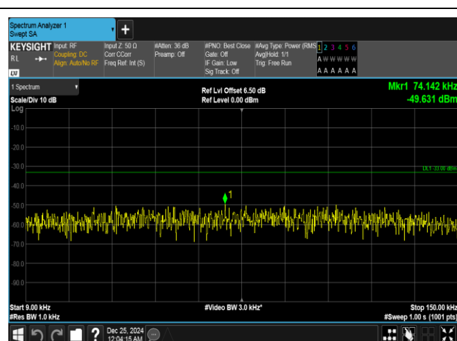
Band26(814-824)-1.4MHz-OPSK-26740-6RB#0-0.009~0.15-PASS
