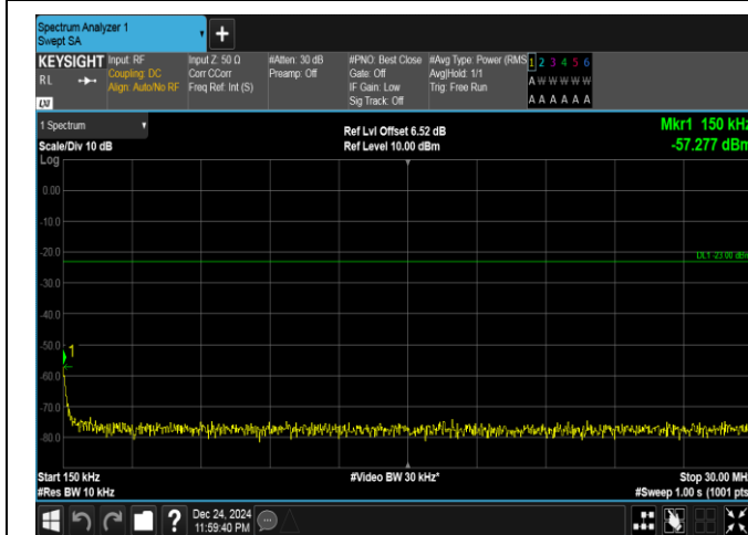
Band26(814-824)-1.4MHz-QPSK-26740-1RB#0-0.15~30-PASS
