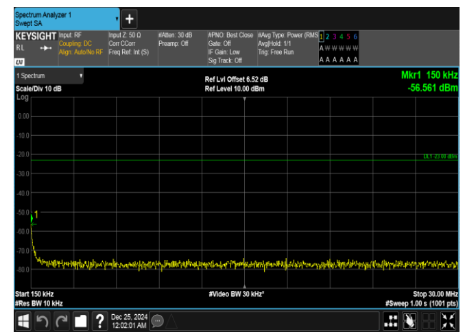
Band26(814-824)-1.4MHz-QPSK-26740-1RB#5-0.15~30-PASS
