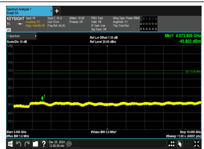
Band26(814-824)-1.4MHz-QPSK-26740-1RB#0-3000~10000-PASS
