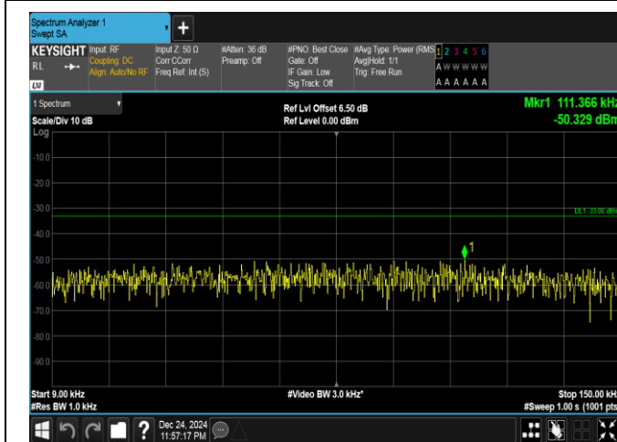
Band26(814-824)-1.4MHz-QPSK-26697-6RB#0-0.009~0.15-PASS
