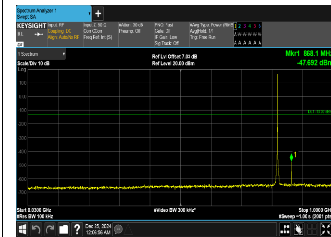
Band26(814-824)-1.4MHz-QPSK-26783-1RB#0-30~1000-PASS
