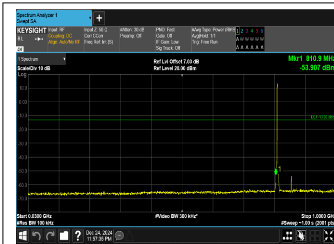
Band26(814-824)-1.4MHz-QPSK-26697-6RB#0-30~1000-PASS
