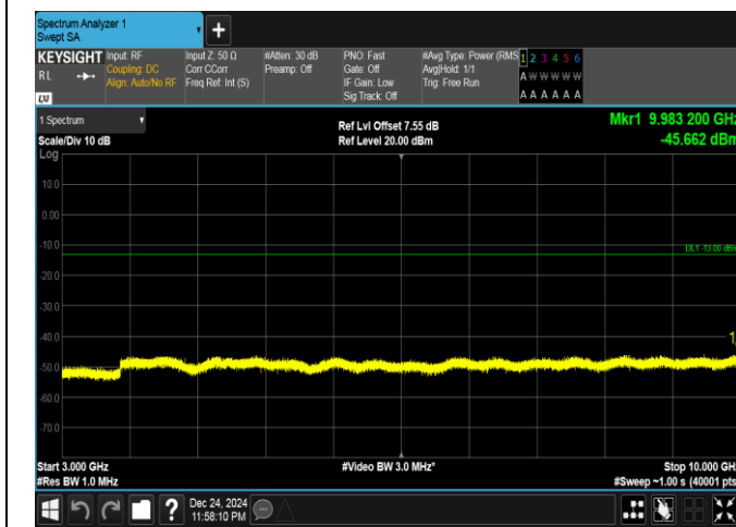
Band26(814-824)-1.4MHz-QPSK-26697-6RB#0-3000~10000-PASS
