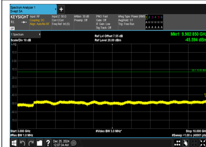
Band26(814-824)-1.4MHz-QPSK-26783-1RB#0-3000~10000-PASS
