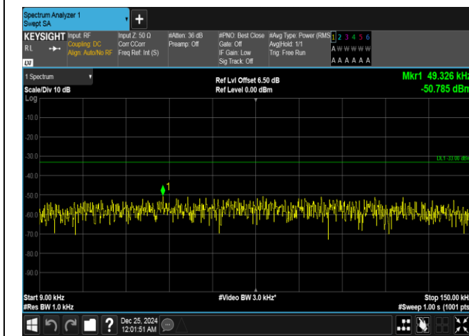
Band26(814-824)-1.4MHz-QPSK-26740-1RB#5-0.009~0.15-PASS
