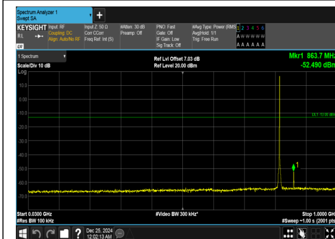
Band26(814-824)-1.4MHz-QPSK-26740-1RB#5-30~1000-PASS
