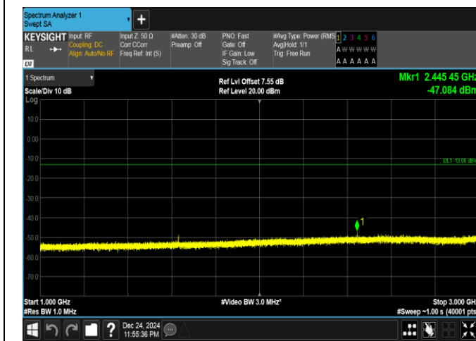
Band26(814-824)-1.4MHz-QPSK-26697-1RB#5-1000~3000-PASS
