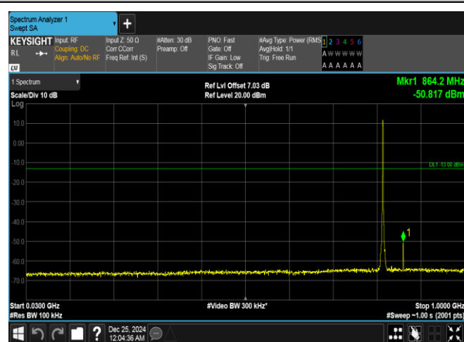
Band26(814-824)-1.4MHz-QPSK-26740-6RB#0-30~1000-PASS
