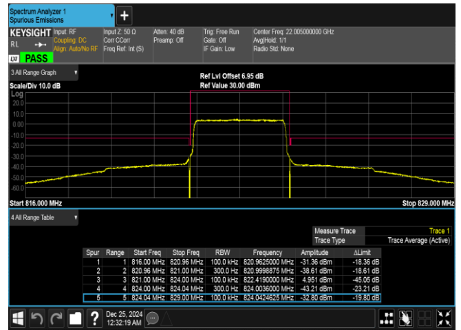
Band26(814-824)-3MHz-16QAM-26775-15RB#0-PASS
