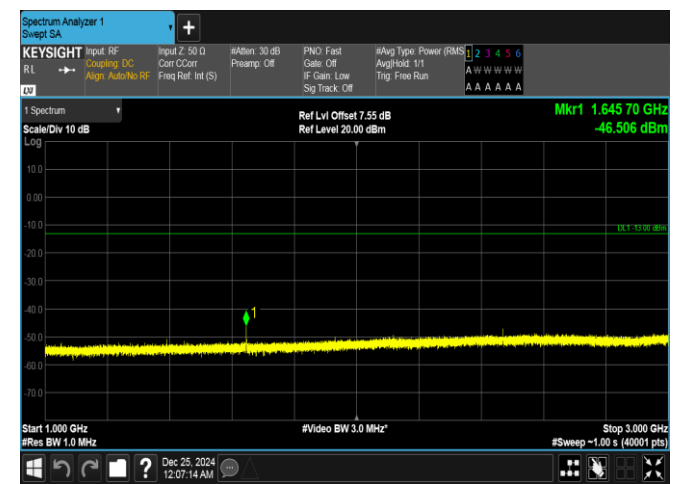
Band26(814-824)-1.4MHz-QPSK-26783-1RB#0-1000~3000-PASS
