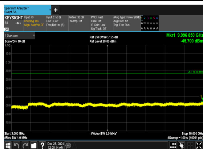
Band26(814-824)-1.4MHz-QPSK-26740-6RB#0-3000~10000-PASS
