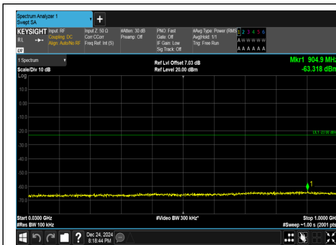
Band25-10MHz-QPSK-26090-50RB#0-30~1000-PASS
