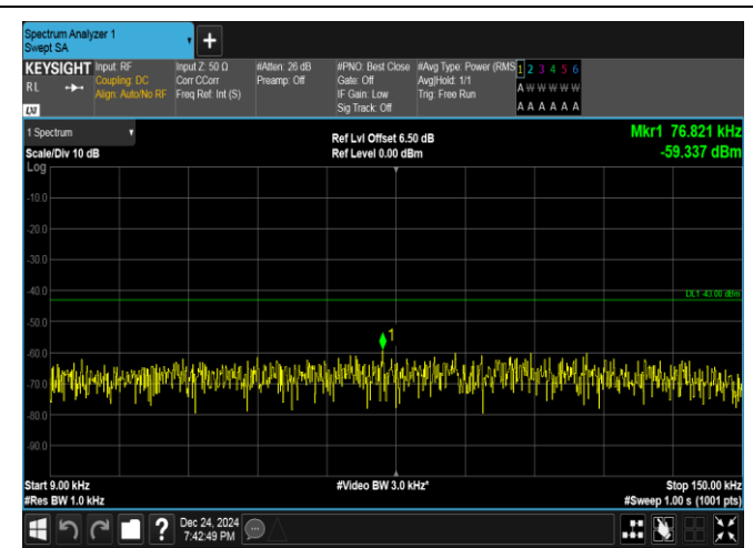
Band25-5MHz-16QAM-26665-25RB#0-0.009~0.15-PASS
