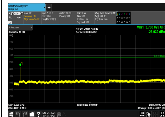
Band25-10MHz-QPSK-26090-1RB#0-3000~20000-PASS
