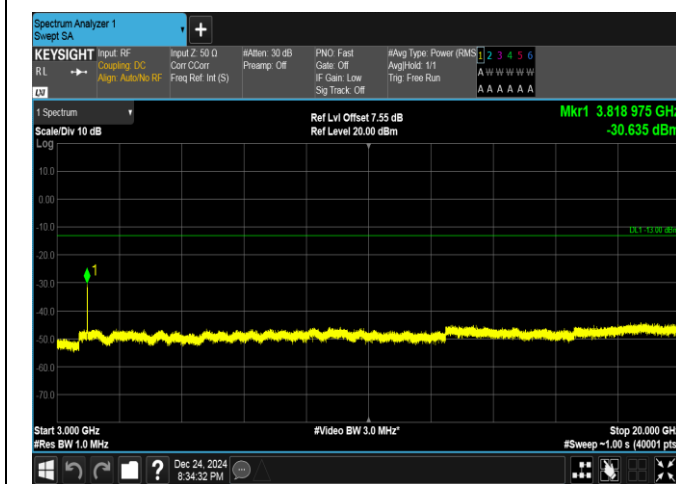
Band25-10MHz-QPSK-26640-50RB#0-3000~20000-PASS
