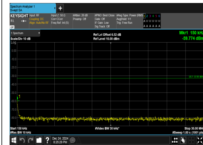
Band25-10MHz-QPSK-26365-50RB#0-0.15~30-PASS
