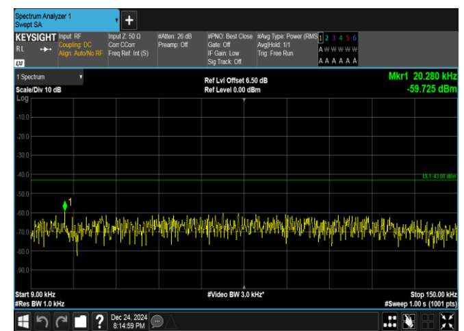
Band25-10MHz-16QAM-26090-1RB#0-0.009~0.15-PASS
