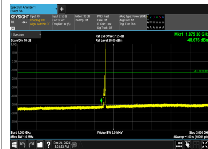
Band25-10MHz-QPSK-26640-1RB#49-1000~3000-PASS
