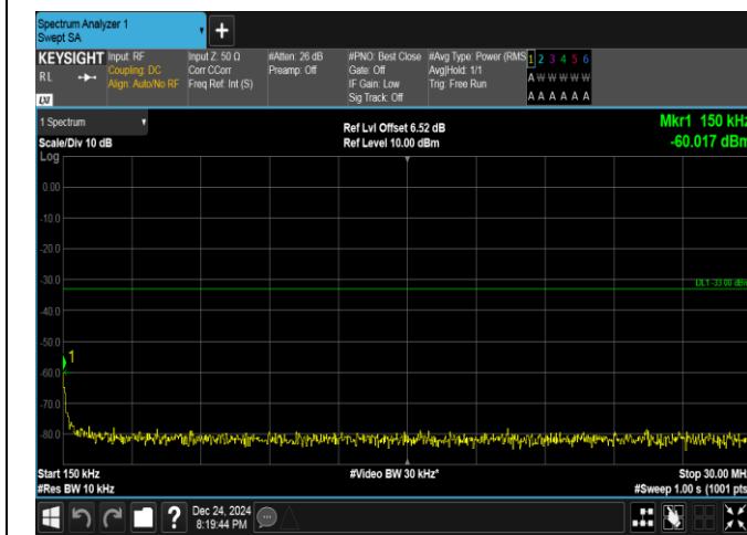
Band25-10MHz-16QAM-26090-50RB#0-0.15~30-PASS
