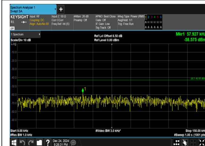
Band25-10MHz-16QAM-26365-50RB#0-0.009~0.15-PASS
