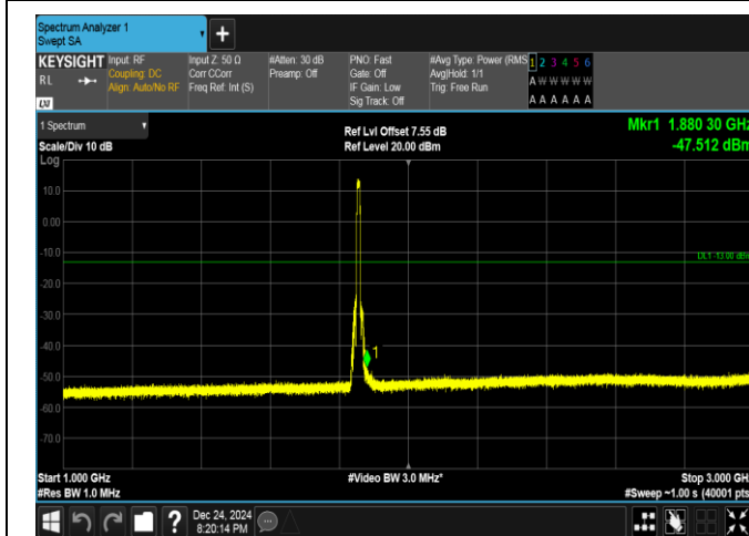
Band25-10MHz-16QAM-26090-50RB#0-1000~3000-PASS
