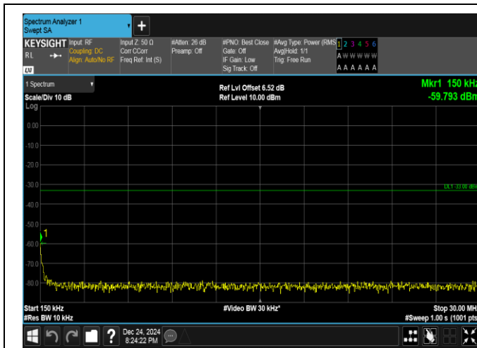
Band25-10MHz-16QAM-26365-1RB#49-0.15~30-PASS
