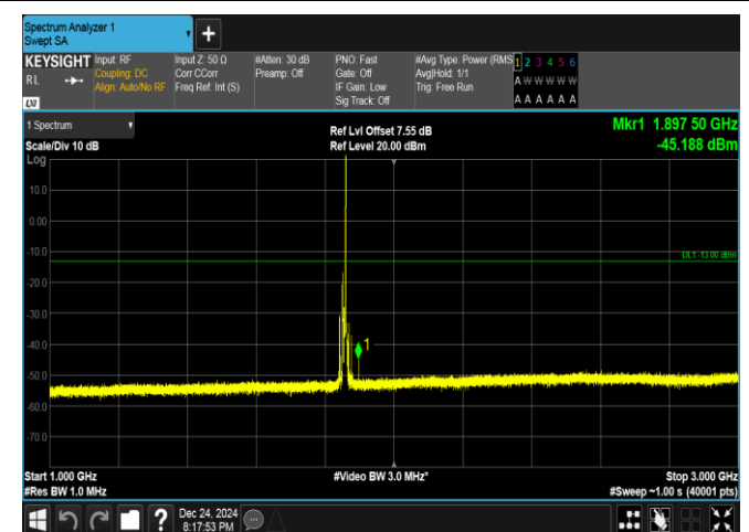
Band25-10MHz-16QAM-26090-1RB#49-1000~3000-PASS
