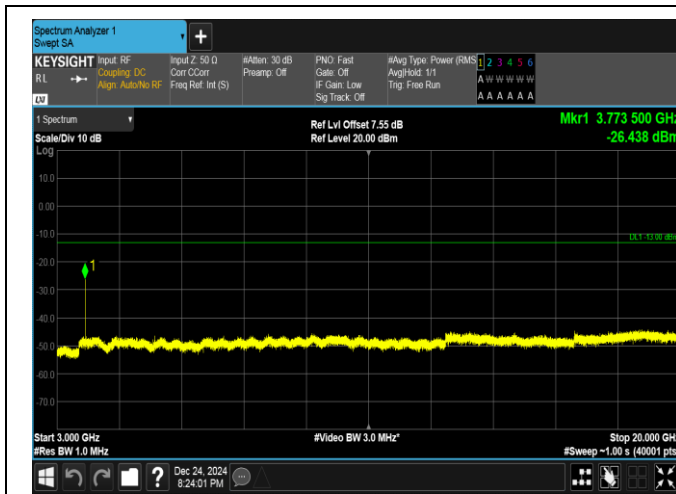
Band25-10MHz-QPSK-26365-1RB#49-3000~20000-PASS
