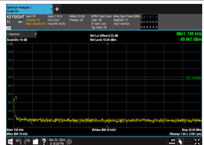
Band25-10MHz-QPSK-26090-50RB#0-0.15~30-PASS
