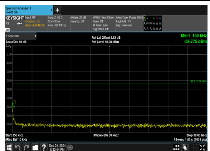
Band25-10MHz-QPSK-26640-50RB#0-0.15~30-PASS
