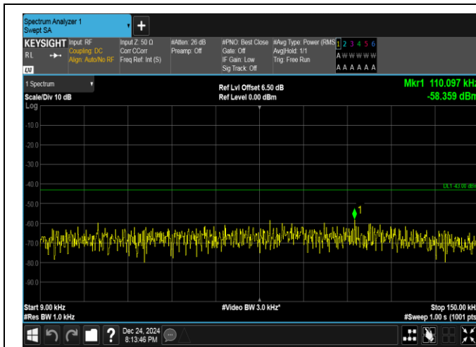
Band25-10MHz-QPSK-26090-1RB#0-0.009~0.15-PASS
