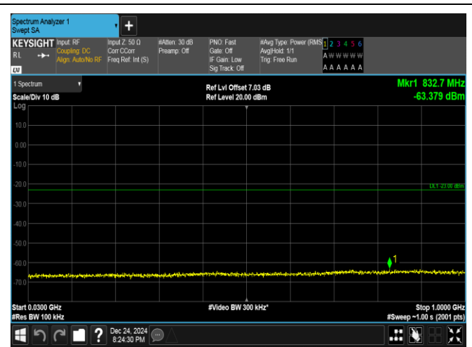
Band25-10MHz-16QAM-26365-1RB#49-30~1000-PASS
