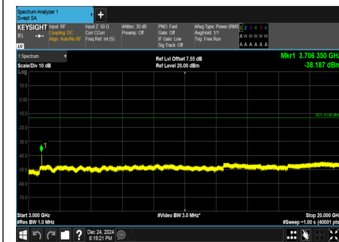
Band25-10MHz-QPSK-26090-50RB#0-3000~20000-PASS
