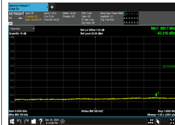
Band25-10MHz-QPSK-26090-1RB#0-30~1000-PASS
