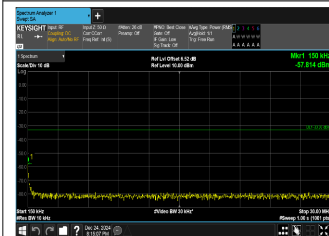
Band25-10MHz-16QAM-26090-1RB#0-0.15~30-PASS
