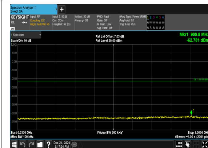
Band25-10MHz-16QAM-26090-1RB#49-30~1000-PASS
