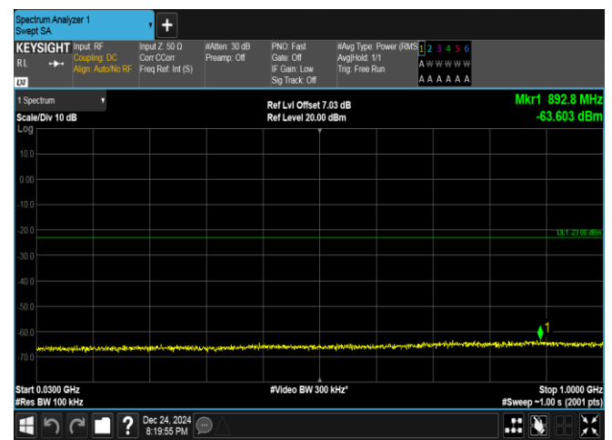
Band25-10MHz-16QAM-26090-50RB#0-30~1000-PASS
