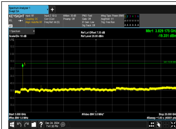
Band25-5MHz-16QAM-26665-1RB#24-3000~20000-PASS
