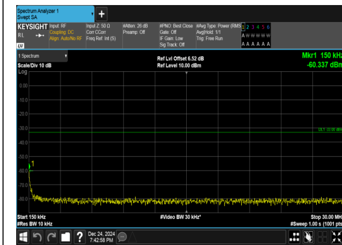
Band25-5MHz-16QAM-26665-25RB#0-0.15~30-PASS
