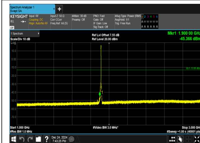
Band25-5MHz-16QAM-26665-25RB#0-1000~3000-PASS
