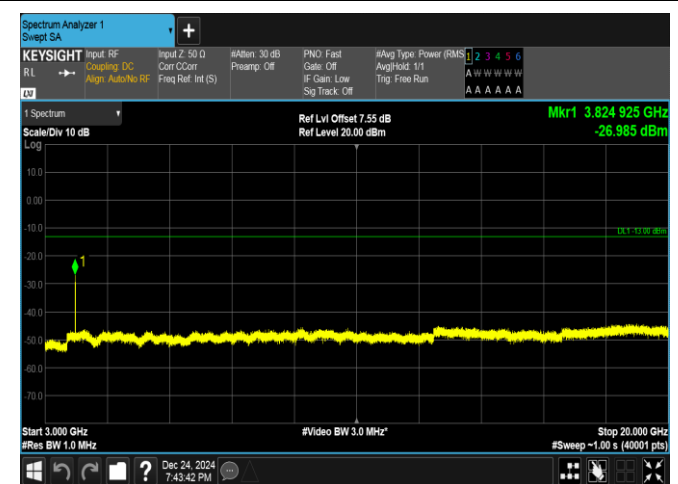
Band25-5MHz-16QAM-26665-25RB#0-3000~20000-PASS
