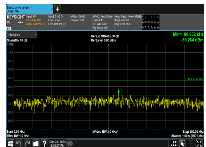
Band25-10MHz-QPSK-26090-1RB#49-0.009~0.15-PASS
