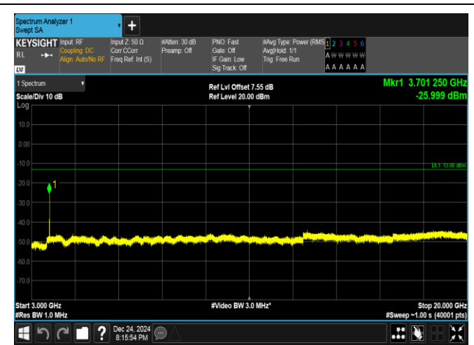
Band25-10MHz-16QAM-26090-1RB#0-3000~20000-PASS
