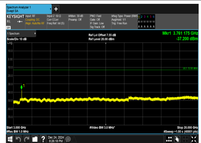
Band25-10MHz-QPSK-26365-50RB#0-3000~20000-PASS
