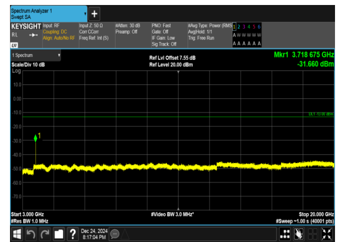
Band25-10MHz-QPSK-26090-1RB#49-3000~20000-PASS
