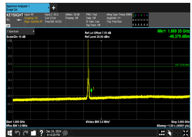
Band25-10MHz-QPSK-26090-1RB#0-1000~3000-PASS
