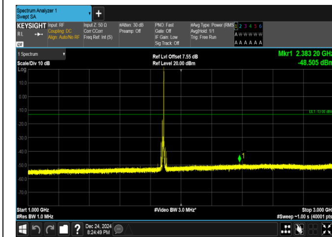
Band25-10MHz-16QAM-26365-1RB#49-1000~3000-PASS
