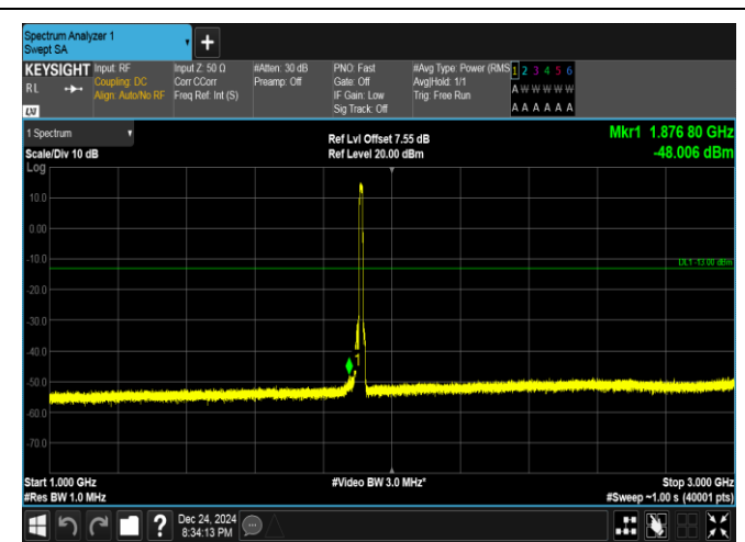
Band25-10MHz-QPSK-26640-50RB#0-1000~3000-PASS
