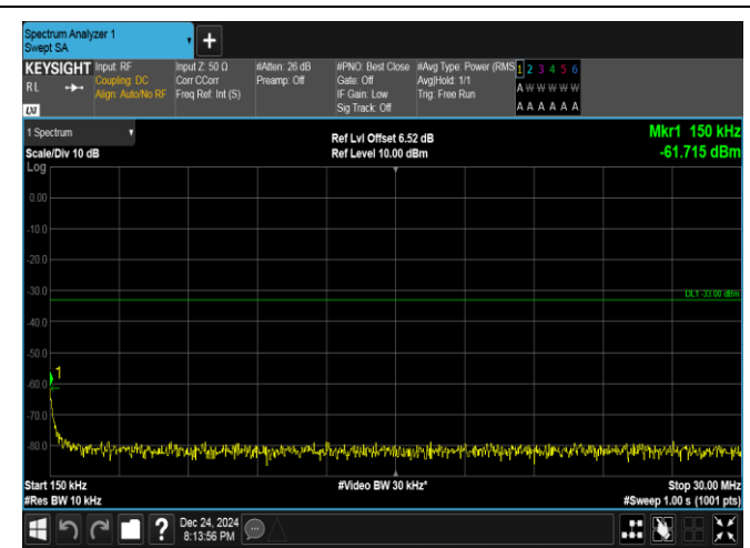
Band25-10MHz-QPSK-26090-1RB#0-0.15~30-PASS
