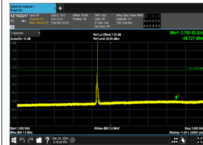
Band25-10MHz-QPSK-26090-1RB#49-1000~3000-PASS
