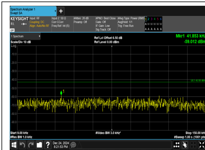
Band25-10MHz-16QAM-26365-1RB#0-0.009~0.15-PASS
