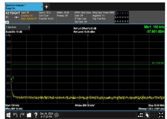
Band25-10MHz-16QAM-26090-1RB#49-0.15~30-PASS
