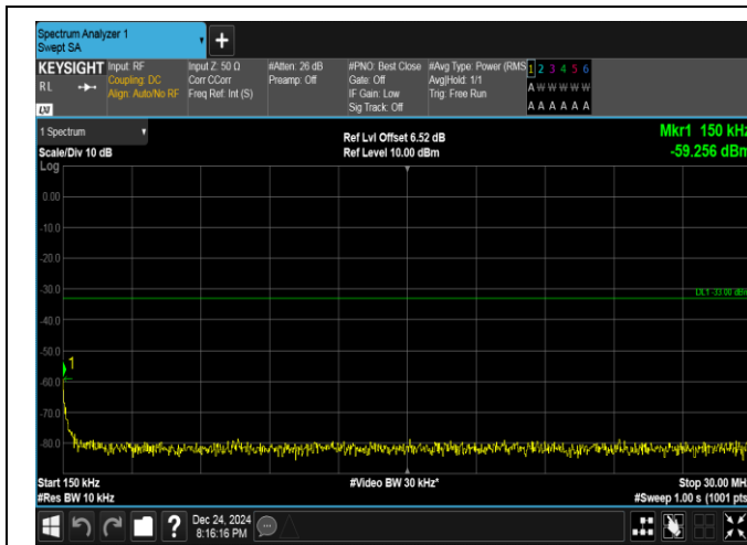
Band25-10MHz-QPSK-26090-1RB#49-0.15~30-PASS
