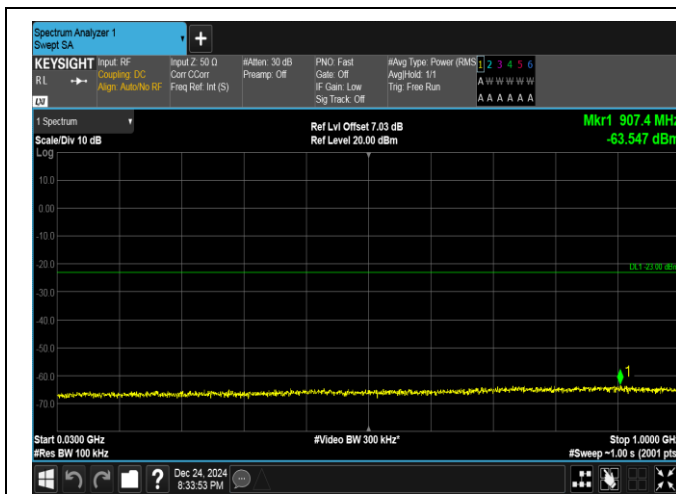
Band25-10MHz-QPSK-26640-50RB#0-30~1000-PASS
