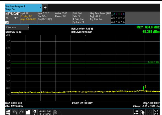
Band25-10MHz-16QAM-26090-1RB#0-30~1000-PASS
