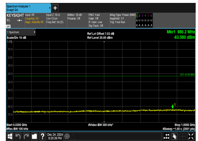
Band25-10MHz-QPSK-26365-50RB#0-30~1000-PASS
