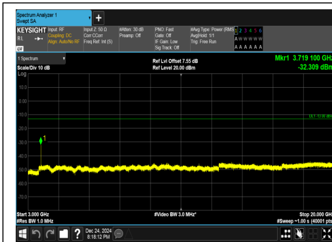
Band25-10MHz-16QAM-26090-1RB#49-3000~20000-PASS
