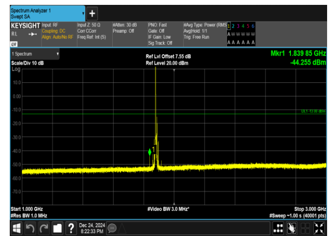
Band25-10MHz-16QAM-26365-1RB#0-1000~3000-PASS
