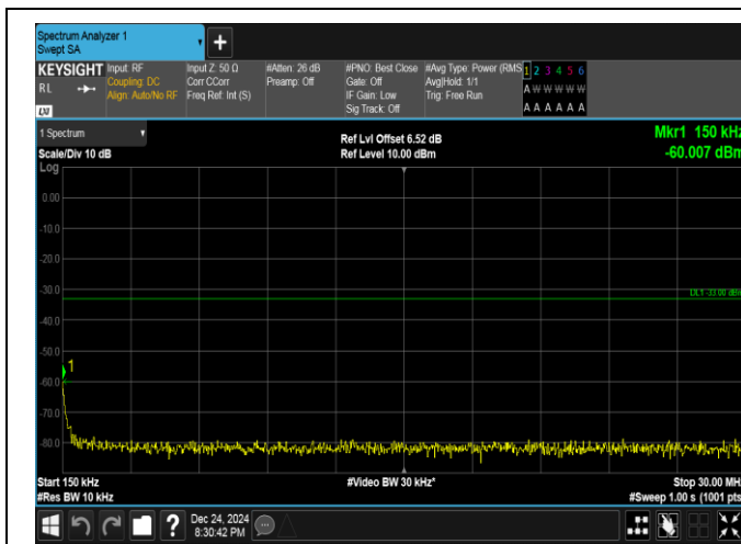
Band25-10MHz-QPSK-26640-1RB#49-0.15~30-PASS
