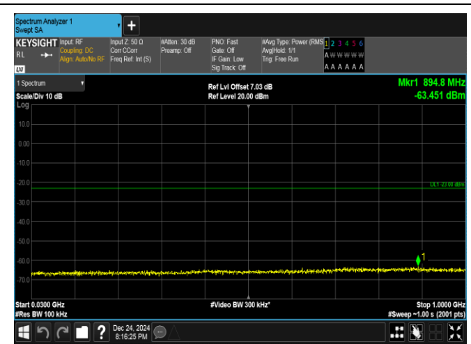
Band25-10MHz-QPSK-26090-1RB#49-30~1000-PASS
