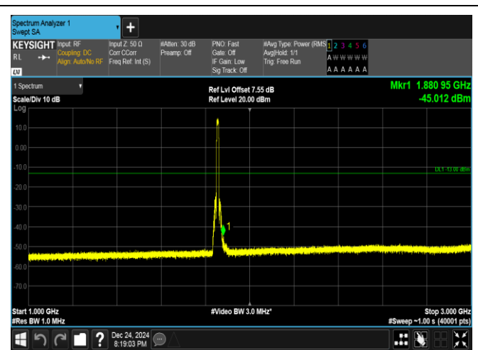
Band25-10MHz-QPSK-26090-50RB#0-1000~3000-PASS
