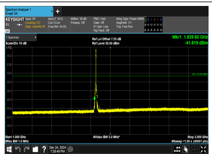
Band25-5MHz-QPSK-26065-25RB#0-1000~3000-PASS
