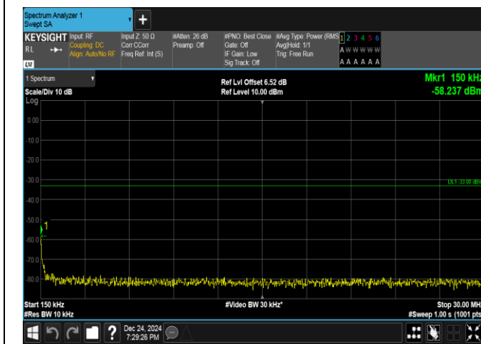
Band25-5MHz-16QAM-26065-25RB#0-0.15~30-PASS
