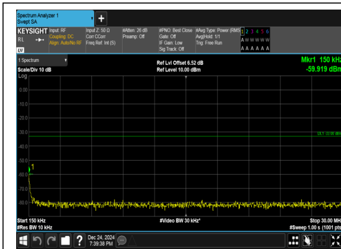
Band25-5MHz-QPSK-26665-1RB#24-0.15~30-PASS
