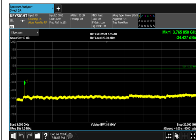
Band25-5MHz-16QAM-26365-25RB#0-3000~20000-PASS
