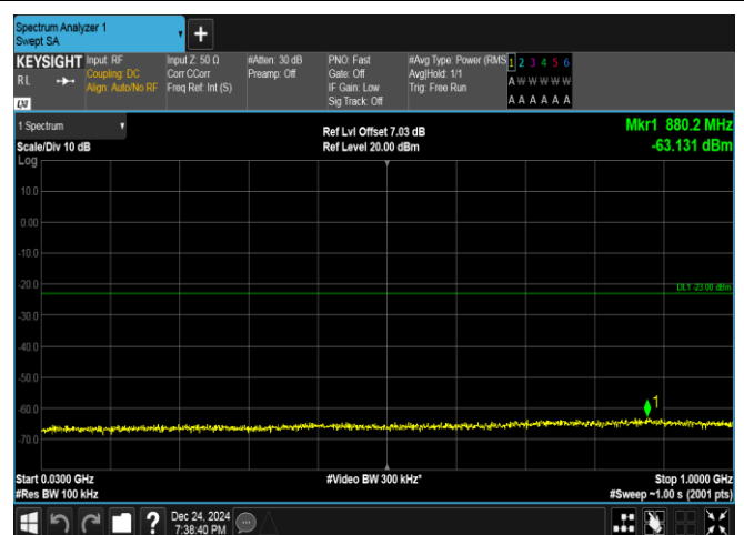
Band25-5MHz-16QAM-26665-1RB#0-30~1000-PASS
