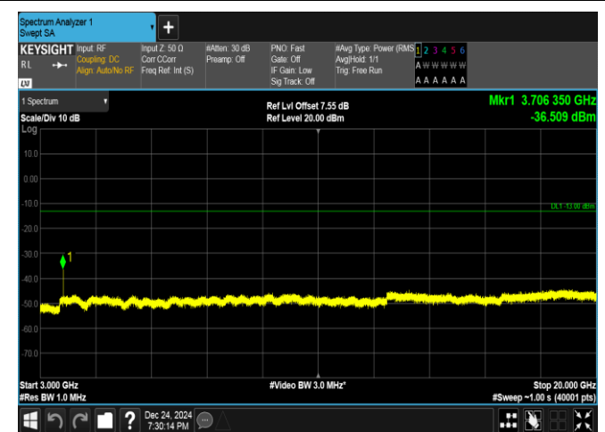
Band25-5MHz-16QAM-26065-25RB#0-3000~20000-PASS
