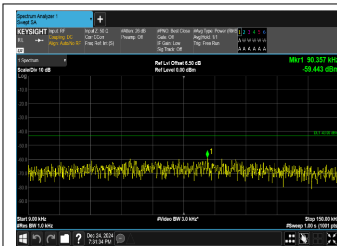
Band25-5MHz-16QAM-26365-1RB#0-0.009~0.15-PASS
