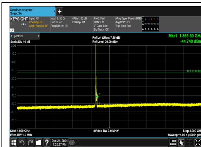
Band25-5MHz-16QAM-26065-1RB#0-1000~3000-PASS
