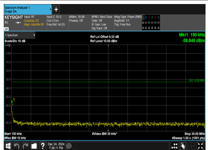
Band25-5MHz-16QAM-26365-25RB#0-0.15~30-PASS
