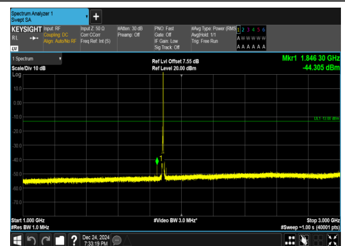
Band25-5MHz-QPSK-26365-1RB#24-1000~3000-PASS
