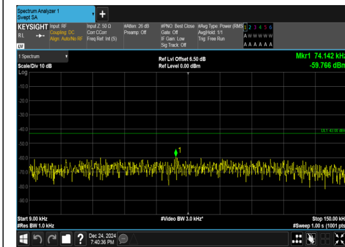
Band25-5MHz-16QAM-26665-1RB#24-0.009~0.15-PASS
