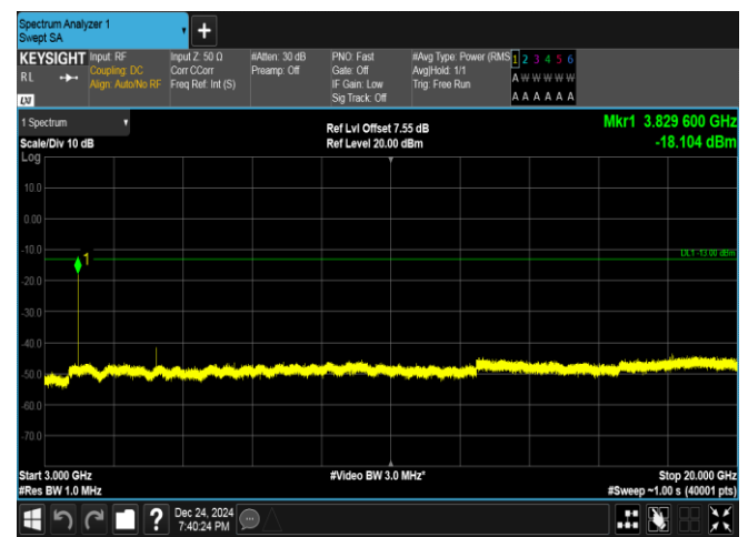
Band25-5MHz-QPSK-26665-1RB#24-3000~20000-PASS
