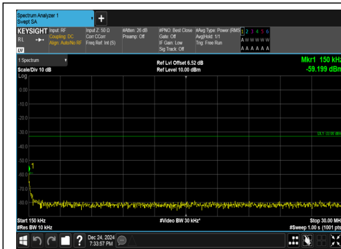
Band25-5MHz-16QAM-26365-1RB#24-0.15~30-PASS
