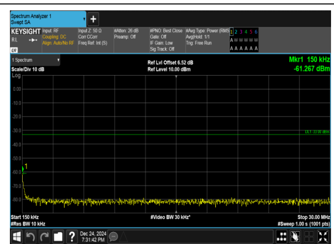
Band25-5MHz-16QAM-26365-1RB#0-0.15~30-PASS
