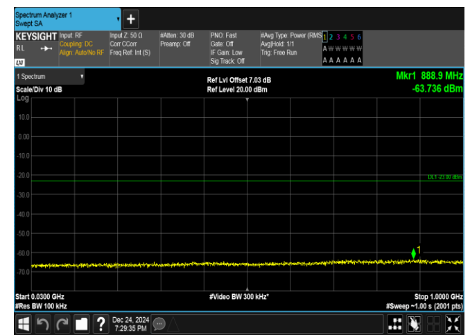
Band25-5MHz-16QAM-26065-25RB#0-30~1000-PASS
