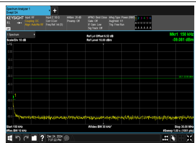
Band25-5MHz-QPSK-26665-1RB#0-0.15~30-PASS
