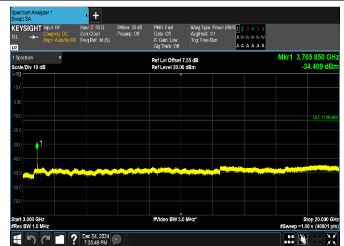
Band25-5MHz-QPSK-26365-25RB#0-3000~20000-PASS
