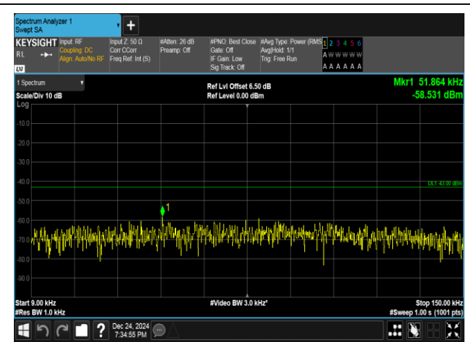
Band25-5MHz-QPSK-26365-25RB#0-0.009~0.15-PASS
