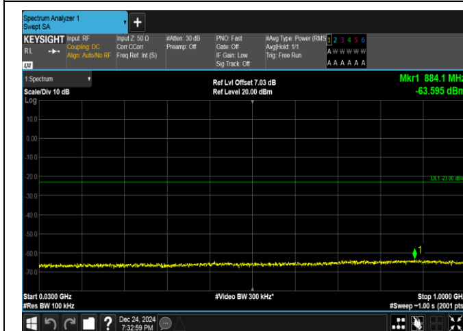
Band25-5MHz-QPSK-26365-1RB#24-30~1000-PASS
