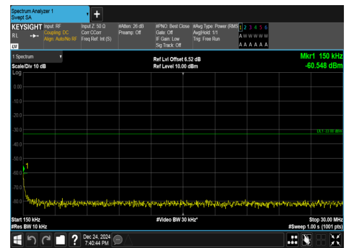
Band25-5MHz-16QAM-26665-1RB#24-0.15~30-PASS
