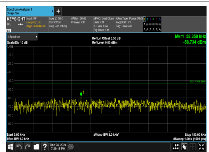
Band25-5MHz-16QAM-26065-25RB#0-0.009~0.15-PASS
