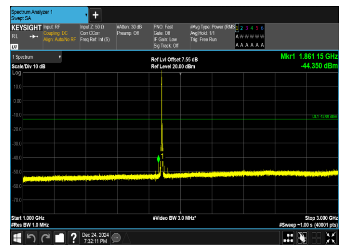
Band25-5MHz-16QAM-26365-1RB#0-1000~3000-PASS
