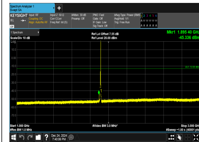
Band25-5MHz-QPSK-26665-1RB#24-1000~3000-PASS
