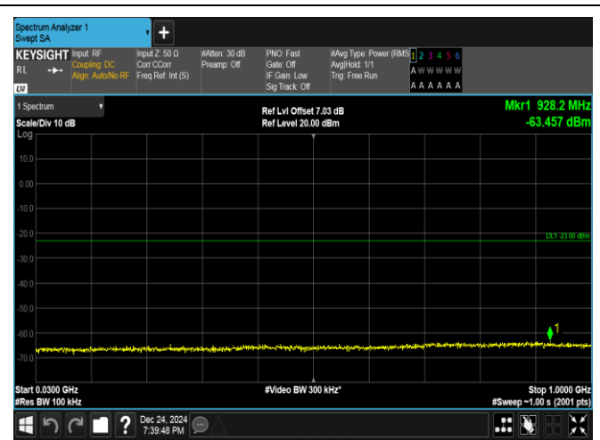
Band25-5MHz-QPSK-26665-1RB#24-30~1000-PASS
