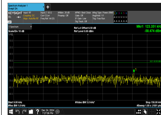
Band25-5MHz-16QAM-26065-1RB#24-0.009~0.15-PASS
