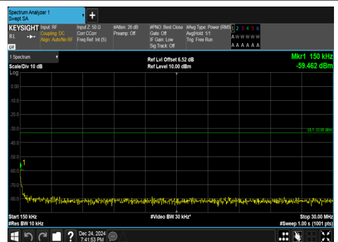
Band25-5MHz-QPSK-26665-25RB#0-0.15~30-PASS
