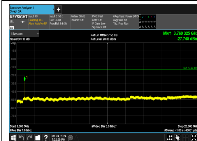
Band25-5MHz-16QAM-26365-1RB#0-3000~20000-PASS
