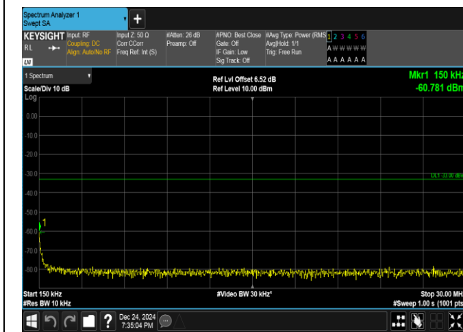
Band25-5MHz-QPSK-26365-25RB#0-0.15~30-PASS
