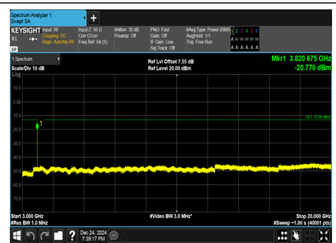
Band25-5MHz-16QAM-26665-1RB#0-3000~20000-PASS
