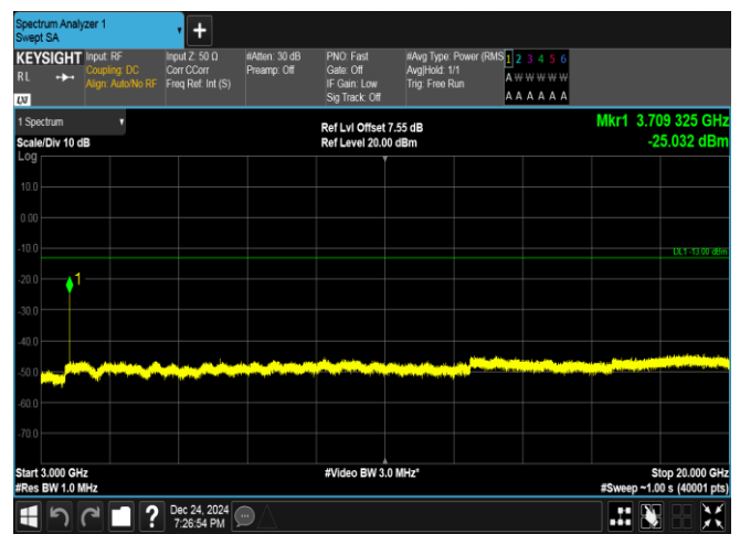
Band25-5MHz-QPSK-26065-1RB#24-3000~20000-PASS
