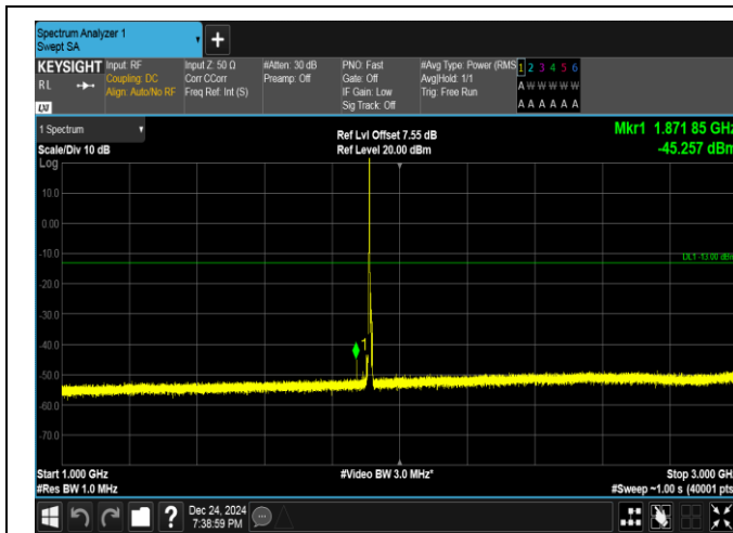
Band25-5MHz-16QAM-26665-1RB#0-1000~3000-PASS
