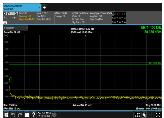
Band25-5MHz-QPSK-26065-25RB#0-0.15~30-PASS
