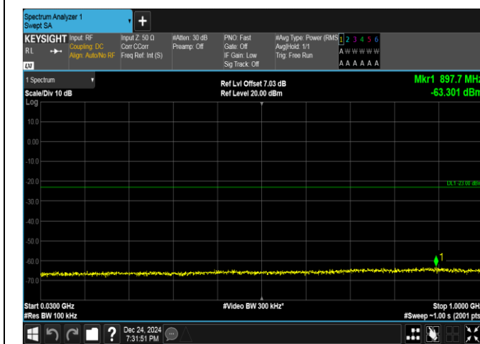
Band25-5MHz-16QAM-26365-1RB#0-30~1000-PASS
