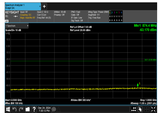
Band25-5MHz-QPSK-26365-25RB#0-30~1000-PASS
