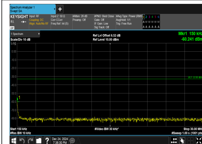
Band25-5MHz-16QAM-26665-1RB#0-0.15~30-PASS
