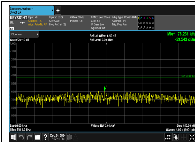
Band25-5MHz-QPSK-26665-1RB#0-0.009~0.15-PASS
