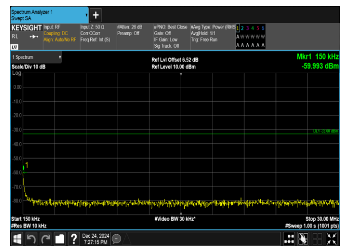
Band25-5MHz-16QAM-26065-1RB#24-0.15~30-PASS
