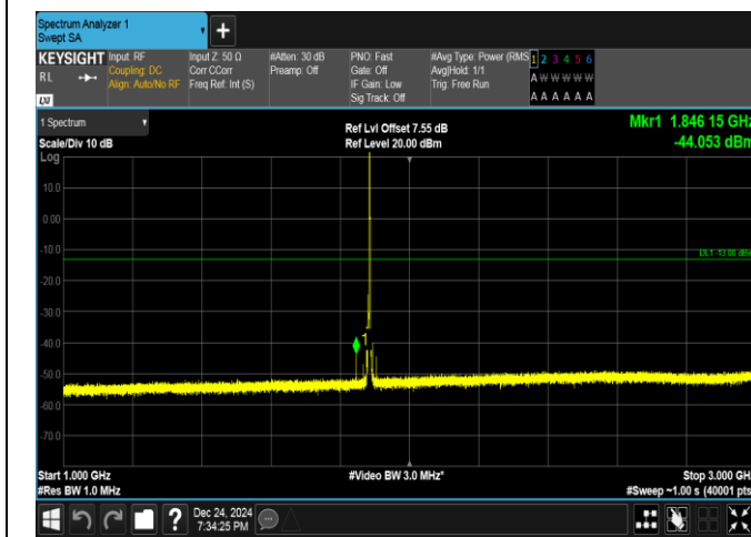
Band25-5MHz-16QAM-26365-1RB#24-1000~3000-PASS
