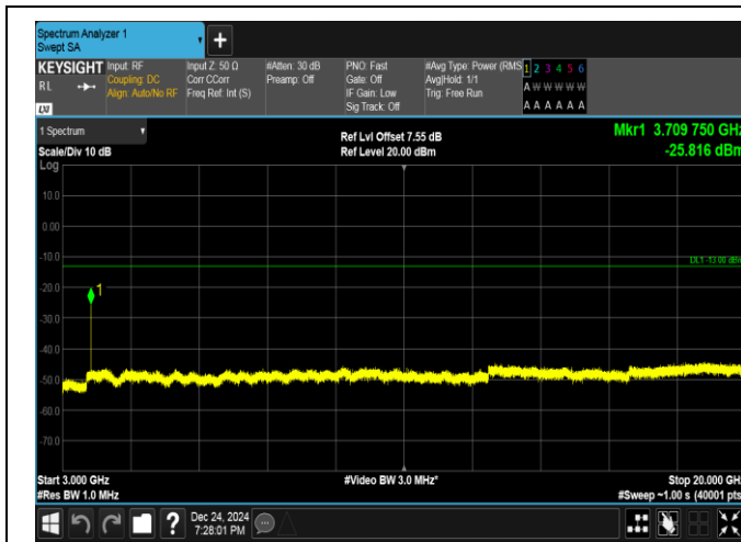
Band25-5MHz-16QAM-26065-1RB#24-3000~20000-PASS
