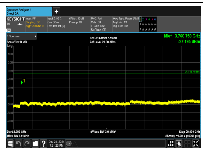
Band25-5MHz-QPSK-26365-1RB#0-3000~20000-PASS
