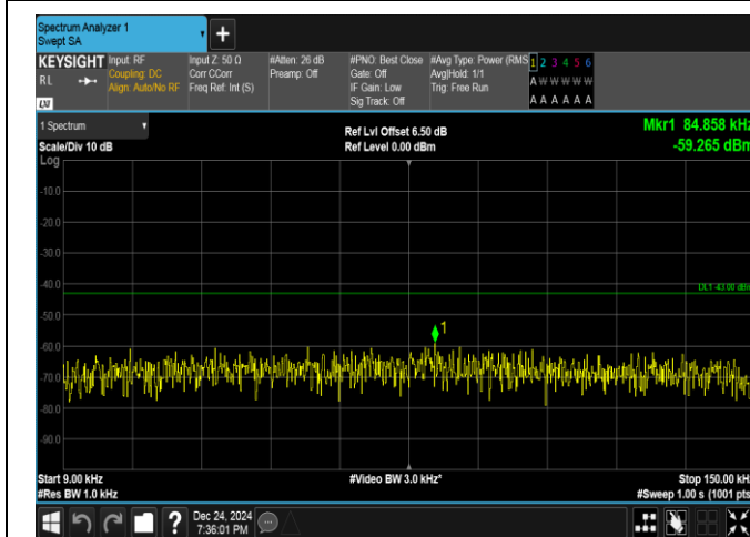
Band25-5MHz-16QAM-26365-25RB#0-0.009~0.15-PASS
