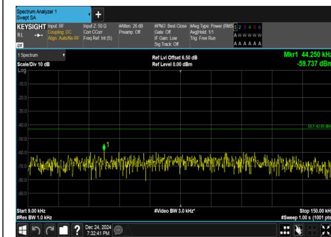
Band25-5MHz-QPSK-26365-1RB#24-0.009~0.15-PASS
