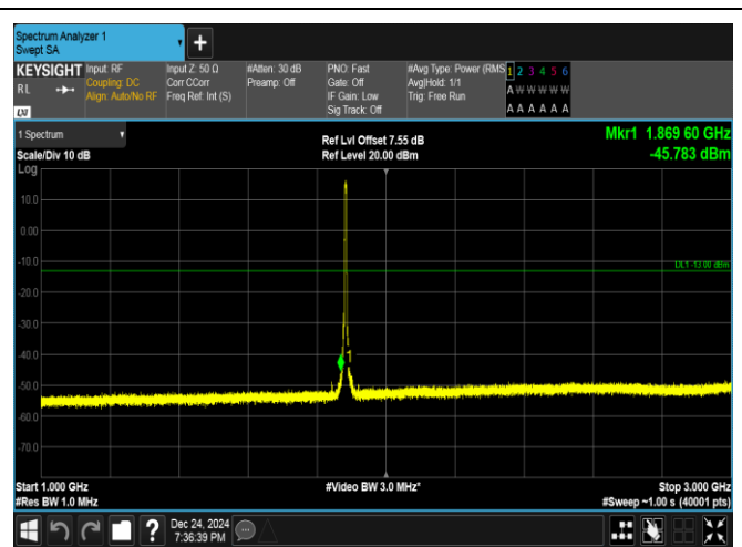
Band25-5MHz-16QAM-26365-25RB#0-1000~3000-PASS
