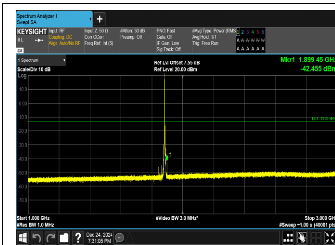
Band25-5MHz-QPSK-26365-1RB#0-1000~3000-PASS
