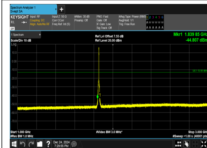
Band25-5MHz-16QAM-26065-25RB#0-1000~3000-PASS
