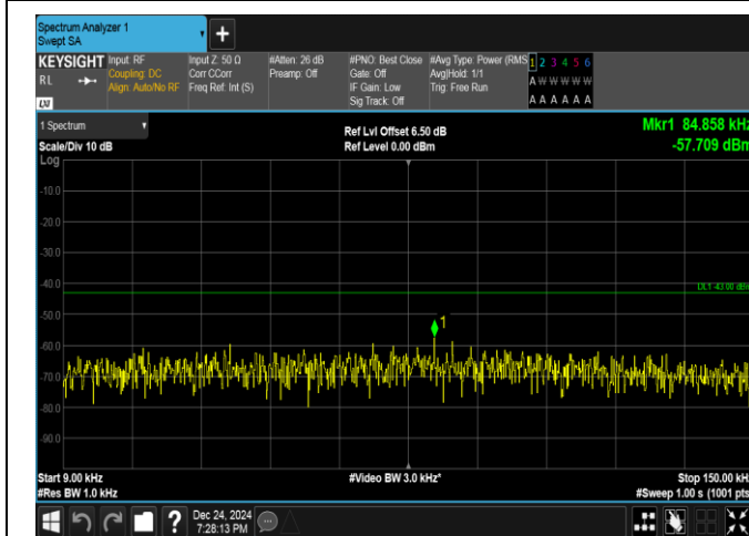
Band25-5MHz-QPSK-26065-25RB#0-0.009~0.15-PASS
