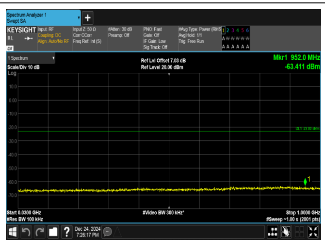
Band25-5MHz-QPSK-26065-1RB#24-30~1000-PASS
