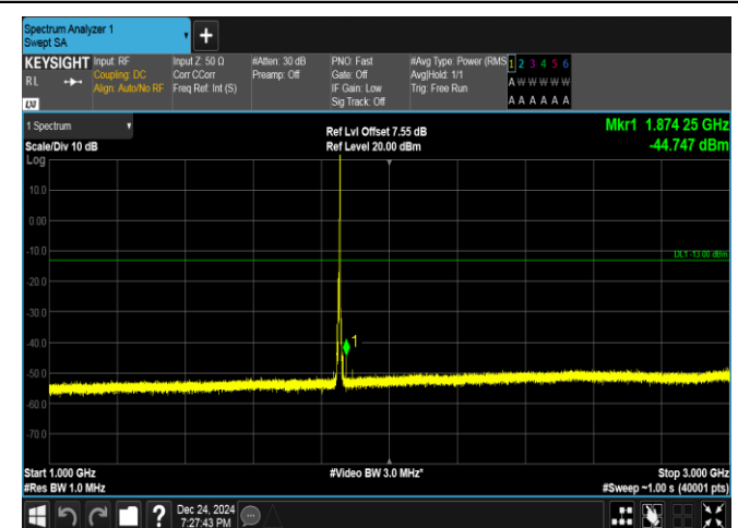
Band25-5MHz-16QAM-26065-1RB#24-1000~3000-PASS
