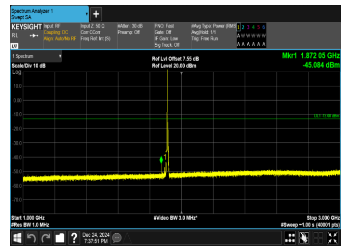
Band25-5MHz-QPSK-26665-1RB#0-1000~3000-PASS
