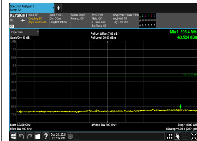
Band25-5MHz-QPSK-26665-1RB#0-30~1000-PASS
