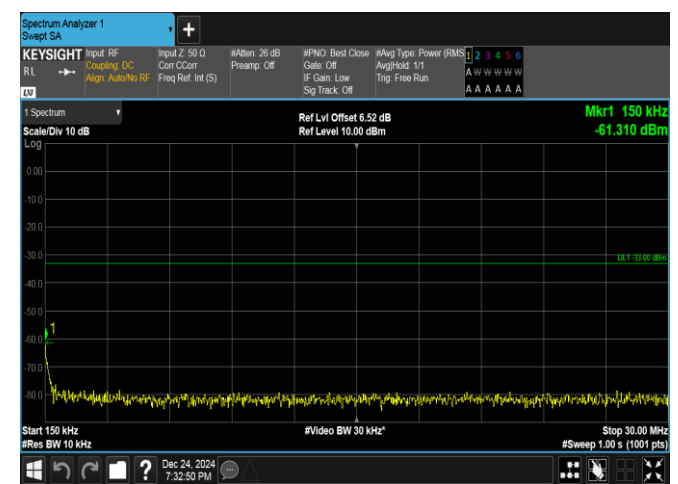
Band25-5MHz-QPSK-26365-1RB#24-0.15~30-PASS
