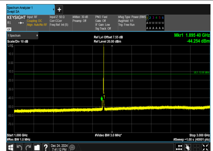
Band25-5MHz-16QAM-26665-1RB#24-1000~3000-PASS
