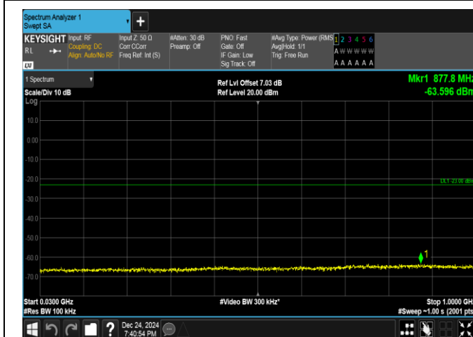
Band25-5MHz-16QAM-26665-1RB#24-30~1000-PASS
