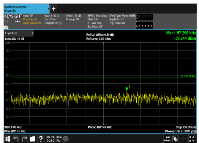
Band25-5MHz-16QAM-26665-1RB#0-0.009~0.15-PASS
