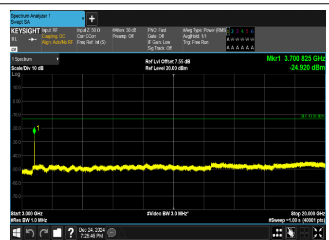
Band25-5MHz-16QAM-26065-1RB#0-3000~20000-PASS
