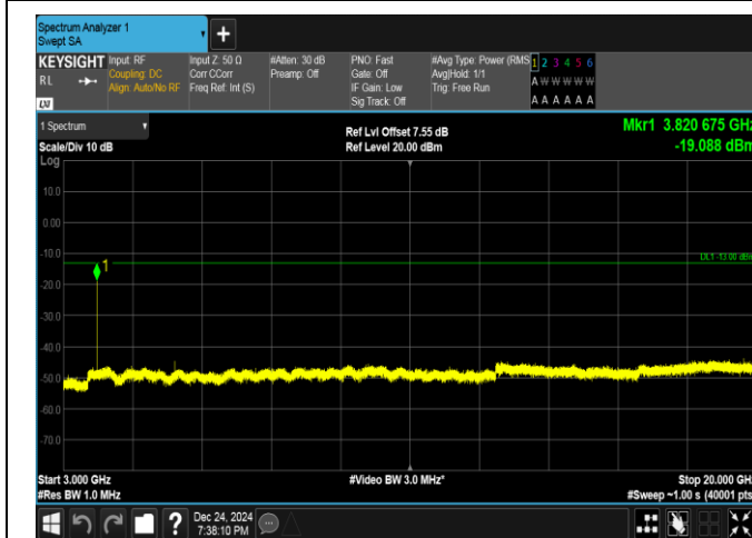
Band25-5MHz-QPSK-26665-1RB#0-3000~20000-PASS
