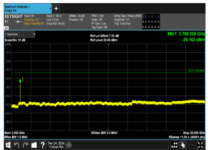
Band25-5MHz-16QAM-26365-1RB#24-3000~20000-PASS
