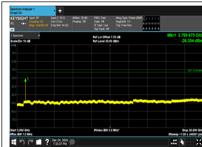
Band25-5MHz-QPSK-26365-1RB#24-3000~20000-PASS
