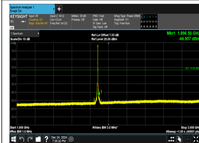
Band25-5MHz-QPSK-26365-25RB#0-1000~3000-PASS
