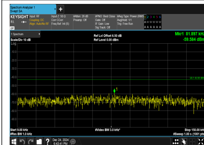
Band25-3MHz-16QAM-26365-15RB#0-0.009~0.15-PASS
