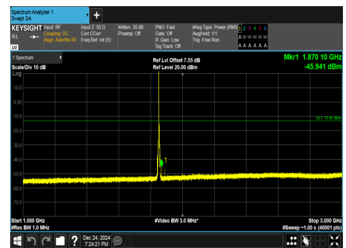
Band25-5MHz-QPSK-26065-1RB#0-1000~3000-PASS
