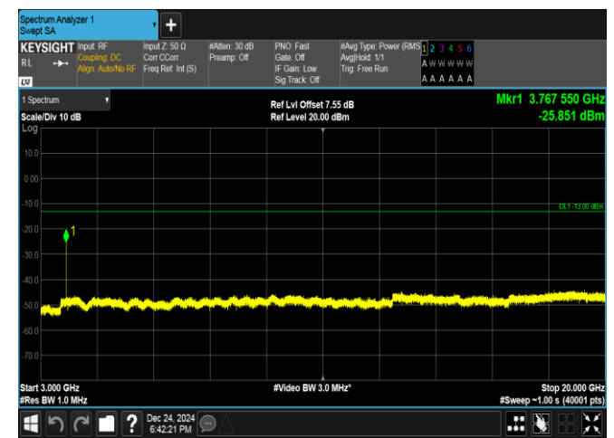
Band25-3MHz-16QAM-26365-1RB#14-3000~20000-PASS
