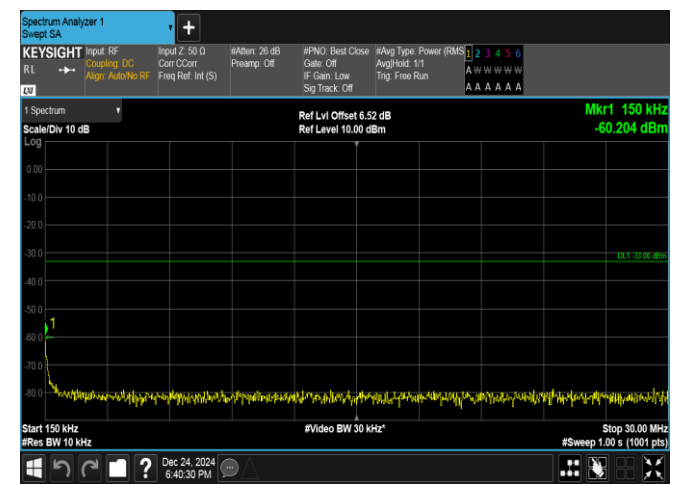
Band25-3MHz-QPSK-26365-1RB#14-0.15~30-PASS
