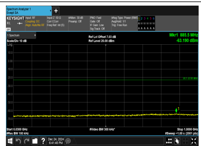
Band25-3MHz-16QAM-26365-1RB#14-30~1000-PASS
