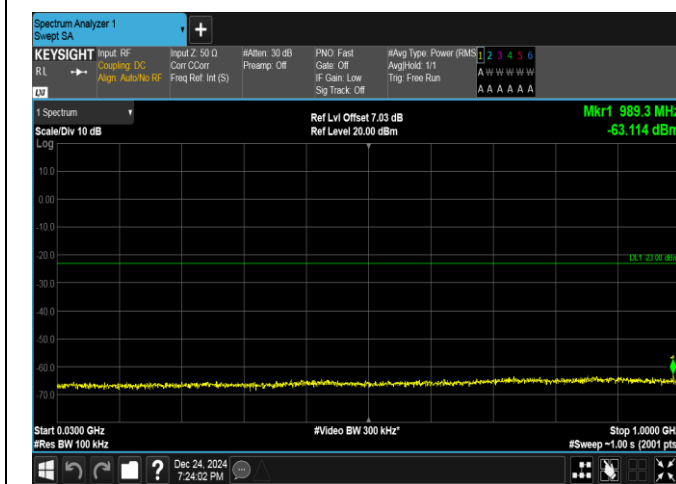
Band25-5MHz-QPSK-26065-1RB#0-30~1000-PASS
