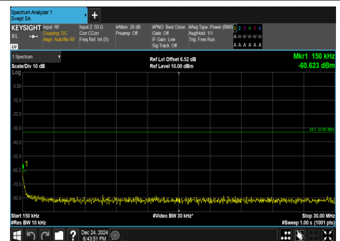
Band25-3MHz-16QAM-26365-15RB#0-0.15~30-PASS
