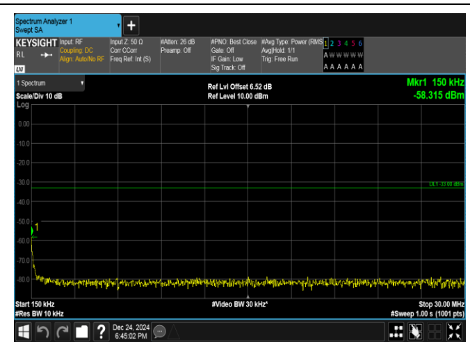
Band25-3MHz-QPSK-26675-1RB#0-0.15~30-PASS
