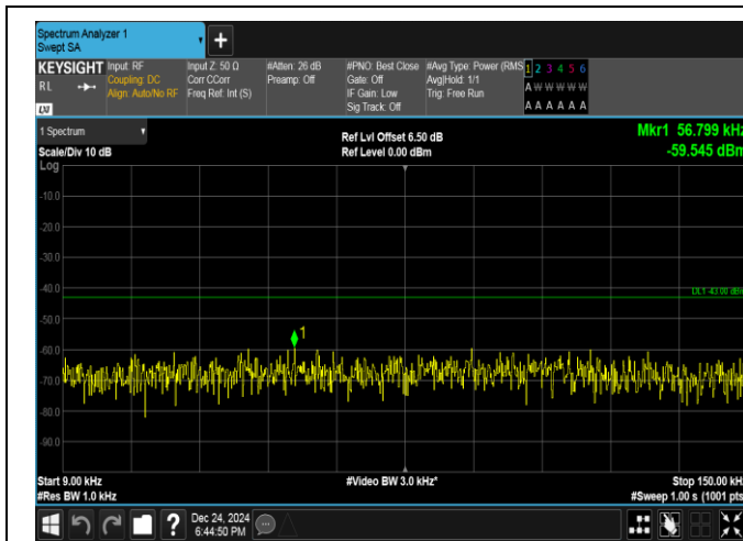
Band25-3MHz-QPSK-26675-1RB#0-0.009~0.15-PASS
