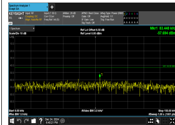
Band25-3MHz-QPSK-26365-1RB#14-0.009~0.15-PASS
