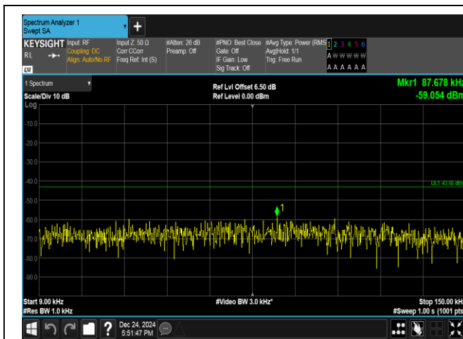
Band25-1.4MHz-QPSK-26683-1RB#0-0.009~0.15-PASS
