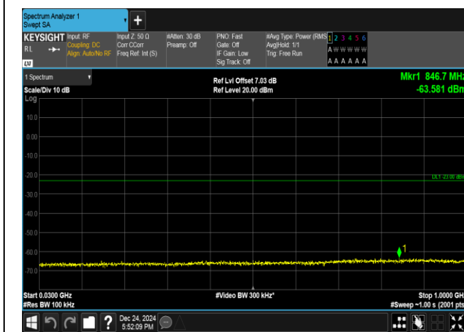
Band25-1.4MHz-QPSK-26683-1RB#0-30~1000-PASS
