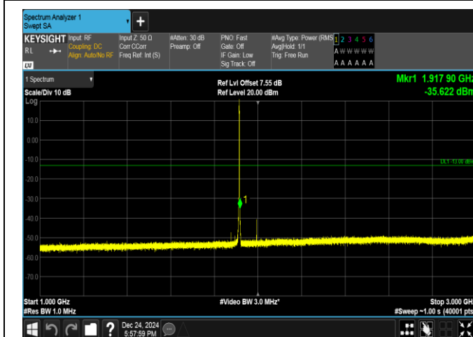
Band25-1.4MHz-16QAM-26683-6RB#0-1000~3000-PASS
