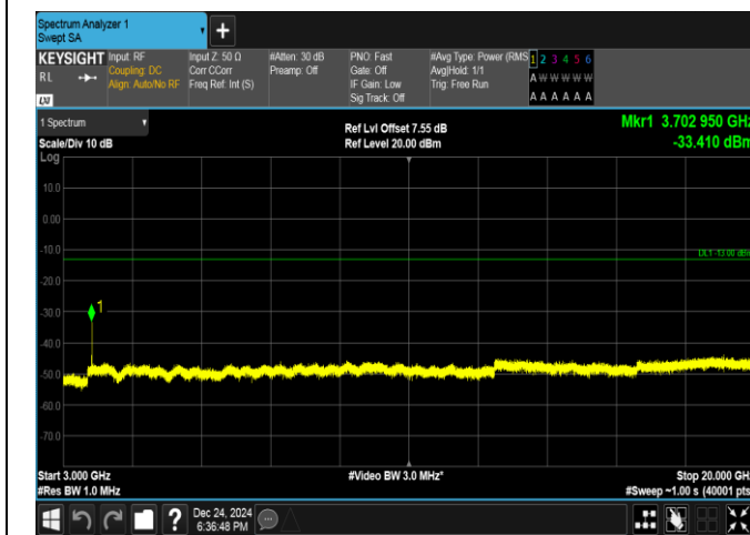
Band25-3MHz-QPSK-26055-15RB#0-3000~20000-PASS
