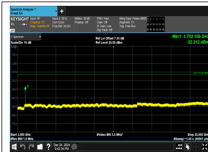
Band25-1.4MHz-16QAM-26047-1RB#5-3000~20000-PASS
