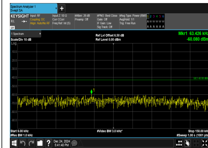
Band25-1.4MHz-16QAM-26047-1RB#5-0.009~0.15-PASS
