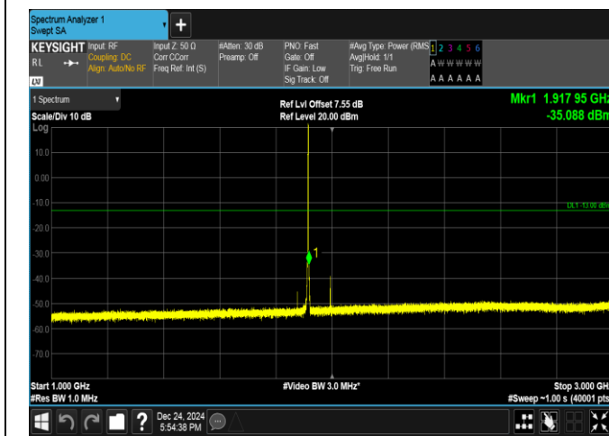
Band25-1.4MHz-QPSK-26683-1RB#5-1000~3000-PASS
