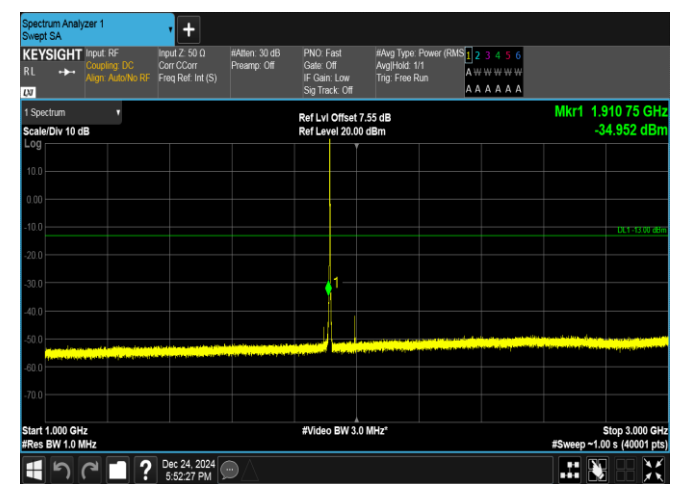
Band25-1.4MHz-QPSK-26683-1RB#0-1000~3000-PASS
