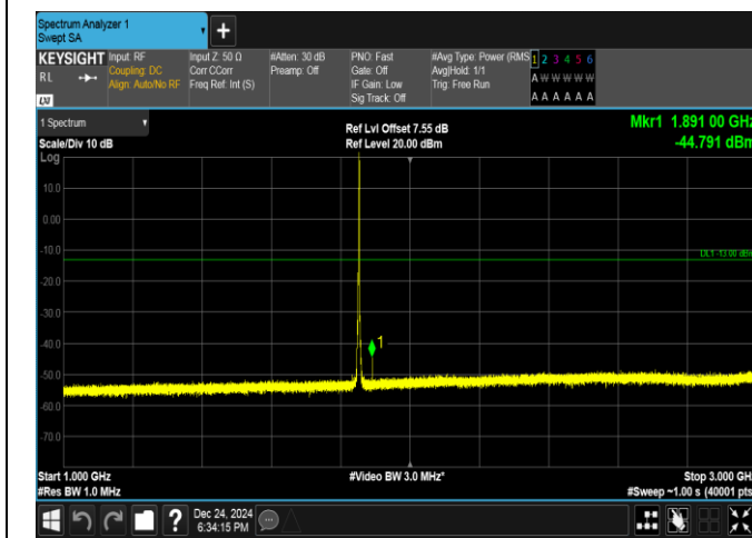
Band25-3MHz-QPSK-26055-1RB#14-1000~3000-PASS
