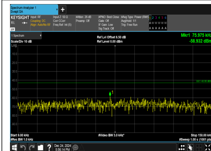
Band25-1.4MHz-QPSK-26683-6RB#0-0.009~0.15-PASS
