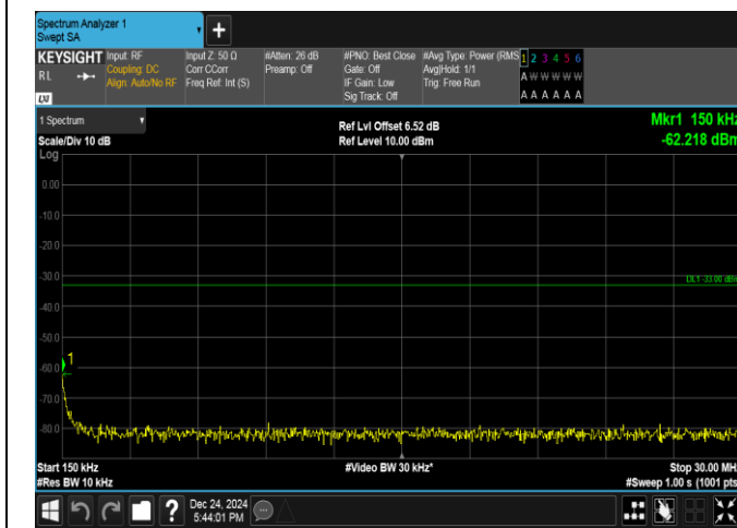
Band25-1.4MHz-16QAM-26047-6RB#0-0.15~30-PASS
