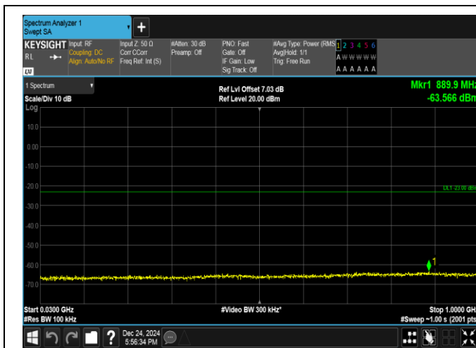
Band25-1.4MHz-QPSK-26683-6RB#0-30~1000-PASS
