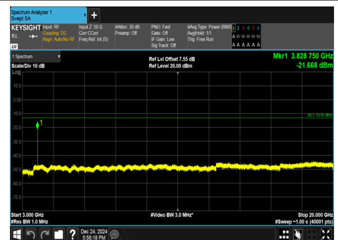
Band25-1.4MHz-16QAM-26683-6RB#0-3000~20000-PASS
