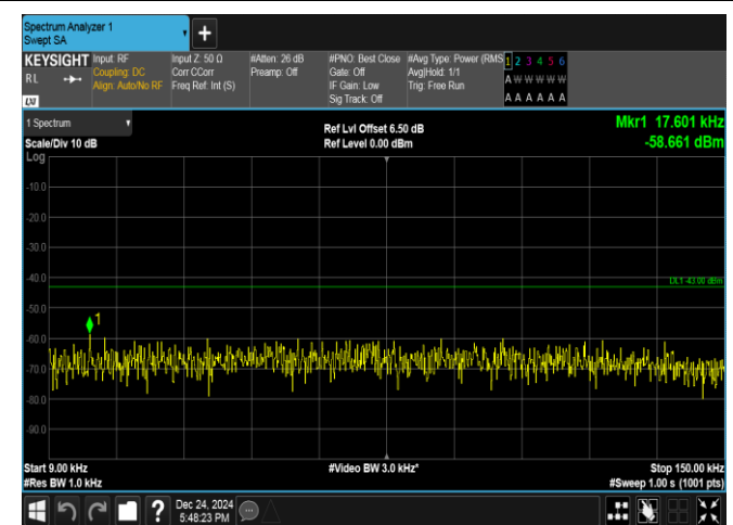
Band25-1.4MHz-16QAM-26365-1RB#5-0.009~0.15-PASS
