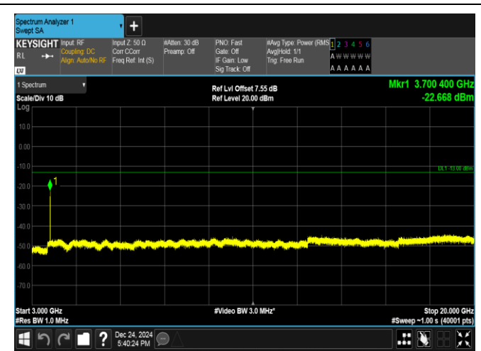
Band25-1.4MHz-16QAM-26047-1RB#0-3000~20000-PASS
