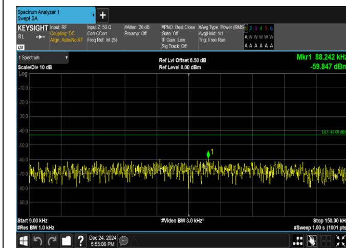
Band25-1.4MHz-16QAM-26683-1RB#5-0.009~0.15-PASS
