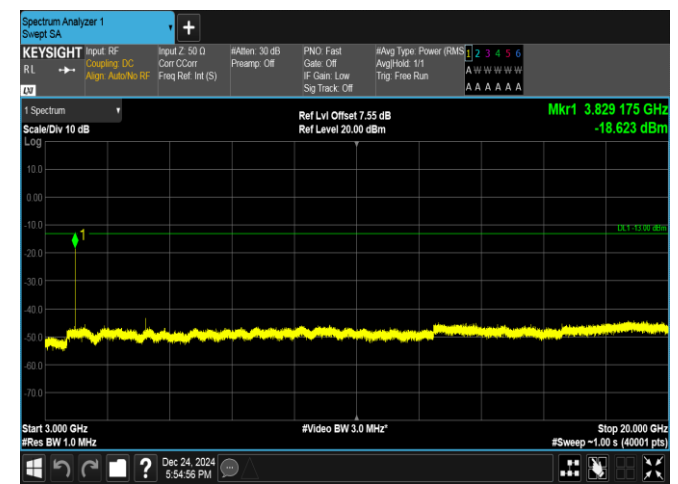
Band25-1.4MHz-QPSK-26683-1RB#5-3000~20000-PASS
