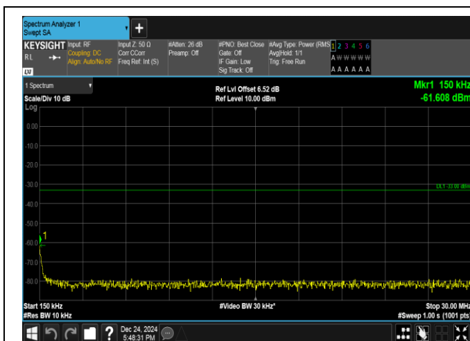
Band25-1.4MHz-16QAM-26365-1RB#5-0.15~30-PASS
