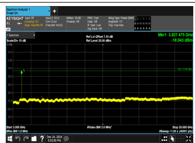
Band25-1.4MHz-16QAM-26683-1RB#0-3000~20000-PASS
