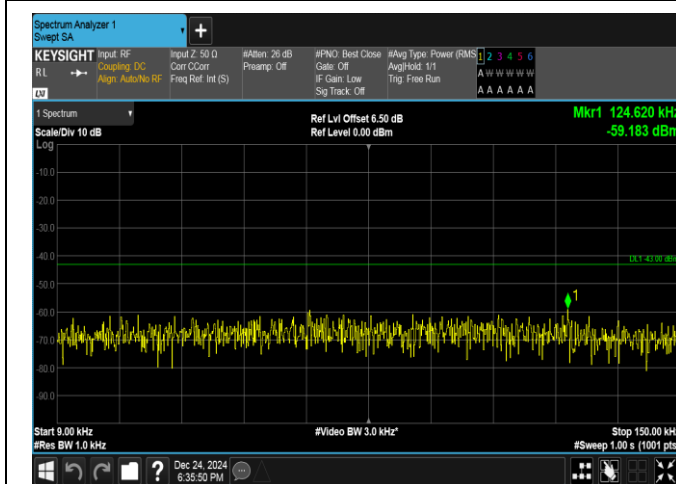
Band25-3MHz-QPSK-26055-15RB#0-0.009~0.15-PASS
