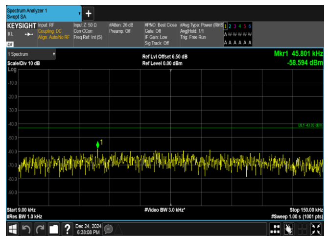
Band25-3MHz-QPSK-26365-1RB#0-0.009~0.15-PASS
