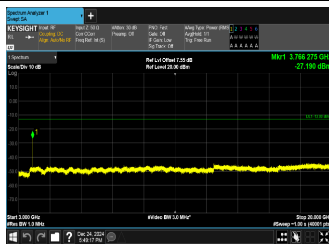
Band25-1.4MHz-16QAM-26365-1RB#5-3000~20000-PASS
