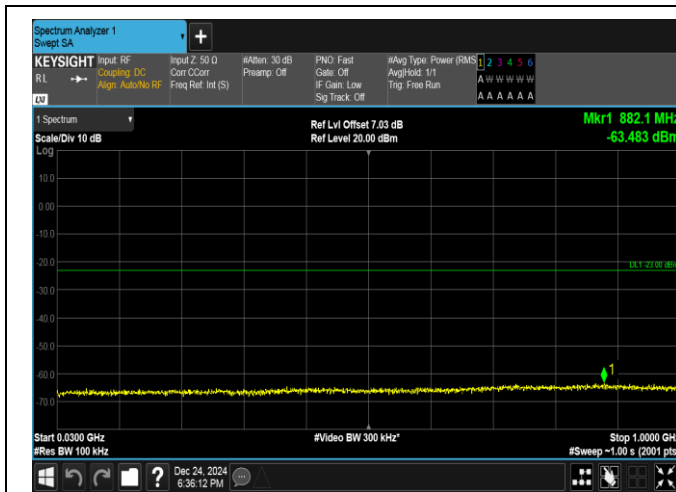
Band25-3MHz-QPSK-26055-15RB#0-30~1000-PASS
