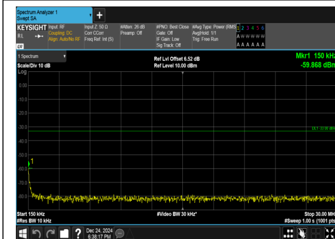
Band25-3MHz-QPSK-26365-1RB#0-0.15~30-PASS
