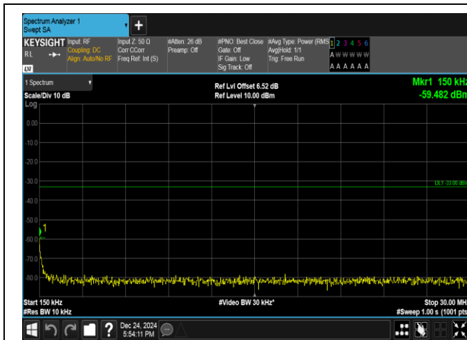
Band25-1.4MHz-QPSK-26683-1RB#5-0.15~30-PASS
