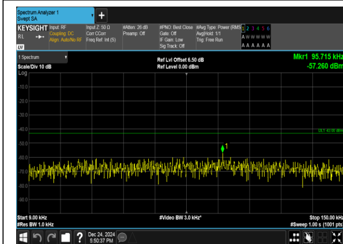
Band25-1.4MHz-16QAM-26365-6RB#0-0.009~0.15-PASS
