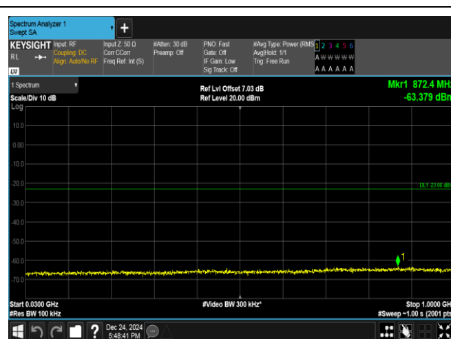
Band25-1.4MHz-16QAM-26365-1RB#5-30~1000-PASS
