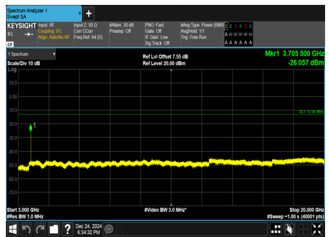
Band25-3MHz-QPSK-26055-1RB#14-3000~20000-PASS
