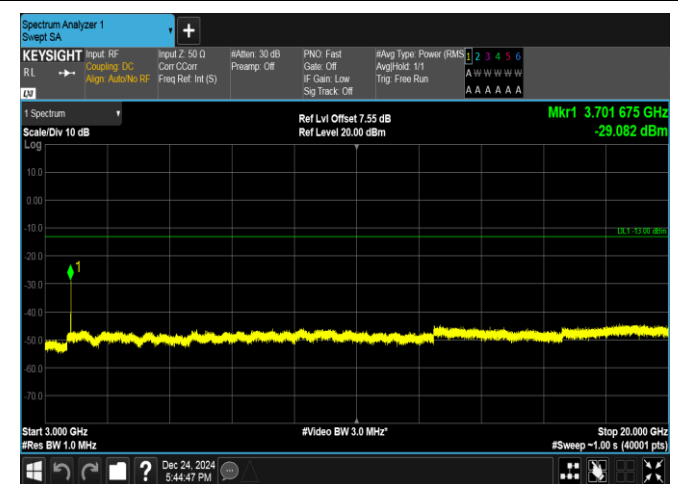
Band25-1.4MHz-16QAM-26047-6RB#0-3000~20000-PASS
