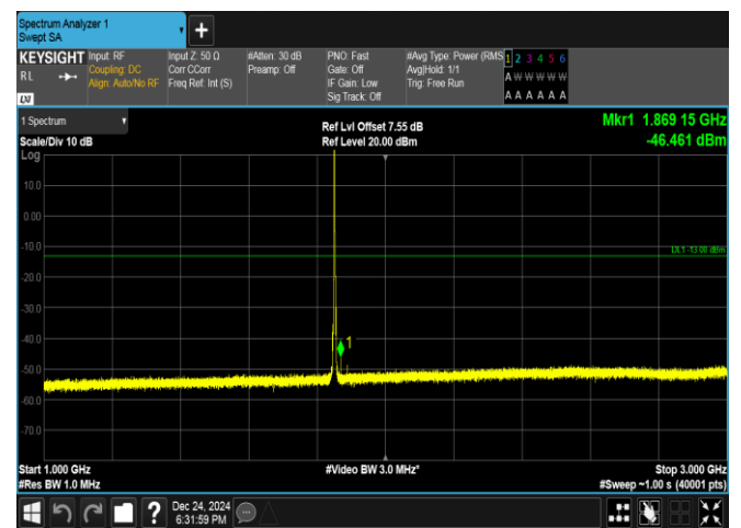
Band25-3MHz-QPSK-26055-1RB#0-1000~3000-PASS
