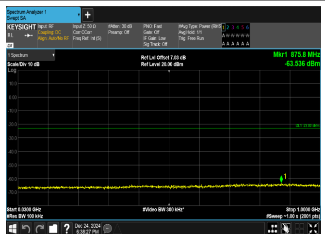
Band25-3MHz-QPSK-26365-1RB#0-30~1000-PASS
