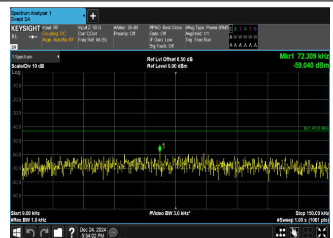
Band25-1.4MHz-QPSK-26683-1RB#5-0.009~0.15-PASS
