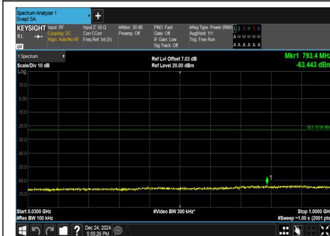
Band25-1.4MHz-16QAM-26683-1RB#5-30~1000-PASS
