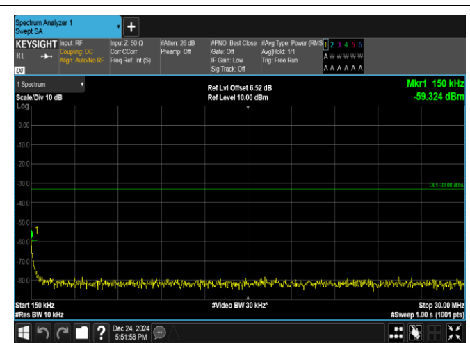
Band25-1.4MHz-QPSK-26683-1RB#0-0.15~30-PASS
