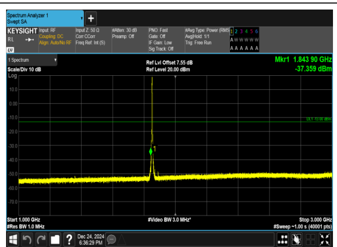
Band25-3MHz-QPSK-26055-15RB#0-1000~3000-PASS
