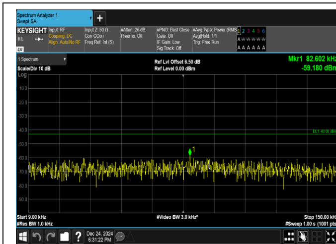
Band25-3MHz-QPSK-26055-1RB#0-0.009~0.15-PASS
