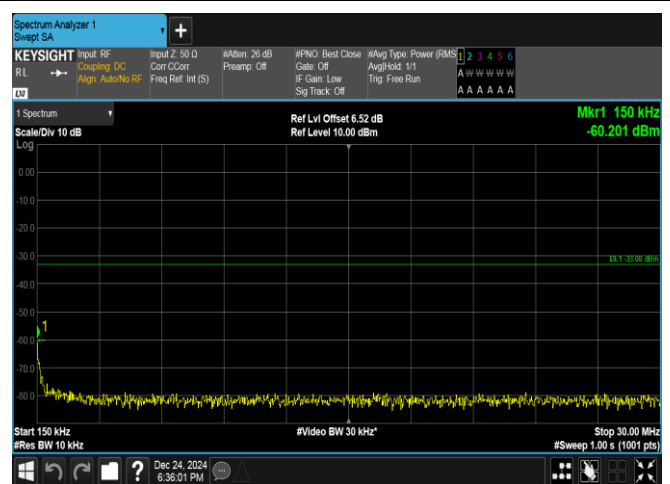
Band25-3MHz-QPSK-26055-15RB#0-0.15~30-PASS
