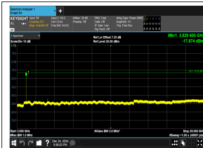
Band25-1.4MHz-16QAM-26683-1RB#5-3000~20000-PASS
