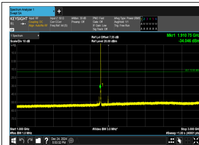
Band25-1.4MHz-16QAM-26683-1RB#0-1000~3000-PASS
