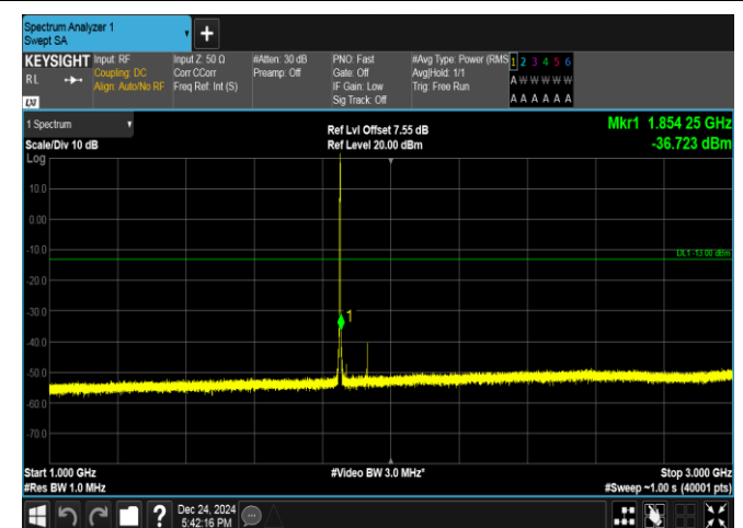
Band25-1.4MHz-16QAM-26047-1RB#5-1000~3000-PASS
