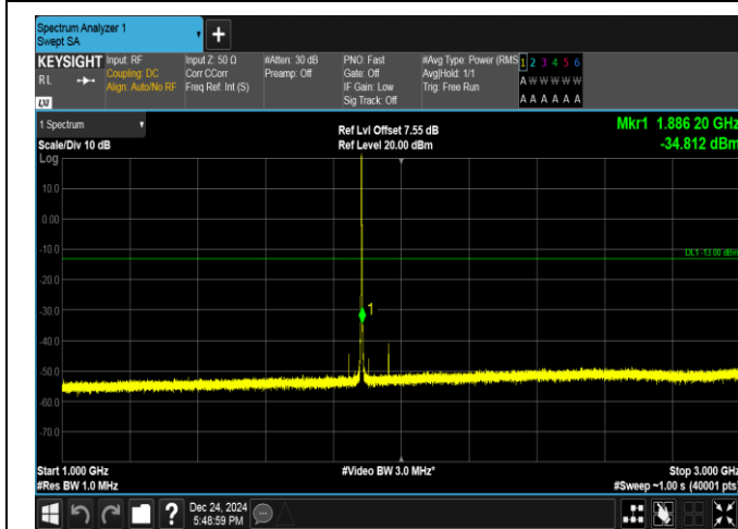
Band25-1.4MHz-16QAM-26365-1RB#5-1000~3000-PASS
