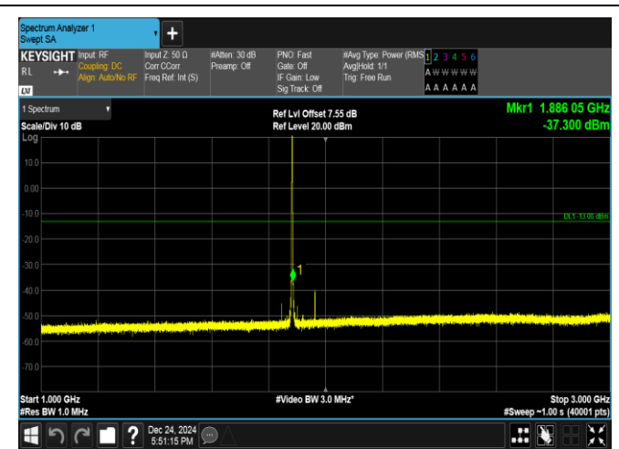
Band25-1.4MHz-16QAM-26365-6RB#0-1000~3000-PASS
