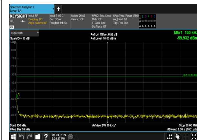
Band25-1.4MHz-16QAM-26047-1RB#0-0.15~30-PASS
