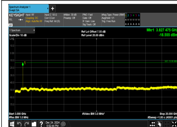
Band25-1.4MHz-QPSK-26683-1RB#0-3000~20000-PASS
