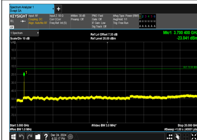
Band25-3MHz-QPSK-26055-1RB#0-3000~20000-PASS
