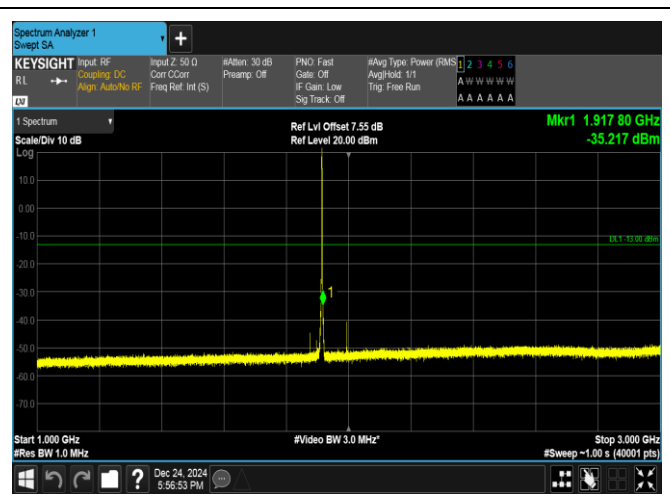
Band25-1.4MHz-QPSK-26683-6RB#0-1000~3000-PASS
