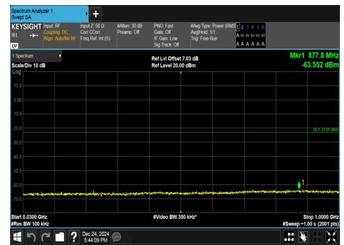
Band25-1.4MHz-16QAM-26047-6RB#0-30~1000-PASS
