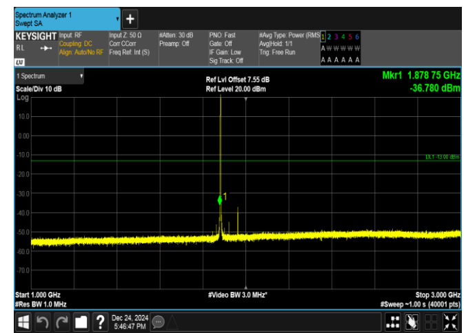
Band25-1.4MHz-16QAM-26365-1RB#0-1000~3000-PASS
