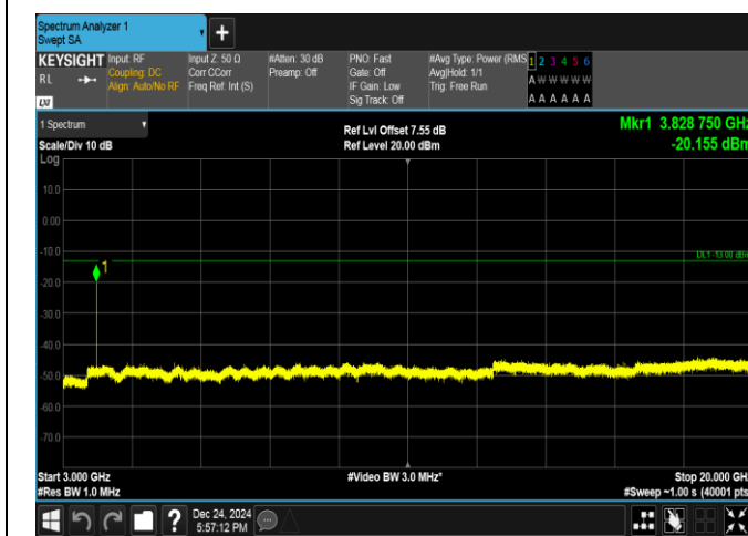
Band25-1.4MHz-QPSK-26683-6RB#0-3000~20000-PASS
