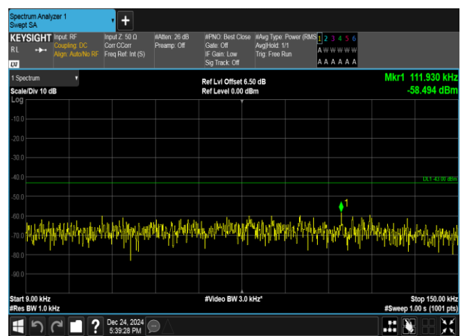
Band25-1.4MHz-16QAM-26047-1RB#0-0.009~0.15-PASS
