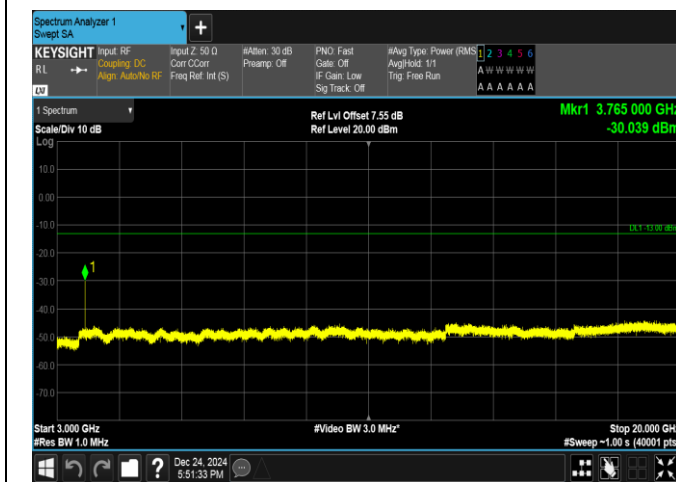
Band25-1.4MHz-16QAM-26365-6RB#0-3000~20000-PASS
