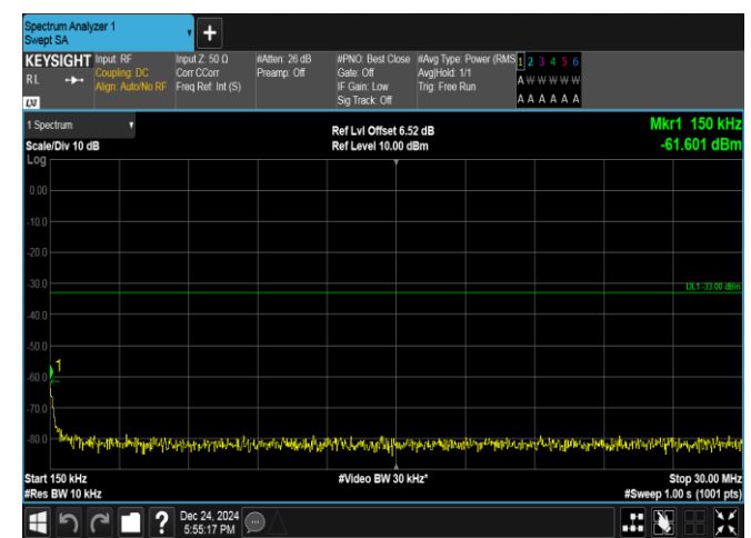
Band25-1.4MHz-16QAM-26683-1RB#5-0.15~30-PASS
