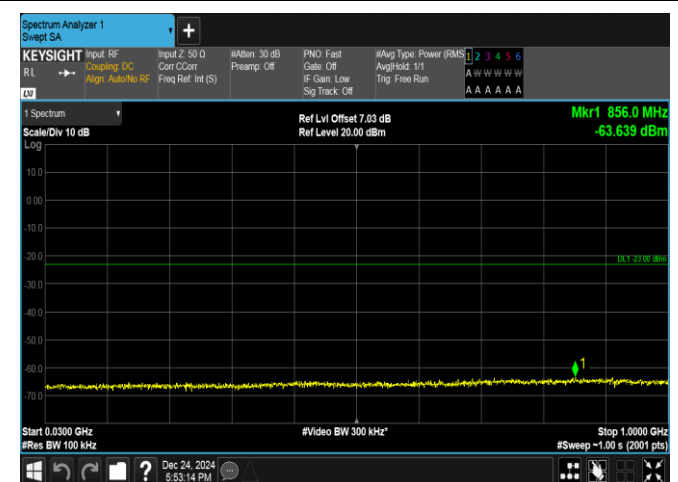
Band25-1.4MHz-16QAM-26683-1RB#0-30~1000-PASS
