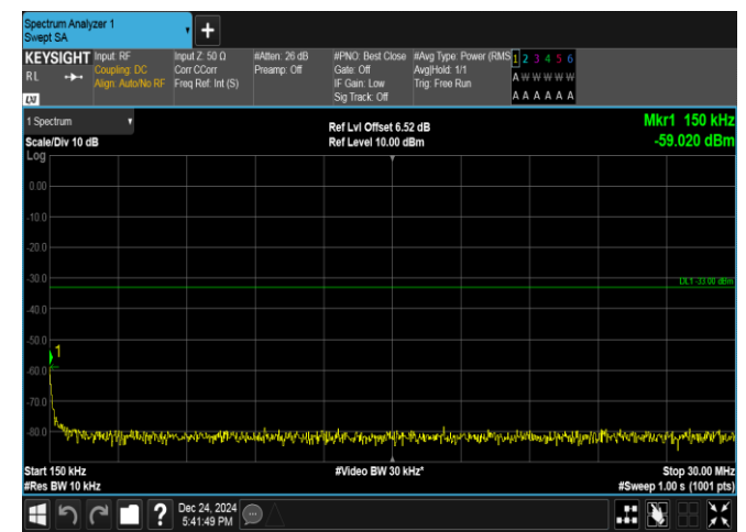
Band25-1.4MHz-16QAM-26047-1RB#5-0.15~30-PASS
