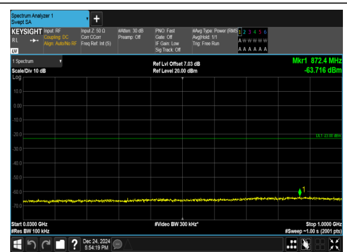
Band25-1.4MHz-QPSK-26683-1RB#5-30~1000-PASS
