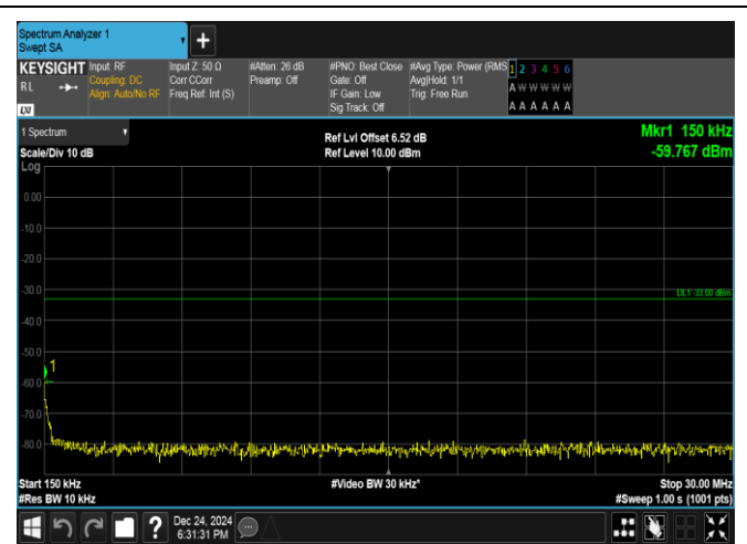
Band25-3MHz-QPSK-26055-1RB#0-0.15~30-PASS
