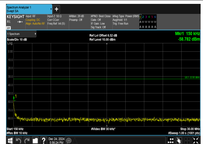
Band25-1.4MHz-QPSK-26683-6RB#0-0.15~30-PASS
