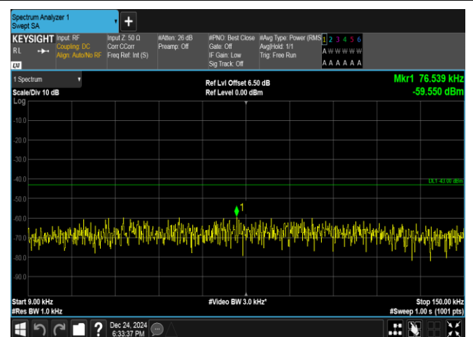
Band25-3MHz-QPSK-26055-1RB#14-0.009~0.15-PASS
