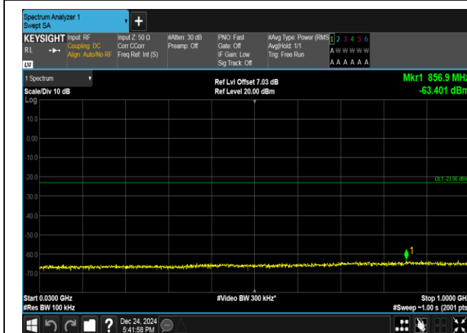
Band25-1.4MHz-16QAM-26047-1RB#5-30~1000-PASS
