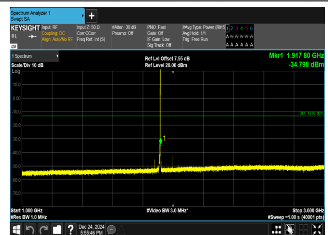
Band25-1.4MHz-16QAM-26683-1RB#5-1000~3000-PASS
