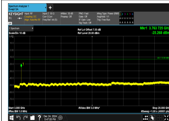
Band25-1.4MHz-16QAM-26365-1RB#0-3000~20000-PASS
