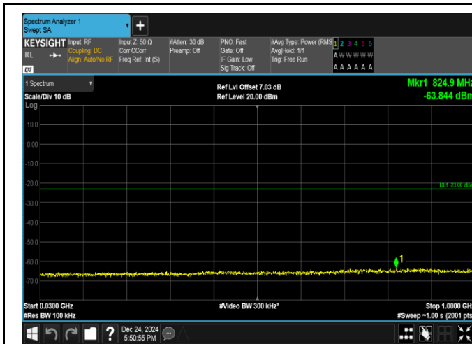
Band25-1.4MHz-16QAM-26365-6RB#0-30~1000-PASS
