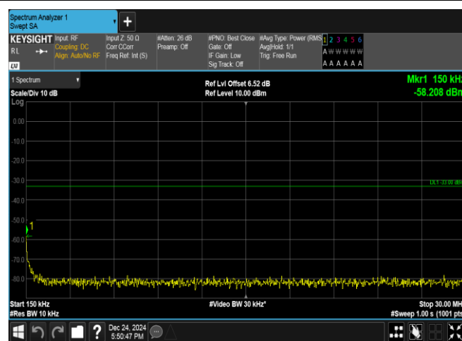
Band25-1.4MHz-16QAM-26365-6RB#0-0.15~30-PASS
