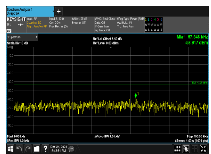
Band25-1.4MHz-16QAM-26047-6RB#0-0.009~0.15-PASS
