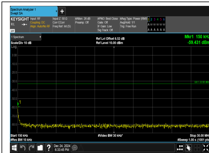
Band25-3MHz-QPSK-26055-1RB#14-0.15~30-PASS
