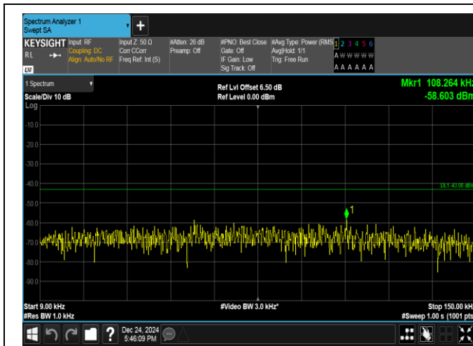
Band25-1.4MHz-16QAM-26365-1RB#0-0.009~0.15-PASS
