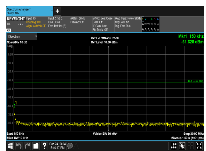
Band25-1.4MHz-16QAM-26365-1RB#0-0.15~30-PASS
