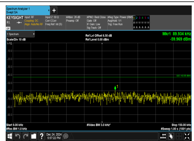
Band25-1.4MHz-16QAM-26683-6RB#0-0.009~0.15-PASS
