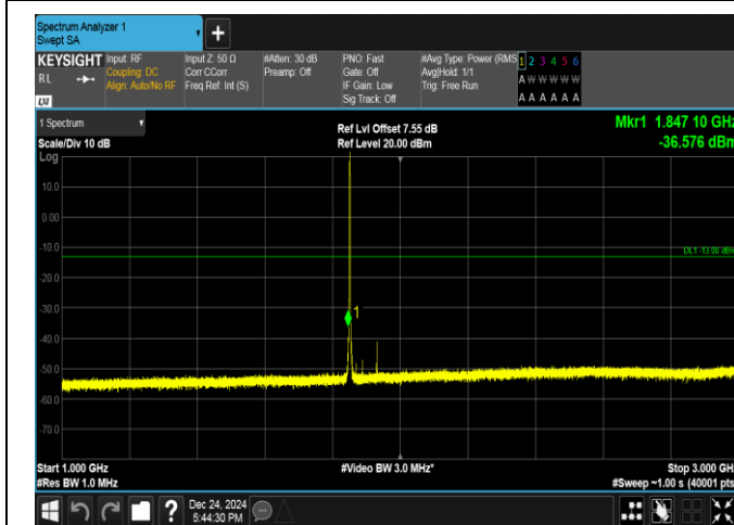
Band25-1.4MHz-16QAM-26047-6RB#0-1000~3000-PASS
