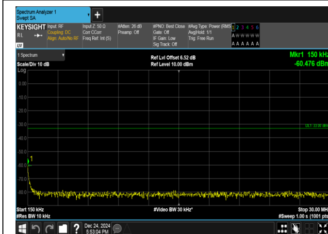
Band25-1.4MHz-16QAM-26683-1RB#0-0.15~30-PASS
