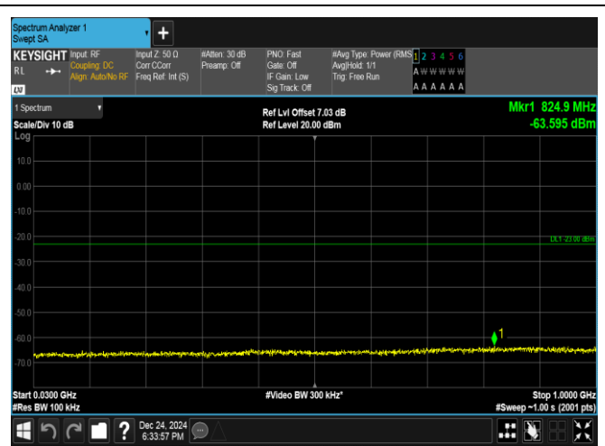
Band25-3MHz-QPSK-26055-1RB#14-30~1000-PASS
