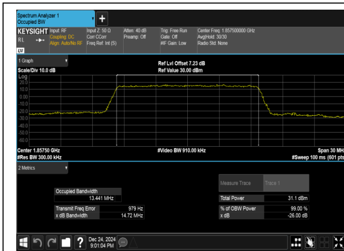
Band25-15MHz-QPSK-26115-75RB#0-PASS
