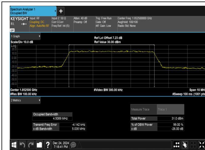
Band25-5MHz-QPSK-26065-25RB#0-PASS
