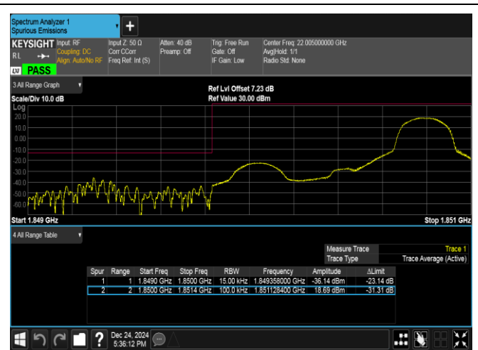
Band25-1.4MHz-16QAM-26047-1RB#5-PASS
