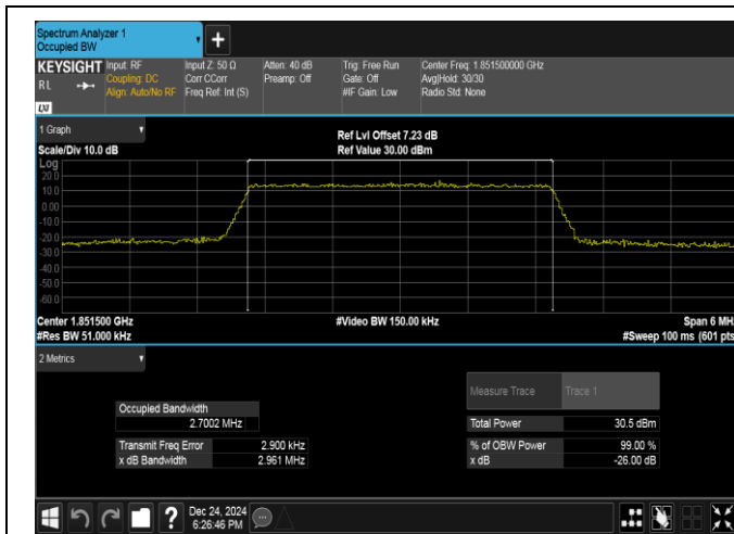
Band25-3MHz-QPSK-26055-15RB#0-PASS
