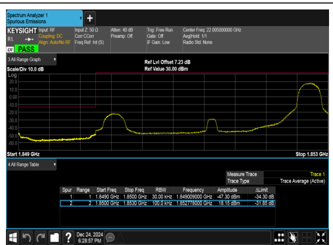
Band25-3MHz-16QAM-26055-1RB#14-PASS
