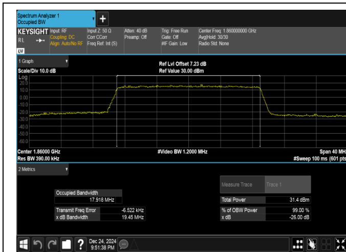
Band25-20MHz-QPSK-26140-100RB#0-PASS
