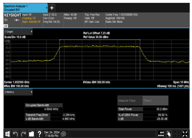
Band25-5MHz-16QAM-26065-25RB#0-PASS
