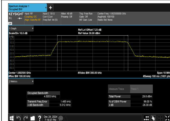
Band25-5MHz-16QAM-26365-25RB#0-PASS
