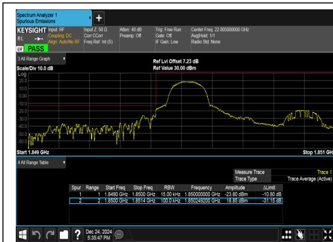
Band25-1.4MHz-16QAM-26047-1RB#0-PASS
