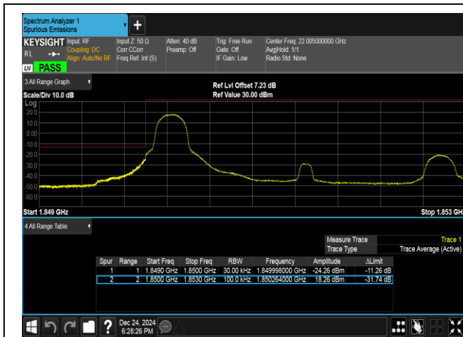
Band25-3MHz-16QAM-26055-1RB#0-PASS
