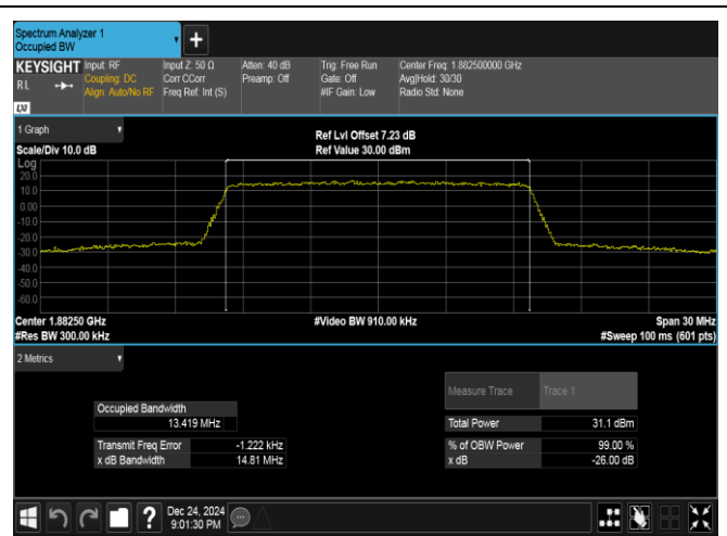
Band25-15MHz-QPSK-26365-75RB#0-PASS
