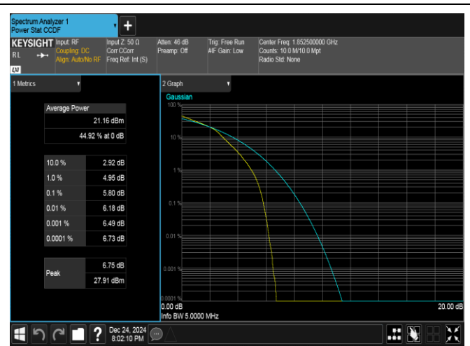
Band25-5MHz-16QAM-26065-25RB#0-PASS
