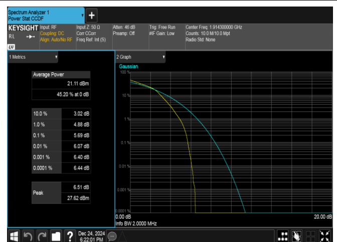
Band25-1.4MHz-16QAM-26683-6RB#0-PASS
