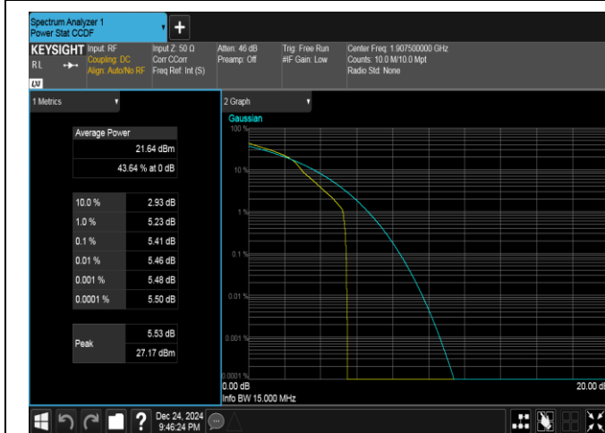
Band25-15MHz-16QAM-26615-1RB#0-PASS
