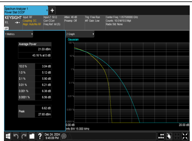
Band25-15MHz-16QAM-26115-75RB#0-PASS
