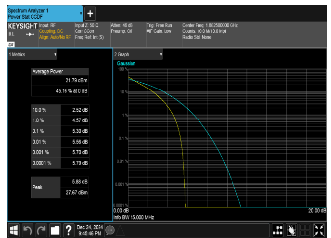
Band25-15MHz-QPSK-26365-75RB#0-PASS
