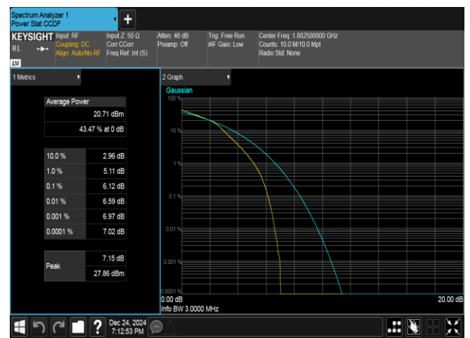
Band25-3MHz-16QAM-26365-15RB#0-PASS
