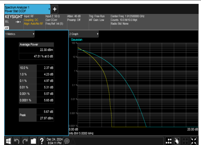
Band25-5MHz-QPSK-26665-25RB#0-PASS
