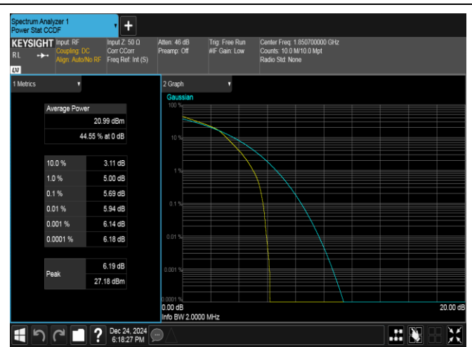
Band25-1.4MHz-16QAM-26047-6RB#0-PASS
