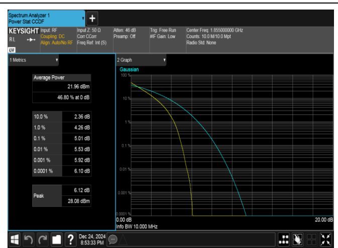
Band25-10MHz-QPSK-26090-50RB#0-PASS
