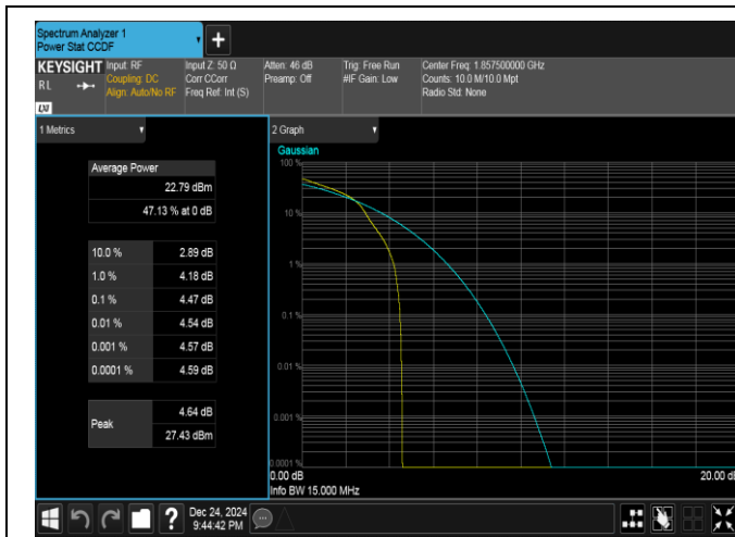
Band25-15MHz-16QAM-26115-1RB#0-PASS
