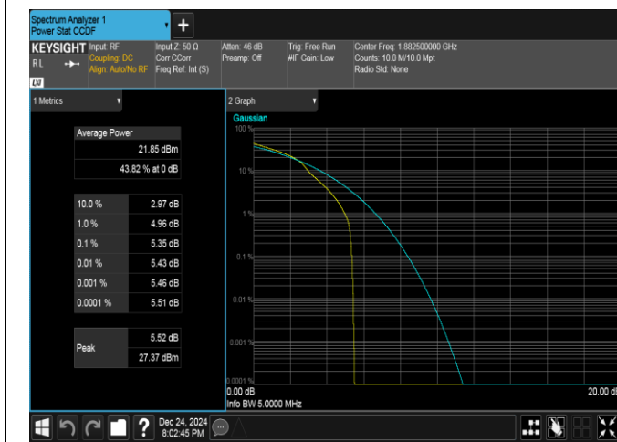
Band25-5MHz-16QAM-26365-1RB#0-PASS
