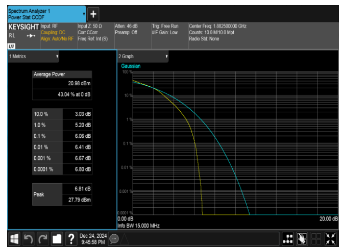
Band25-15MHz-16QAM-26365-75RB#0-PASS
