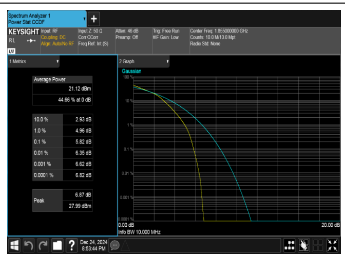
Band25-10MHz-16QAM-26090-50RB#0-PASS
