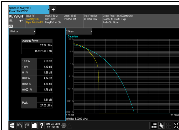
Band25-5MHz-16QAM-26065-1RB#0-PASS
