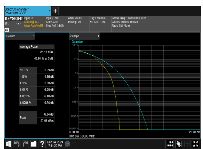
Band25-3MHz-16QAM-26055-15RB#0-PASS
