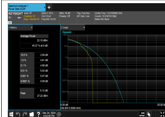
Band25-5MHz-16QAM-26665-1RB#0-PASS
