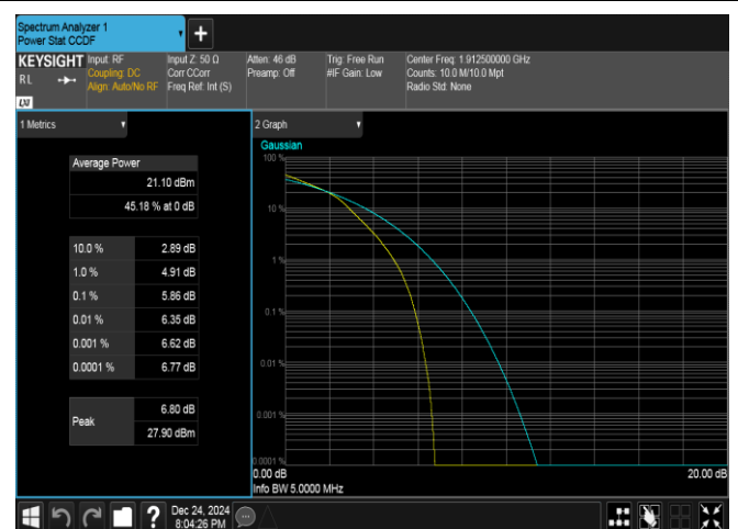
Band25-5MHz-16QAM-26665-25RB#0-PASS
