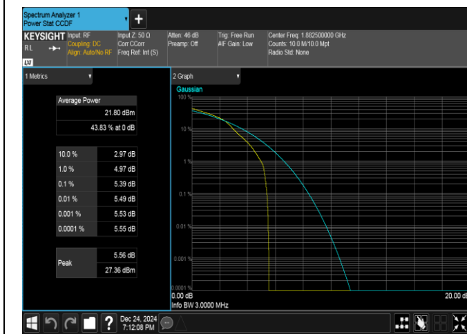
Band25-3MHz-16QAM-26365-1RB#0-PASS
