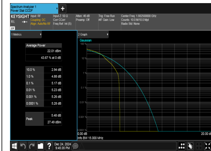
Band25-15MHz-16QAM-26365-1RB#0-PASS
