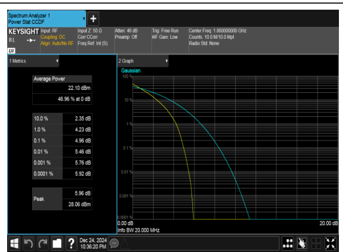
Band25-20MHz-QPSK-26140-100RB#0-PASS
