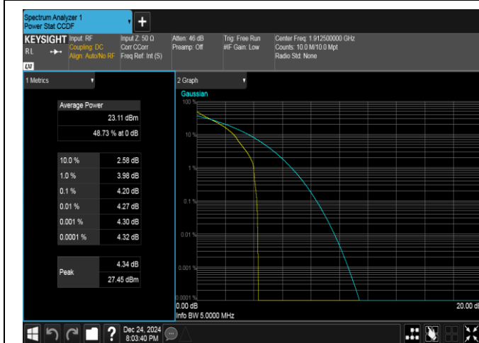
Band25-5MHz-QPSK-26665-1RB#0-PASS
