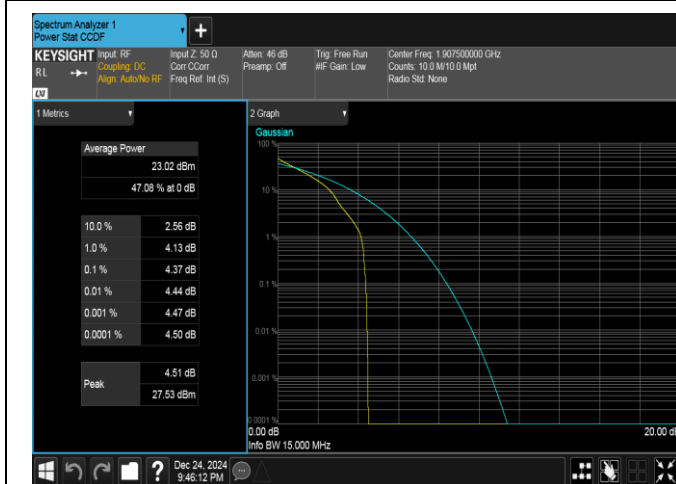
Band25-15MHz-QPSK-26615-1RB#0-PASS
