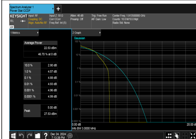
Band25-3MHz-16QAM-26675-1RB#0-PASS
