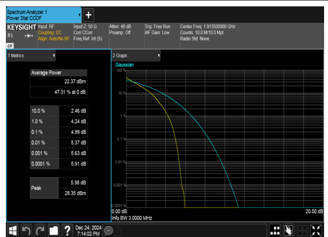
Band25-3MHz-QPSK-26675-15RB#0-PASS
