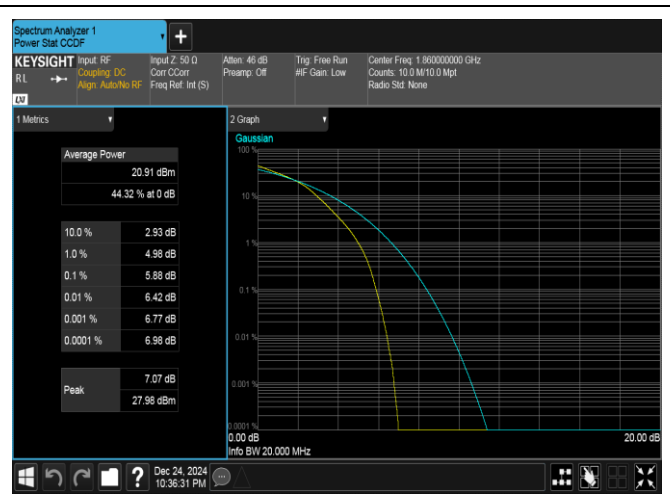
Band25-20MHz-16QAM-26140-100RB#0-PASS
