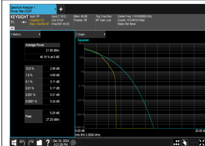
Band25-1.4MHz-16QAM-26683-1RB#0-PASS
