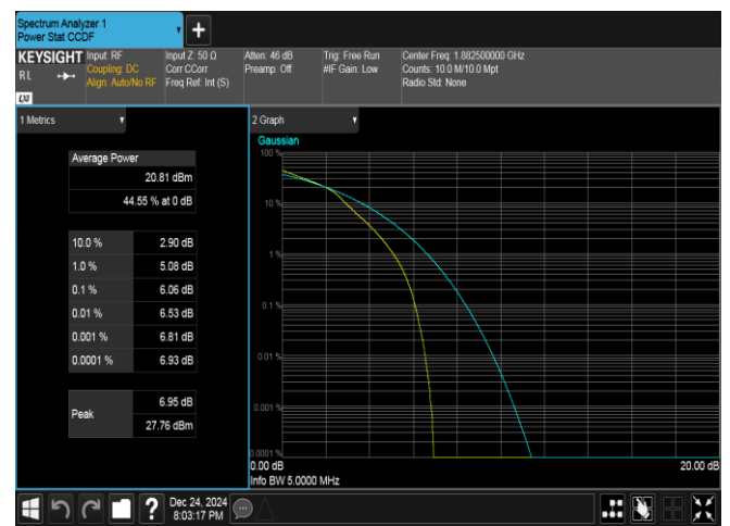
Band25-5MHz-16QAM-26365-25RB#0-PASS
