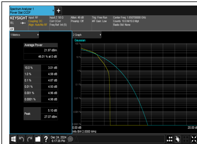
Band25-1.4MHz-16QAM-26047-1RB#0-PASS
