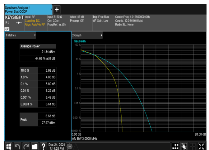
Band25-3MHz-16QAM-26675-15RB#0-PASS
