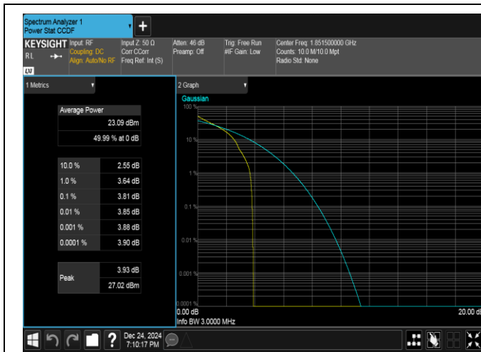
Band25-3MHz-QPSK-26055-1RB#0-PASS
