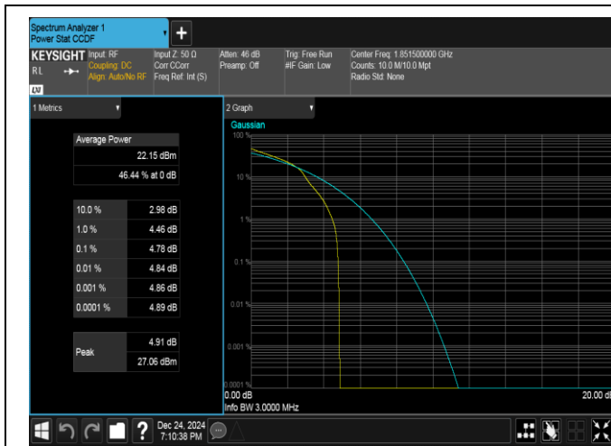
Band25-3MHz-16QAM-26055-1RB#0-PASS
