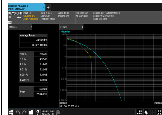
Band25-20MHz-16QAM-26590-1RB#0-PASS
