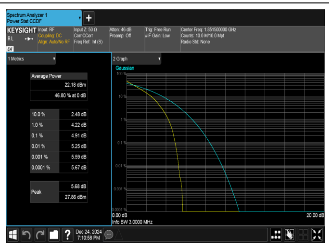
Band25-3MHz-QPSK-26055-15RB#0-PASS
