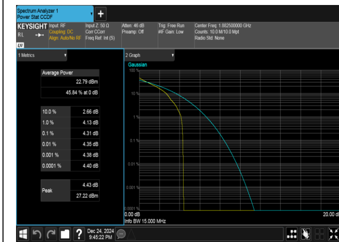
Band25-15MHz-QPSK-26365-1RB#0-PASS
