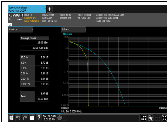
Band25-5MHz-QPSK-26065-1RB#0-PASS
