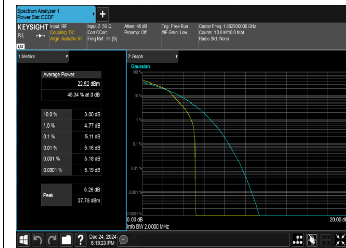
Band25-1.4MHz-16QAM-26365-1RB#0-PASS
