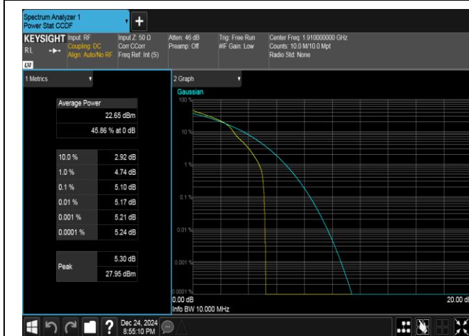
Band25-10MHz-16QAM-26640-1RB#0-PASS
