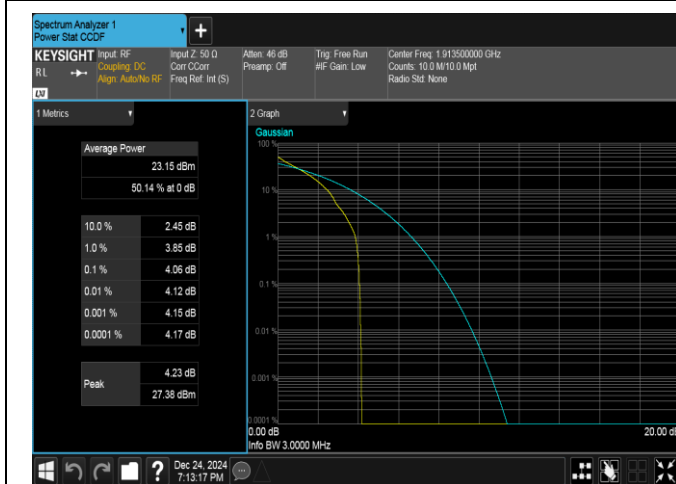
Band25-3MHz-QPSK-26675-1RB#0-PASS
