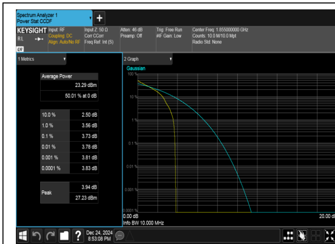
Band25-10MHz-QPSK-26090-1RB#0-PASS
