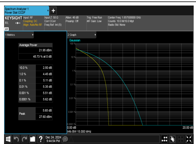
Band25-15MHz-QPSK-26115-75RB#0-PASS
