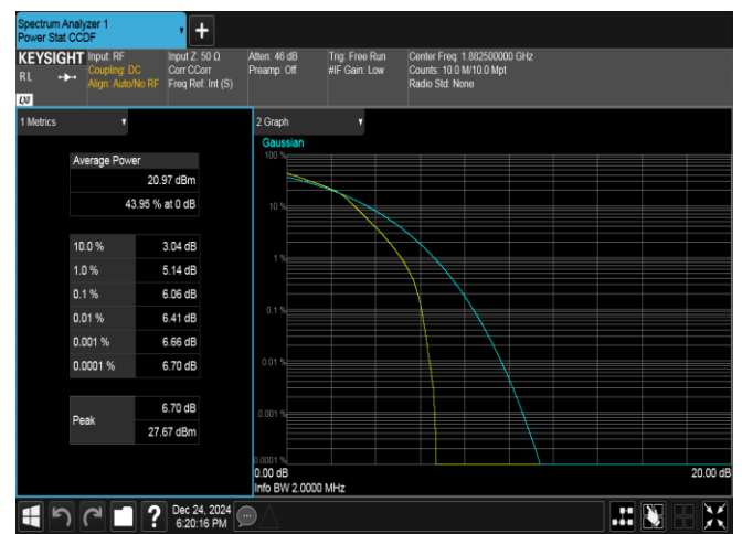
Band25-1.4MHz-16QAM-26365-6RB#0-PASS
