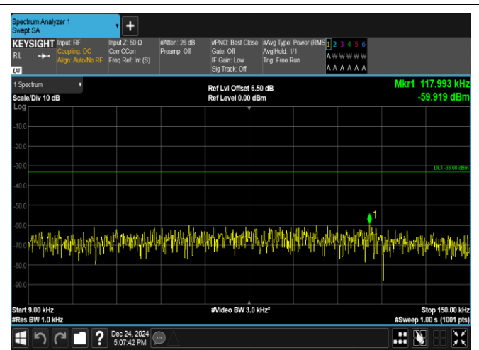
Band17-10MHz-16QAM-23800-50RB#0-0.009~0.15-PASS
