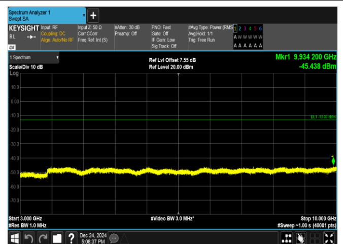
Band17-10MHz-16QAM-23800-50RB#0-3000~10000-PASS
