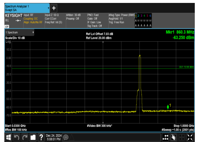
Band17-10MHz-16QAM-23800-50RB#0-30~1000-PASS
