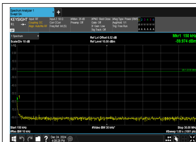
Band17-5MHz-16OAM-23790-1RB#24-0.15~30-PASS
