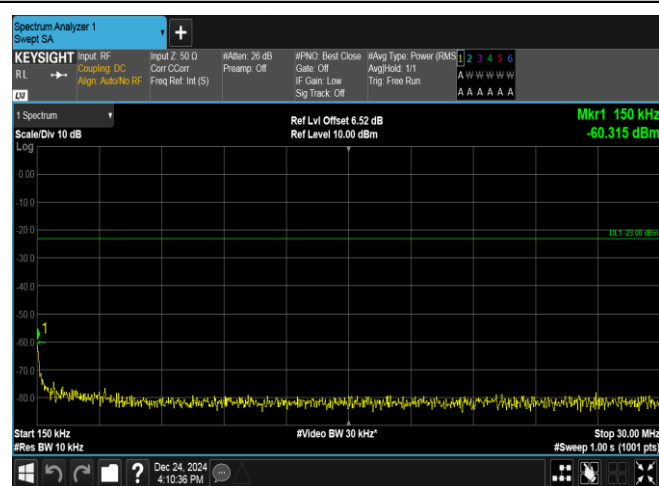
Band17-5MHz-16OAM-23790-25RB#0-0.15~30-PASS
