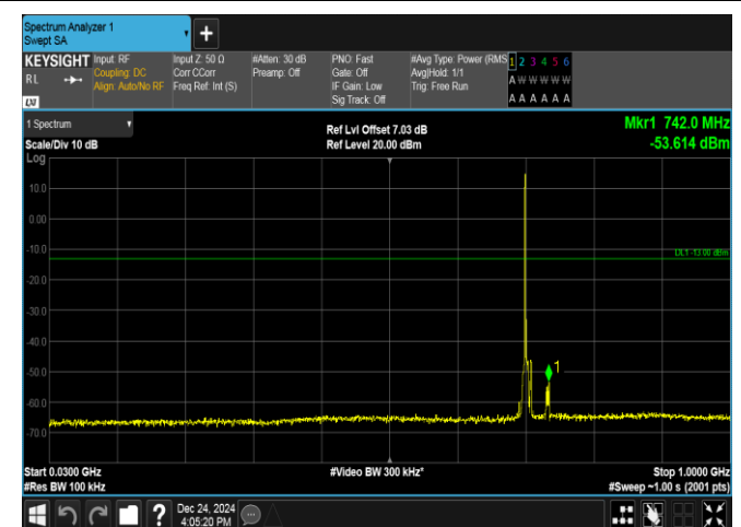
Band17-5MHz-QPSK-23790-1RB#0-30~1000-PASS
