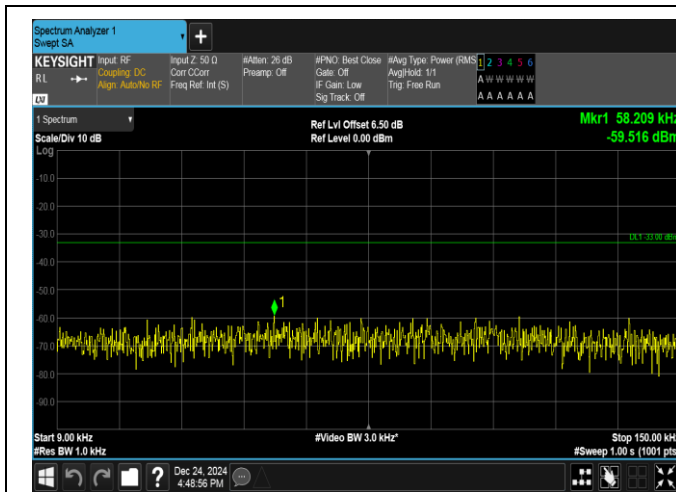
Band17-10MHz-QPSK-23780-1RB#0-0.009~0.15-PASS
