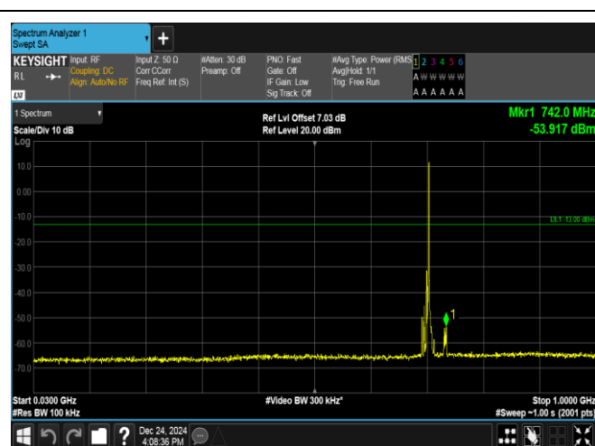
Band17-5MHz-16OAM-23790-1RB#24-30~1000-PASS
