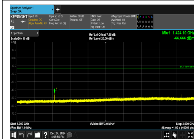
Band17-5MHz-16OAM-23790-1RB#24-1000~3000-PASS
