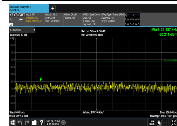
Band17-5MHz-16OAM-23790-25RB#0-0.009~0.15-PASS
