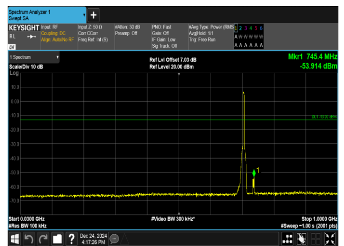
Band17-5MHz-16QAM-23825-25RB#0-30~1000-PASS
