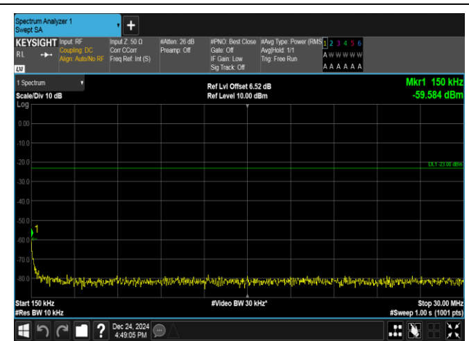
Band17-10MHz-QPSK-23780-1RB#0-0.15~30-PASS
