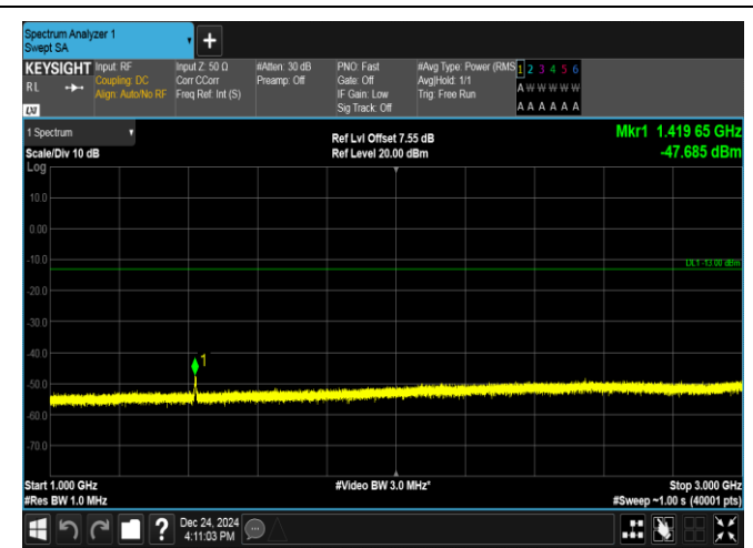
Band17-5MHz-16QAM-23790-25RB#0-1000~3000-PASS
