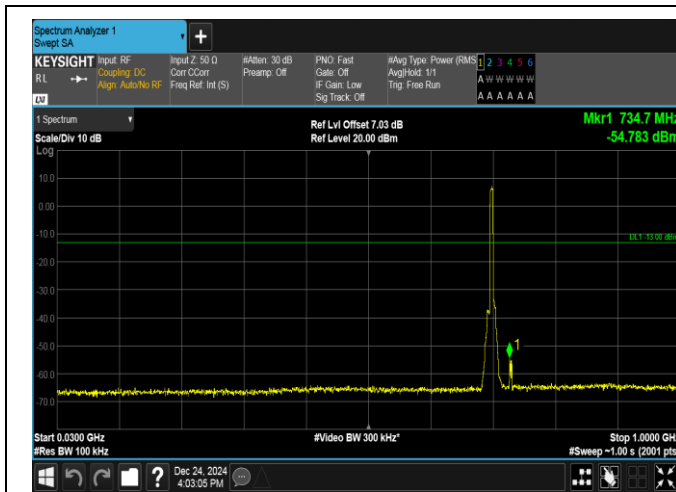
Band17-5MHz-QPSK-23755-25RB#0-30~1000-PASS
