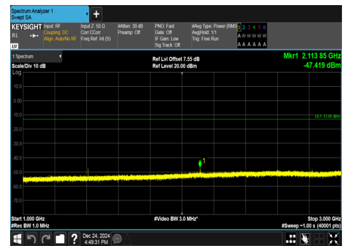
Band17-10MHz-QPSK-23780-1RB#0-1000~3000-PASS
