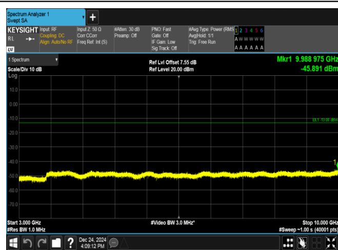
Band17-5MHz-16OAM-23790-1RB#24-3000~10000-PASS
