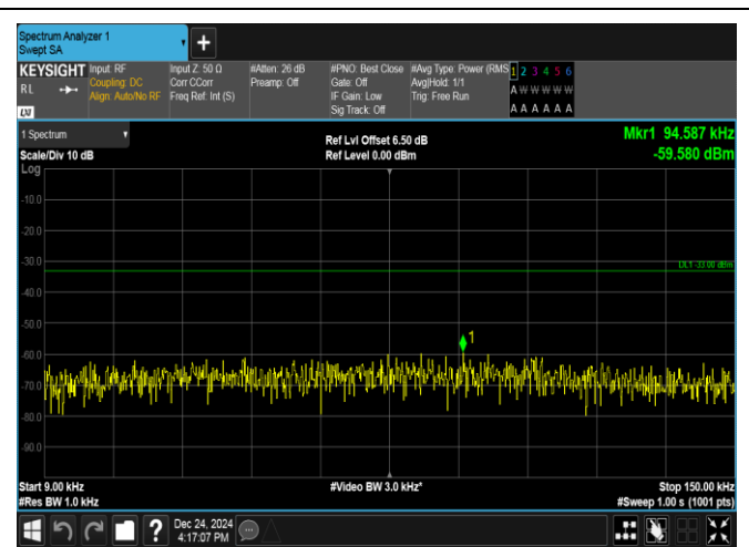
Band17-5MHz-16QAM-23825-25RB#0-0.009~0.15-PASS
