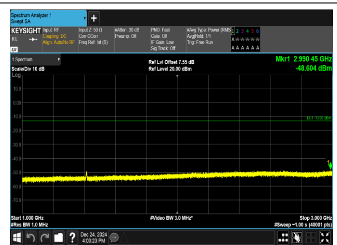
Band17-5MHz-QPSK-23755-25RB#0-1000~3000-PASS
