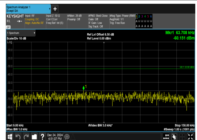
Band17-10MHz-QPSK-23780-1RB#49-0.009~0.15-PASS
