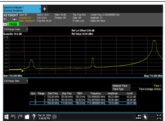
Band17-10MHz-QPSK-23780-1RB#49-PASS
