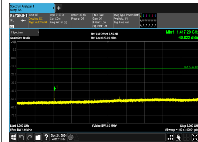
Band17-5MHz-QPSK-23755-1RB#24-1000~3000-PASS
