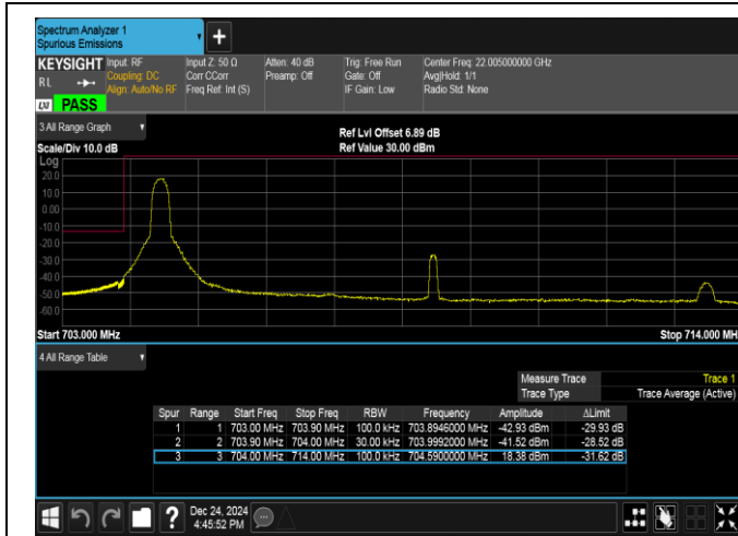
Band17-10MHz-16QAM-23780-1RB#0-PASS
