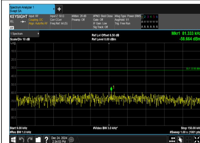
Band13-10MHz-16QAM-23230-1RB#49-0.009~0.15-PASS
