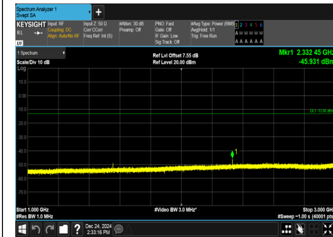
Band13-10MHz-16QAM-23230-1RB#0-1000~3000-PASS
