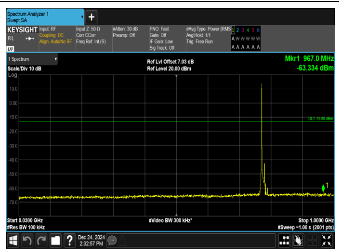
Band13-10MHz-16QAM-23230-1RB#0-30~1000-PASS
