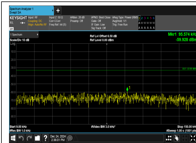
Band13-10MHz-QPSK-23230-50RB#0-0.009~0.15-PASS
