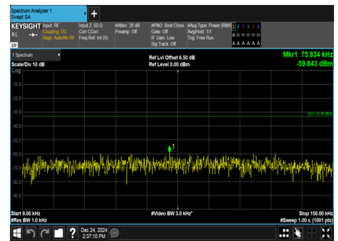
Band13-10MHz-16QAM-23230-50RB#0-0.009~0.15-PASS
