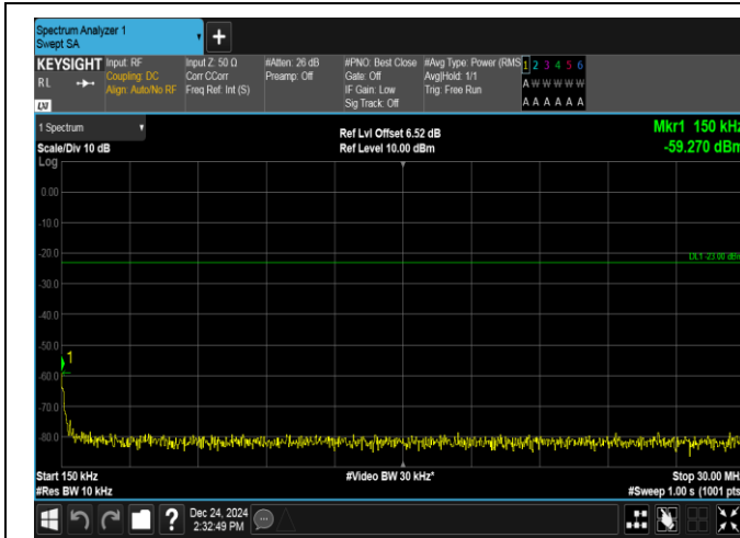
Band13-10MHz-16QAM-23230-1RB#0-0.15~30-PASS
