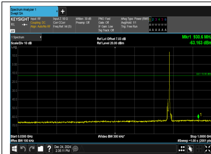
Band13-10MHz-16QAM-23230-1RB#49-30~1000-PASS
