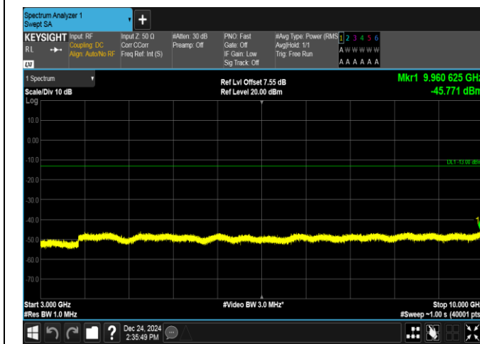
Band13-10MHz-16QAM-23230-1RB#49-3000~10000-PASS
