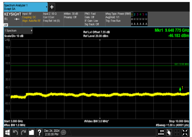
Band13-10MHz-16QAM-23230-1RB#0-3000~10000-PASS
