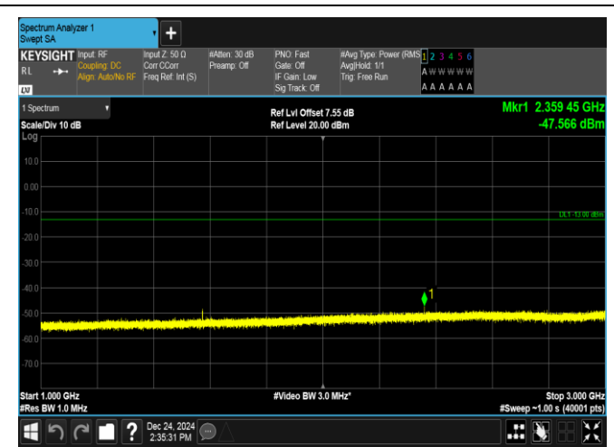
Band13-10MHz-16QAM-23230-1RB#49-1000~3000-PASS
