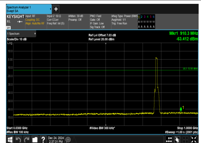
Band13-10MHz-16QAM-23230-50RB#0-30~1000-PASS
