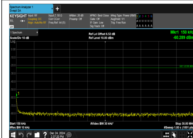
Band13-10MHz-16QAM-23230-50RB#0-0.15~30-PASS
