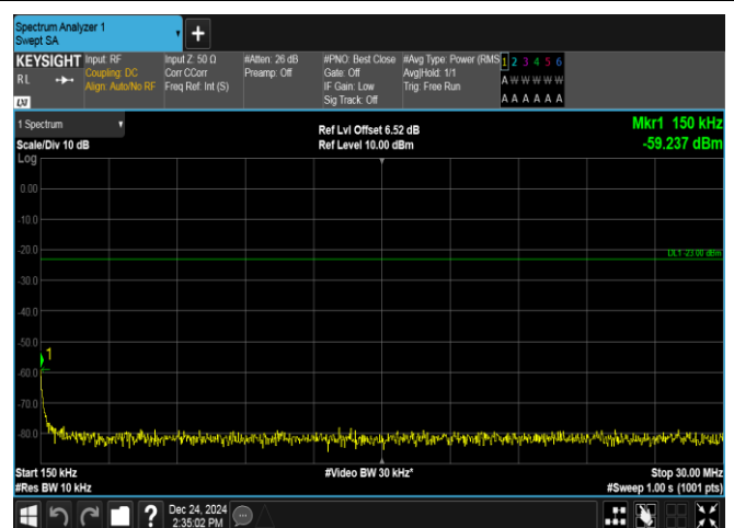
Band13-10MHz-16QAM-23230-1RB#49-0.15~30-PASS
