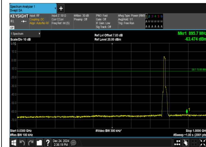
Band13-10MHz-QPSK-23230-50RB#0-30~1000-PASS
