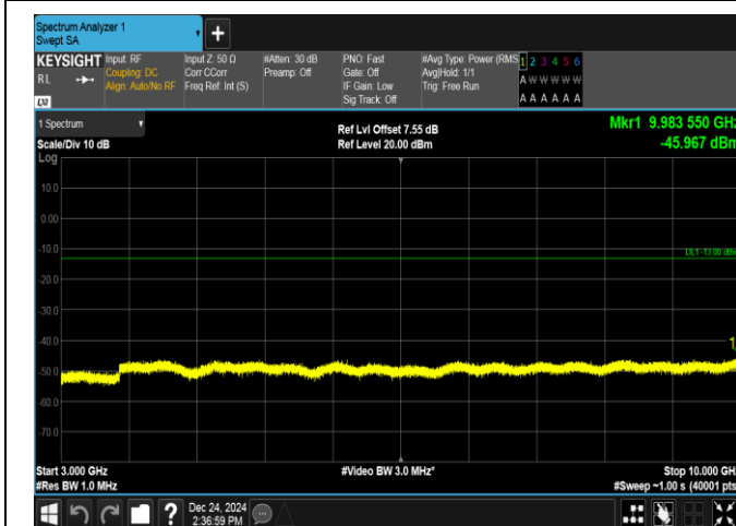
Band13-10MHz-QPSK-23230-50RB#0-3000~10000-PASS
