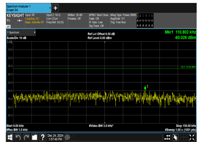
Band13-5MHz-QPSK-23230-25RB#0-0.009~0.15-PASS
