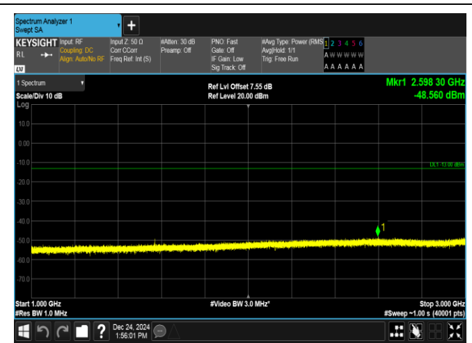
Band13-5MHz-QPSK-23230-1RB#24-1000~3000-PASS
