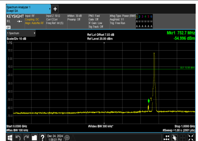
Band13-5MHz-QPSK-23230-25RB#0-30~1000-PASS
