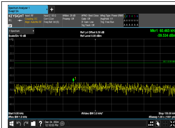
Band12-5MHz-QPSK-23095-1RB#24-0.009~0.15-PASS
