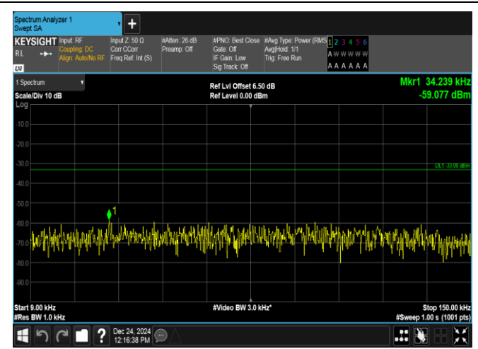
Band12-5MHz-16QAM-23155-1RB#0-0.009~0.15-PASS
