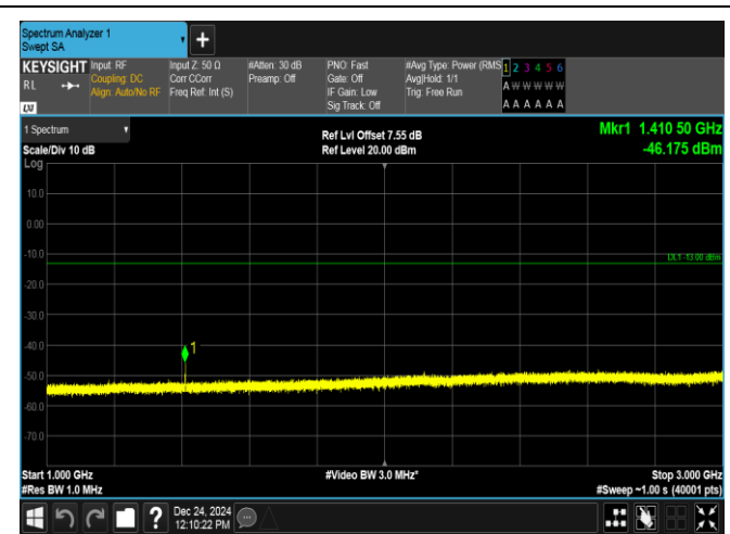
Band12-5MHz-16QAM-23095-1RB#0-1000~3000-PASS
