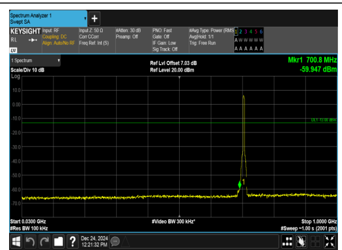
Band12-5MHz-16QAM-23155-25RB#0-30~1000-PASS
