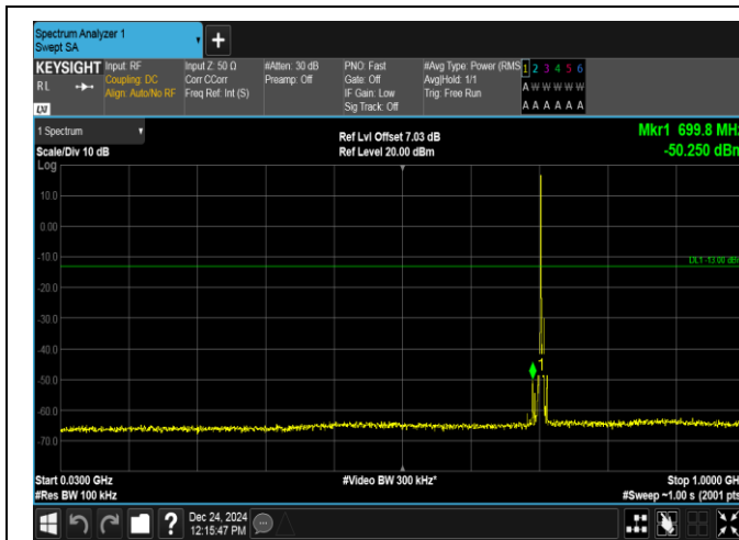
Band12-5MHz-QPSK-23155-1RB#0-30~1000-PASS
