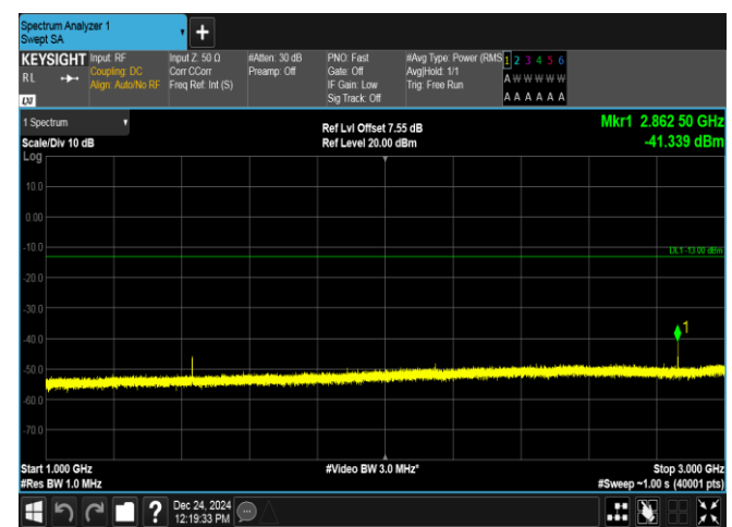
Band12-5MHz-16QAM-23155-1RB#24-1000~3000-PASS
