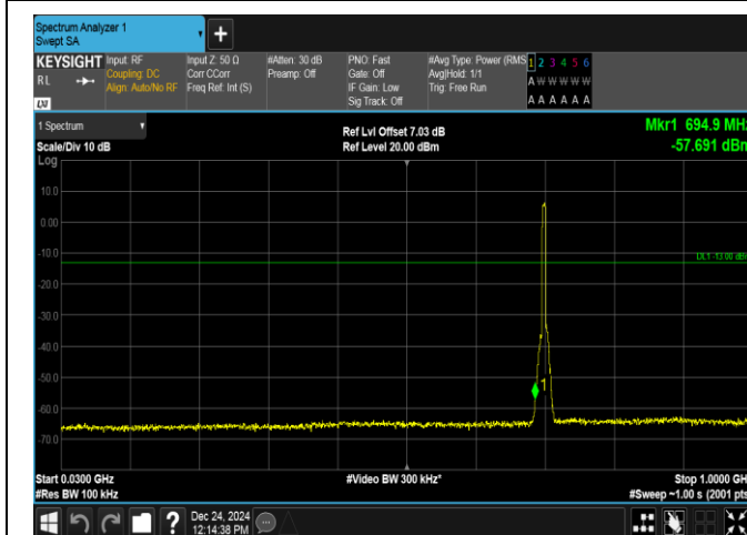
Band12-5MHz-16QAM-23095-25RB#0-30~1000-PASS
