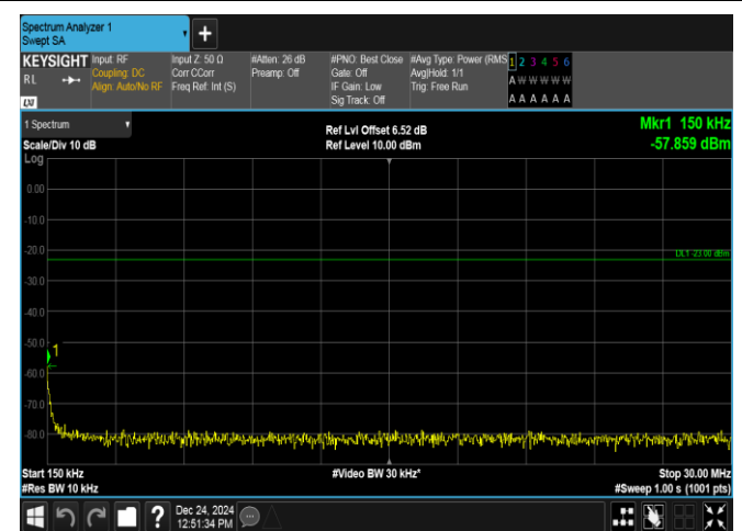
Band12-10MHz-QPSK-23060-1RB#0-0.15~30-PASS
