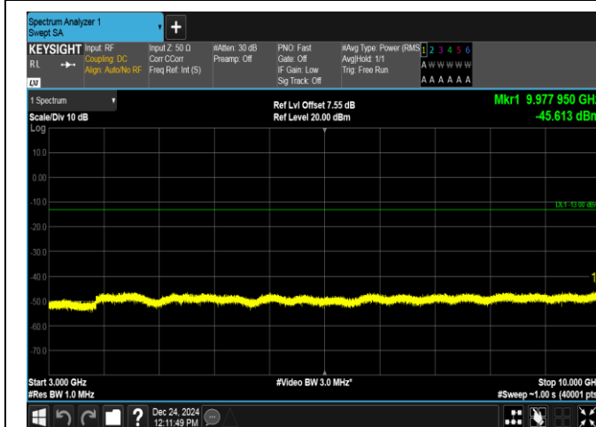
Band12-5MHz-QPSK-23095-1RB#24-3000~10000-PASS
