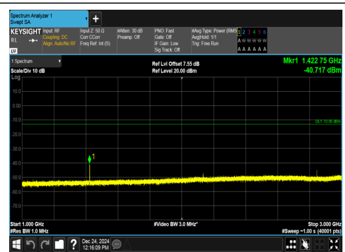
Band12-5MHz-QPSK-23155-1RB#0-1000~3000-PASS
