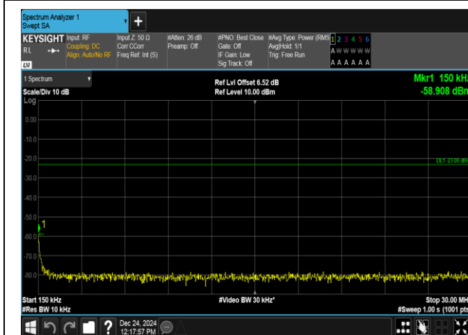
Band12-5MHz-QPSK-23155-1RB#24-0.15~30-PASS
