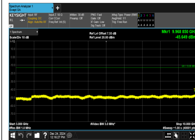
Band12-5MHz-QPSK-23155-1RB#0-3000~10000-PASS
