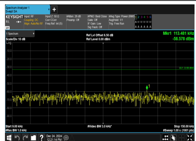
Band12-5MHz-16QAM-23155-25RB#0-0.009~0.15-PASS
