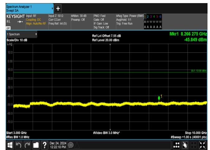
Band12-5MHz-16QAM-23155-25RB#0-3000~10000-PASS
