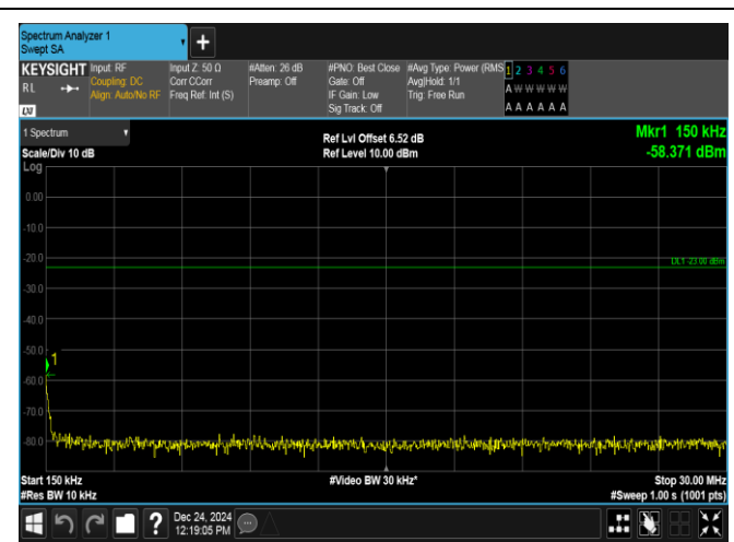
Band12-5MHz-16QAM-23155-1RB#24-0.15~30-PASS
