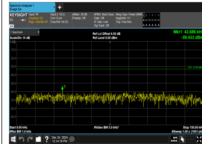
Band12-5MHz-16QAM-23095-25RB#0-0.009~0.15-PASS
