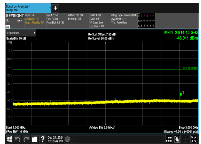
Band12-5MHz-16QAM-23035-1RB#24-1000~3000-PASS
