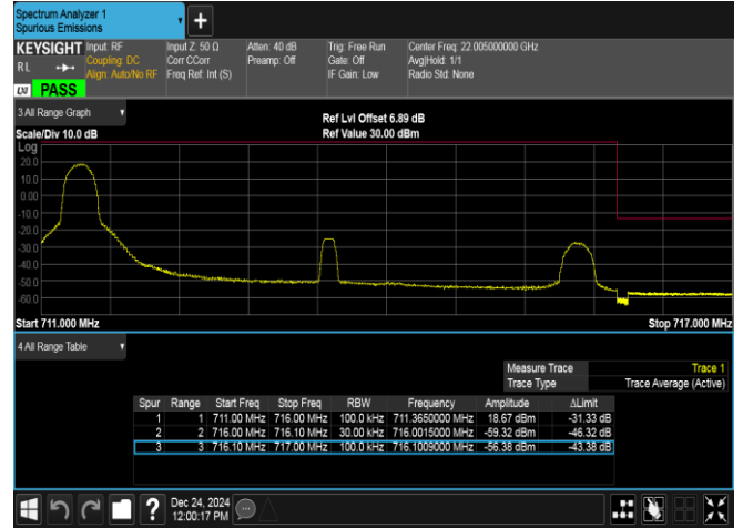
Band12-5MHz-16QAM-23155-1RB#0-PASS
