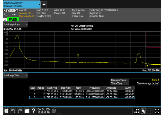
Band12-10MHz-QPSK-23130-1RB#0-PASS
