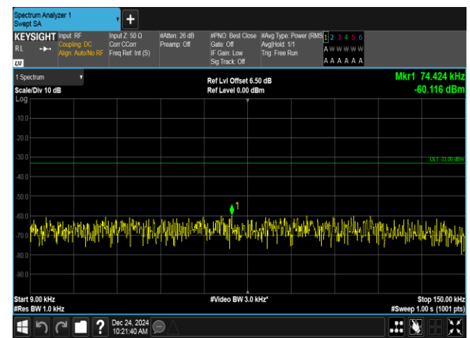
Band12-1.4MHz-QPSK-23017-1RB#5-0.009~0.15-PASS
