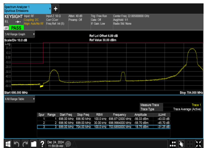
Band12-5MHz-16QAM-23035-1RB#24-PASS
