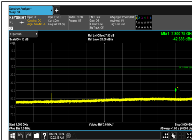
Band12-1.4MHz-QPSK-23017-1RB#5-1000~3000-PASS
