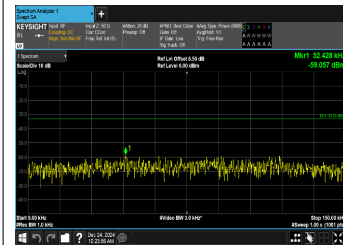
Band12-1.4MHz-QPSK-23017-6RB#0-0.009~0.15-PASS
