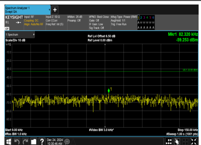
Band12-1.4MHz-QPSK-23095-6RB#0-0.009~0.15-PASS
