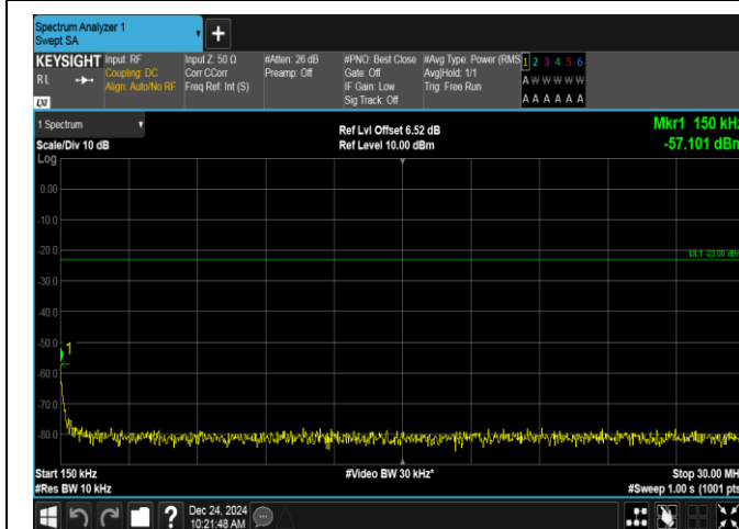
Band12-1.4MHz-QPSK-23017-1RB#5-0.15~30-PASS
