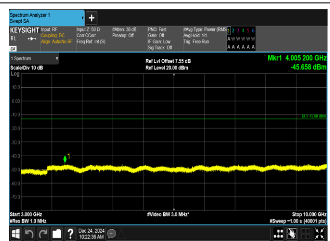
Band12-1.4MHz-QPSK-23017-1RB#5-3000~10000-PASS
