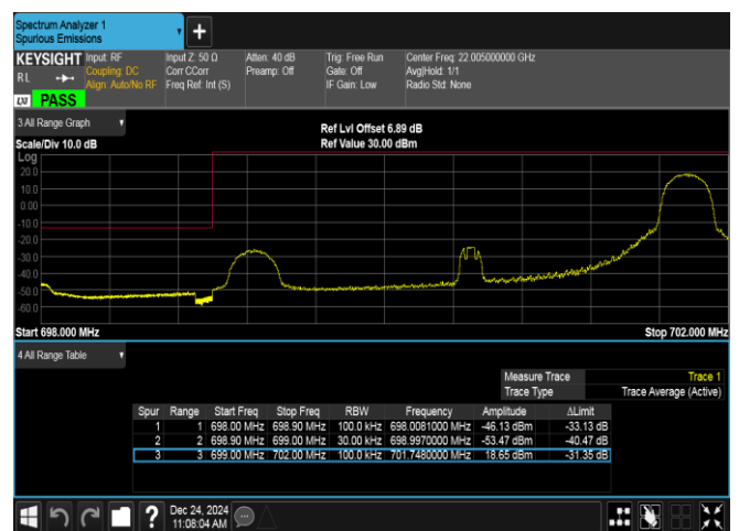
Band12-3MHz-16QAM-23025-1RB#14-PASS
