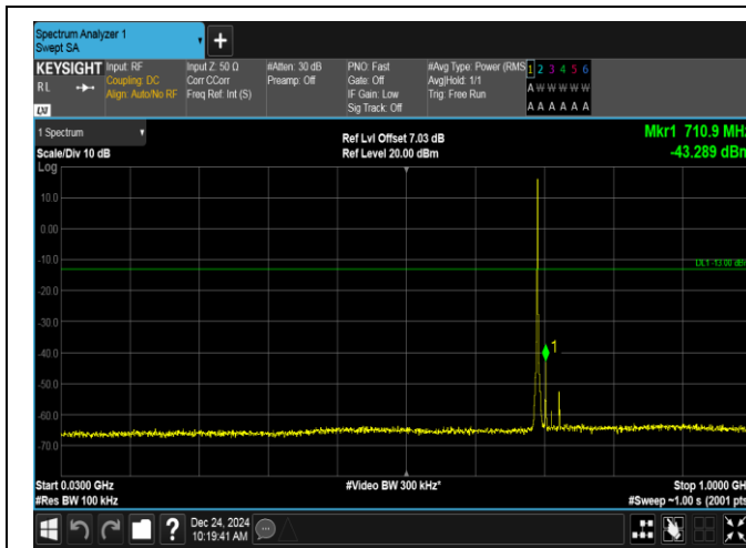
Band12-1.4MHz-QPSK-23017-1RB#0-30~1000-PASS
