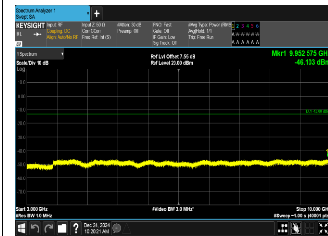
Band12-1.4MHz-QPSK-23017-1RB#0-3000~10000-PASS
