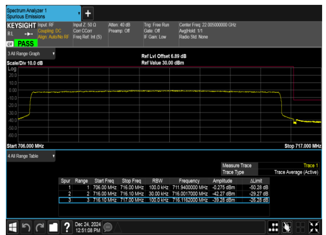
Band12-10MHz-16QAM-23130-50RB#0-PASS
