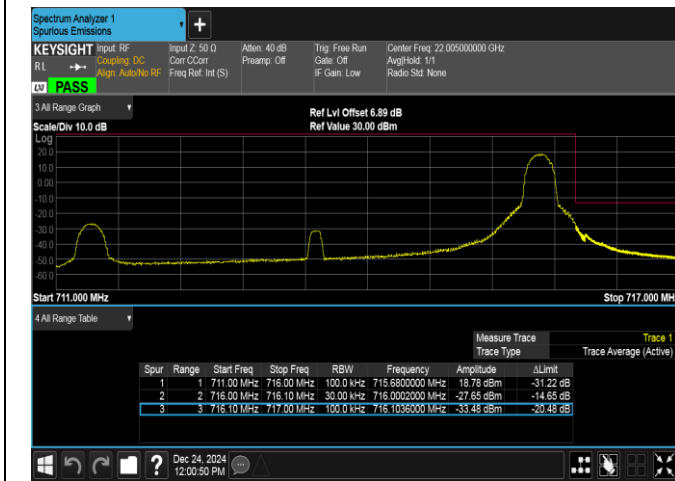
Band12-5MHz-16QAM-23155-1RB#24-PASS
