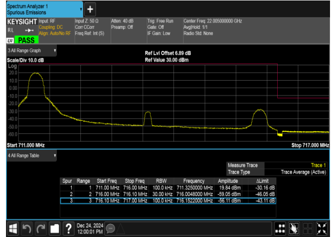
Band12-5MHz-QPSK-23155-1RB#0-PASS
