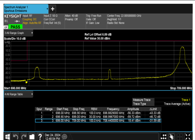
Band12-10MHz-16QAM-23060-1RB#49-PASS
