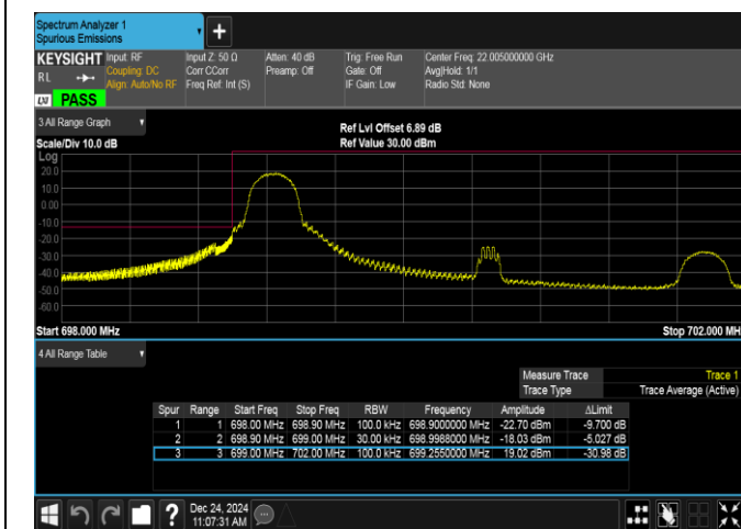
Band12-3MHz-16QAM-23025-1RB#0-PASS
