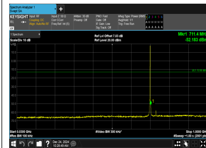
Band12-1.4MHz-QPSK-23095-1RB#5-30~1000-PASS
