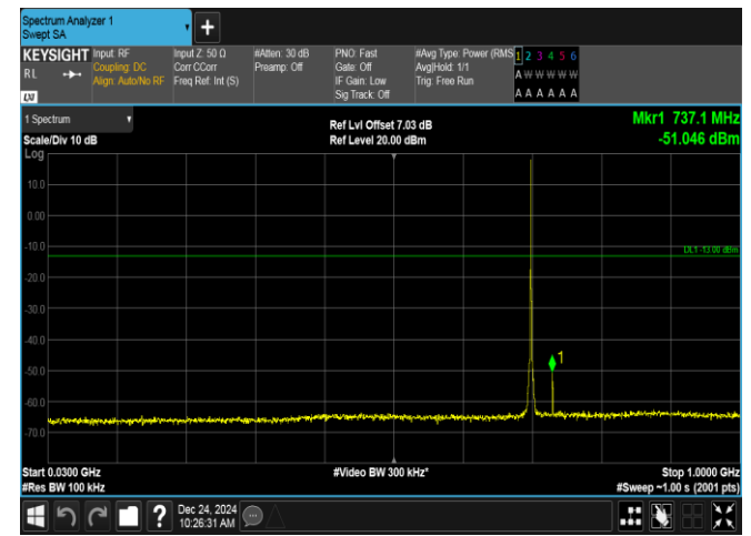
Band12-1.4MHz-QPSK-23095-1RB#0-30~1000-PASS
