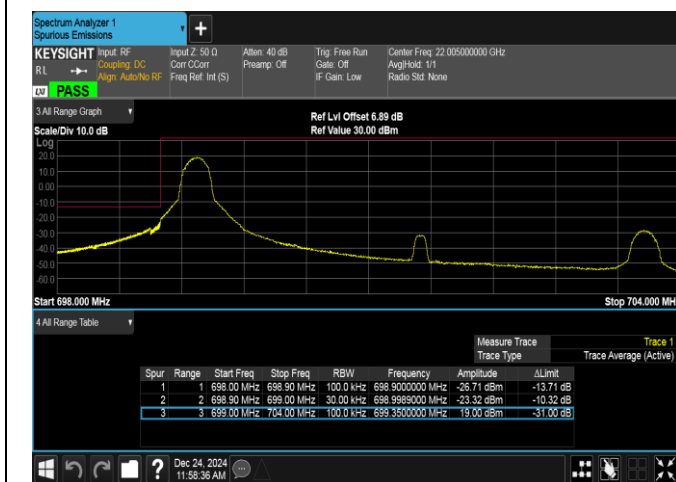
Band12-5MHz-16QAM-23035-1RB#0-PASS
