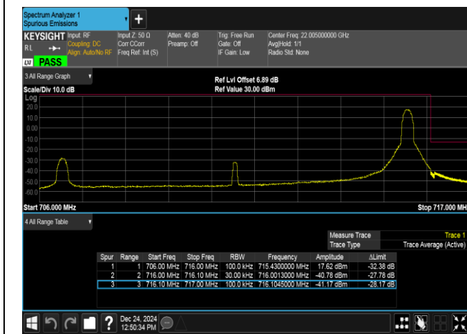
Band12-10MHz-16QAM-23130-1RB#49-PASS
