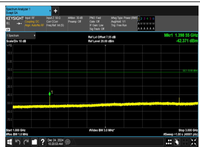
Band12-1.4MHz-QPSK-23017-1RB#0-1000~3000-PASS
