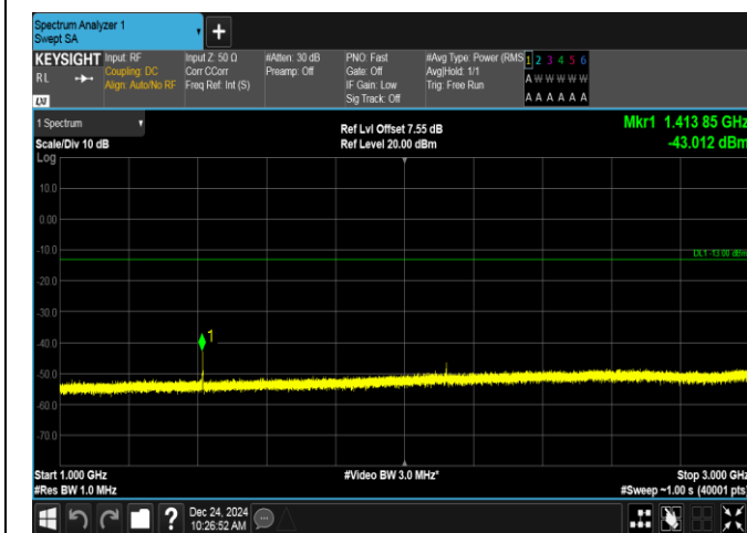
Band12-1.4MHz-QPSK-23095-1RB#0-1000~3000-PASS
