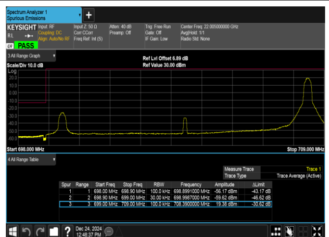
Band12-10MHz-QPSK-23060-1RB#49-PASS
