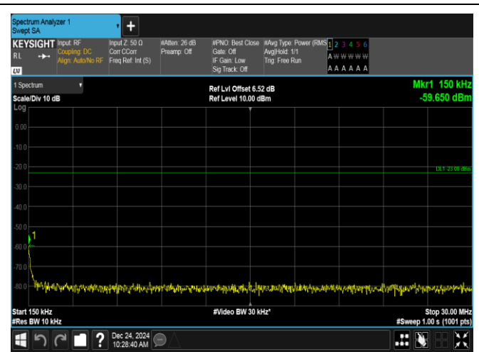
Band12-1.4MHz-QPSK-23095-1RB#5-0.15~30-PASS
