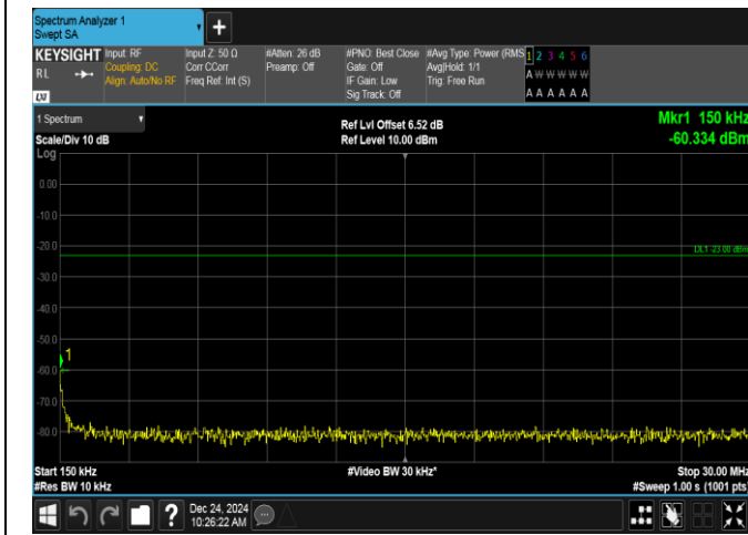
Band12-1.4MHz-QPSK-23095-1RB#0-0.15~30-PASS
