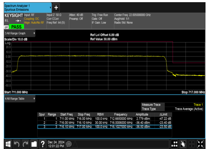
Band12-5MHz-16QAM-23155-25RB#0-PASS
