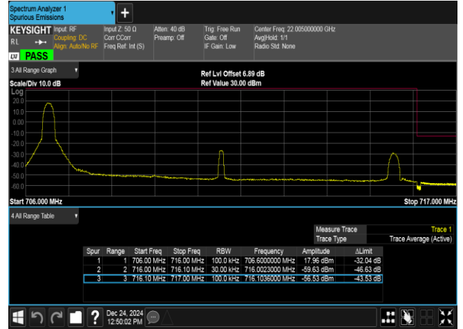
Band12-10MHz-16QAM-23130-1RB#0-PASS
