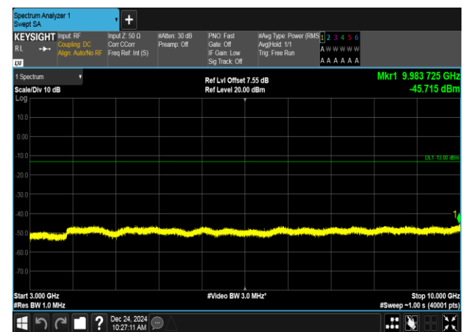
Band12-1.4MHz-QPSK-23095-1RB#0-3000~10000-PASS
