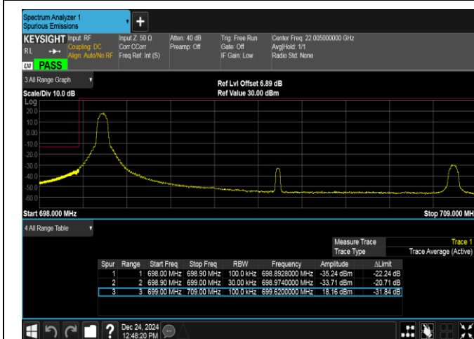
Band12-10MHz-16QAM-23060-1RB#0-PASS
