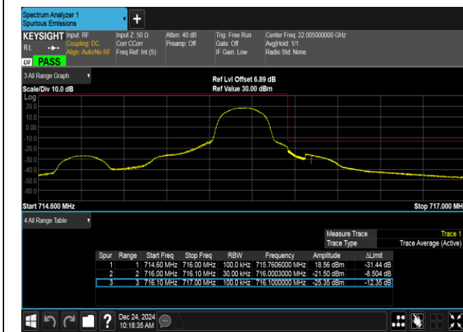
Band12-1.4MHz-16QAM-23173-1RB#5-PASS
