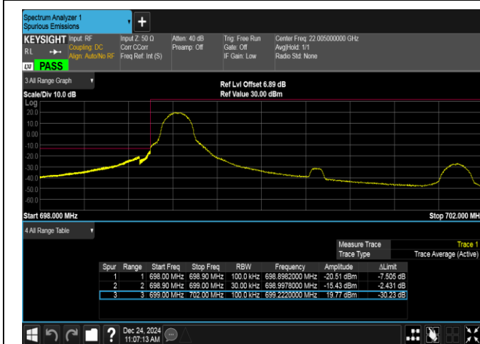
Band12-3MHz-QPSK-23025-1RB#0-PASS
