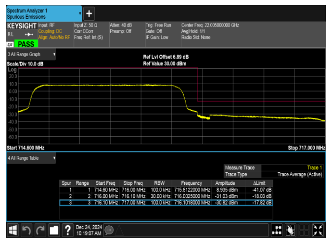
Band12-1.4MHz-16QAM-23173-6RB#0-PASS
