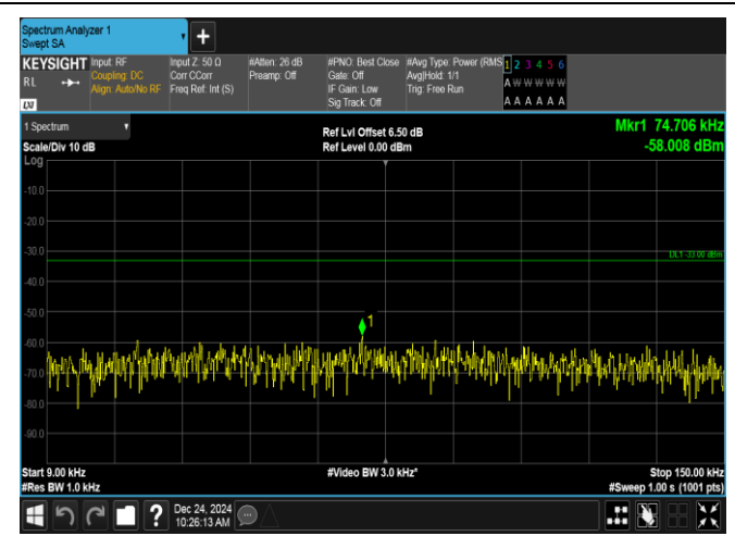
Band12-1.4MHz-QPSK-23095-1RB#0-0.009~0.15-PASS
