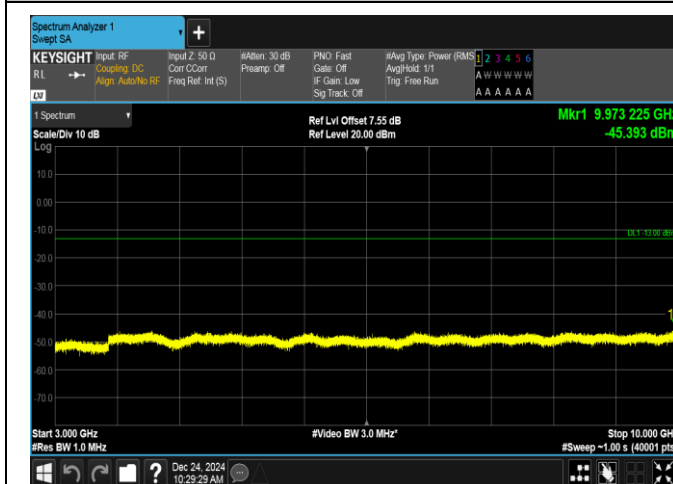
Band12-1.4MHz-QPSK-23095-1RB#5-3000~10000-PASS
