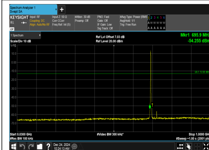
Band12-1.4MHz-QPSK-23017-6RB#0-30~1000-PASS
