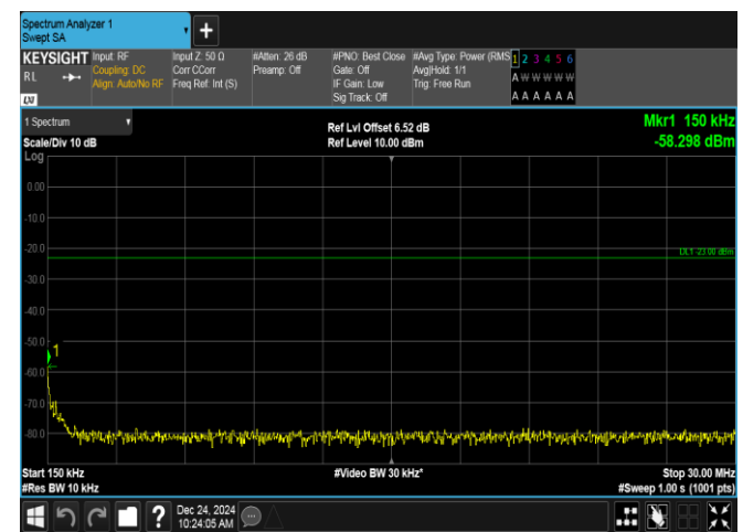
Band12-1.4MHz-QPSK-23017-6RB#0-0.15~30-PASS
