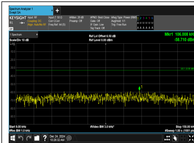
Band12-1.4MHz-QPSK-23095-1RB#5-0.009~0.15-PASS
