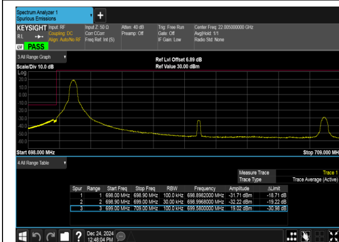
Band12-10MHz-QPSK-23060-1RB#0-PASS
