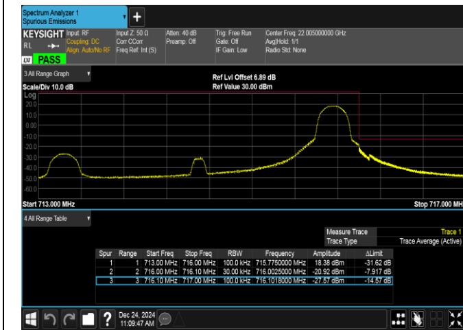
Band12-3MHz-16QAM-23165-1RB#14-PASS
