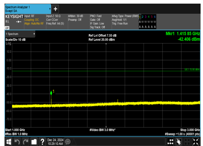
Band12-1.4MHz-QPSK-23095-1RB#5-1000~3000-PASS
