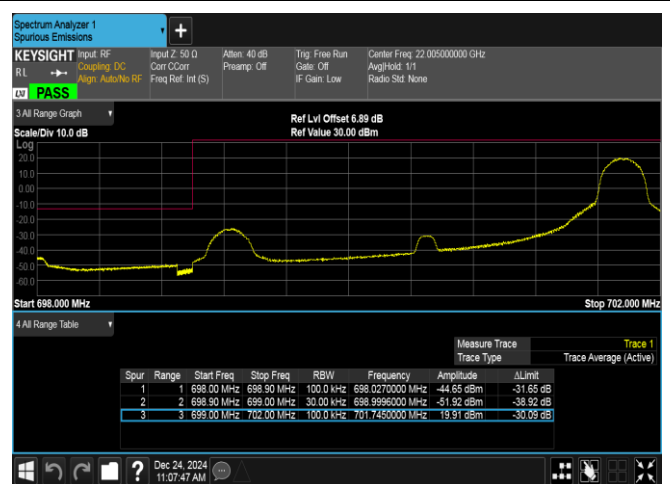
Band12-3MHz-QPSK-23025-1RB#14-PASS
