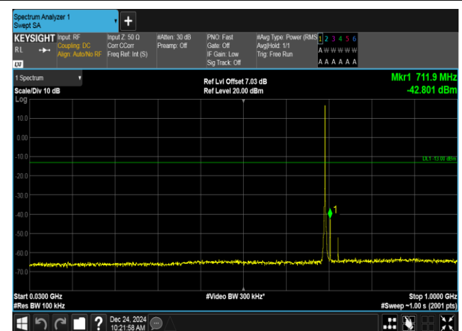
Band12-1.4MHz-QPSK-23017-1RB#5-30~1000-PASS
