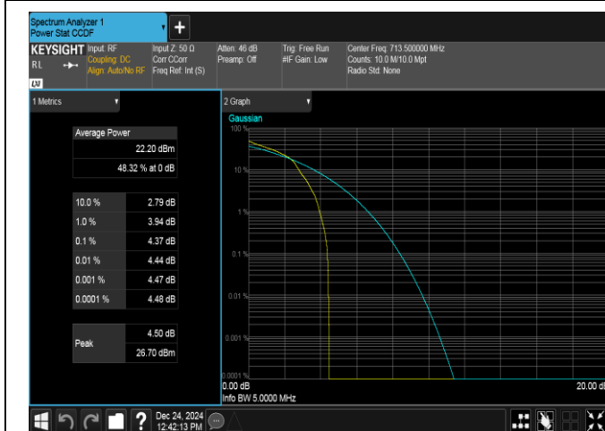
Band12-5MHz-16QAM-23155-1RB#0-PASS
