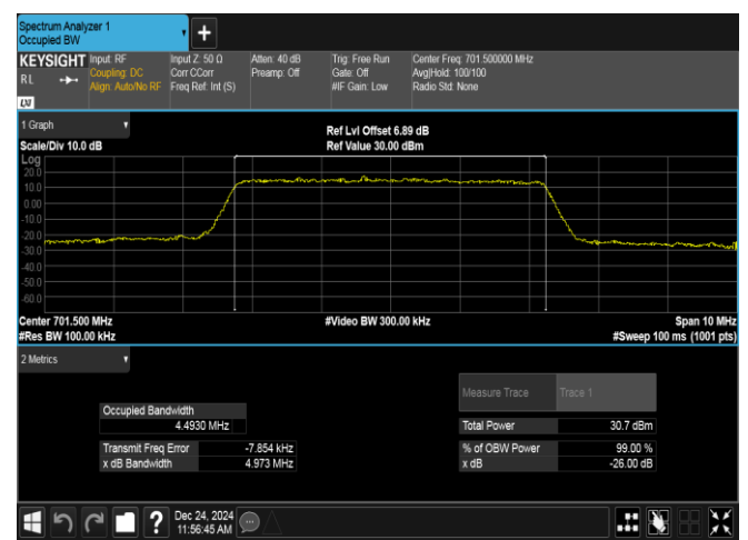
Band12-5MHz-16QAM-23035-25RB#0-PASS
