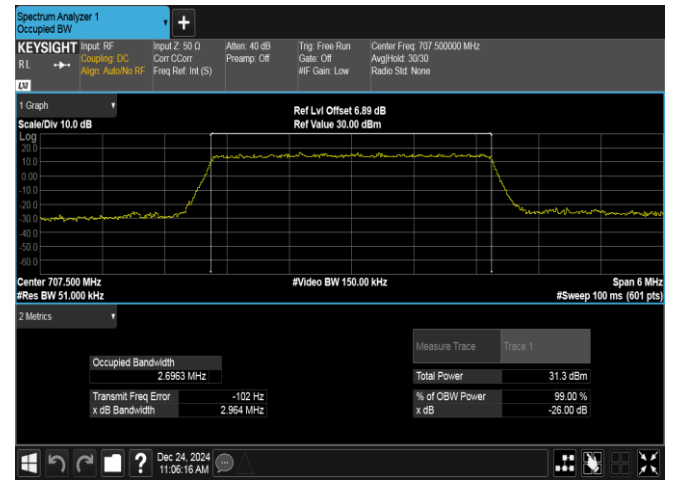
Band12-3MHz-QPSK-23095-15RB#0-PASS
