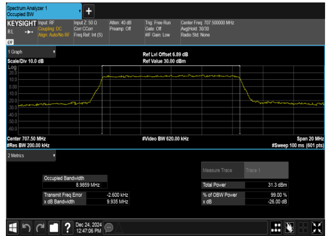
Band12-10MHz-QPSK-23095-50RB#0-PASS
