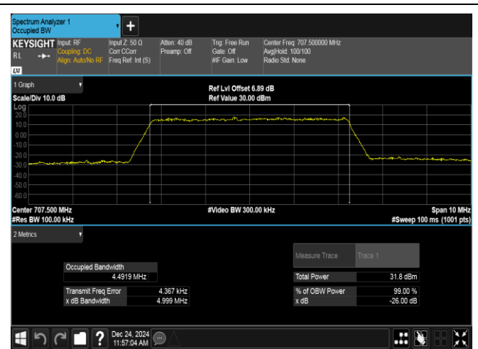
Band12-5MHz-QPSK-23095-25RB#0-PASS
