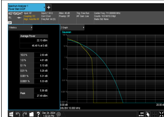
Band12-10MHz-16QAM-23130-1RB#0-PASS
