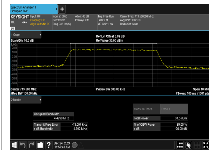
Band12-5MHz-QPSK-23155-25RB#0-PASS
