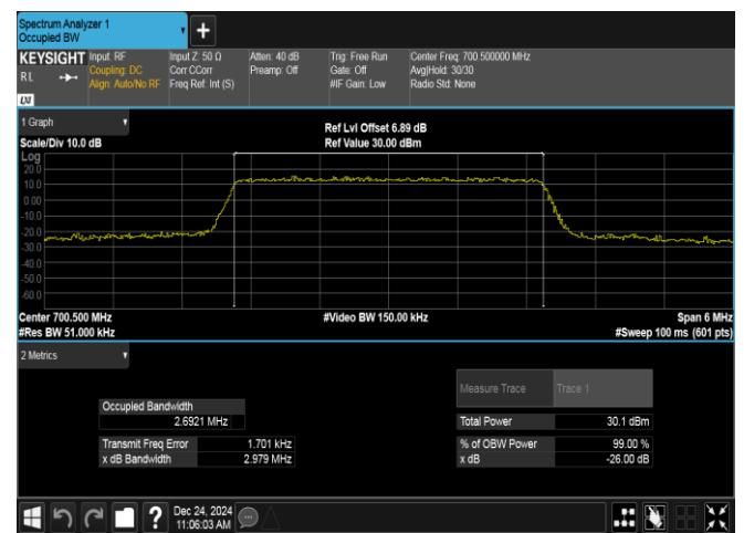
Band12-3MHz-16QAM-23025-15RB#0-PASS
