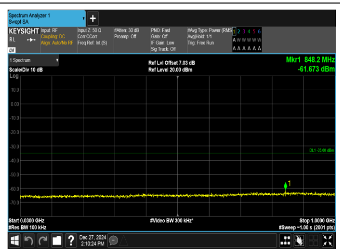
Band7-20MHz-16QAM-21350-100RB#0-30~1000-PASS
