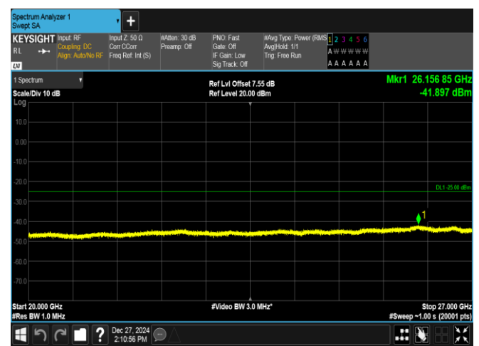
Band7-20MHz-16QAM-21350-100RB#0-20000~27000-PASS
