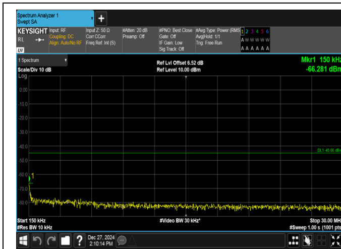
Band7-20MHz-16QAM-21350-100RB#0-0.15~30-PASS
