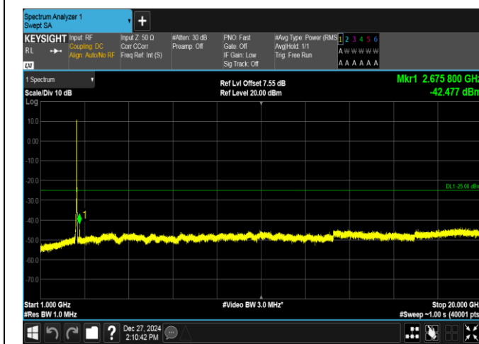
Band7-20MHz-16QAM-21350-100RB#0-1000~20000-PASS
