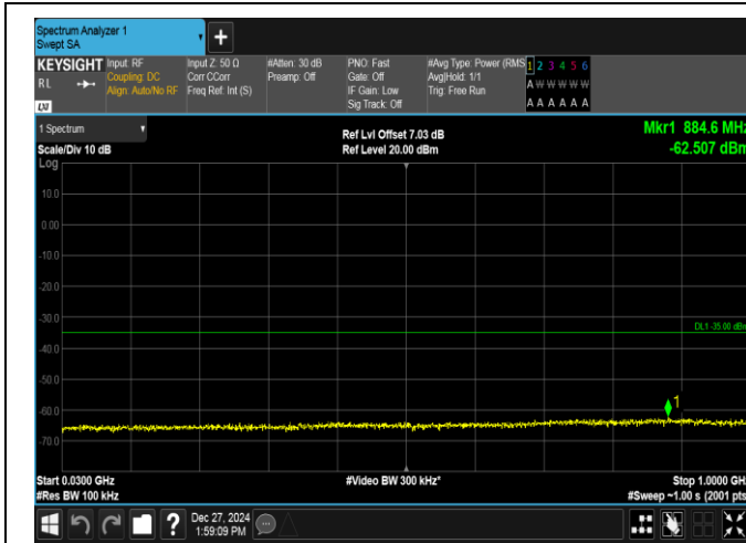
Band7-20MHz-16QAM-21100-1RB#0-30~1000-PASS
