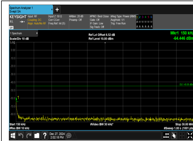
Band7-20MHz-QPSK-21100-100RB#0-0.15~30-PASS
