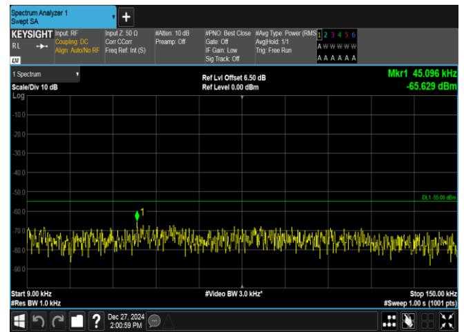
Band7-20MHz-16QAM-21100-1RB#99-0.009~0.15-PASS
