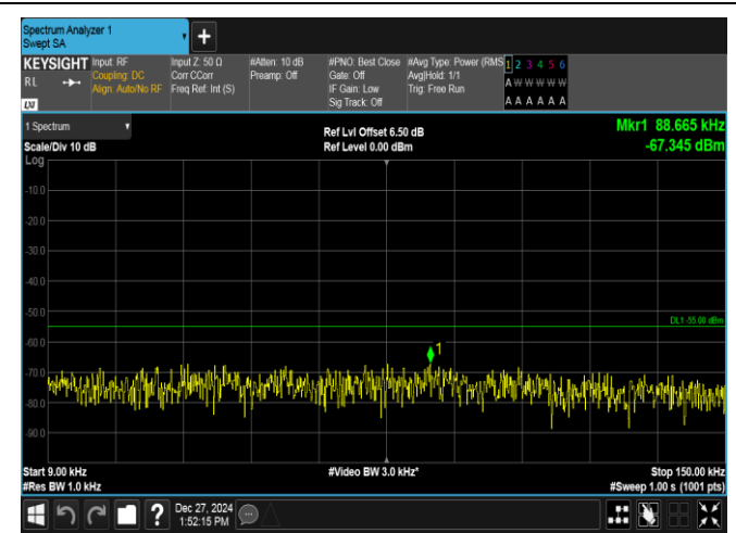
Band7-20MHz-16QAM-20850-1RB#0-0.009~0.15-PASS
