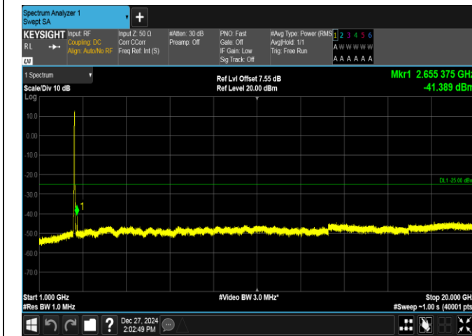
Band7-20MHz-QPSK-21100-100RB#0-1000~20000-PASS
