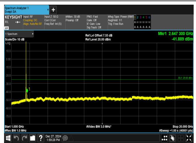
Band7-20MHz-16QAM-21100-1RB#0-1000~20000-PASS
