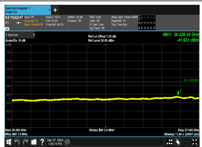
Band7-20MHz-QPSK-20850-1RB#99-20000~27000-PASS
