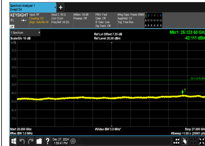
Band7-20MHz-16QAM-21100-1RB#0-20000~27000-PASS
