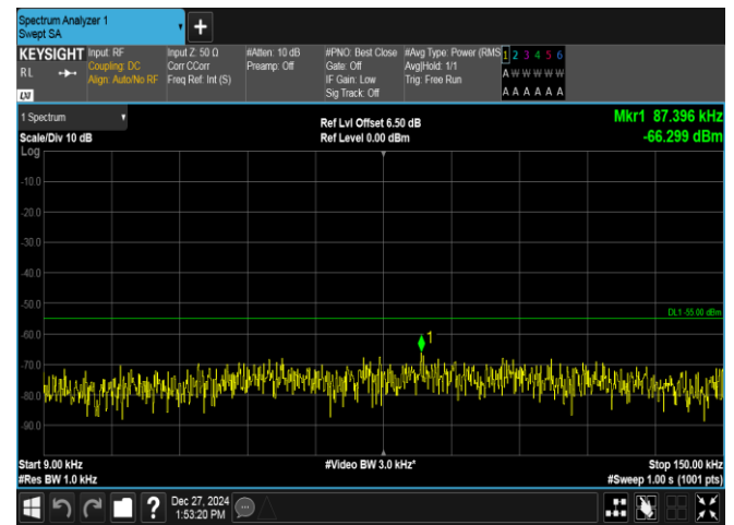
Band7-20MHz-QPSK-20850-1RB#99-0.009~0.15-PASS
