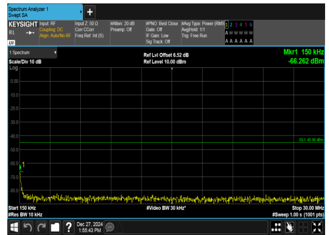
Band7-20MHz-QPSK-20850-100RB#0-0.15~30-PASS
