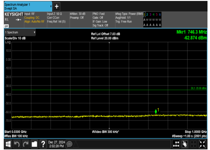
Band7-20MHz-QPSK-21100-100RB#0-30~1000-PASS
