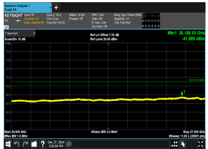
Band7-20MHz-QPSK-21100-100RB#0-20000~27000-PASS
