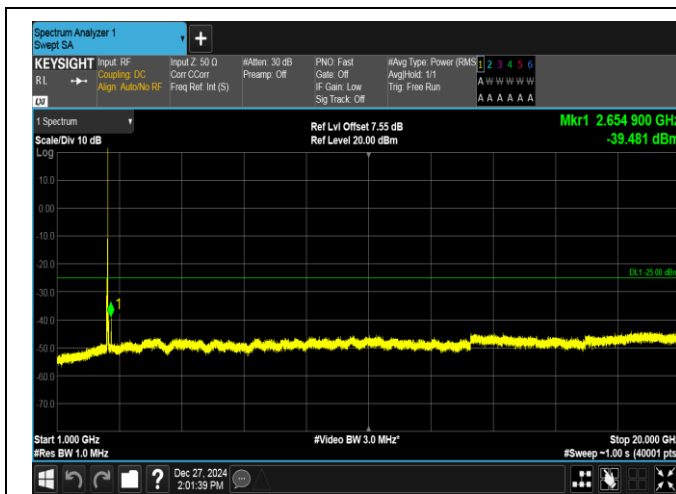
Band7-20MHz-16QAM-21100-1RB#99-1000~20000-PASS
