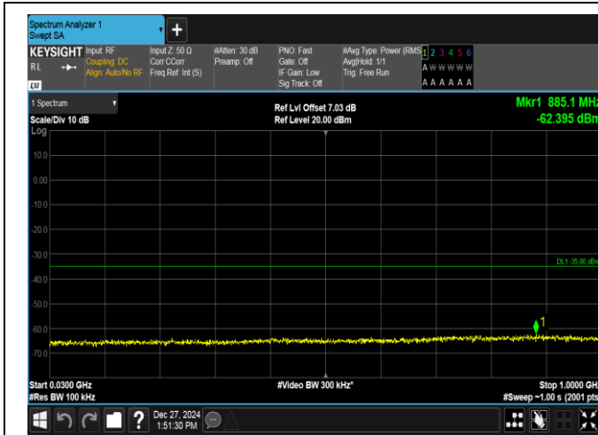
Band7-20MHz-QPSK-20850-1RB#0-30~1000-PASS
