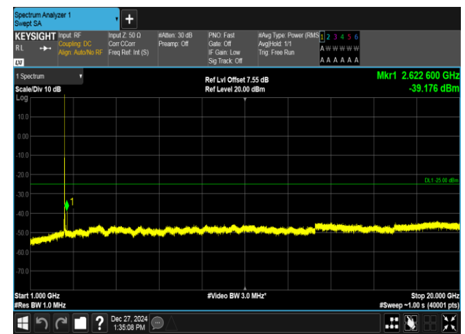
Band7-15MHz-16QAM-20825-1RB#74-1000~20000-PASS
