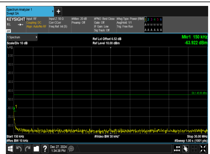
Band7-15MHz-16QAM-20825-1RB#74-0.15~30-PASS
