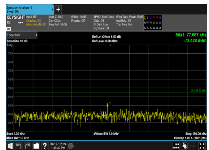
Band7-15MHz-16QAM-20825-75RB#0-0.009~0.15-PASS
