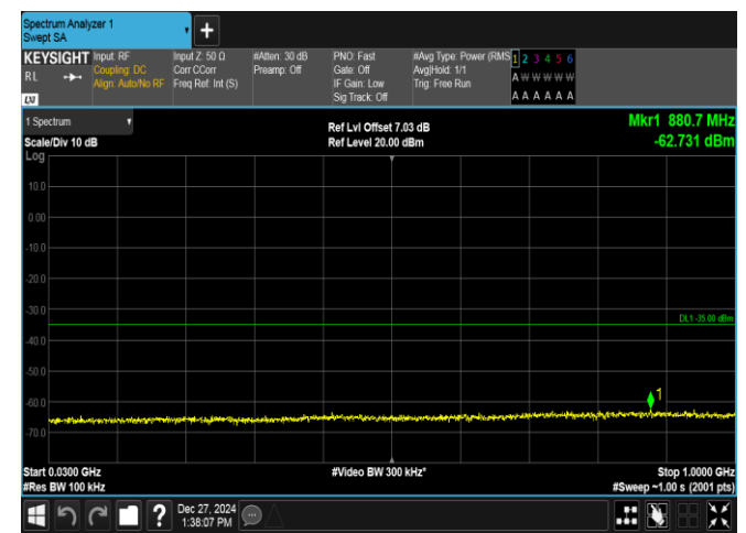
Band7-15MHz-QPSK-21100-1RB#0-30~1000-PASS
