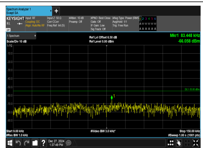
Band7-15MHz-QPSK-21100-1RB#0-0.009~0.15-PASS
