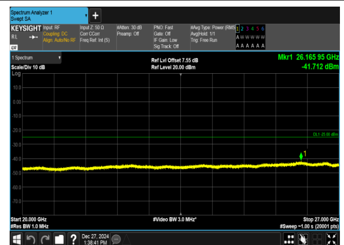
Band7-15MHz-QPSK-21100-1RB#0-20000~27000-PASS
