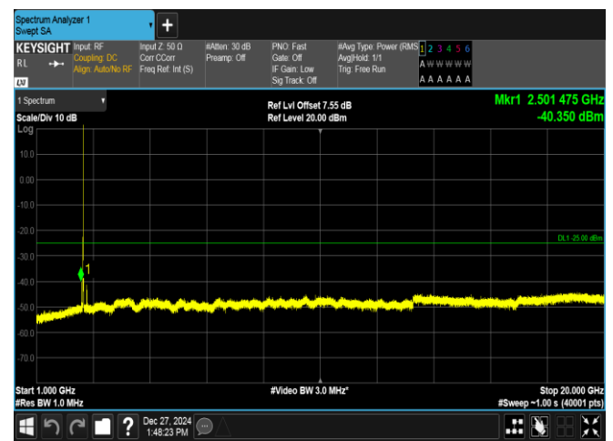
Band7-15MHz-16QAM-21375-1RB#74-1000~20000-PASS
