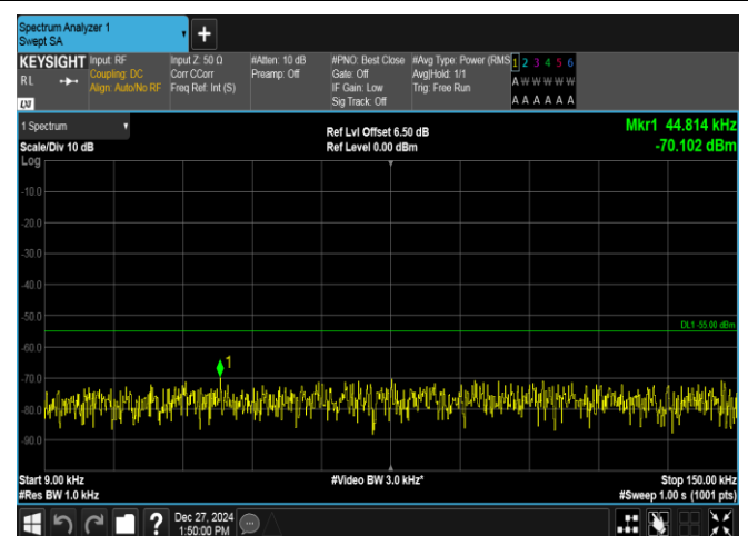
Band7-15MHz-16QAM-21375-75RB#0-0.009~0.15-PASS
