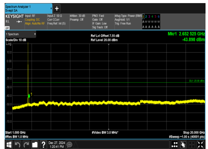
Band7-10MHz-QPSK-21100-1RB#49-1000~20000-PASS
