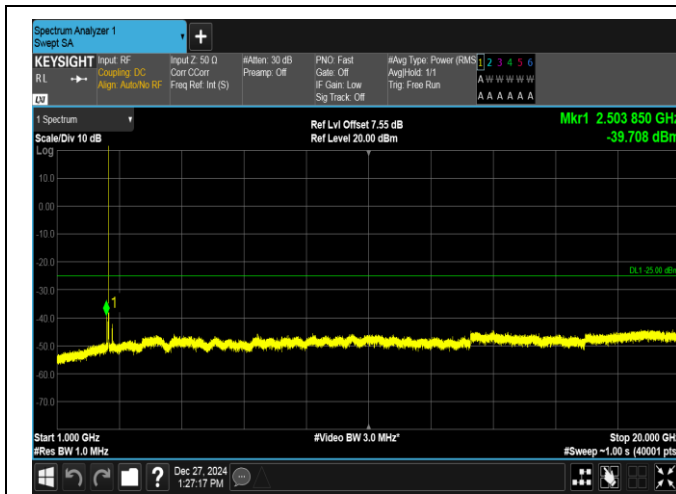
Band7-10MHz-QPSK-21400-1RB#49-1000~20000-PASS
