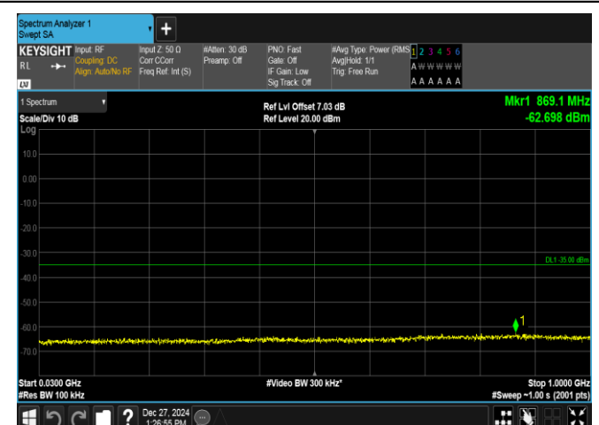
Band7-10MHz-QPSK-21400-1RB#49-30~1000-PASS
