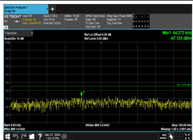
Band7-15MHz-QPSK-20825-1RB#74-0.009~0.15-PASS
