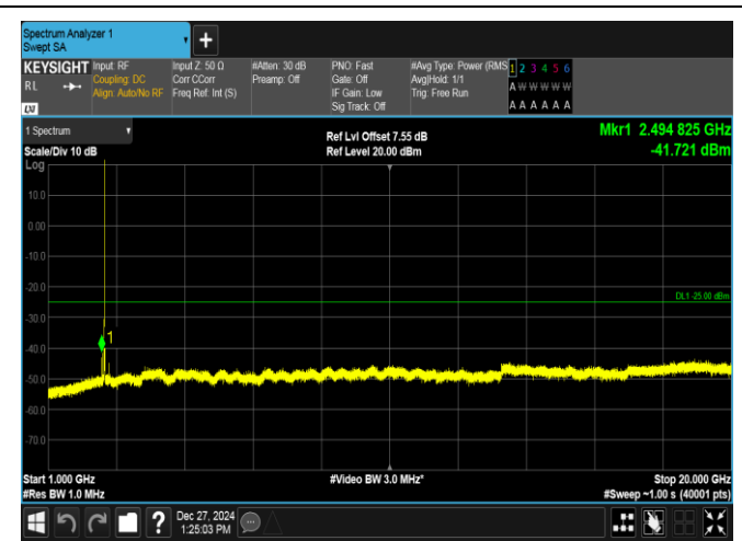
Band7-10MHz-QPSK-21400-1RB#0-1000~20000-PASS
