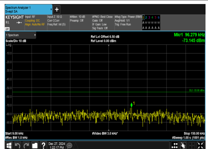
Band7-10MHz-QPSK-21100-50RB#0-0.009~0.15-PASS
