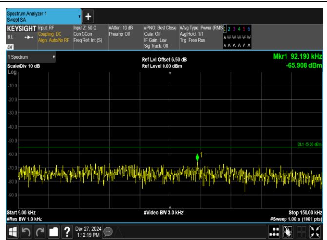
Band7-10MHz-16QAM-20800-1RB#0-0.009~0.15-PASS
