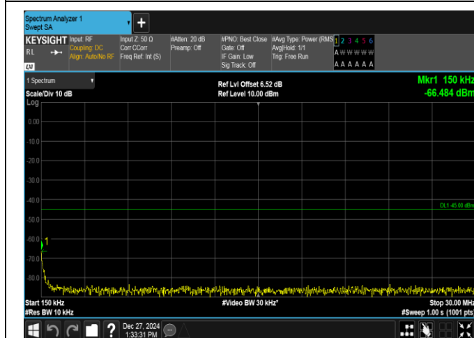
Band7-15MHz-QPSK-20825-1RB#74-0.15~30-PASS
