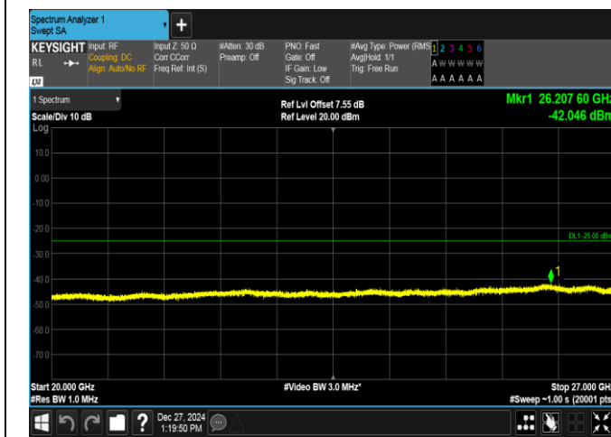
Band7-10MHz-16QAM-21100-1RB#0-20000~27000-PASS
