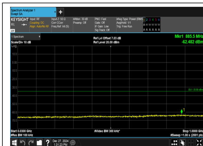
Band7-15MHz-QPSK-20825-1RB#0-30~1000-PASS
