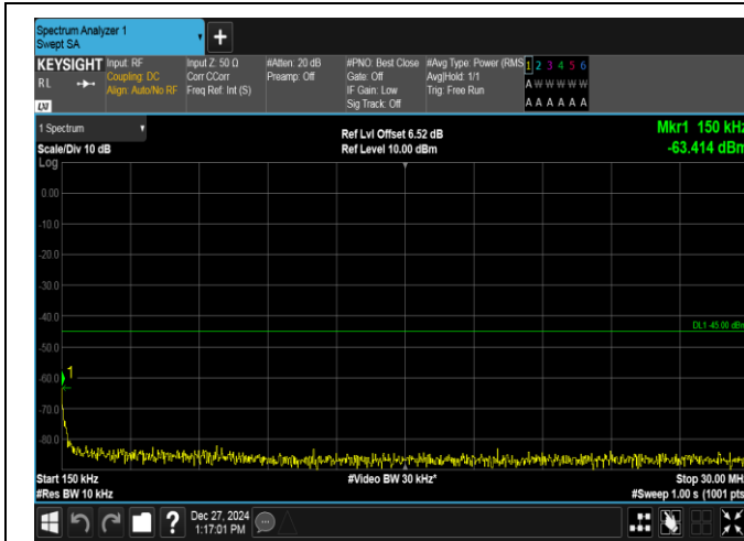
Band7-10MHz-16QAM-20800-50RB#0-0.15~30-PASS
