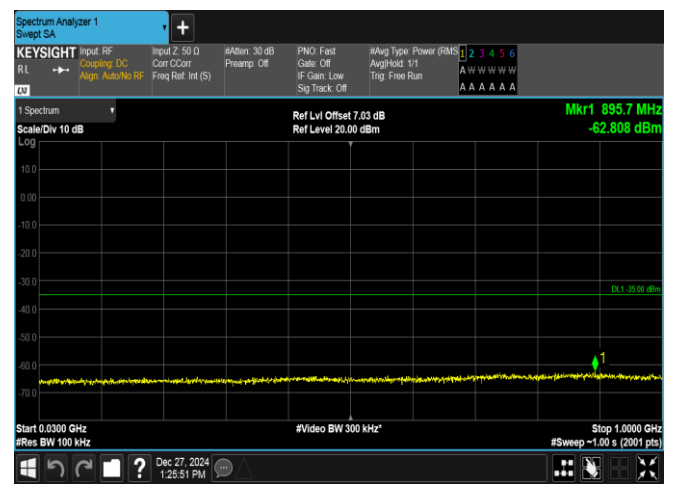
Band7-10MHz-16QAM-21400-1RB#0-30~1000-PASS
