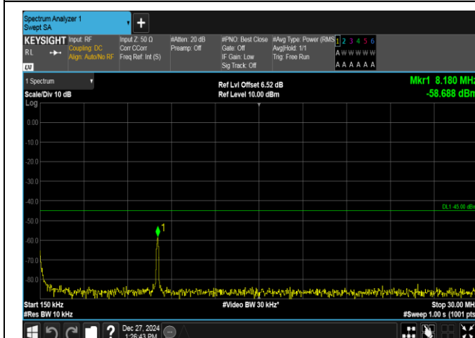
Band7-10MHz-QPSK-21400-1RB#49-0.15~30-PASS
