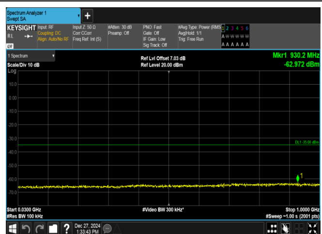
Band7-15MHz-QPSK-20825-1RB#74-30~1000-PASS
