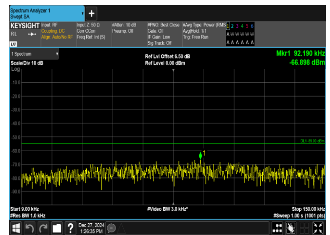
Band7-10MHz-QPSK-21400-1RB#49-0.009~0.15-PASS
