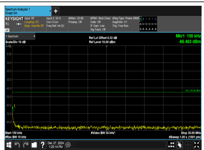
Band7-10MHz-QPSK-21100-1RB#49-0.15~30-PASS
