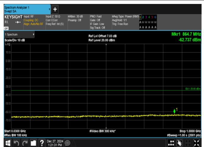
Band7-10MHz-16QAM-21100-1RB#49-30~1000-PASS
