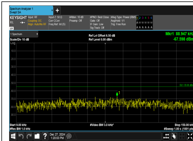
Band7-10MHz-QPSK-21100-1RB#49-0.009~0.15-PASS
