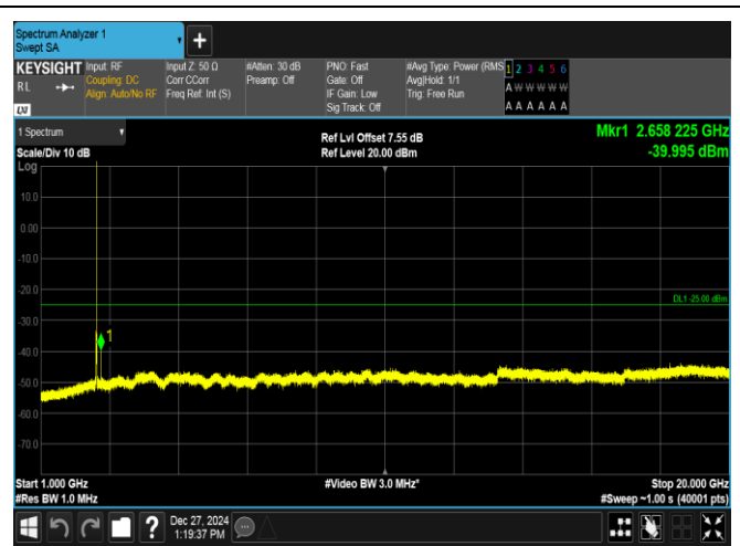
Band7-10MHz-16QAM-21100-1RB#0-1000~20000-PASS
