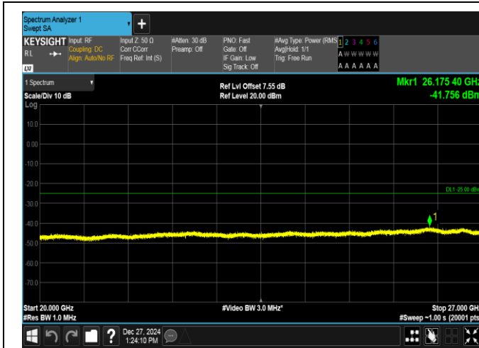
Band7-10MHz-16QAM-21100-50RB#0-20000~27000-PASS
