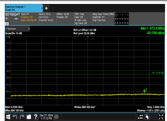
Band7-10MHz-16QAM-20800-50RB#0-30~1000-PASS
