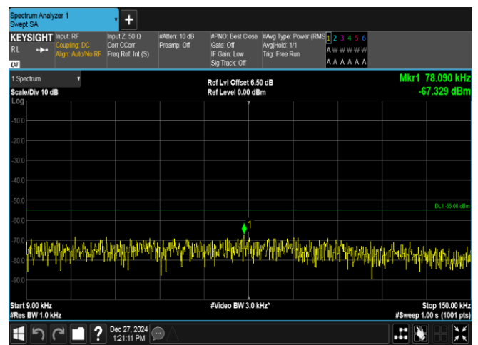
Band7-10MHz-16QAM-21100-1RB#49-0.009~0.15-PASS
