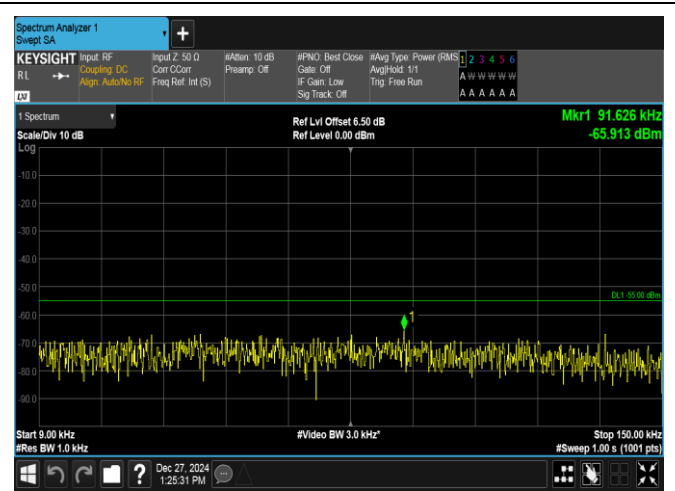
Band7-10MHz-16QAM-21400-1RB#0-0.009~0.15-PASS
