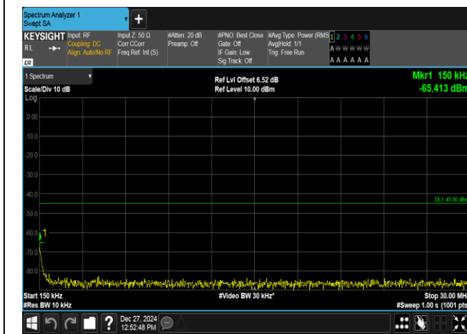
Band7-5MHz-16QAM-20775-1RB#0-0.15~30-PASS
