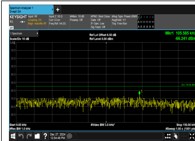
Band7-5MHz-16QAM-20775-1RB#24-0.009~0.15-PASS
