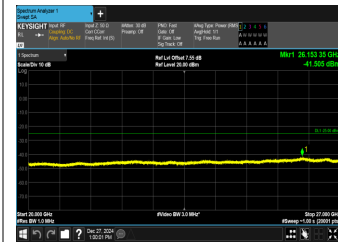
Band7-5MHz-16QAM-21100-1RB#0-20000~27000-PASS
