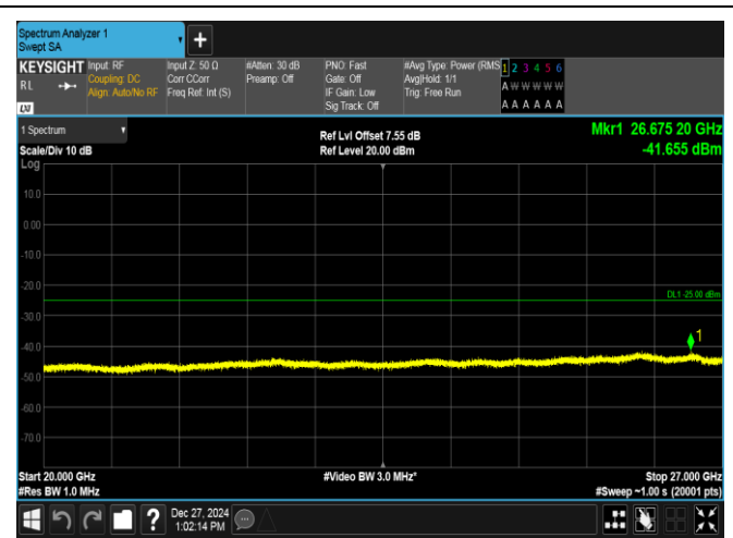
Band7-5MHz-16QAM-21100-1RB#24-20000~27000-PASS
