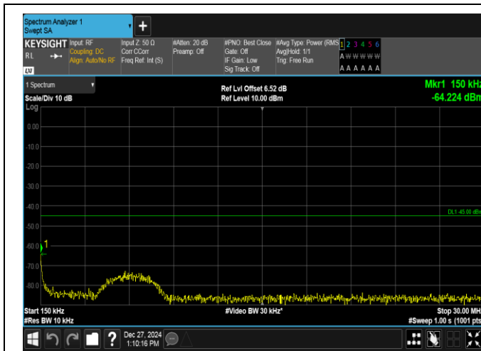
Band7-5MHz-16QAM-21425-25RB#0-0.15~30-PASS
