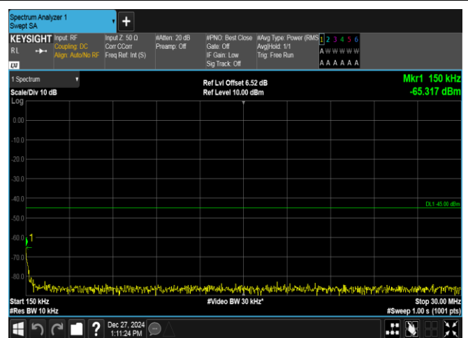
Band7-10MHz-QPSK-20800-1RB#0-0.15~30-PASS
