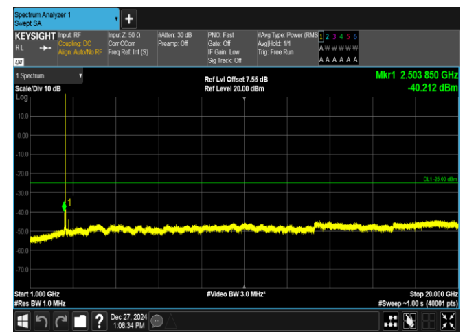
Band7-5MHz-16QAM-21425-1RB#24-1000~20000-PASS
