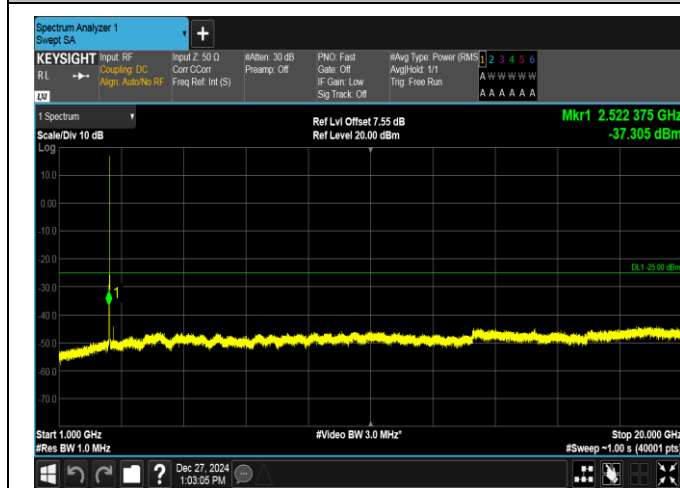
Band7-5MHz-QPSK-21100-25RB#0-1000~20000-PASS
