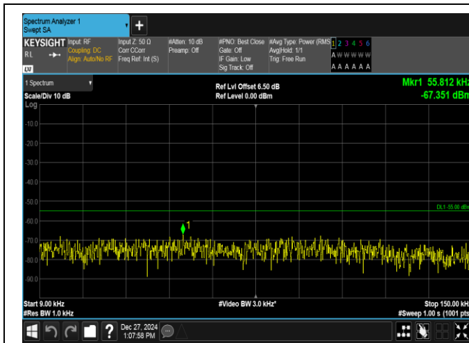
Band7-5MHz-16QAM-21425-1RB#24-0.009~0.15-PASS
