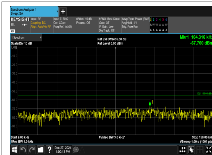
Band7-5MHz-QPSK-21100-1RB#24-0.009~0.15-PASS
