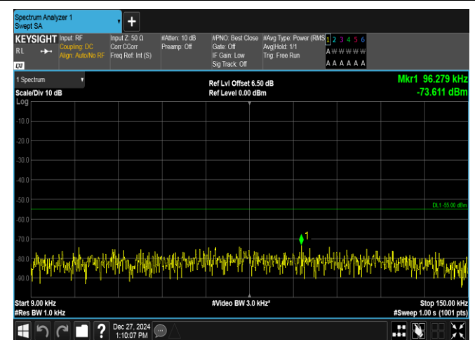
Band7-5MHz-16QAM-21425-25RB#0-0.009~0.15-PASS
