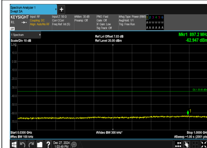
Band7-5MHz-16QAM-21100-25RB#0-30~1000-PASS
