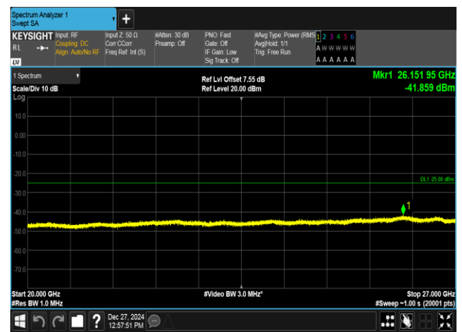
Band7-5MHz-16QAM-20775-25RB#0-20000~27000-PASS
