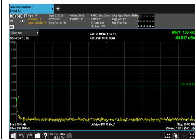
Band7-10MHz-QPSK-20800-1RB#49-0.15~30-PASS
