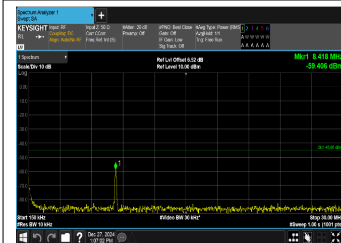
Band7-5MHz-QPSK-21425-1RB#24-0.15~30-PASS
