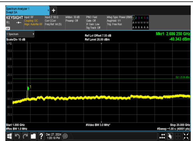
Band7-5MHz-QPSK-21425-1RB#0-1000~20000-PASS
