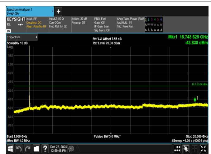
Band7-5MHz-16QAM-21100-1RB#0-1000~20000-PASS
