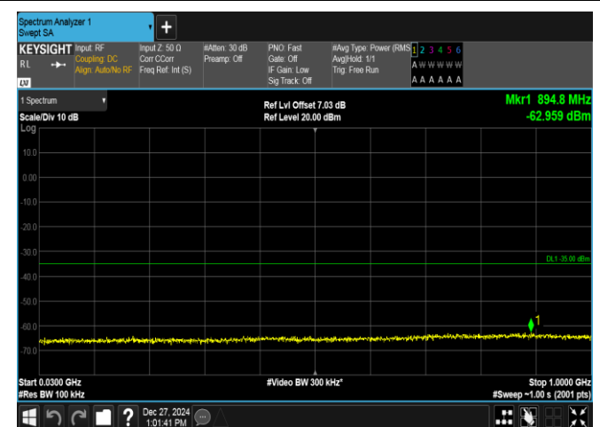
Band7-5MHz-16QAM-21100-1RB#24-30~1000-PASS
