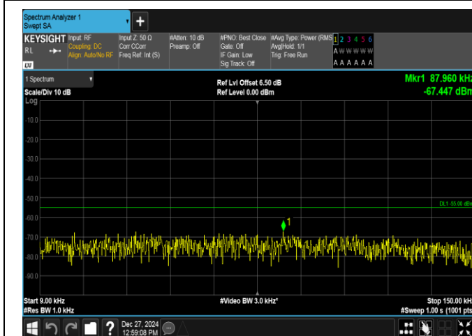
Band7-5MHz-16QAM-21100-1RB#0-0.009~0.15-PASS
