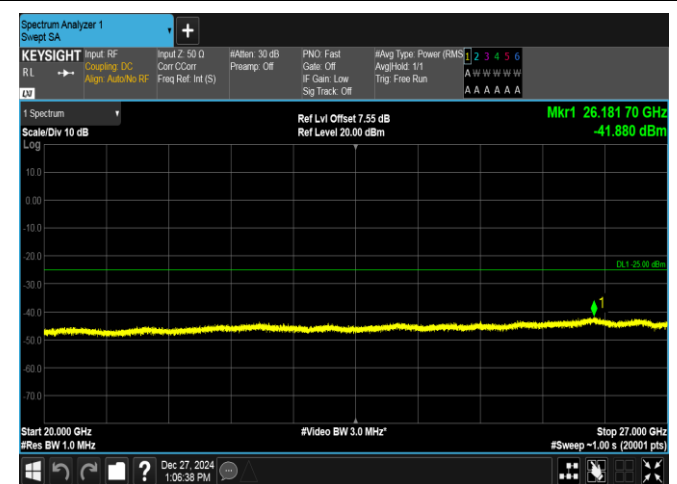
Band7-5MHz-16QAM-21425-1RB#0-20000~27000-PASS
