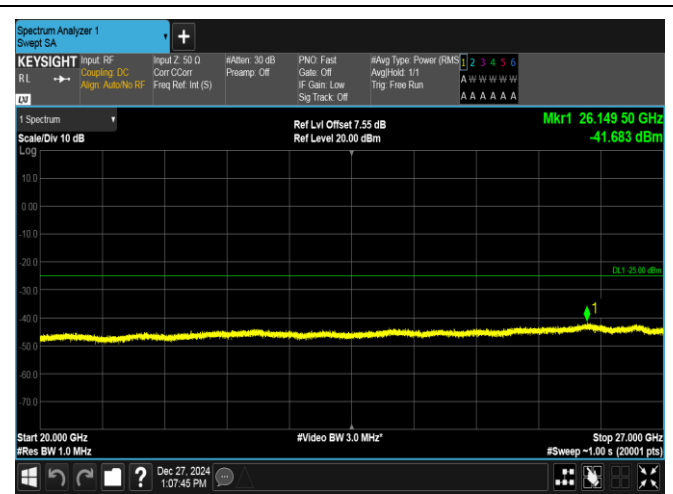
Band7-5MHz-QPSK-21425-1RB#24-20000~27000-PASS
