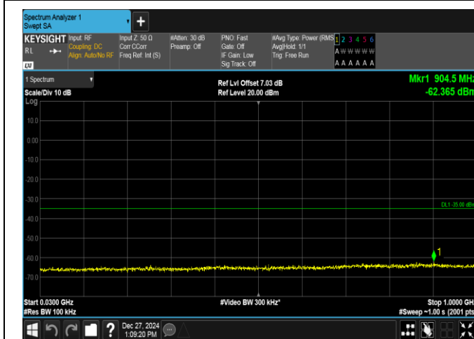
Band7-5MHz-QPSK-21425-25RB#0-30~1000-PASS
