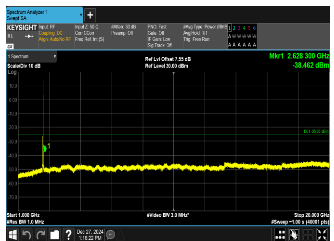
Band7-10MHz-QPSK-20800-50RB#0-1000~20000-PASS
