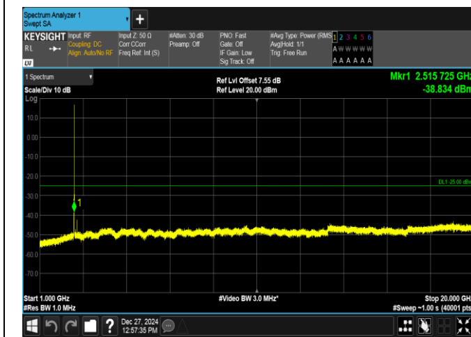
Band7-5MHz-16QAM-20775-25RB#0-1000~20000-PASS
