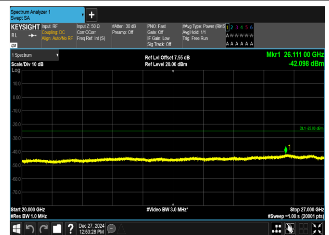
Band7-5MHz-16QAM-20775-1RB#0-20000~27000-PASS
