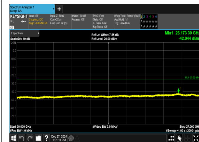
Band7-5MHz-QPSK-21100-1RB#24-20000~27000-PASS
