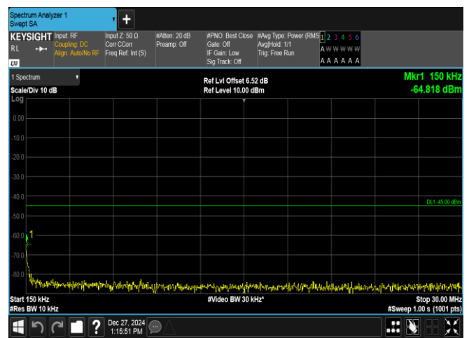
Band7-10MHz-QPSK-20800-50RB#0-0.15~30-PASS
