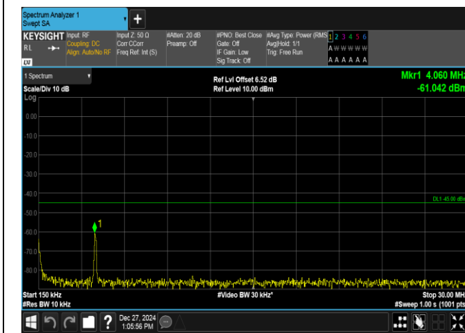
Band7-5MHz-16QAM-21425-1RB#0-0.15~30-PASS
