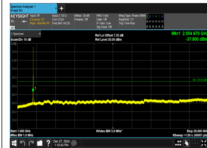
Band7-5MHz-16QAM-21425-25RB#0-1000~20000-PASS
