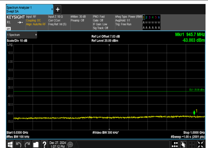
Band7-5MHz-QPSK-21425-1RB#24-30~1000-PASS
