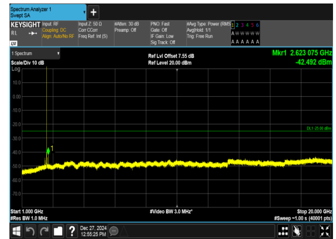
Band7-5MHz-16QAM-20775-1RB#24-1000~20000-PASS
