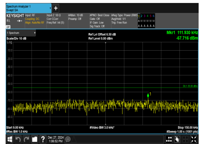
Band7-5MHz-QPSK-21425-1RB#24-0.009~0.15-PASS
