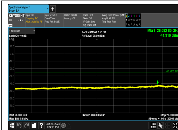
Band7-5MHz-16QAM-21100-25RB#0-20000~27000-PASS
