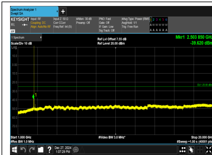
Band7-5MHz-QPSK-21425-1RB#24-1000~20000-PASS
