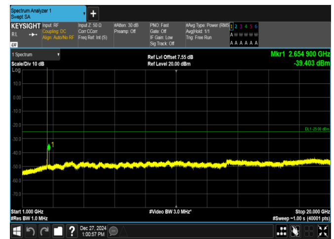
Band7-5MHz-QPSK-21100-1RB#24-1000~20000-PASS
