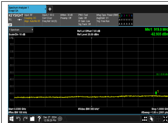
Band7-5MHz-16QAM-21100-1RB#0-30~1000-PASS
