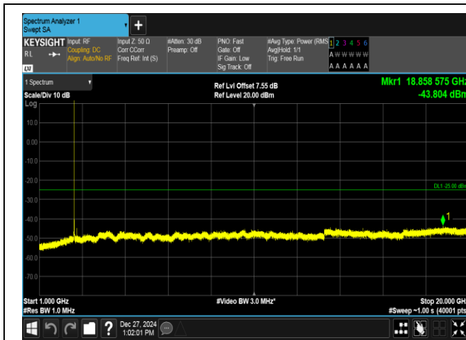
Band7-5MHz-16QAM-21100-1RB#24-1000~20000-PASS
