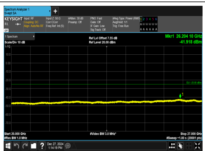
Band7-10MHz-QPSK-20800-1RB#49-20000~27000-PASS
