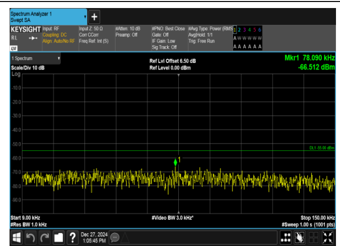
Band7-5MHz-16QAM-21425-1RB#0-0.009~0.15-PASS
