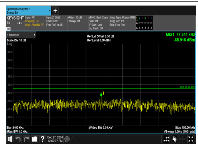
Band7-5MHz-16QAM-20775-1RB#0-0.009~0.15-PASS
