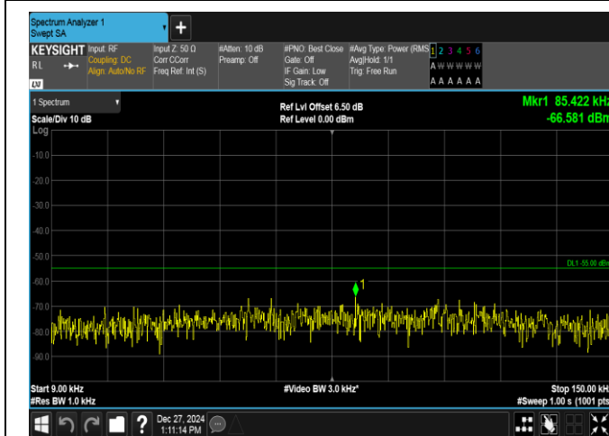
Band7-10MHz-QPSK-20800-1RB#0-0.009~0.15-PASS
