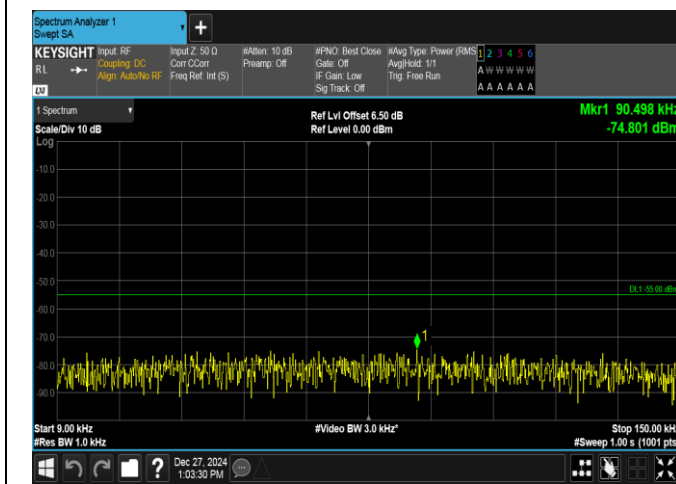
Band7-5MHz-16QAM-21100-25RB#0-0.009~0.15-PASS
