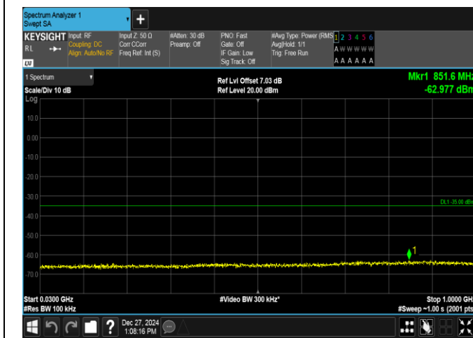
Band7-5MHz-16QAM-21425-1RB#24-30~1000-PASS
