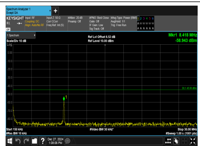
Band7-5MHz-16QAM-21425-1RB#24-0.15~30-PASS
