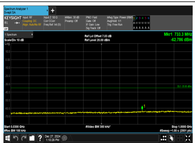
Band7-5MHz-16QAM-21425-25RB#0-30~1000-PASS
