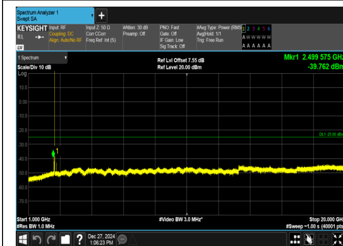
Band7-5MHz-16QAM-21425-1RB#0-1000~20000-PASS
