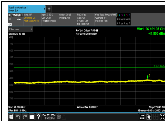
Band7-5MHz-QPSK-21425-25RB#0-20000~27000-PASS
