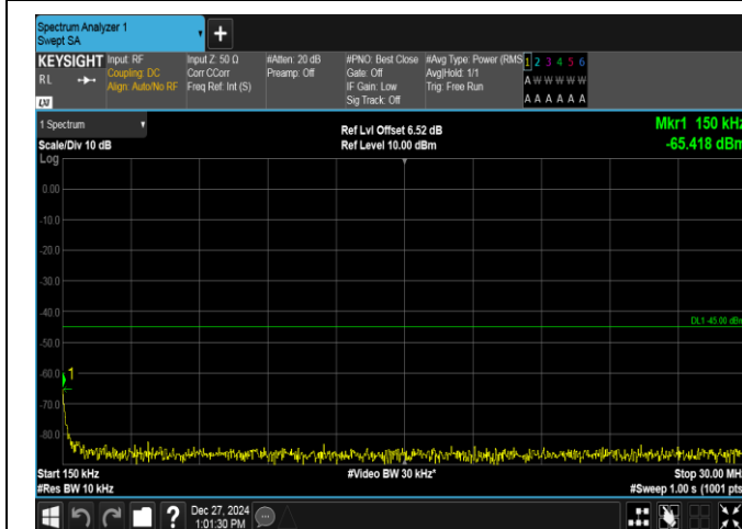
Band7-5MHz-16QAM-21100-1RB#24-0.15~30-PASS
