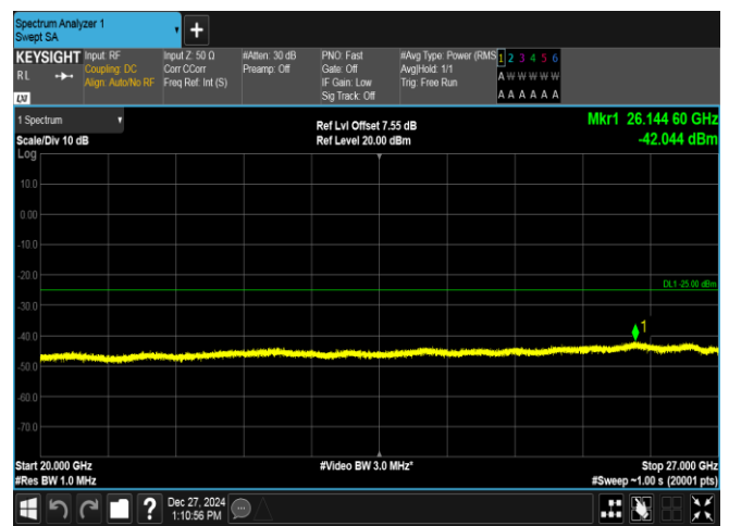
Band7-5MHz-16QAM-21425-25RB#0-20000~27000-PASS
