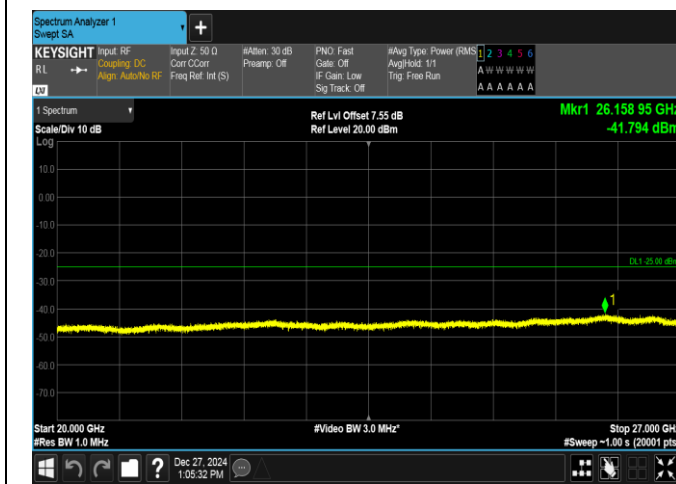
Band7-5MHz-QPSK-21425-1RB#0-20000~27000-PASS
