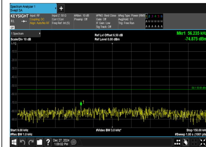
Band7-5MHz-QPSK-21425-25RB#0-0.009~0.15-PASS
