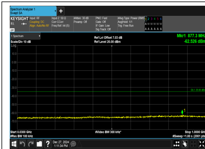
Band7-10MHz-QPSK-20800-1RB#0-30~1000-PASS
