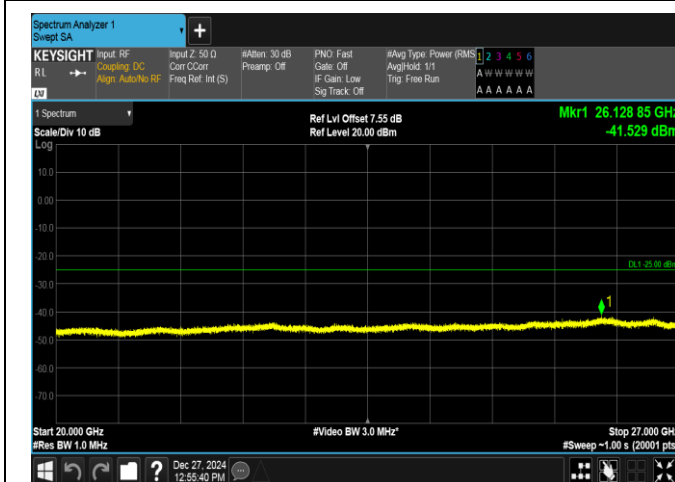
Band7-5MHz-16QAM-20775-1RB#24-20000~27000-PASS
