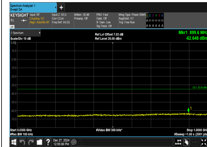
Band7-5MHz-16QAM-20775-1RB#24-30~1000-PASS
