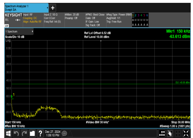
Band7-5MHz-QPSK-21425-25RB#0-0.15~30-PASS
