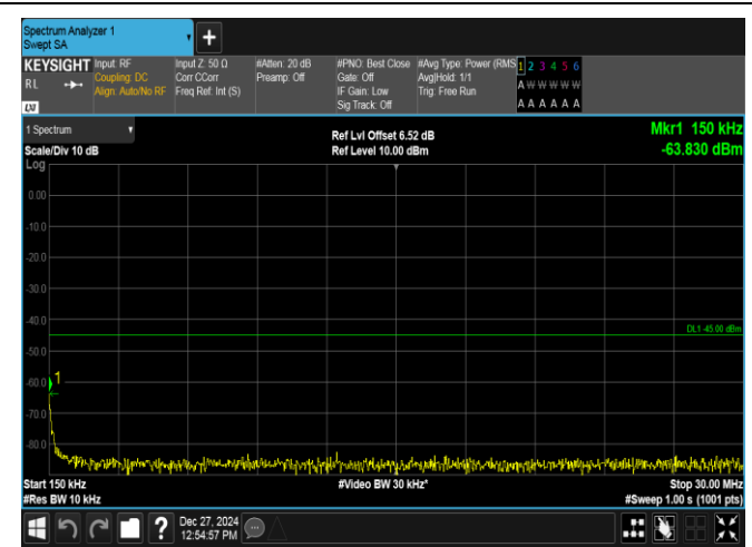
Band7-5MHz-16QAM-20775-1RB#24-0.15~30-PASS
