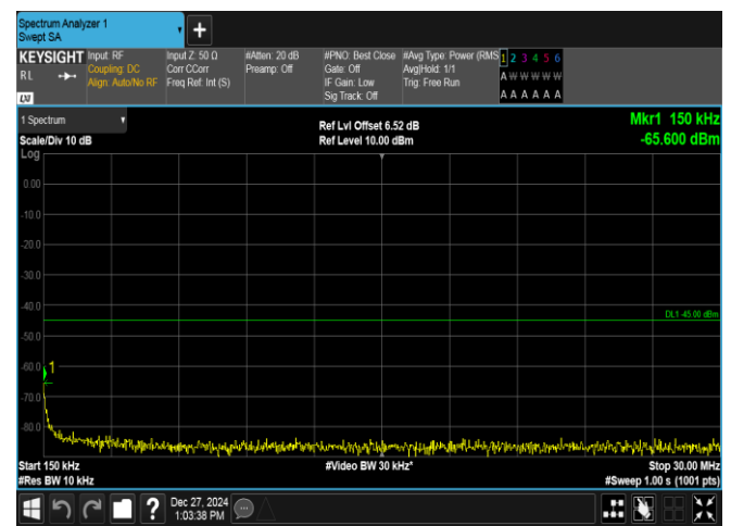
Band7-5MHz-16QAM-21100-25RB#0-0.15~30-PASS
