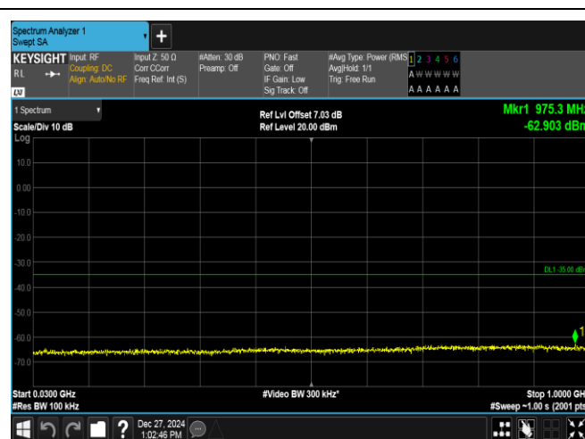
Band7-5MHz-QPSK-21100-25RB#0-30~1000-PASS
