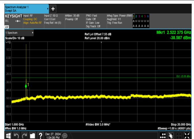
Band7-5MHz-16QAM-21100-25RB#0-1000~20000-PASS
