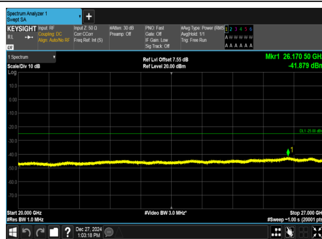
Band7-5MHz-QPSK-21100-25RB#0-20000~27000-PASS
