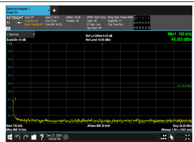
Band7-5MHz-QPSK-21100-1RB#24-0.15~30-PASS
