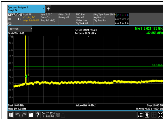
Band7-10MHz-QPSK-20800-1RB#49-1000~20000-PASS
