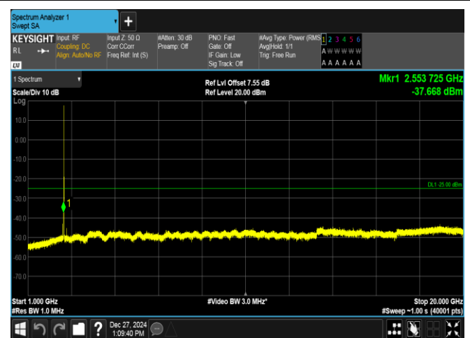
Band7-5MHz-QPSK-21425-25RB#0-1000~20000-PASS
