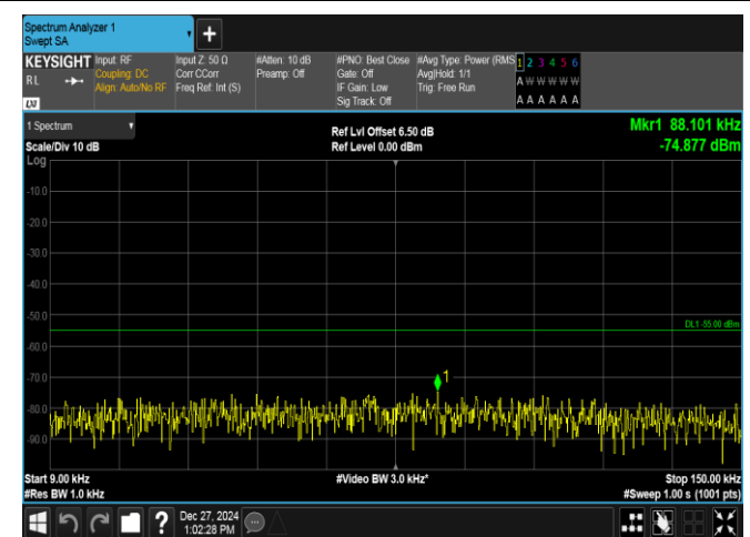
Band7-5MHz-QPSK-21100-25RB#0-0.009~0.15-PASS
