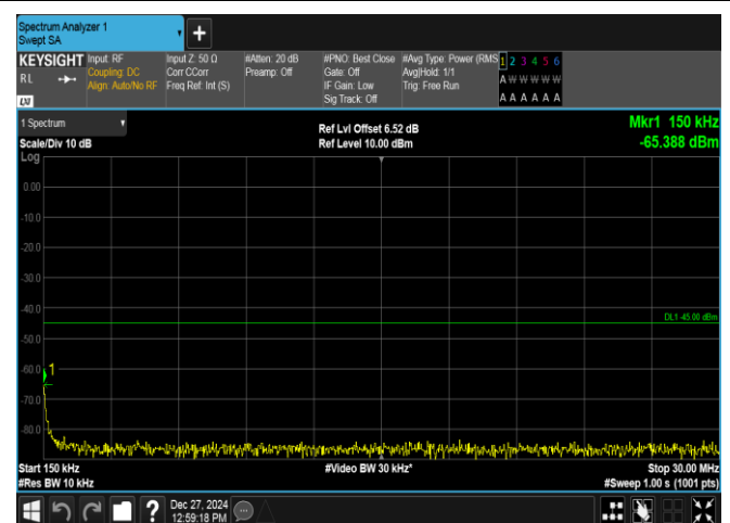
Band7-5MHz-16QAM-21100-1RB#0-0.15~30-PASS
