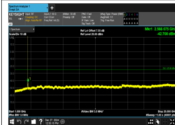
Band7-5MHz-16QAM-20775-1RB#0-1000~20000-PASS
