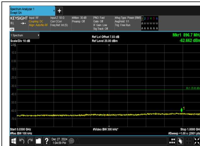
Band7-5MHz-QPSK-21425-1RB#0-30~1000-PASS
