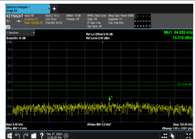
Band7-5MHz-16QAM-20775-25RB#0-0.009~0.15-PASS
