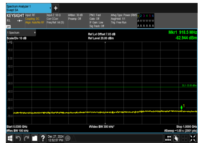
Band7-5MHz-16QAM-20775-1RB#0-30~1000-PASS
