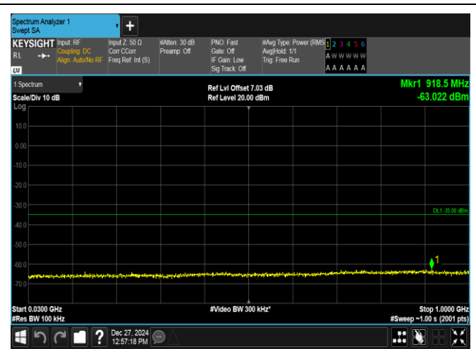
Band7-5MHz-16QAM-20775-25RB#0-30~1000-PASS
