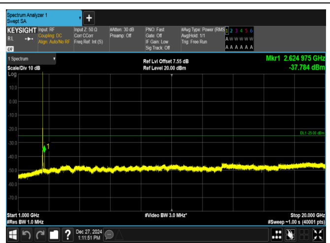
Band7-10MHz-QPSK-20800-1RB#0-1000~20000-PASS
