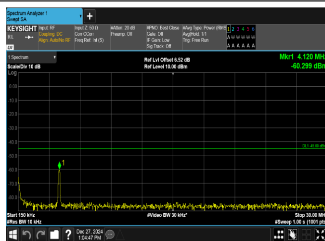
Band7-5MHz-QPSK-21425-1RB#0-0.15~30-PASS
