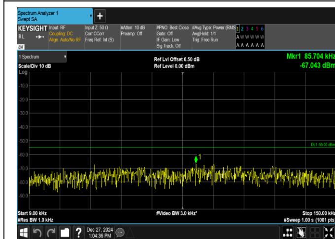
Band7-5MHz-QPSK-21425-1RB#0-0.009~0.15-PASS
