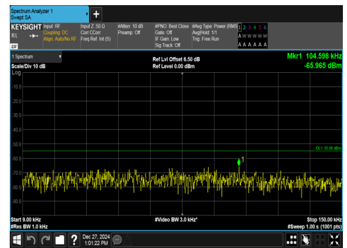
Band7-5MHz-16QAM-21100-1RB#24-0.009~0.15-PASS
