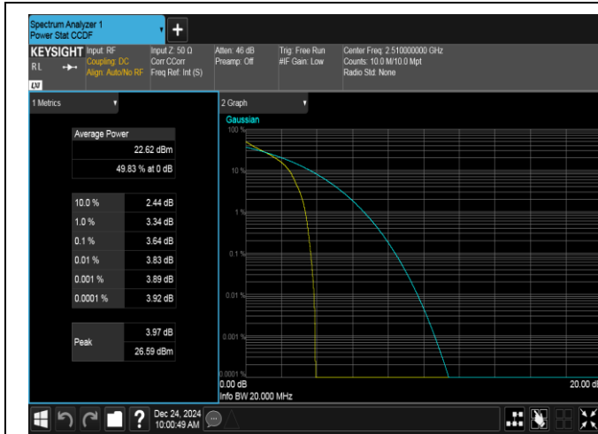
Band7-20MHz-QPSK-20850-1RB#0-PASS
