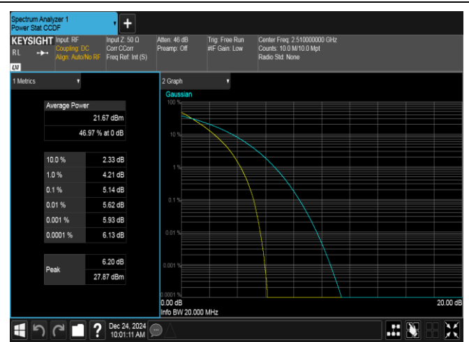
Band7-20MHz-QPSK-20850-100RB#0-PASS
