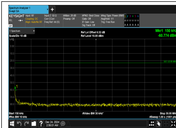
Band5-5MHz-16QAM-20625-25RB#0-0.15~30-PASS
