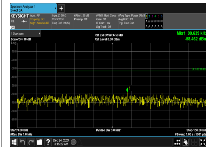
Band5-10MHz-QPSK-20450-50RB#0-0.009~0.15-PASS
