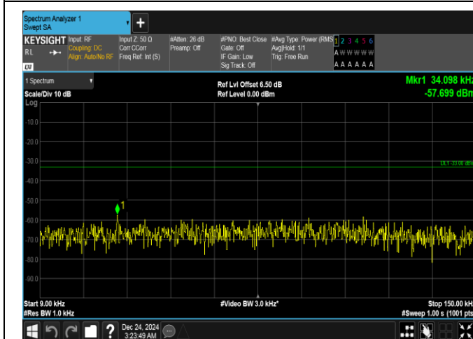
Band5-10MHz-QPSK-20600-1RB#0-0.009~0.15-PASS
