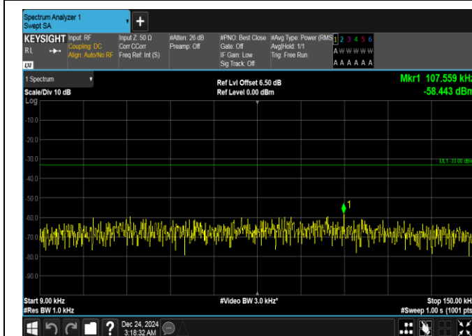
Band5-10MHz-16QAM-20525-1RB#0-0.009~0.15-PASS
