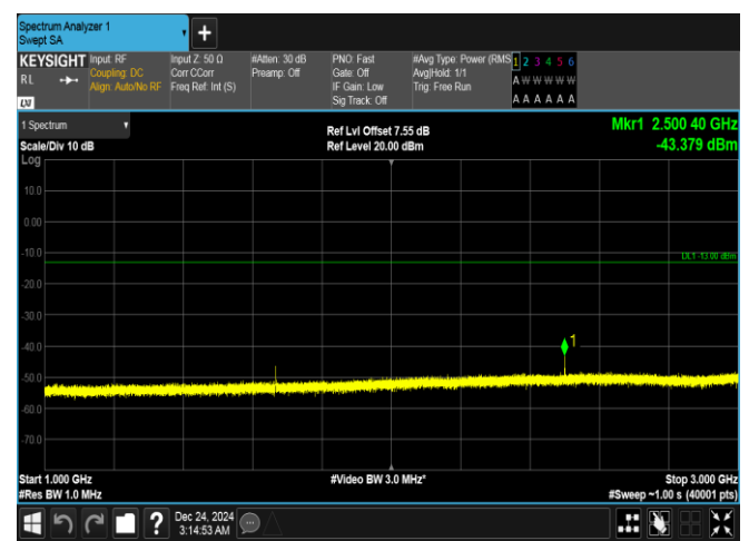
Band5-10MHz-16QAM-20450-1RB#49-1000~3000-PASS
