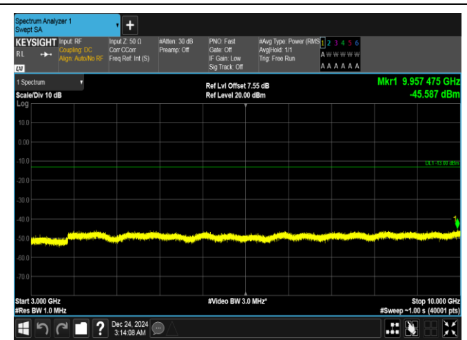
Band5-10MHz-QPSK-20450-1RB#49-3000~10000-PASS
