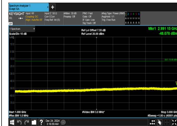
Band5-10MHz-16QAM-20450-50RB#0-1000~3000-PASS
