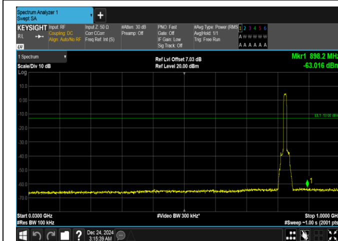
Band5-10MHz-QPSK-20450-50RB#0-30~1000-PASS
