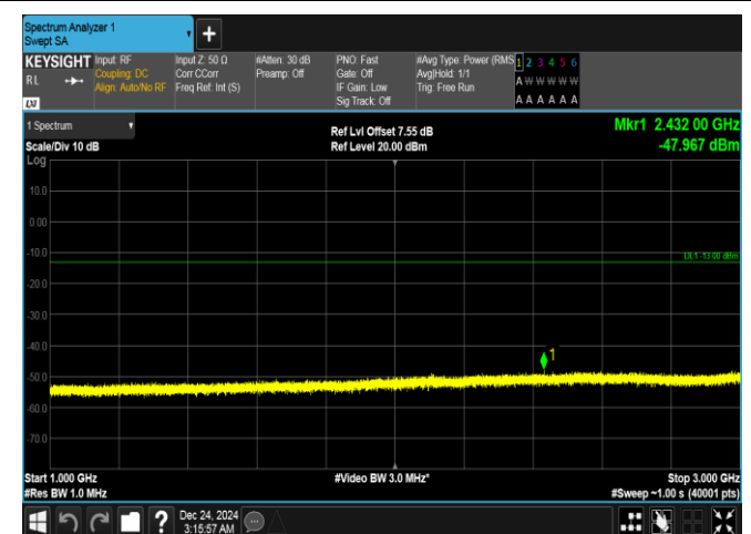
Band5-10MHz-QPSK-20450-50RB#0-1000~3000-PASS
