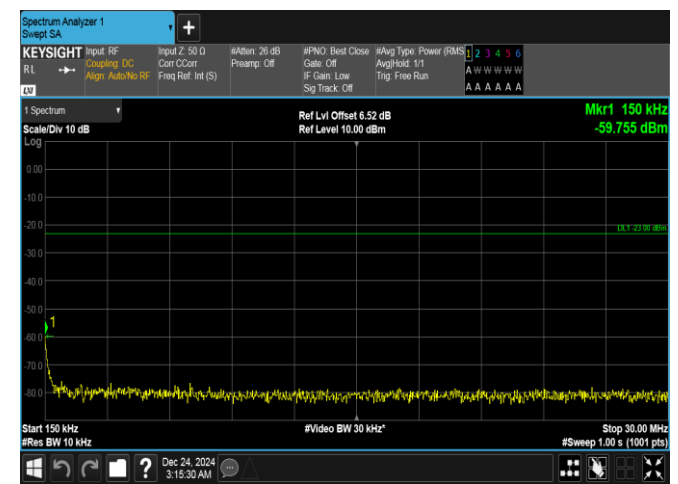
Band5-10MHz-QPSK-20450-50RB#0-0.15~30-PASS
