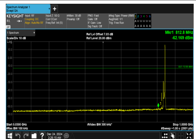
Band5-10MHz-QPSK-20600-1RB#49-30~1000-PASS
