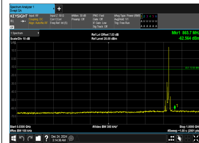
Band5-10MHz-16QAM-20450-1RB#49-30~1000-PASS
