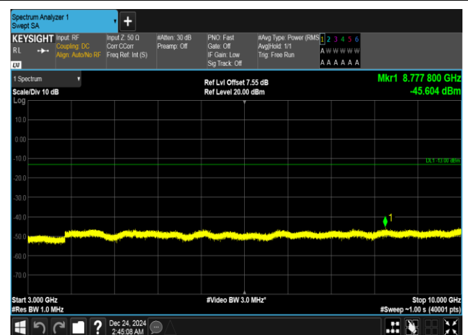
Band5-5MHz-QPSK-20525-1RB#0-3000~10000-PASS
