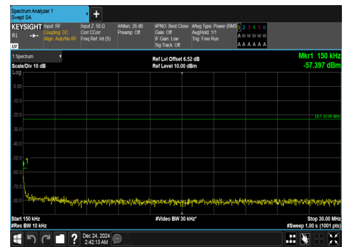
Band5-5MHz-QPSK-20425-25RB#0-0.15~30-PASS
