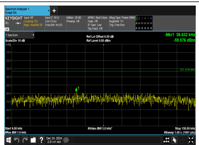
Band5-5MHz-16QAM-20625-1RB#0-0.009~0.15-PASS
