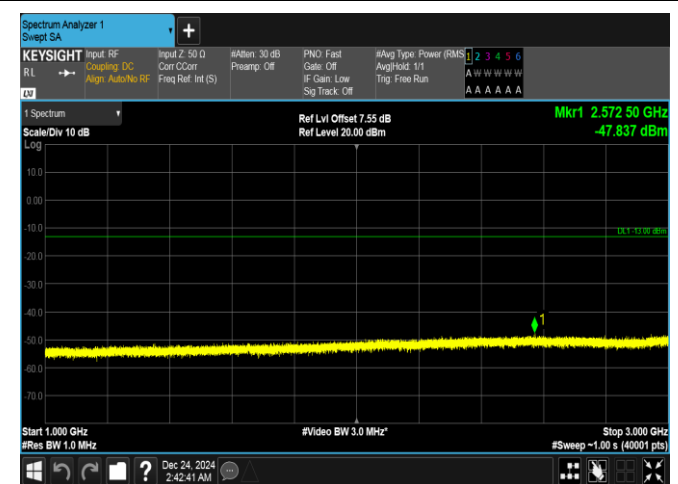
Band5-5MHz-QPSK-20425-25RB#0-1000~3000-PASS
