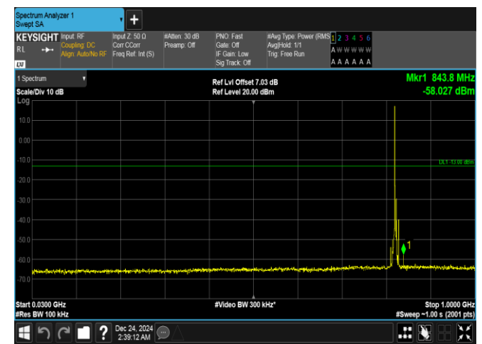
Band5-5MHz-16QAM-20425-1RB#0-30~1000-PASS
