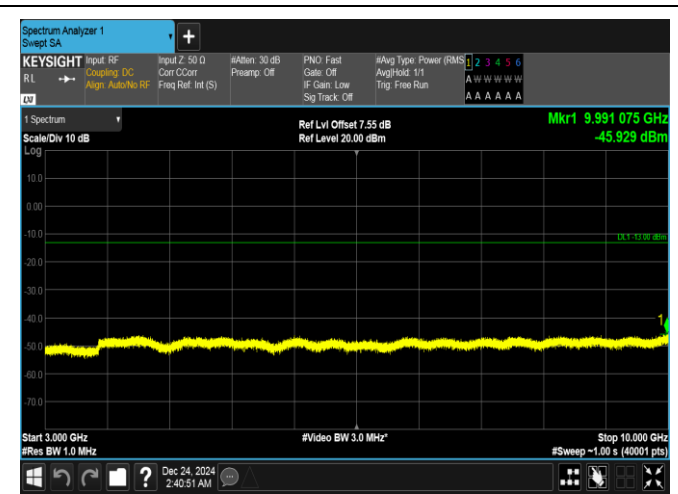
Band5-5MHz-QPSK-20425-1RB#24-3000~10000-PASS
