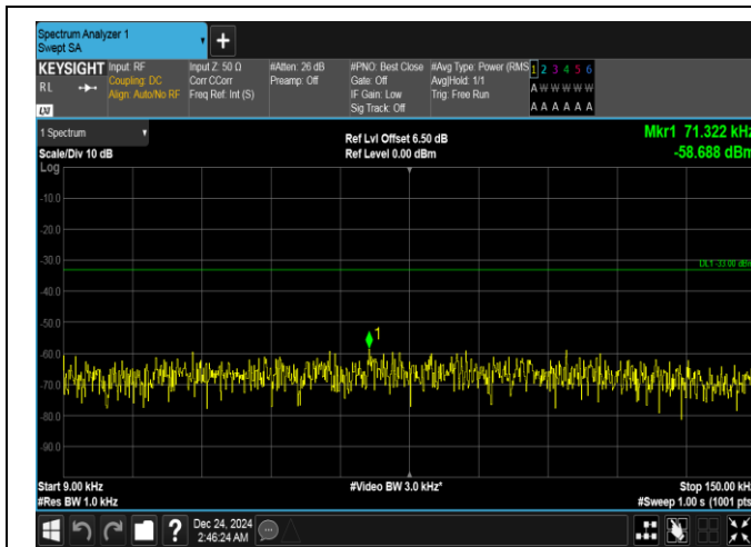
Band5-5MHz-QPSK-20525-1RB#24-0.009~0.15-PASS
