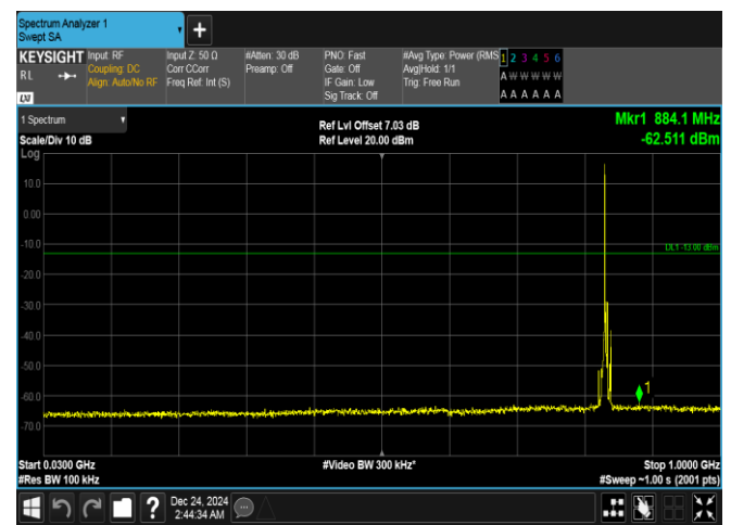
Band5-5MHz-QPSK-20525-1RB#0-30~1000-PASS
