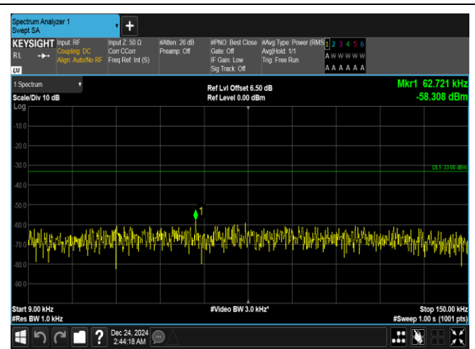
Band5-5MHz-QPSK-20525-1RB#0-0.009~0.15-PASS
