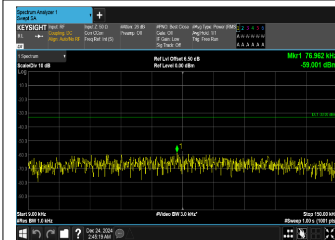
Band5-5MHz-16QAM-20525-1RB#0-0.009~0.15-PASS
