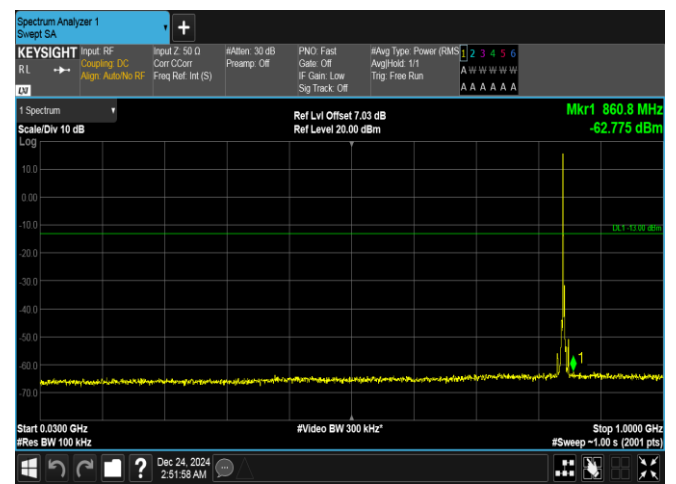
Band5-5MHz-16QAM-20625-1RB#0-30~1000-PASS
