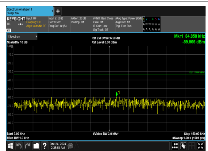
Band5-5MHz-16QAM-20425-1RB#0-0.009~0.15-PASS
