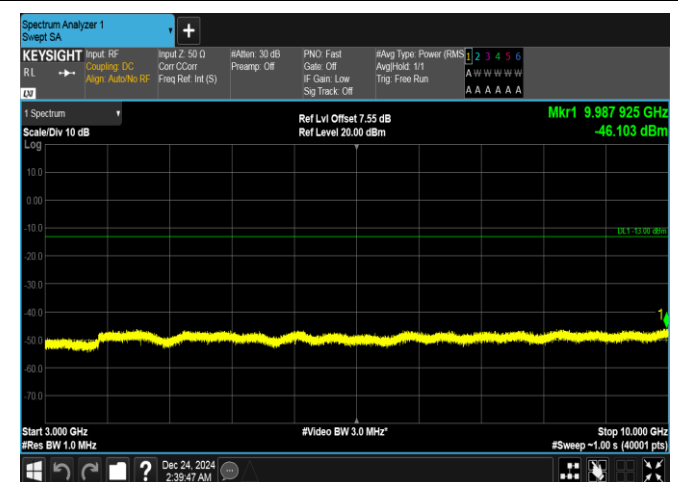
Band5-5MHz-16QAM-20425-1RB#0-3000~10000-PASS
