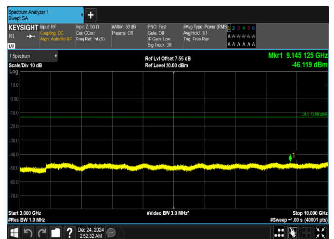
Band5-5MHz-16QAM-20625-1RB#0-3000~10000-PASS
