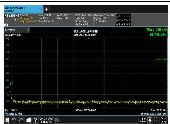
Band5-5MHz-QPSK-20525-1RB#24-0.15~30-PASS
