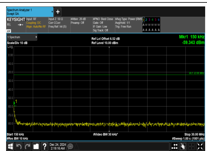
Band5-3MHz-16QAM-20635-1RB#14-0.15~30-PASS
