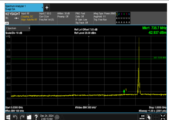
Band5-5MHz-QPSK-20425-1RB#24-30~1000-PASS
