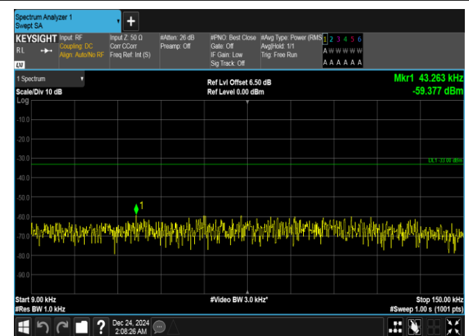
Band5-3MHz-16QAM-20415-15RB#0-0.009~0.15-PASS
