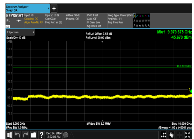
Band5-3MHz-16QAM-20635-15RB#0-3000~10000-PASS
