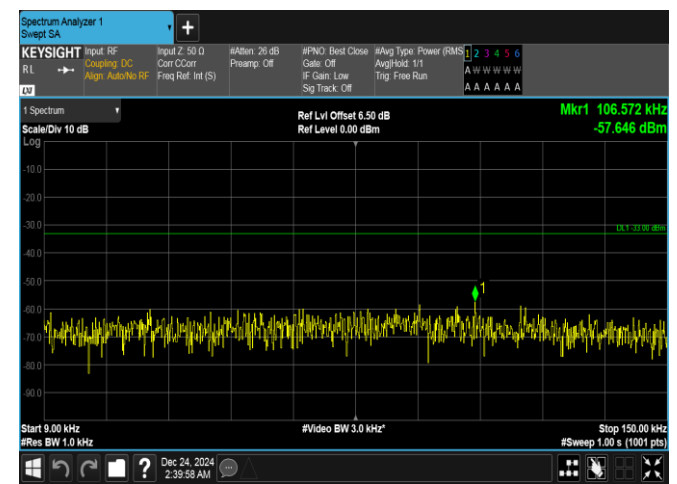
Band5-5MHz-QPSK-20425-1RB#24-0.009~0.15-PASS
