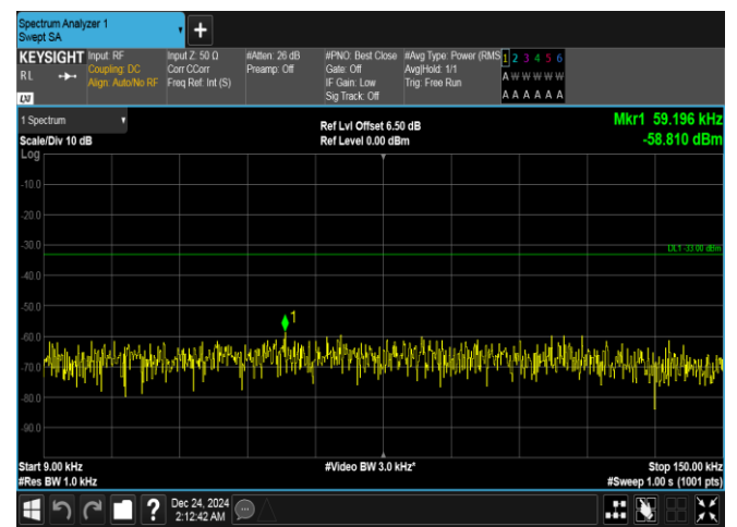
Band5-3MHz-16QAM-20525-1RB#14-0.009~0.15-PASS
