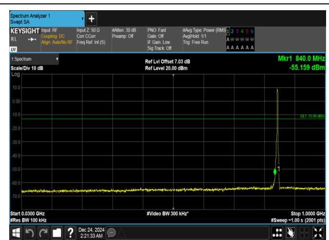
Band5-3MHz-16QAM-20635-15RB#0-30~1000-PASS
