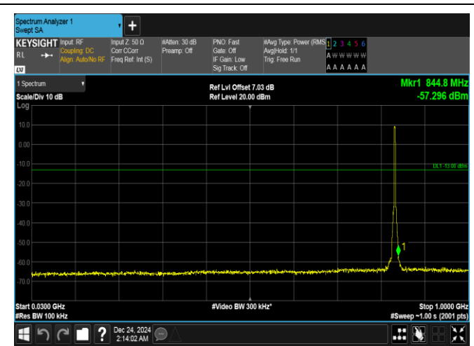
Band5-3MHz-QPSK-20525-15RB#0-30~1000-PASS
