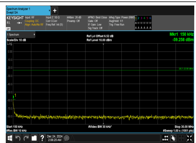
Band5-3MHz-16QAM-20415-1RB#14-0.15~30-PASS
