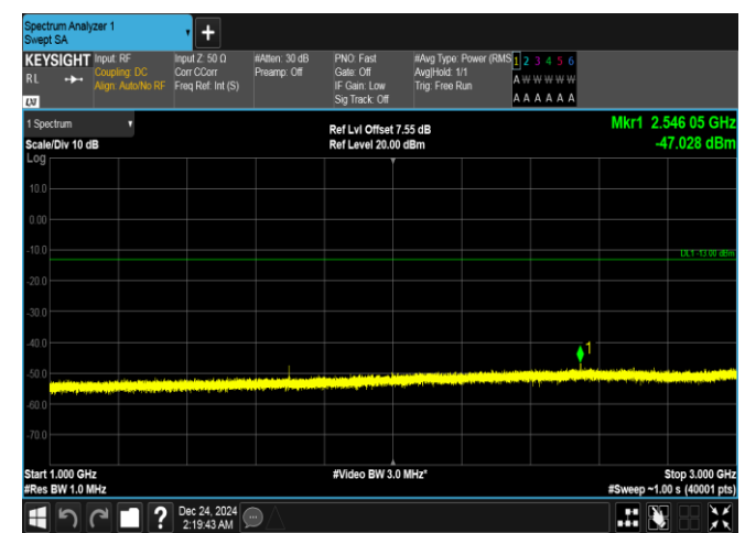
Band5-3MHz-16QAM-20635-1RB#14-1000~3000-PASS
