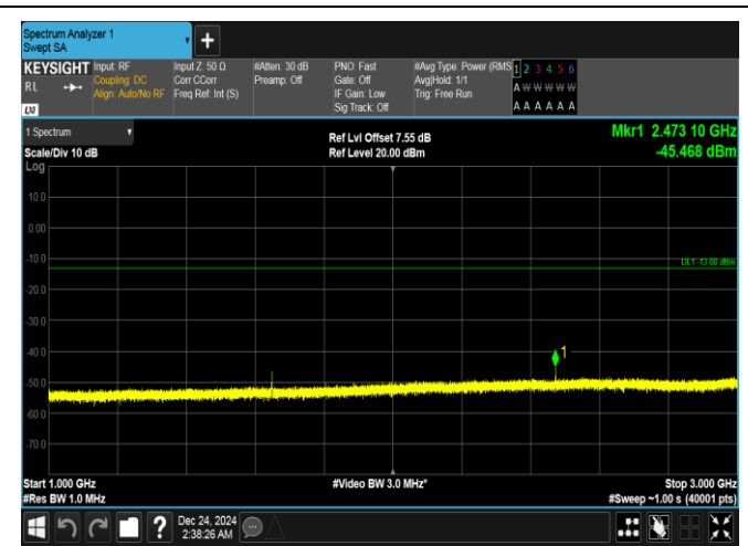
Band5-5MHz-QPSK-20425-1RB#0-1000~3000-PASS
