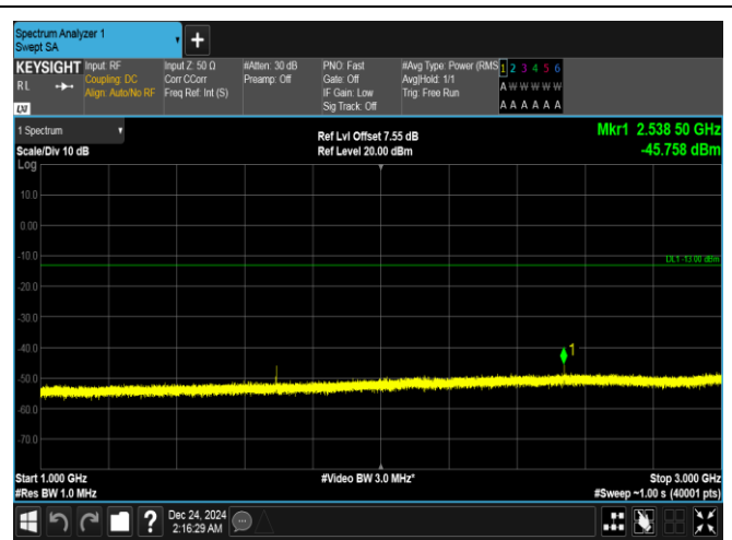
Band5-3MHz-QPSK-20635-1RB#0-1000~3000-PASS
