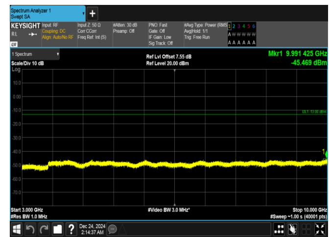
Band5-3MHz-QPSK-20525-15RB#0-3000~10000-PASS
