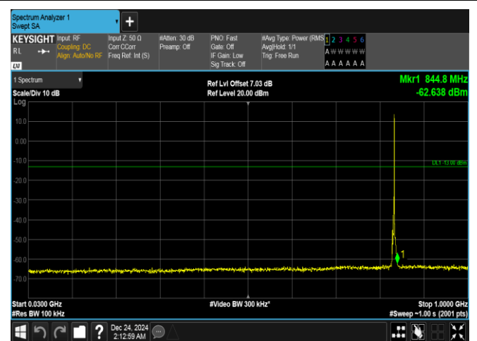
Band5-3MHz-16QAM-20525-1RB#14-30~1000-PASS
