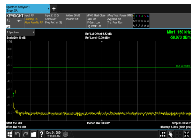
Band5-3MHz-QPSK-20635-1RB#0-0.15~30-PASS
