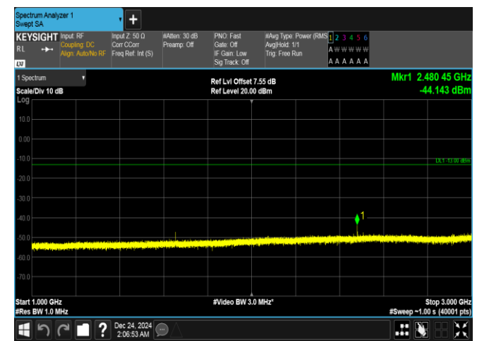
Band5-3MHz-16QAM-20415-1RB#14-1000~3000-PASS
