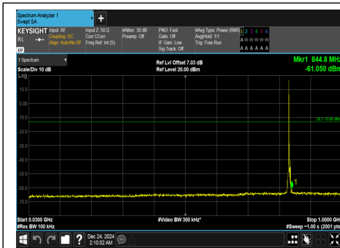
Band5-3MHz-16QAM-20525-1RB#0-30~1000-PASS
