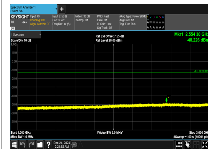
Band5-3MHz-16QAM-20635-15RB#0-1000~3000-PASS
