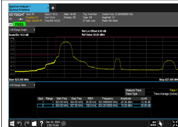
Band5-3MHz-16QAM-20415-1RB#0-PASS
