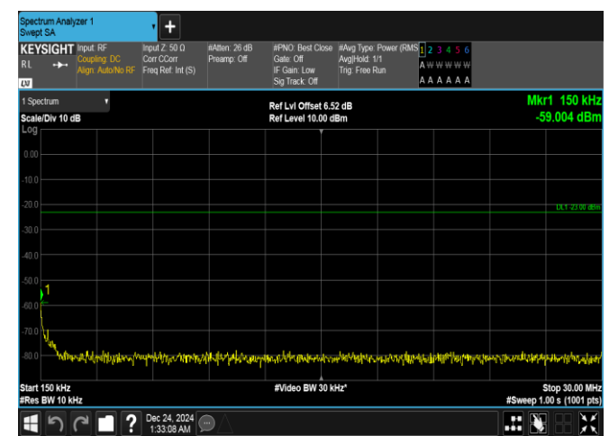
Band5-1.4MHz-QPSK-20407-6RB#0-0.15~30-PASS
