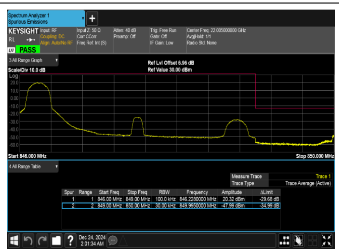
Band5-3MHz-QPSK-20635-1RB#0-PASS
