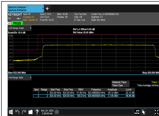
Band5-5MHz-16QAM-20425-25RB#0-PASS
