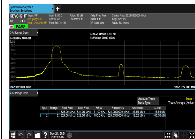
Band5-5MHz-16QAM-20425-1RB#0-PASS
