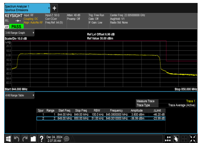
Band5-5MHz-16QAM-20625-25RB#0-PASS
