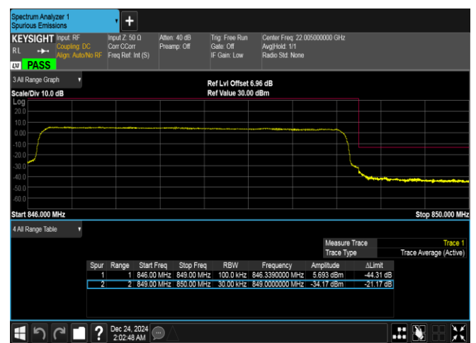
Band5-3MHz-16QAM-20635-15RB#0-PASS
