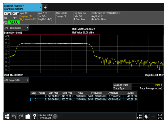
Band5-1.4MHz-16QAM-20643-6RB#0-PASS
