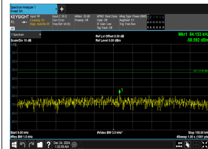
Band5-1.4MHz-QPSK-20407-6RB#0-0.009~0.15-PASS
