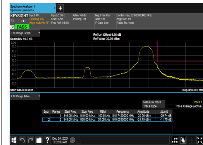
Band5-3MHz-QPSK-20635-1RB#14-PASS
