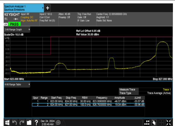
Band5-3MHz-16QAM-20415-1RB#14-PASS
