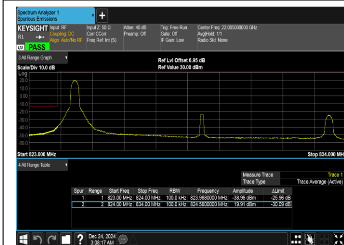
Band5-10MHz-QPSK-20450-1RB#0-PASS
