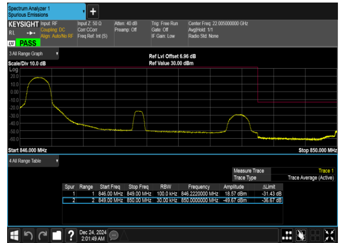
Band5-3MHz-16QAM-20635-1RB#0-PASS
