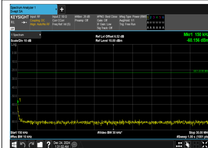
Band5-1.4MHz-QPSK-20407-1RB#5-0.15~30-PASS
