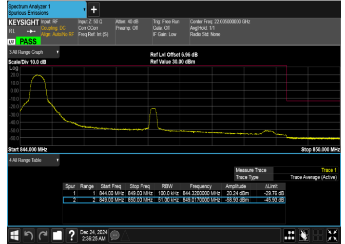
Band5-5MHz-QPSK-20625-1RB#0-PASS
