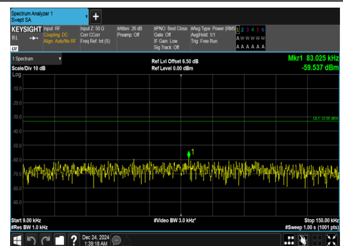
Band5-1.4MHz-QPSK-20525-6RB#0-0.009~0.15-PASS
