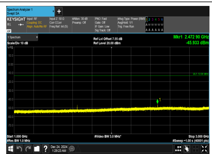
Band5-1.4MHz-QPSK-20407-1RB#0-1000~3000-PASS
