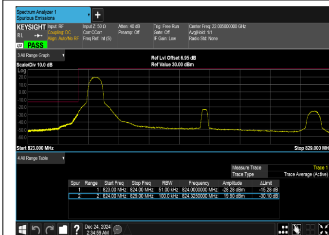
Band5-5MHz-QPSK-20425-1RB#0-PASS
