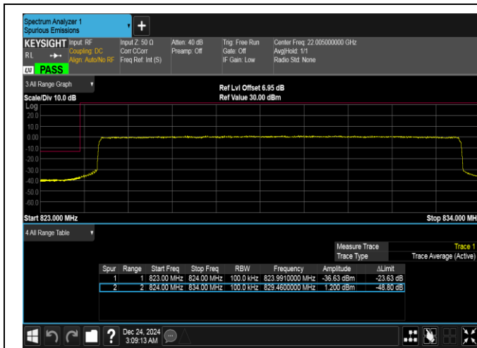
Band5-10MHz-QPSK-20450-50RB#0-PASS
