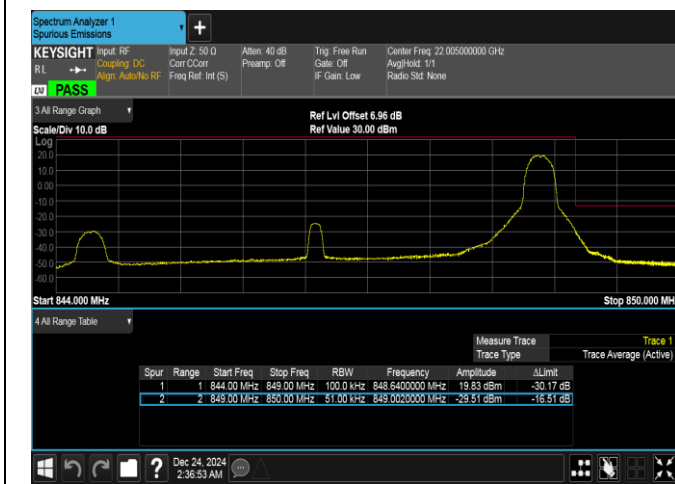
Band5-5MHz-QPSK-20625-1RB#24-PASS
