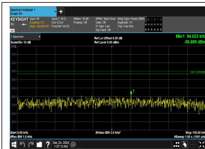
Band5-1.4MHz-QPSK-20525-1RB#5-0.009~0.15-PASS
