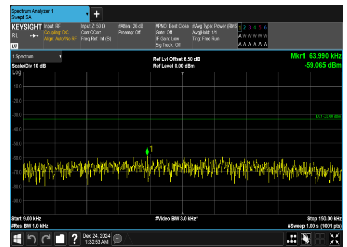
Band5-1.4MHz-QPSK-20407-1RB#5-0.009~0.15-PASS
