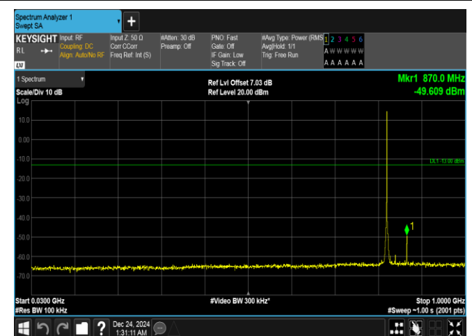
Band5-1.4MHz-QPSK-20407-1RB#5-30~1000-PASS
