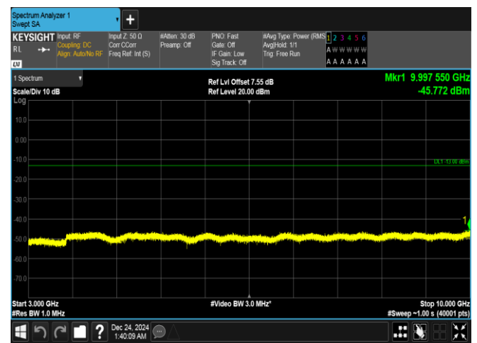
Band5-1.4MHz-QPSK-20525-6RB#0-3000~10000-PASS
