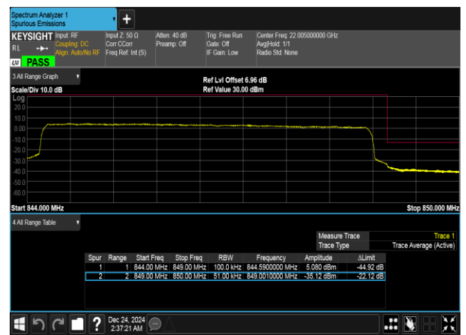
Band5-5MHz-QPSK-20625-25RB#0-PASS
