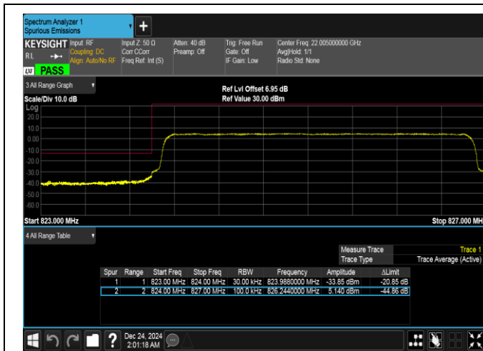
Band5-3MHz-16QAM-20415-15RB#0-PASS
