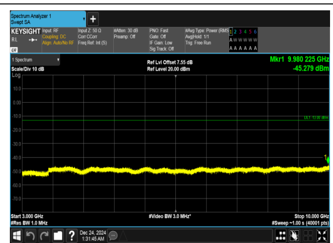
Band5-1.4MHz-QPSK-20407-1RB#5-3000~10000-PASS
