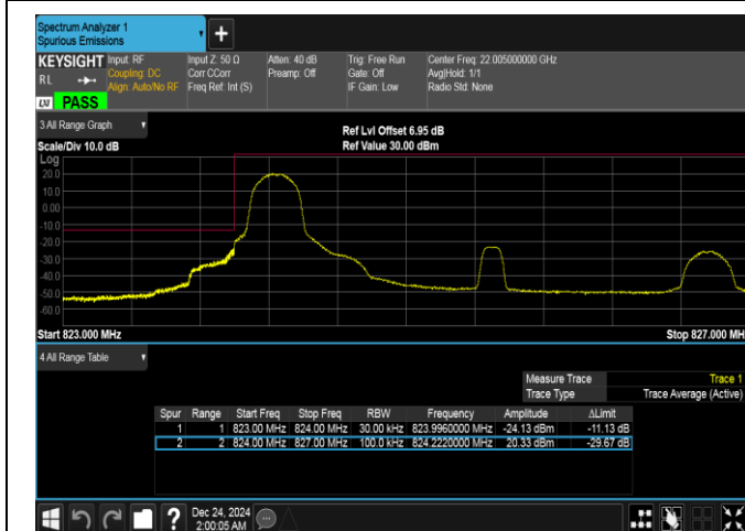
Band5-3MHz-QPSK-20415-1RB#0-PASS
