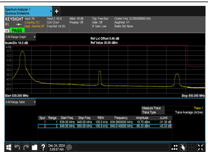
Band5-10MHz-16QAM-20600-1RB#0-PASS
