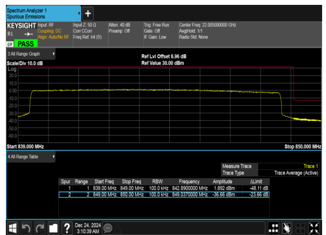
Band5-10MHz-QPSK-20600-50RB#0-PASS
