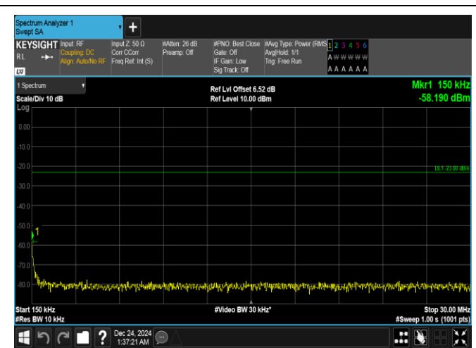
Band5-1.4MHz-QPSK-20525-1RB#5-0.15~30-PASS
