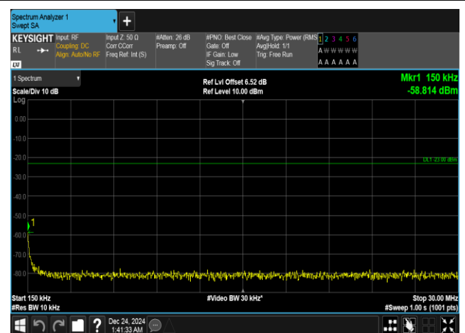
Band5-1.4MHz-QPSK-20643-1RB#0-0.15~30-PASS
