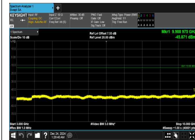
Band5-1.4MHz-QPSK-20407-1RB#0-3000~10000-PASS
