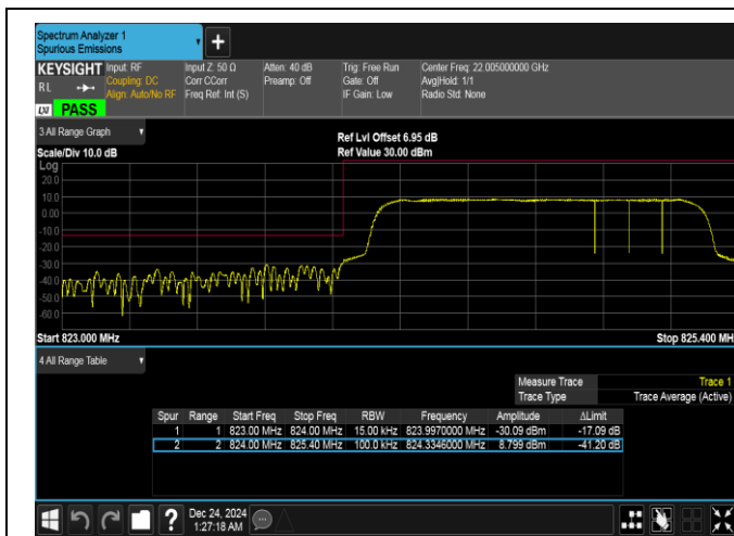
Band5-1.4MHz-16QAM-20407-6RB#0-PASS
