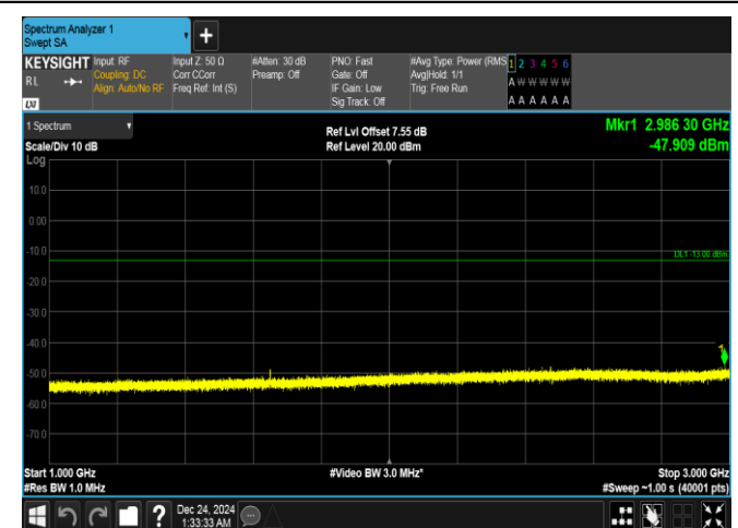
Band5-1.4MHz-QPSK-20407-6RB#0-1000~3000-PASS
