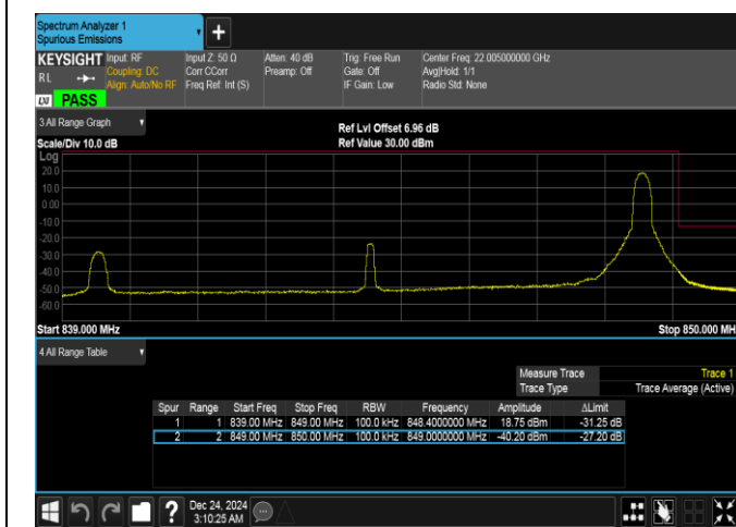
Band5-10MHz-16QAM-20600-1RB#49-PASS
