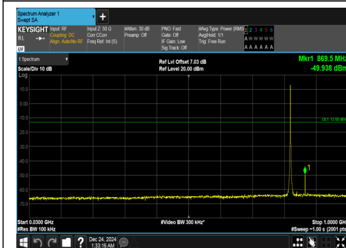
Band5-1.4MHz-QPSK-20407-6RB#0-30~1000-PASS
