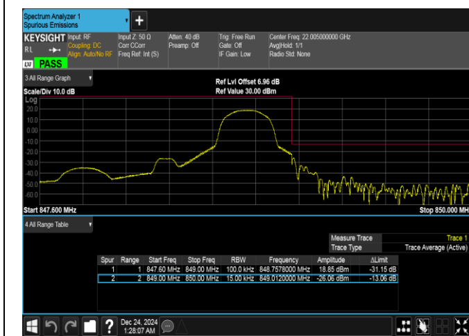
Band5-1.4MHz-16QAM-20643-1RB#5-PASS
