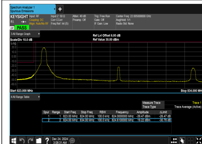
Band5-10MHz-16QAM-20450-1RB#0-PASS
