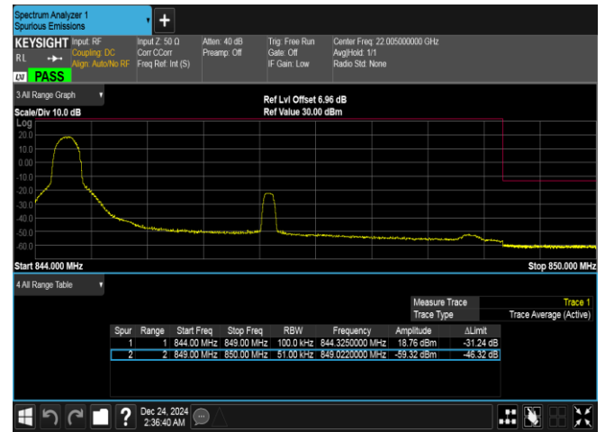
Band5-5MHz-16QAM-20625-1RB#0-PASS
