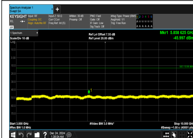
Band5-1.4MHz-QPSK-20525-1RB#5-3000~10000-PASS
