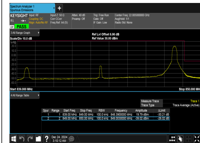
Band5-10MHz-QPSK-20600-1RB#49-PASS
