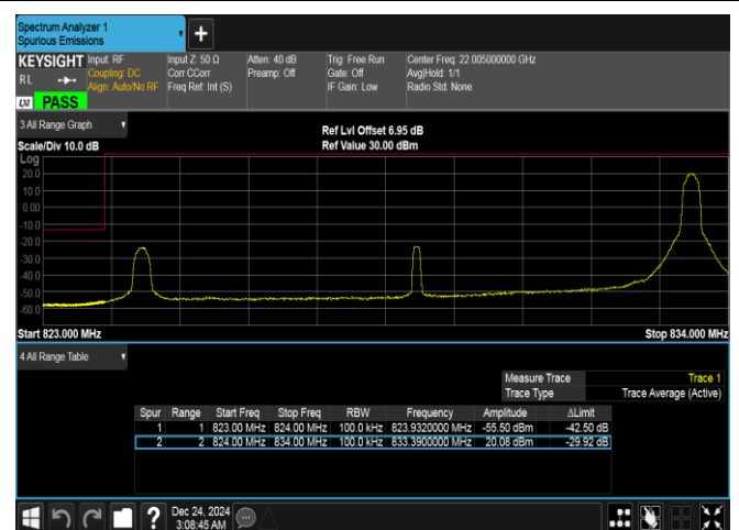
Band5-10MHz-QPSK-20450-1RB#49-PASS
