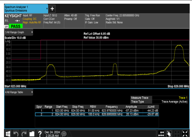
Band5-5MHz-QPSK-20425-1RB#24-PASS
