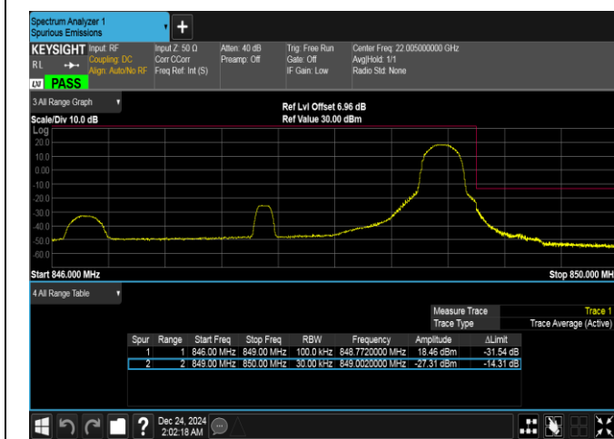
Band5-3MHz-16QAM-20635-1RB#14-PASS
