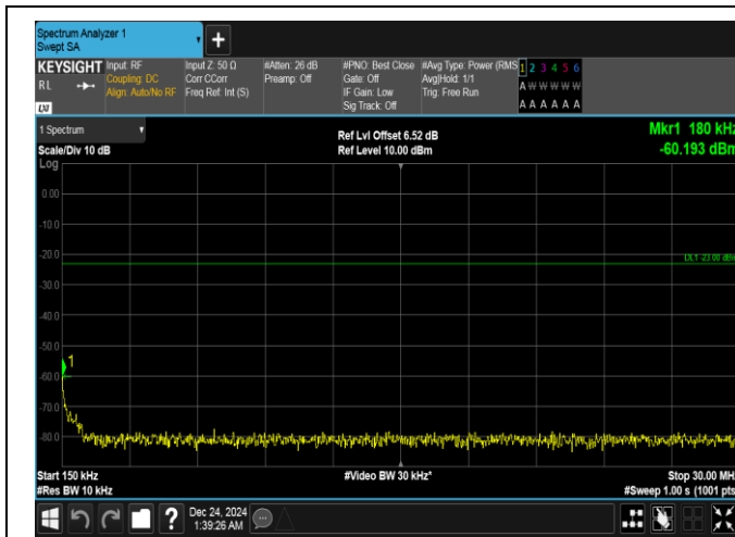
Band5-1.4MHz-QPSK-20525-6RB#0-0.15~30-PASS
