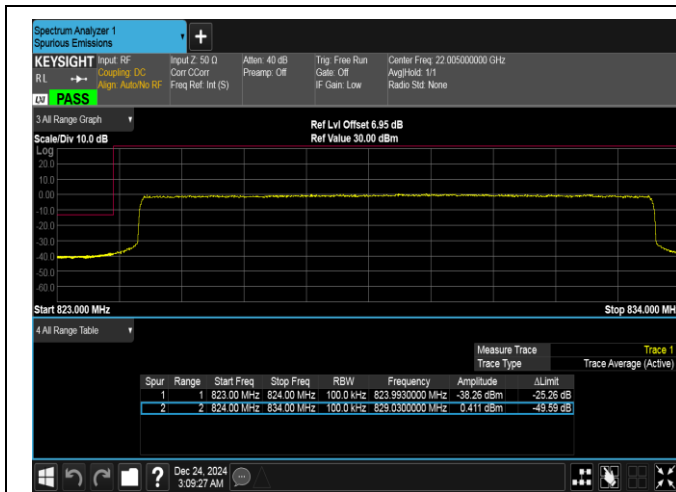
Band5-10MHz-16QAM-20450-50RB#0-PASS
