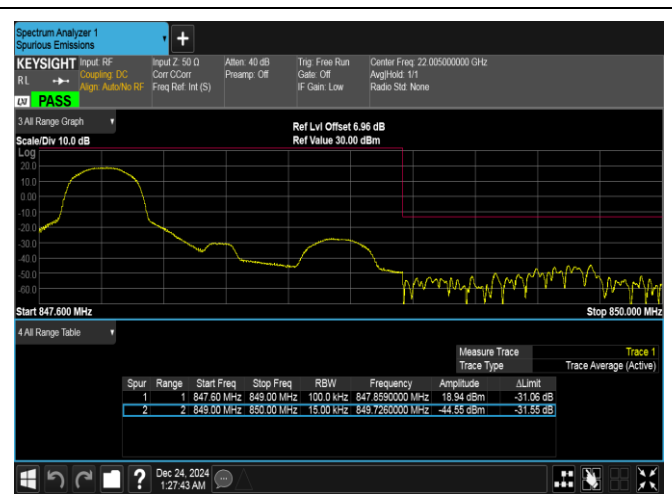
Band5-1.4MHz-16QAM-20643-1RB#0-PASS
