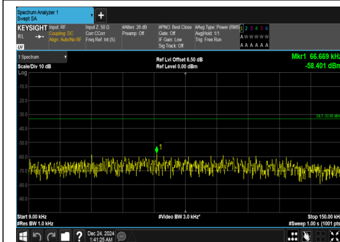
Band5-1.4MHz-QPSK-20643-1RB#0-0.009~0.15-PASS
