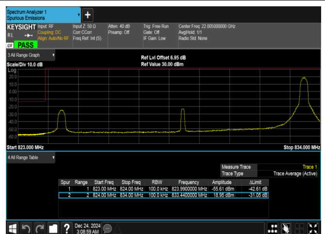
Band5-10MHz-16QAM-20450-1RB#49-PASS
