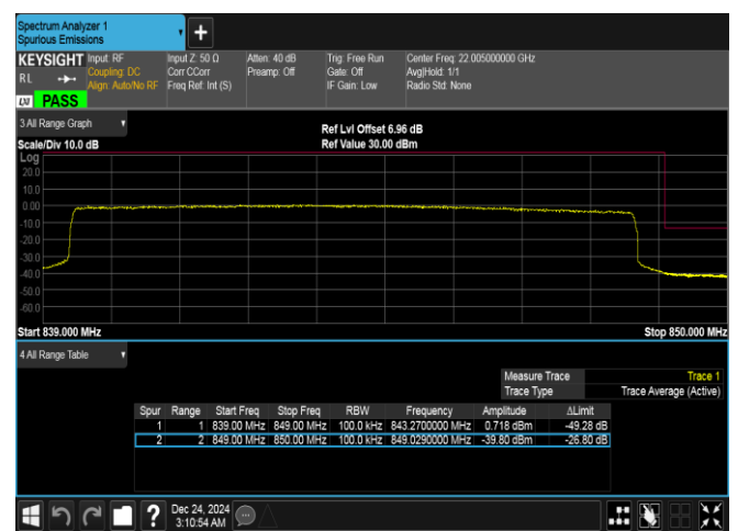
Band5-10MHz-16QAM-20600-50RB#0-PASS
