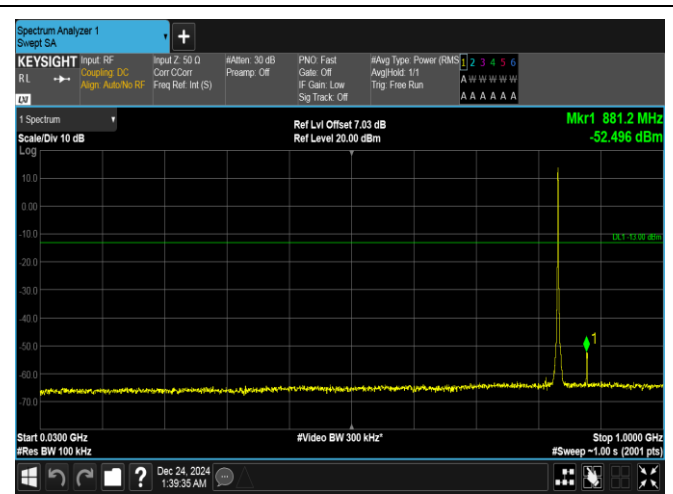
Band5-1.4MHz-QPSK-20525-6RB#0-30~1000-PASS
