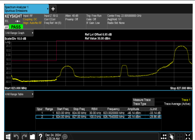
Band5-3MHz-QPSK-20415-1RB#14-PASS
