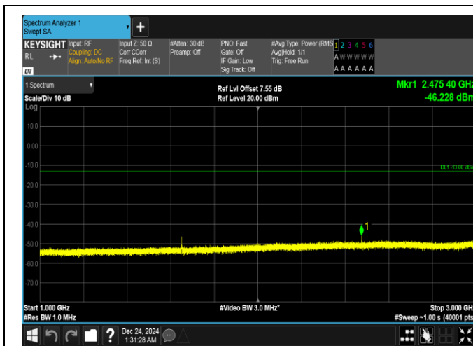
Band5-1.4MHz-QPSK-20407-1RB#5-1000~3000-PASS
