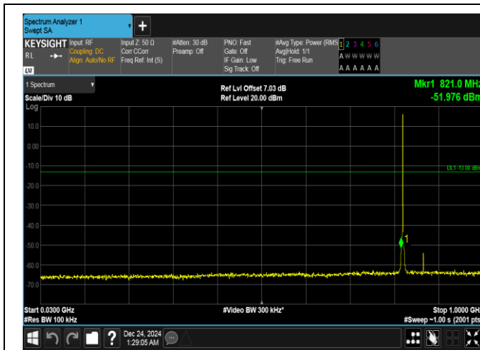
Band5-1.4MHz-QPSK-20407-1RB#0-30~1000-PASS
