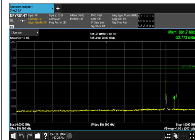
Band5-1.4MHz-QPSK-20525-1RB#5-30~1000-PASS
