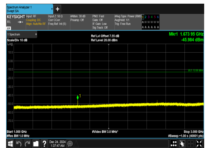
Band5-1.4MHz-QPSK-20525-1RB#5-1000~3000-PASS
