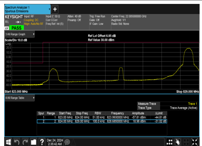
Band5-5MHz-16QAM-20425-1RB#24-PASS
