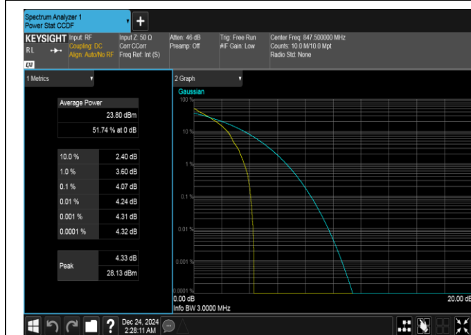
Band5-3MHz-QPSK-20635-1RB#0-PASS
