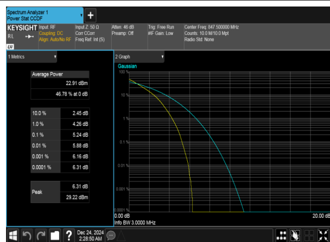
Band5-3MHz-QPSK-20635-15RB#0-PASS
