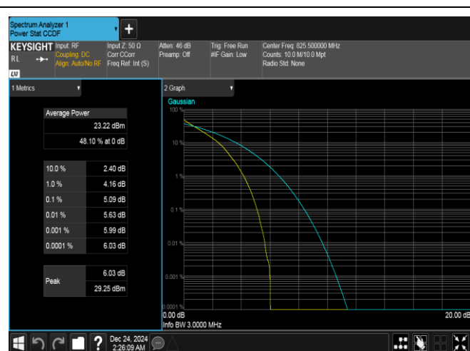
Band5-3MHz-QPSK-20415-15RB#0-PASS
