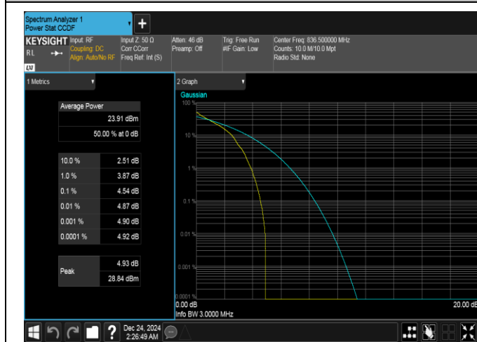
Band5-3MHz-QPSK-20525-1RB#0-PASS
