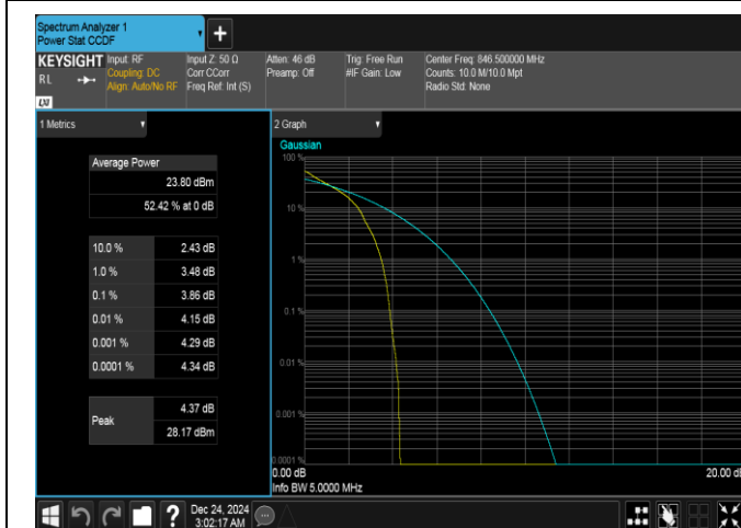
Band5-5MHz-QPSK-20625-1RB#0-PASS
