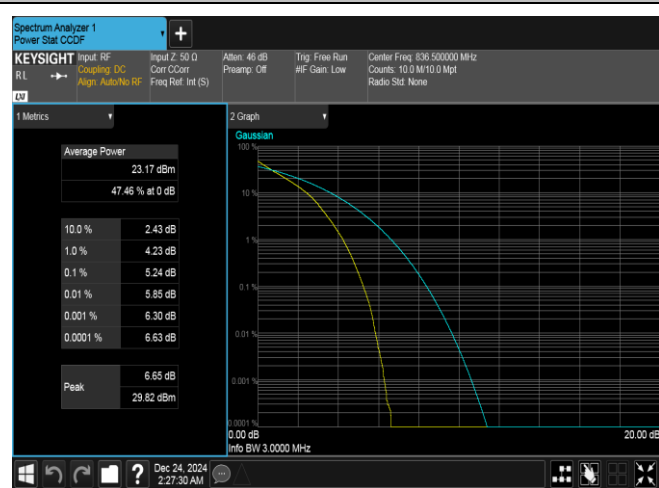
Band5-3MHz-QPSK-20525-15RB#0-PASS
