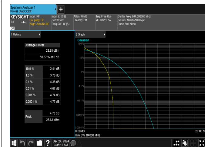
Band5-10MHz-QPSK-20600-1RB#0-PASS
