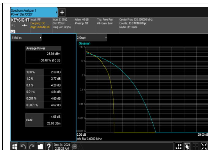
Band5-3MHz-QPSK-20415-1RB#0-PASS
