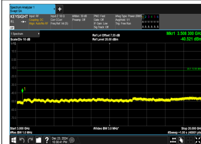
Band4-20MHz-16QAM-20300-1RB#99-3000~20000-PASS
