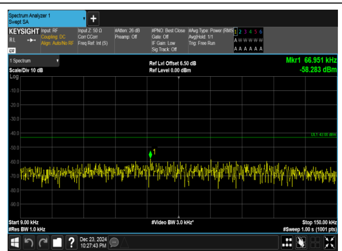
Band4-20MHz-16QAM-20300-1RB#0-0.009~0.15-PASS
