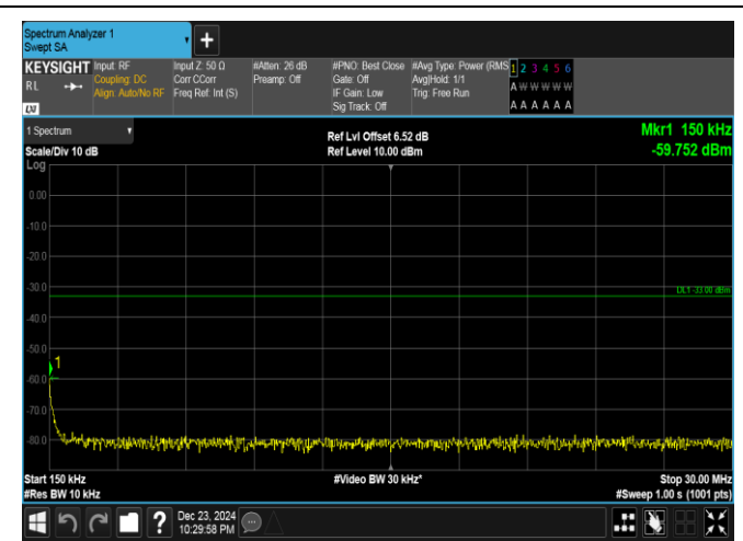
Band4-20MHz-16QAM-20300-1RB#99-0.15~30-PASS
