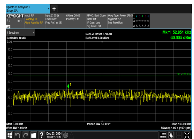
Band4-20MHz-16QAM-20300-100RB#0-0.009~0.15-PASS
