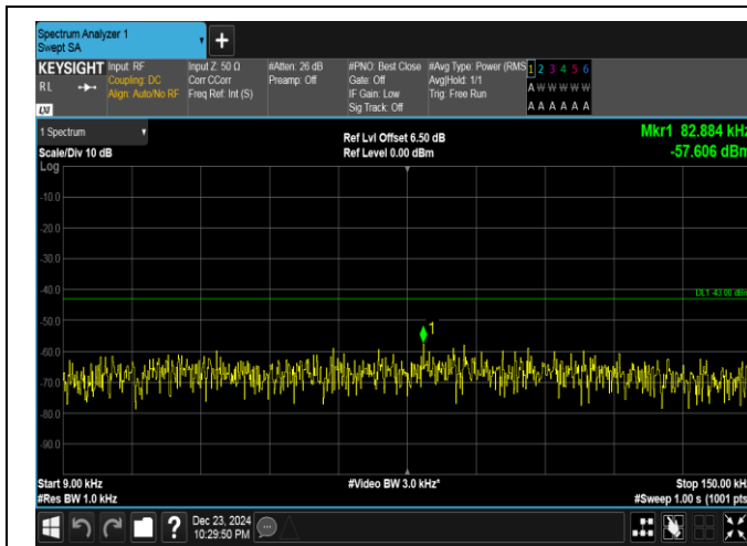
Band4-20MHz-16QAM-20300-1RB#99-0.009~0.15-PASS
