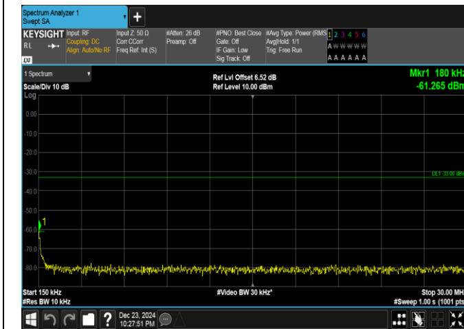
Band4-20MHz-16QAM-20300-1RB#0-0.15~30-PASS
