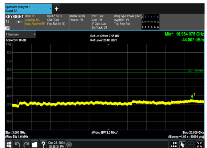
Band4-20MHz-16QAM-20300-1RB#0-3000~20000-PASS
