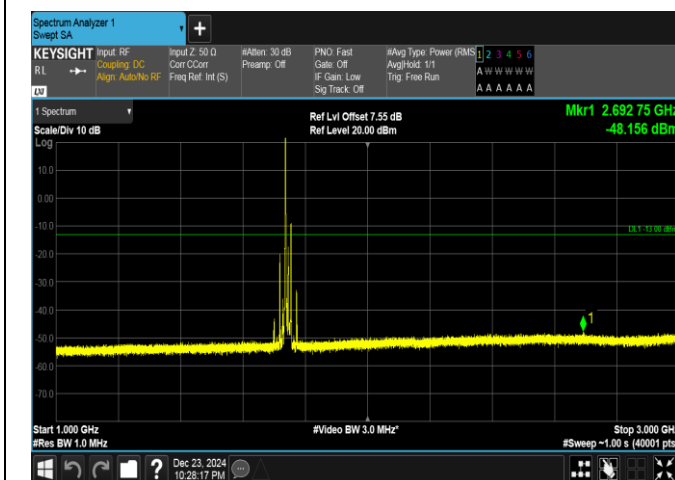
Band4-20MHz-16QAM-20300-1RB#0-1000~3000-PASS
