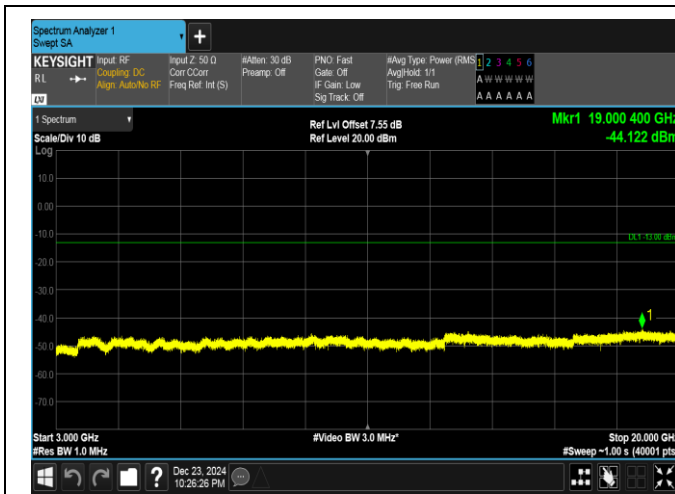
Band4-20MHz-16QAM-20175-100RB#0-3000~20000-PAS S
