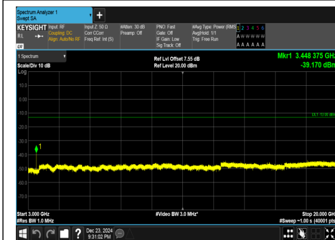
Band4-15MHz-16QAM-2025-1RB#74-3000~20000-PASS
