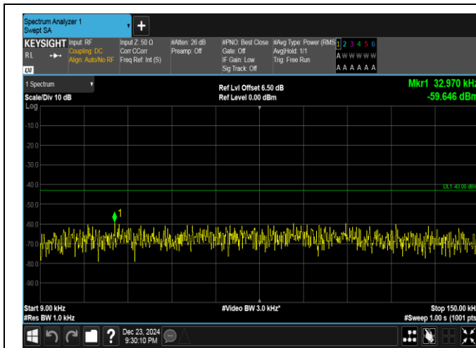
Band4-15MHz-16QAM-2025-1RB#74-0.009~0.15-PASS
