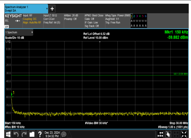
Band4-15MHz-16QAM-20175-1RB#0-0.15~30-PASS
