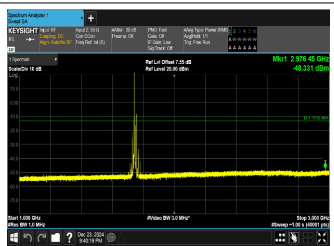
Band4-15MHz-QPSK-20325-1RB#0-1000~3000-PASS
