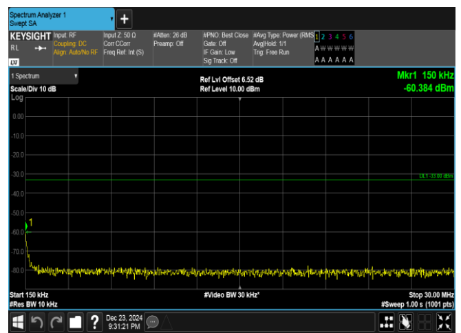
Band4-15MHz-QPSK-2025-75RB#0-0.15~30-PASS
