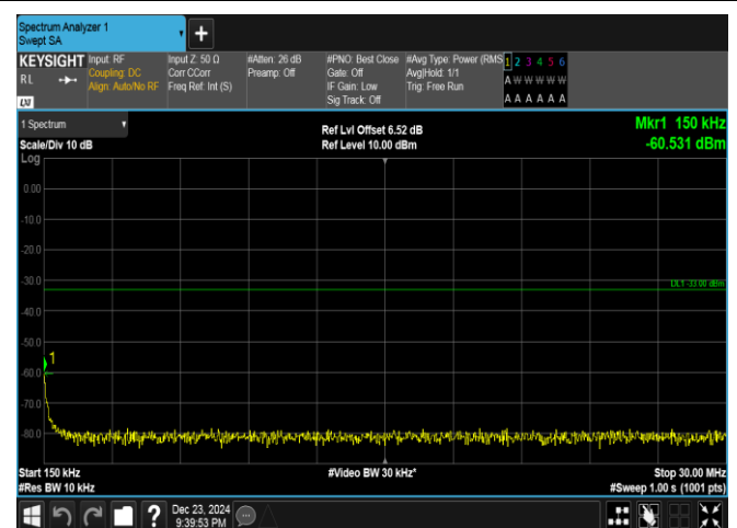
Band4-15MHz-QPSK-20325-1RB#0-0.15~30-PASS
