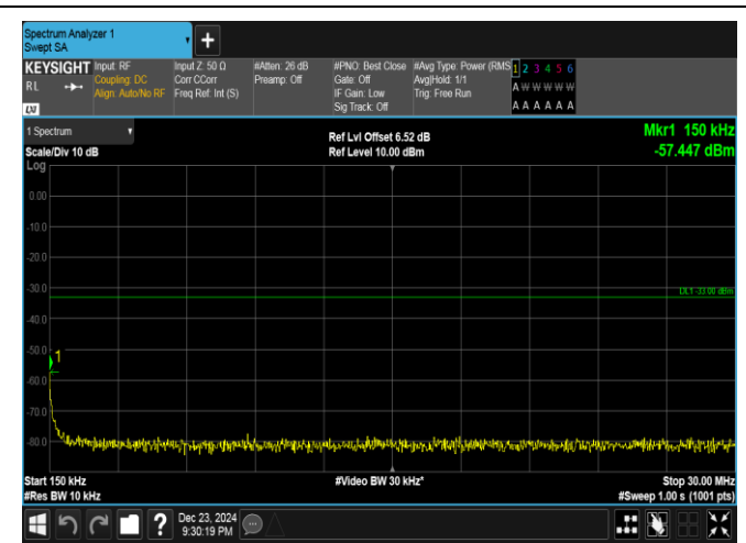
Band4-15MHz-16QAM-2025-1RB#74-0.15~30-PASS
