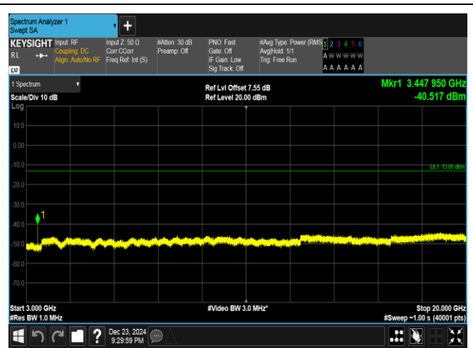
Band4-15MHz-QPSK-2025-1RB#74-3000~20000-PASS
