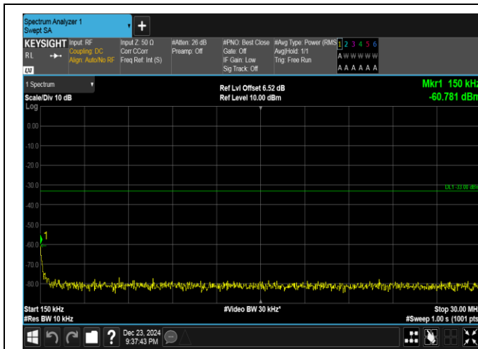
Band4-15MHz-QPSK-20175-75RB#0-0.15~30-PASS
