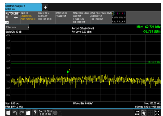
Band4-15MHz-16QAM-2025-75RB#0-0.009~0.15-PASS
