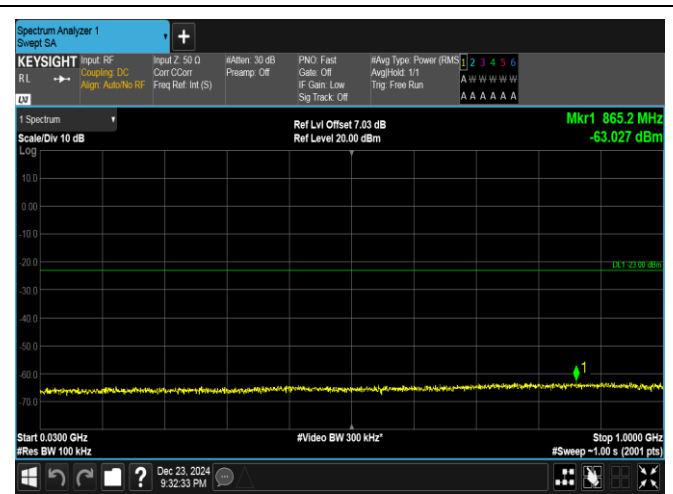
Band4-15MHz-16QAM-20025-75RB#0-30~1000-PASS
