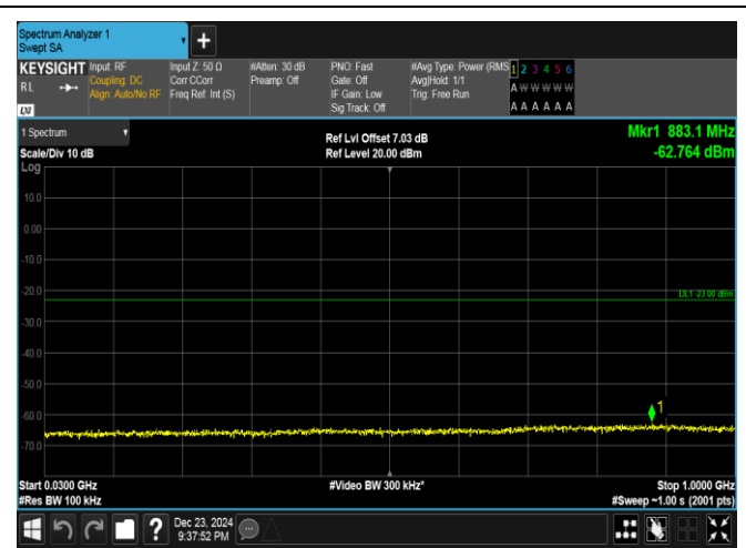
Band4-15MHz-QPSK-20175-75RB#0-30~1000-PASS
