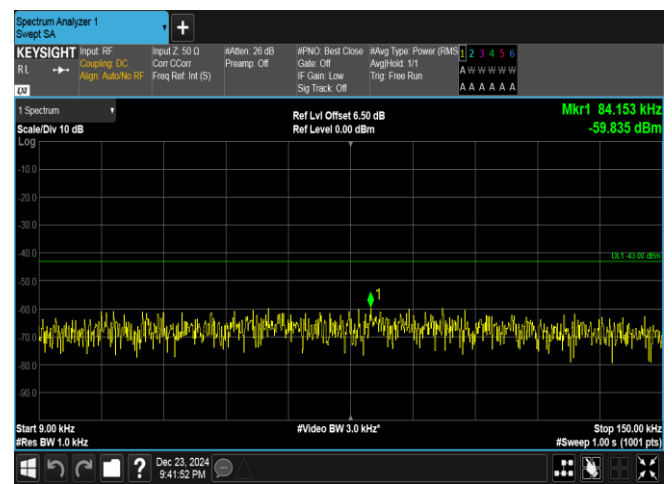
Band4-15MHz-QPSK-20325-1RB#74-0.009~0.15-PASS
