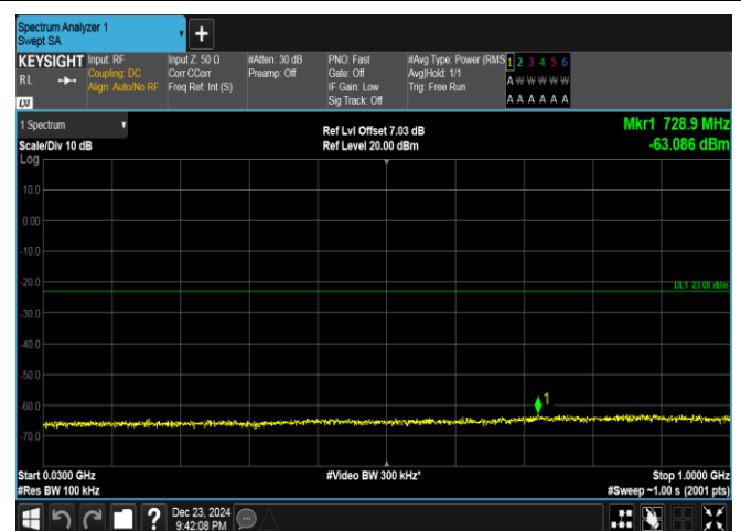
Band4-15MHz-QPSK-20325-1RB#74-30~1000-PASS
