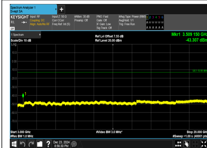
Band4-10MHz-16QAM-20350-1RB#49-3000~20000-PASS
