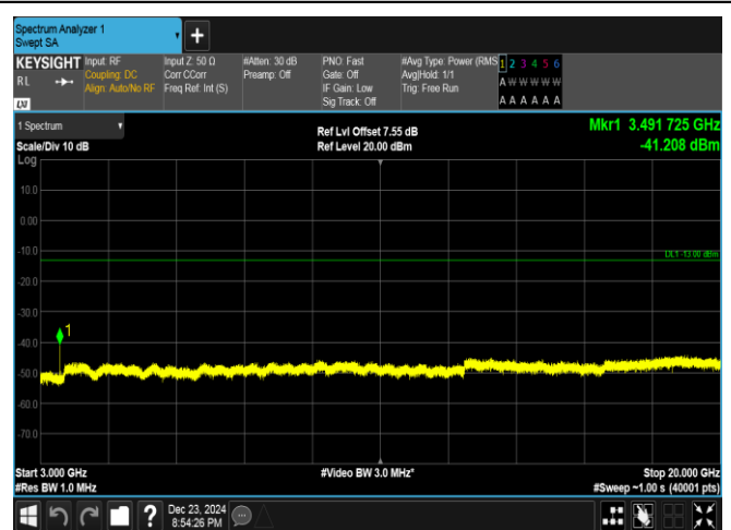
Band4-10MHz-16QAM-20350-1RB#0-3000~20000-PASS
