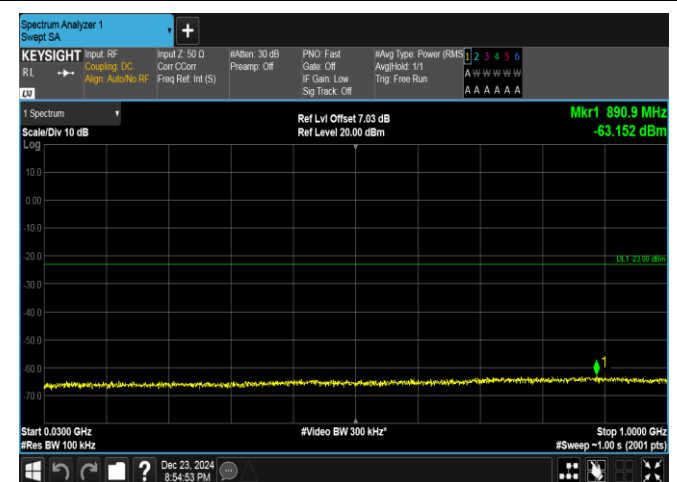
Band4-10MHz-QPSK-20350-1RB#49-30~1000-PASS
