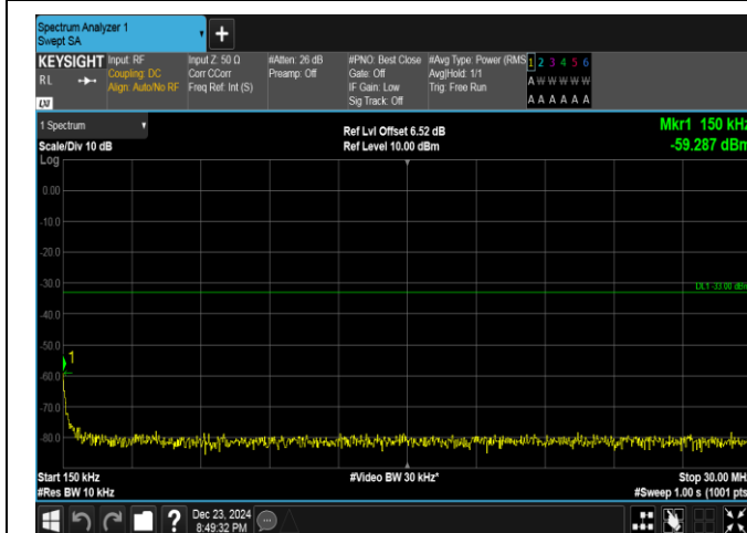
Band4-10MHz-16QAM-20175-1RB#49-0.15~30-PASS
