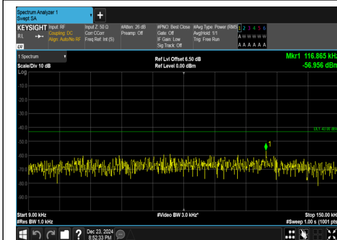
Band4-10MHz-QPSK-20350-1RB#0-0.009~0.15-PASS
