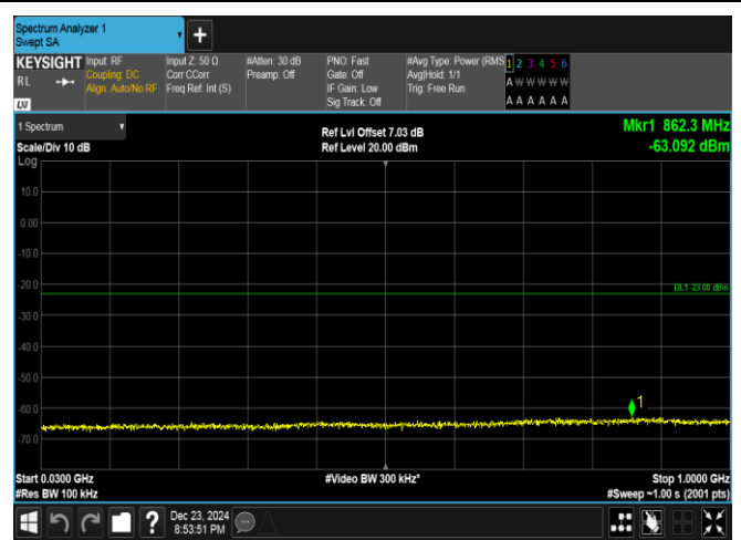
Band4-10MHz-16QAM-20350-1RB#0-30~1000-PASS
