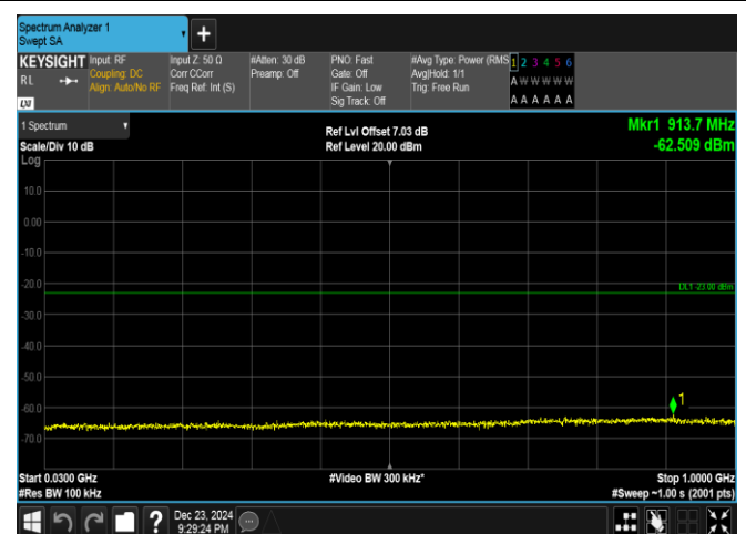
Band4-15MHz-QPSK-2025-1RB#74-30~1000-PASS
