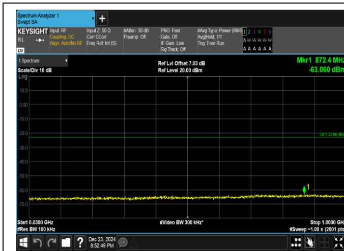
Band4-10MHz-QPSK-20350-1RB#0-30~1000-PASS
