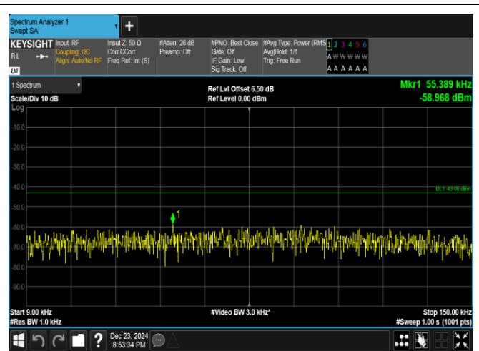
Band4-10MHz-16QAM-20350-1RB#0-0.009~0.15-PASS
