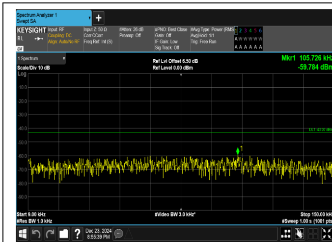
Band4-10MHz-16QAM-20350-1RB#49-0.009~0.15-PASS
