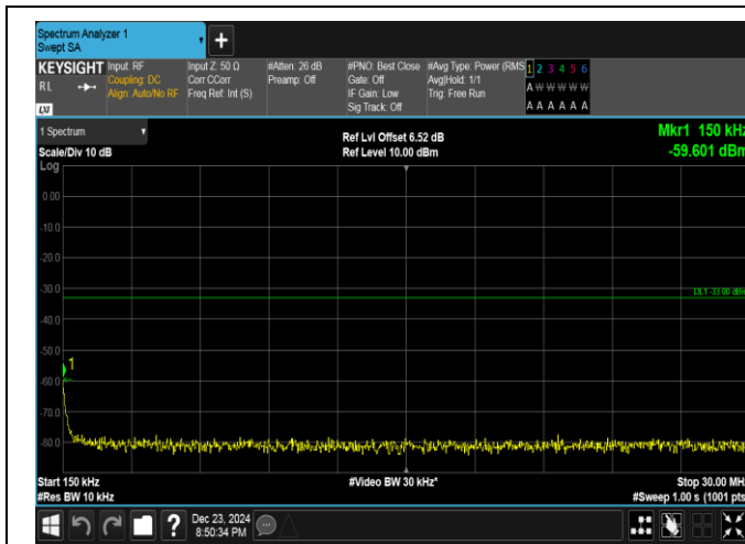
Band4-10MHz-QPSK-20175-50RB#0-0.15~30-PASS
