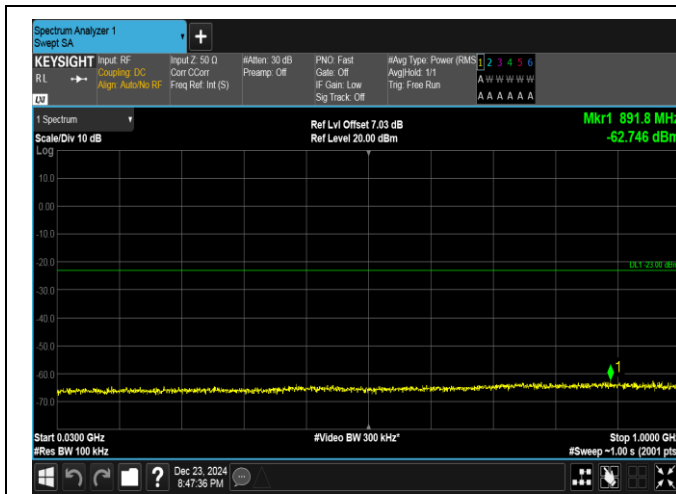
Band4-10MHz-16QAM-20175-1RB#0-30~1000-PASS
