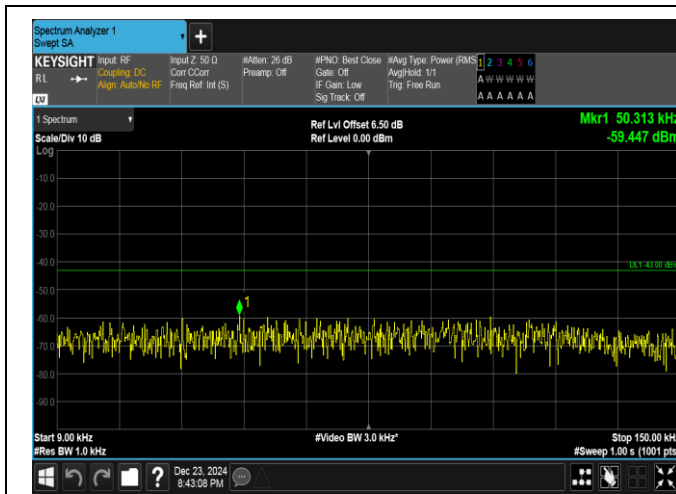
Band4-10MHz-16QAM-20000-1RB#49-0.009~0.15-PASS
