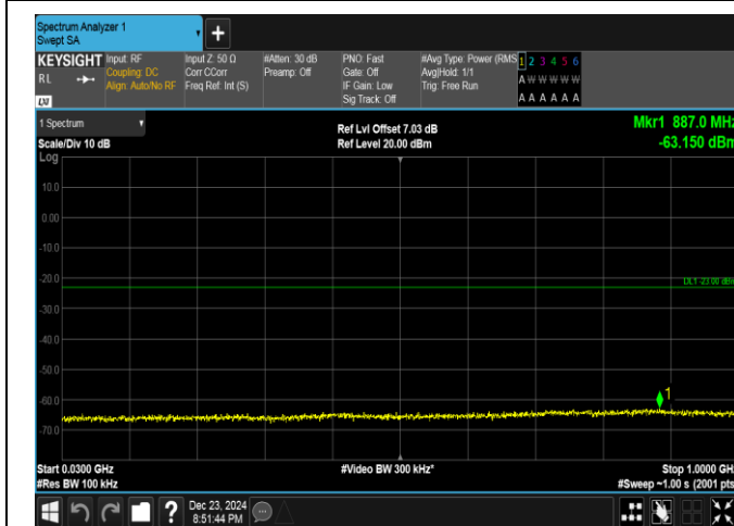
Band4-10MHz-16QAM-20175-50RB#0-30~1000-PASS
