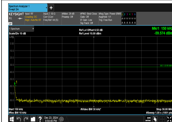
Band4-10MHz-QPSK-20350-1RB#49-0.15~30-PASS
