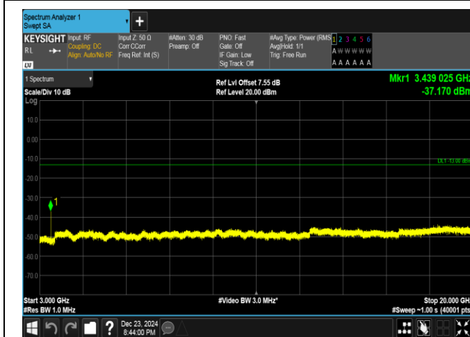
Band4-10MHz-16QAM-20000-1RB#49-3000~20000-PASS
