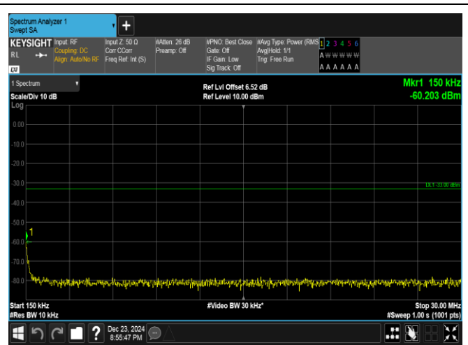
Band4-10MHz-16QAM-20350-1RB#49-0.15~30-PASS
