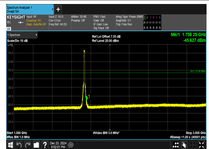
Band4-10MHz-16QAM-20175-50RB#0-1000~3000-PASS
