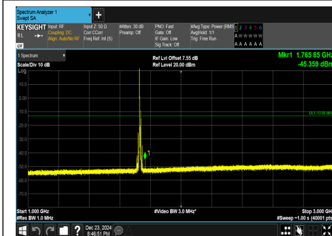
Band4-10MHz-QPSK-20175-1RB#0-1000~3000-PASS
