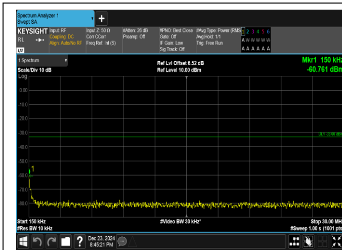
Band4-10MHz-16QAM-20000-50RB#0-0.15~30-PASS
