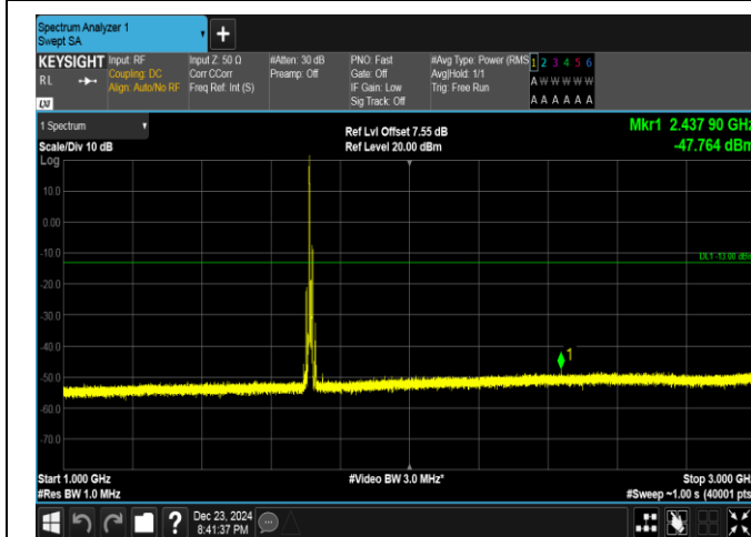
Band4-10MHz-16QAM-20000-1RB#0-1000~3000-PASS
