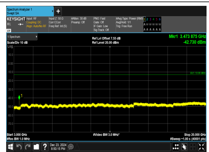
Band4-10MHz-16QAM-20175-1RB#49-3000~20000-PASS
