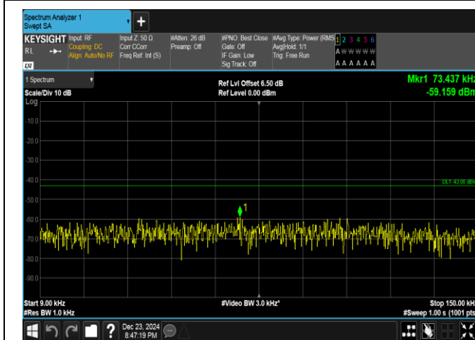
Band4-10MHz-16QAM-20175-1RB#0-0.009~0.15-PASS
