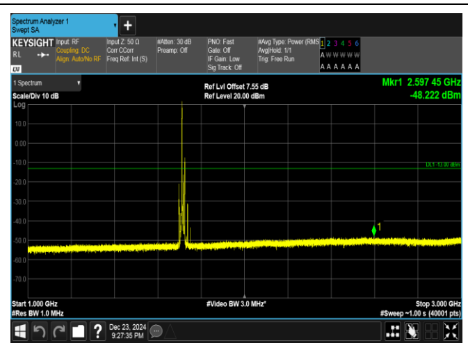
Band4-15MHz-QPSK-2025-1RB#0-1000~3000-PASS
