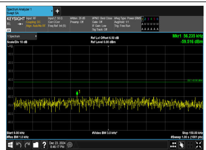
Band4-10MHz-QPSK-20175-1RB#0-0.009~0.15-PASS
