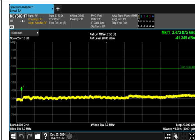
Band4-10MHz-QPSK-20175-1RB#49-3000~20000-PASS
