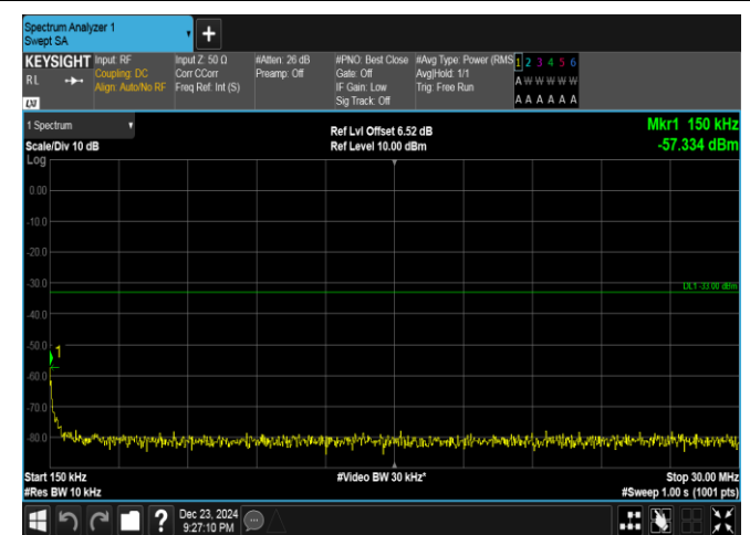
Band4-15MHz-QPSK-20025-1RB#0-0.15~30-PASS
