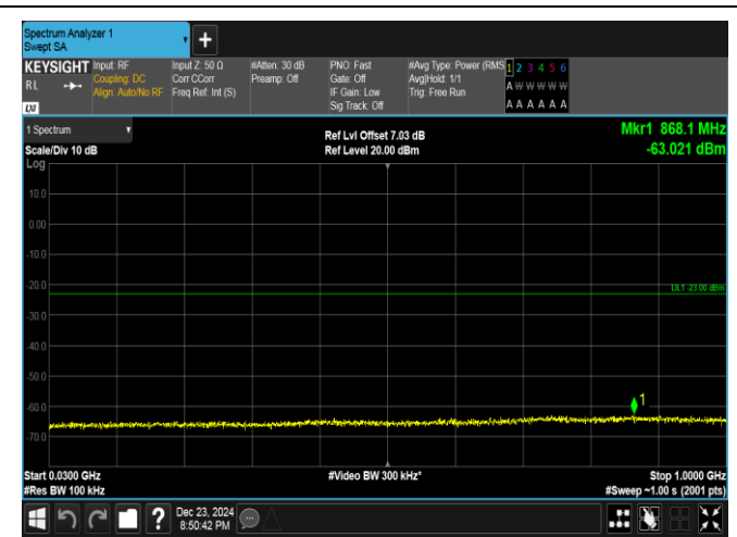
Band4-10MHz-QPSK-20175-50RB#0-30~1000-PASS
