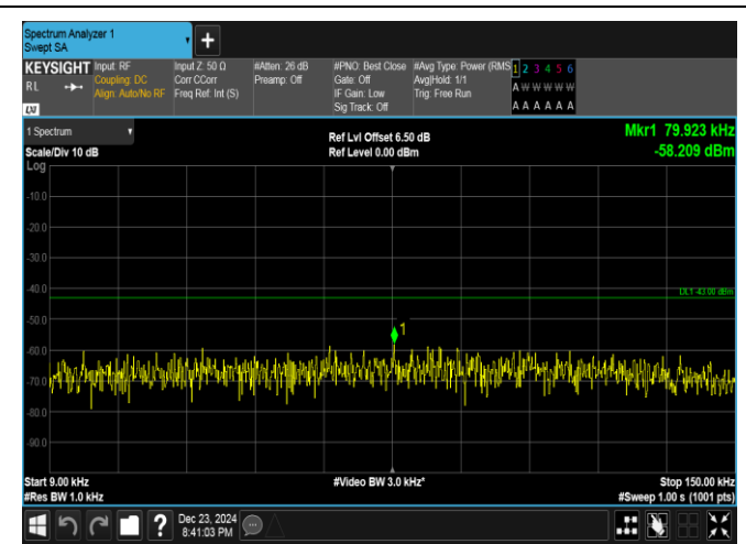
Band4-10MHz-16QAM-20000-1RB#0-0.009~0.15-PASS
