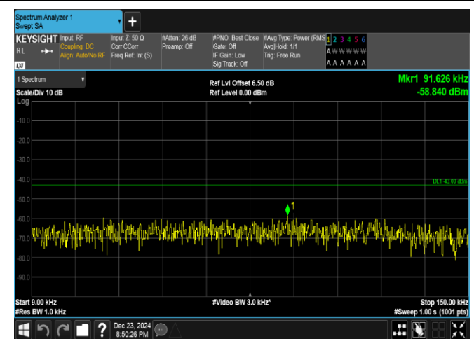
Band4-10MHz-QPSK-20175-50RB#0-0.009~0.15-PASS
