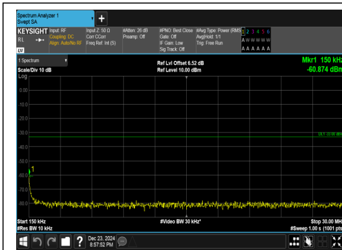
Band4-10MHz-16QAM-20350-50RB#0-0.15~30-PASS
