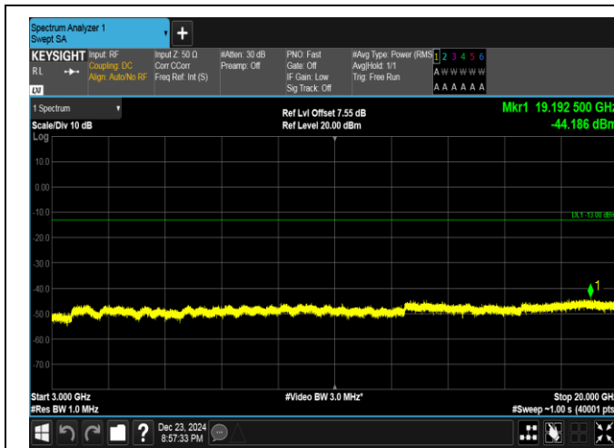
Band4-10MHz-QPSK-20350-50RB#0-3000~20000-PASS
