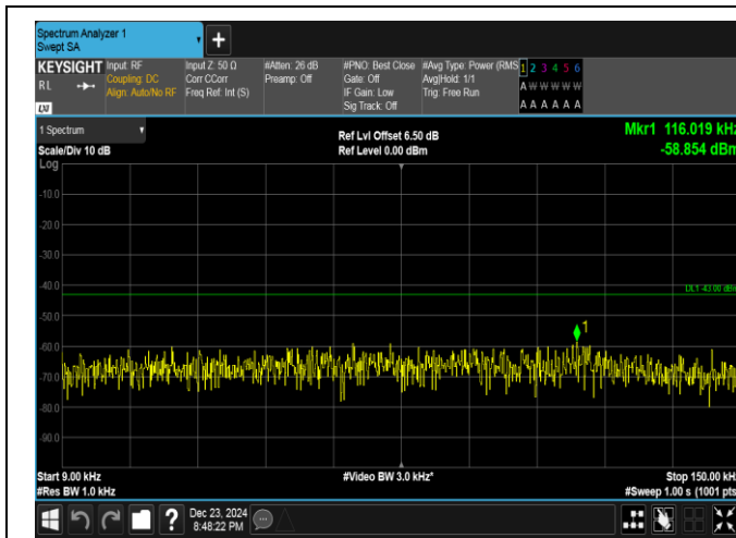
Band4-10MHz-QPSK-20175-1RB#49-0.009~0.15-PASS
