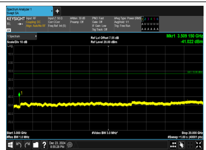
Band4-10MHz-QPSK-20350-1RB#49-3000~20000-PASS
