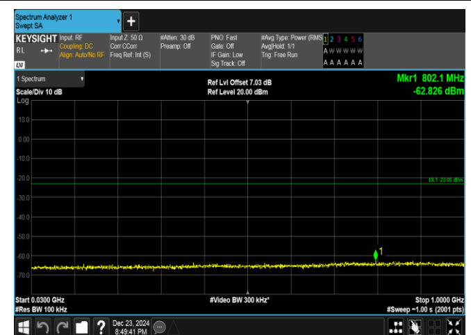
Band4-10MHz-16QAM-20175-1RB#49-30~1000-PASS
