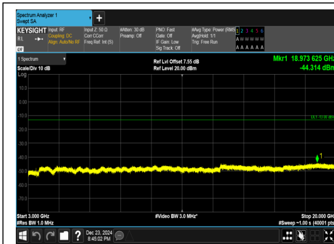
Band4-10MHz-QPSK-20000-50RB#0-3000~20000-PASS
