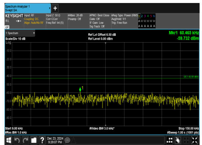
Band4-15MHz-QPSK-2025-1RB#74-0.009~0.15-PASS
