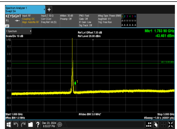
Band4-10MHz-QPSK-20350-1RB#0-1000~3000-PASS
