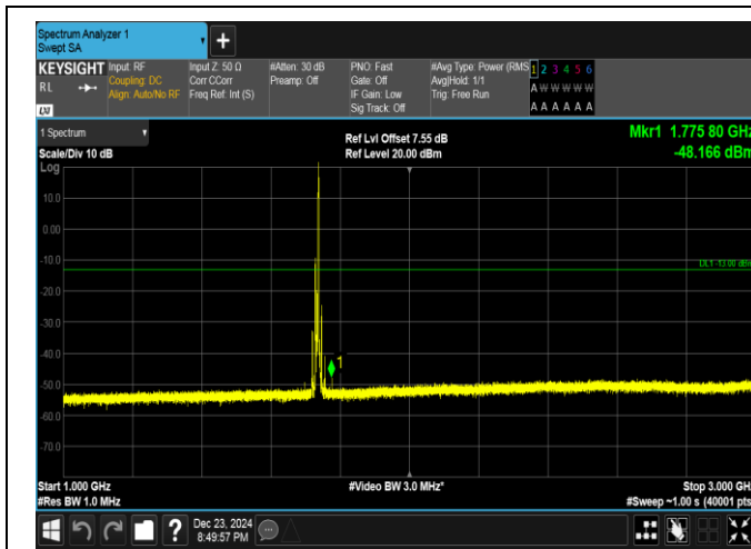
Band4-10MHz-16QAM-20175-1RB#49-1000~3000-PASS
