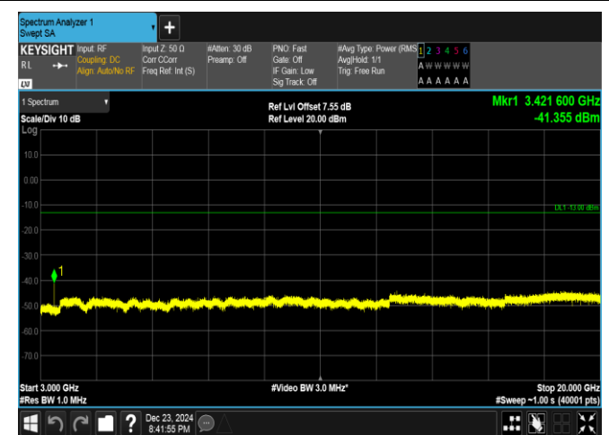
Band4-10MHz-16QAM-20000-1RB#0-3000~20000-PASS
