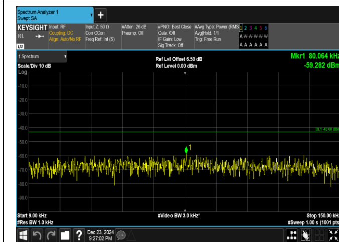
Band4-15MHz-QPSK-20025-1RB#0-0.009~0.15-PASS
