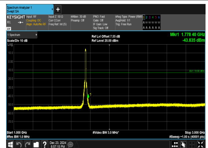
Band4-10MHz-QPSK-20350-50RB#0-1000~3000-PASS
