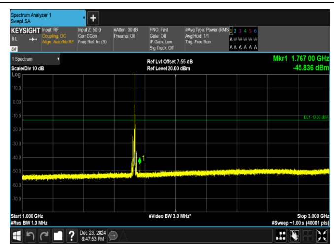
Band4-10MHz-16QAM-20175-1RB#0-1000~3000-PASS
