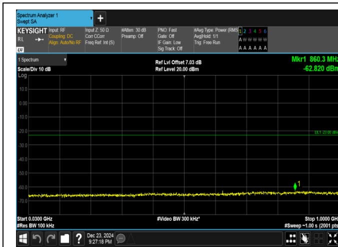
Band4-15MHz-QPSK-2025-1RB#0-30~1000-PASS
