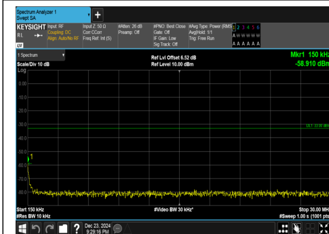
Band4-15MHz-QPSK-2025-1RB#74-0.15~30-PASS
