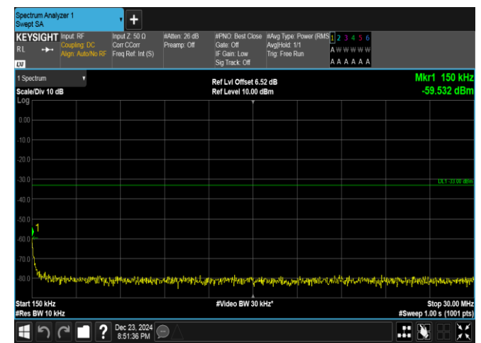
Band4-10MHz-16QAM-20175-50RB#0-0.15~30-PASS
