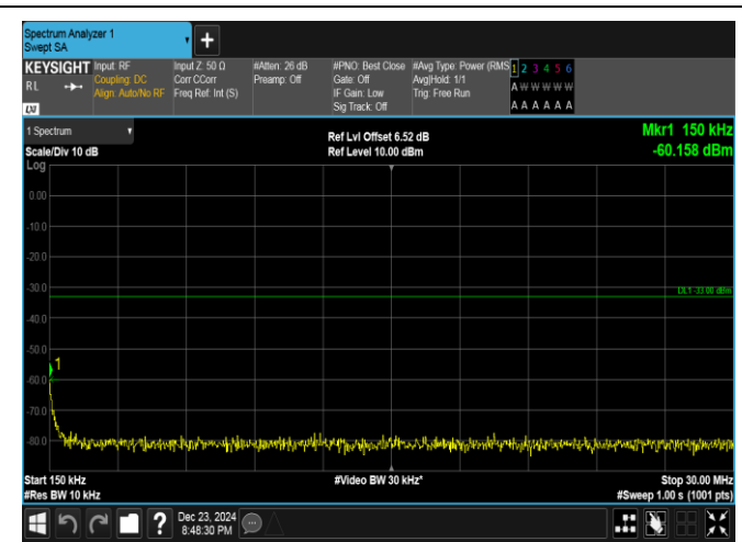
Band4-10MHz-QPSK-20175-1RB#49-0.15~30-PASS
