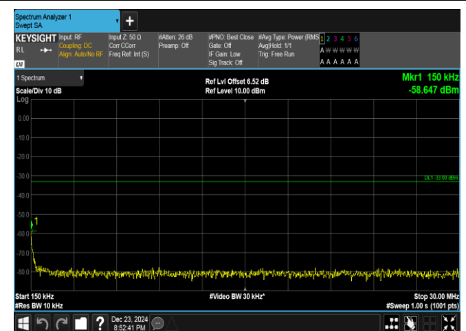
Band4-10MHz-QPSK-20350-1RB#0-0.15~30-PASS
