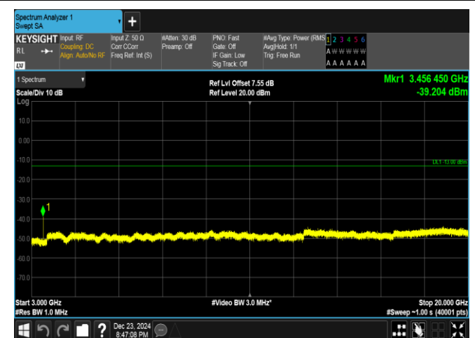
Band4-10MHz-QPSK-20175-1RB#0-3000~20000-PASS
