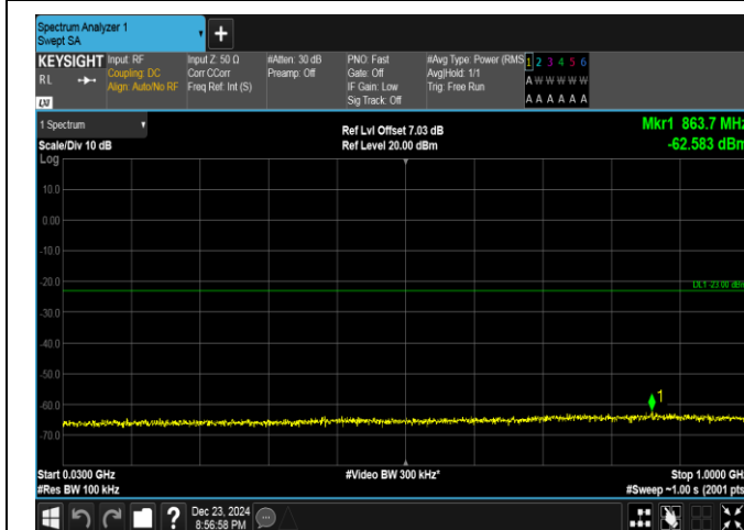
Band4-10MHz-QPSK-20350-50RB#0-30~1000-PASS
