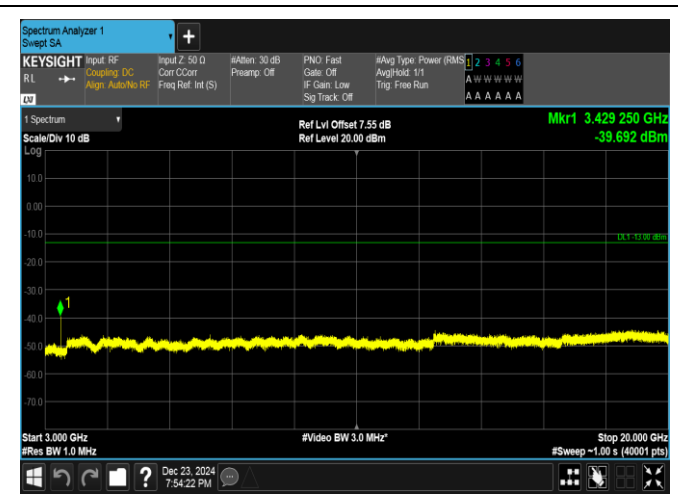
Band4-5MHz-QPSK-19975-1RB#24-3000~20000-PASS
