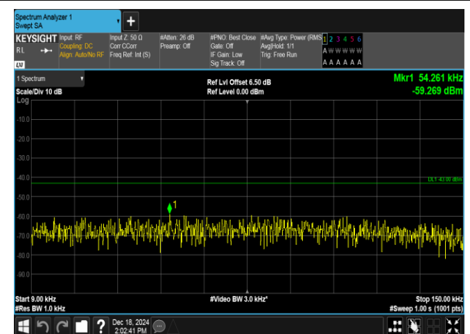
Band4-3MHz-QPSK-20385-1RB#14-0.009~0.15-PASS
