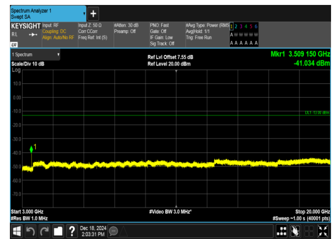
Band4-3MHz-QPSK-20385-1RB#14-3000~20000-PASS
