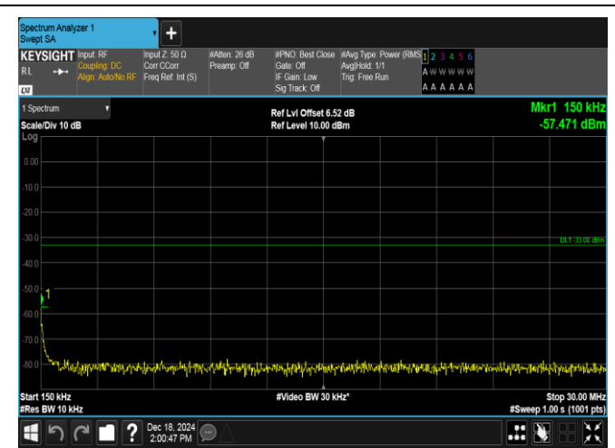
Band4-3MHz-QPSK-20385-1RB#0-0.15~30-PASS
