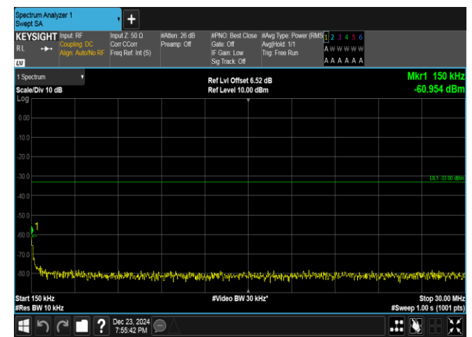
Band4-5MHz-QPSK-19975-25RB#0-0.15~30-PASS
