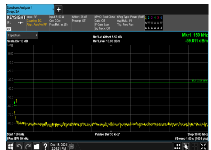
Band4-3MHz-QPSK-20385-15RB#0-0.15~30-PASS
