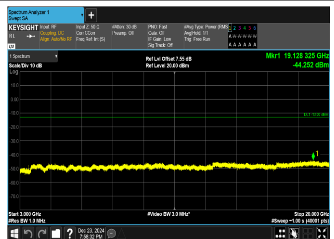
Band4-5MHz-QPSK-20175-1RB#0-3000~20000-PASS
