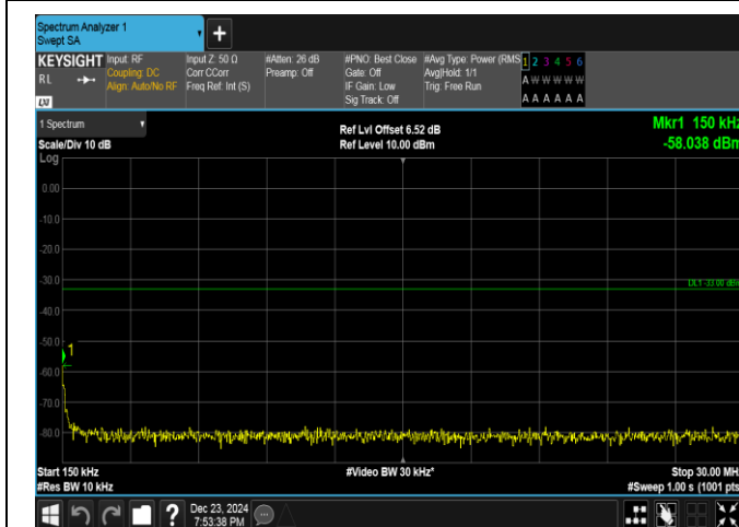
Band4-5MHz-QPSK-19975-1RB#24-0.15~30-PASS
