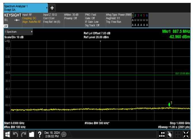
Band4-3MHz-16QAM-20385-15RB#0-30~1000-PASS
