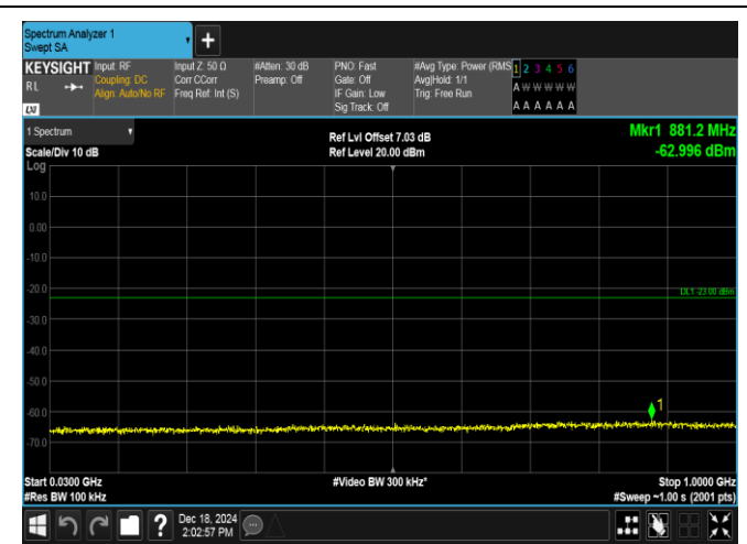
Band4-3MHz-QPSK-20385-1RB#14-30~1000-PASS
