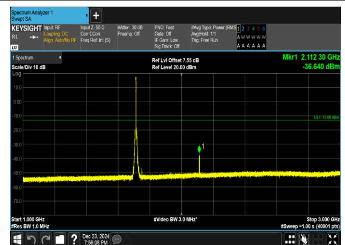
Band4-5MHz-QPSK-19975-25RB#0-1000~3000-PASS
