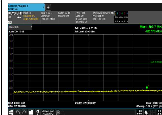
Band4-5MHz-QPSK-19975-25RB#0-30~1000-PASS
