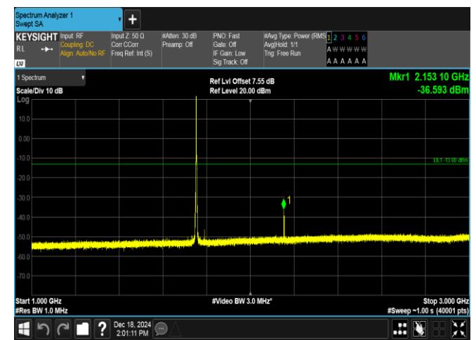
Band4-3MHz-QPSK-20385-1RB#0-1000~3000-PASS
