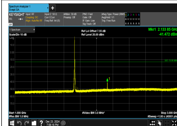
Band4-5MHz-QPSK-20175-1RB#0-1000~3000-PASS
