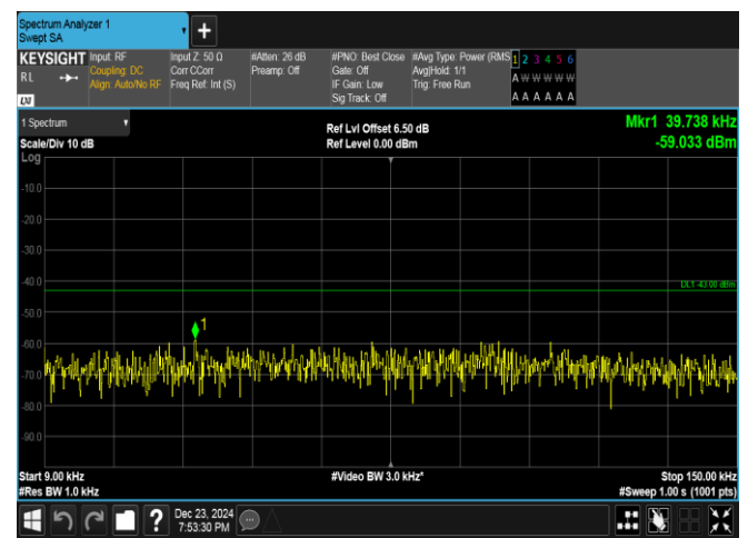
Band4-5MHz-QPSK-19975-1RB#24-0.009~0.15-PASS
