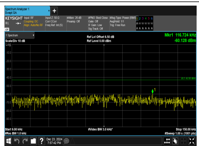
Band4-5MHz-QPSK-20175-1RB#0-0.009~0.15-PASS
