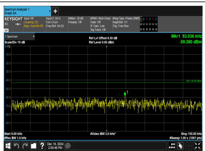
Band4-3MHz-16QAM-20385-15RB#0-0.009~0.15-PASS
