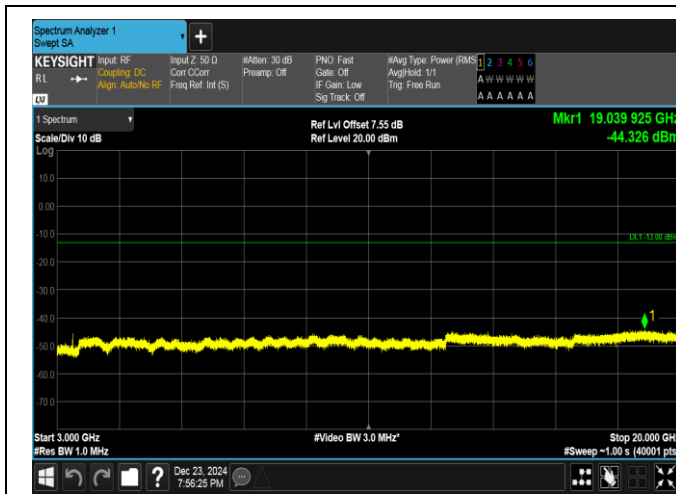
Band4-5MHz-QPSK-19975-25RB#0-3000~20000-PASS
