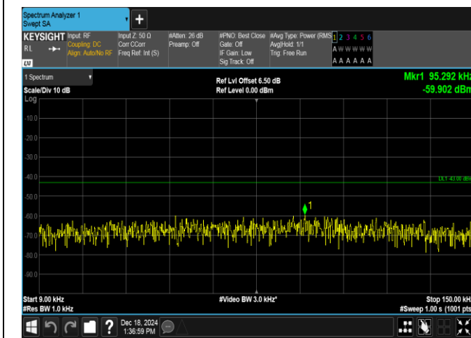
Band4-3MHz-QPSK-20175-1RB#14-0.009~0.15-PASS
