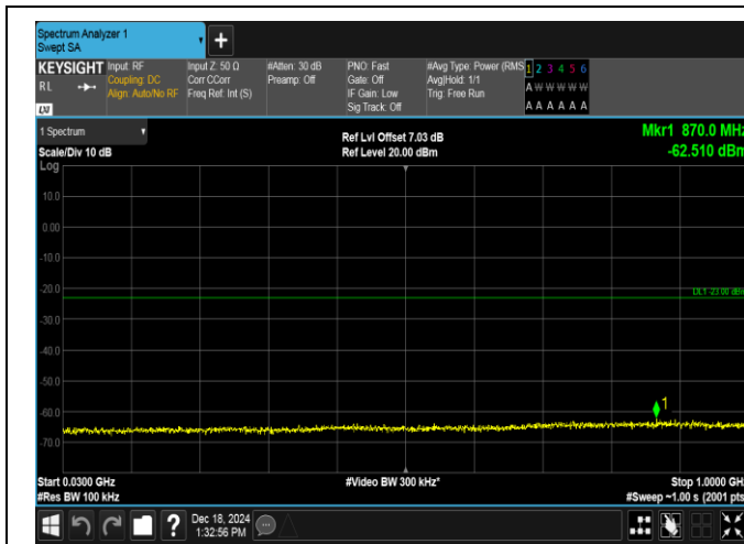
Band4-3MHz-QPSK-19965-15RB#0-30~1000-PASS
