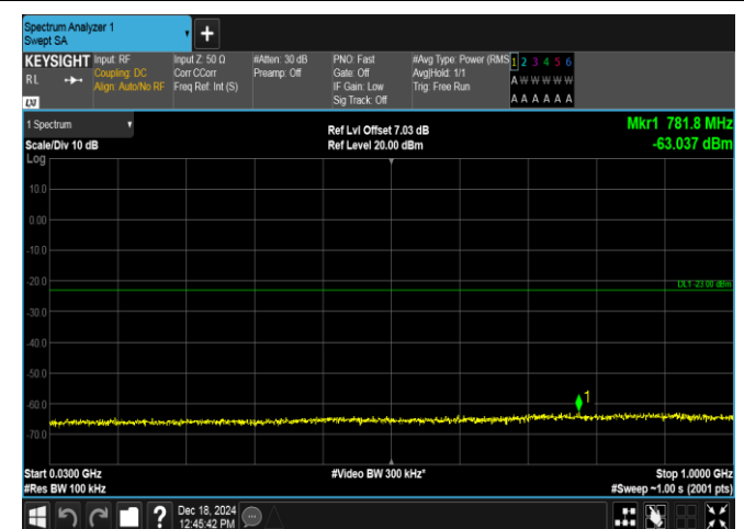
Band4-1.4MHz-16QAM-20393-1RB#0-30~1000-PASS
