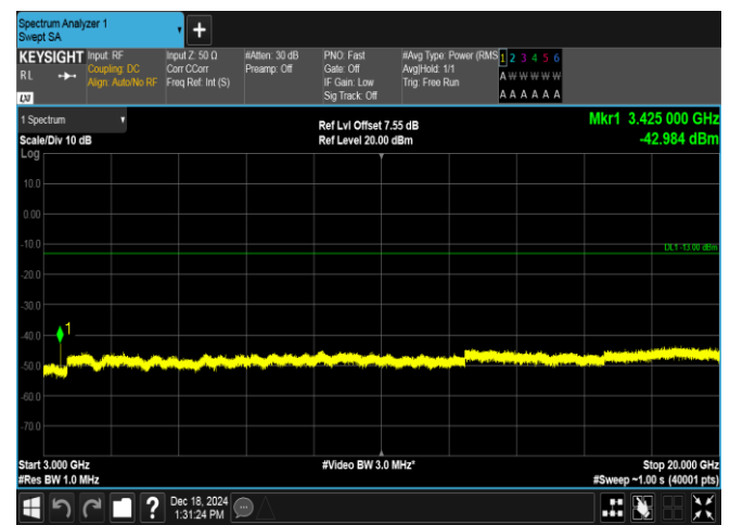
Band4-3MHz-QPSK-19965-1RB#14-3000~20000-PASS
