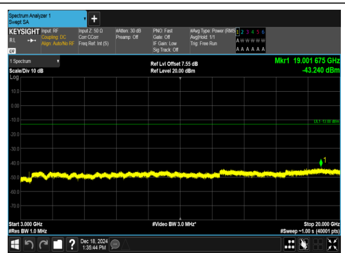
Band4-3MHz-QPSK-20175-1RB#0-3000~20000-PASS
