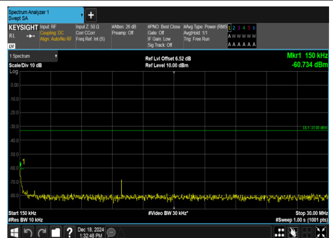
Band4-3MHz-QPSK-19965-15RB#0-0.15~30-PASS
