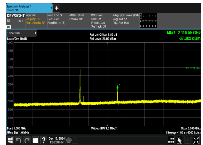
Band4-3MHz-QPSK-19965-1RB#0-1000~3000-PASS
