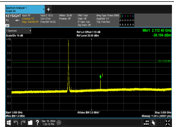
Band4-3MHz-QPSK-19965-15RB#0-1000~3000-PASS
