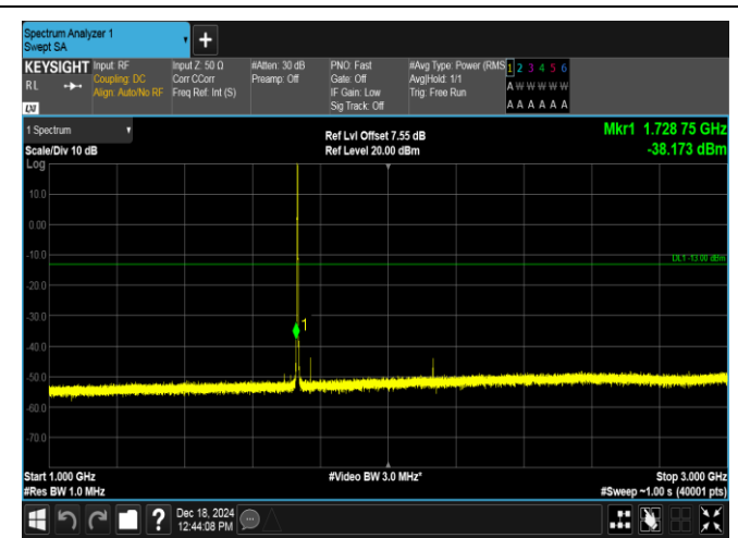
Band4-1.4MHz-16QAM-20175-6RB#0-1000~3000-PASS
