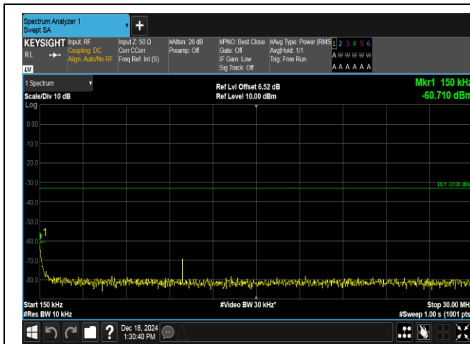
Band4-3MHz-QPSK-19965-1RB#14-0.15~30-PASS
