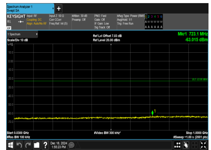
Band4-3MHz-QPSK-20175-15RB#0-30~1000-PASS
