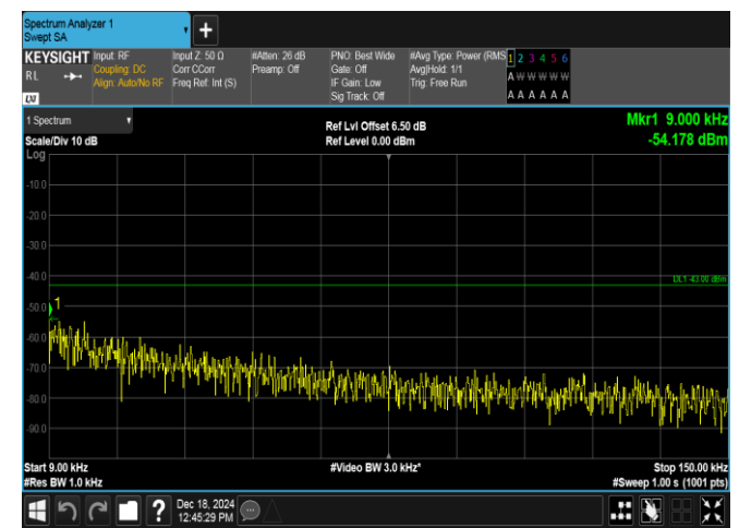
Band4-1.4MHz-16QAM-20393-1RB#0-0.009~0.15-PASS
