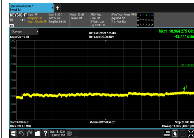
Band4-1.4MHz-QPSK-20393-6RB#0-3000~20000-PASS
