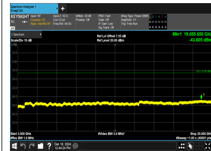
Band4-1.4MHz-16QAM-20175-6RB#0-3000~20000-PASS
