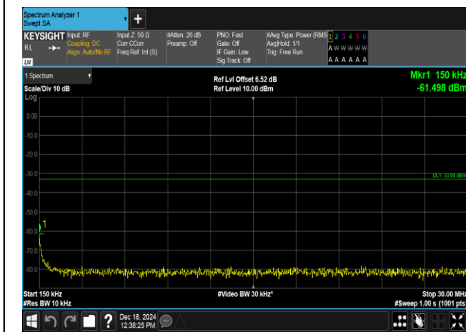
Band4-1.4MHz-16QAM-19957-6RB#0-0.15~30-PASS
