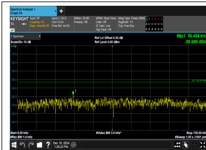
Band4-3MHz-QPSK-19965-1RB#0-0.009~0.15-PASS
