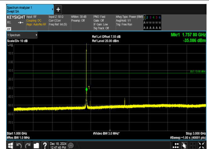
Band4-1.4MHz-16QAM-20393-1RB#5-1000~3000-PASS
