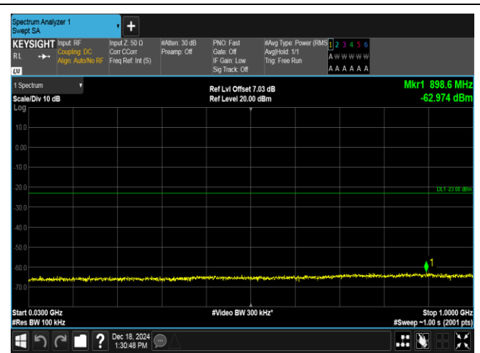
Band4-3MHz-QPSK-19965-1RB#14-30~1000-PASS
