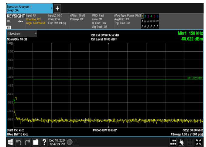
Band4-1.4MHz-16QAM-20393-1RB#5-0.15~30-PASS
