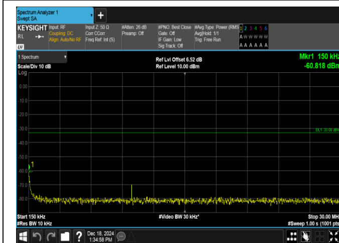
Band4-3MHz-QPSK-20175-1RB#0-0.15~30-PASS
