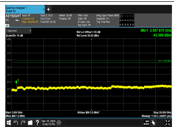
Band4-1.4MHz-16QAM-20393-1RB#0-3000~20000-PASS
