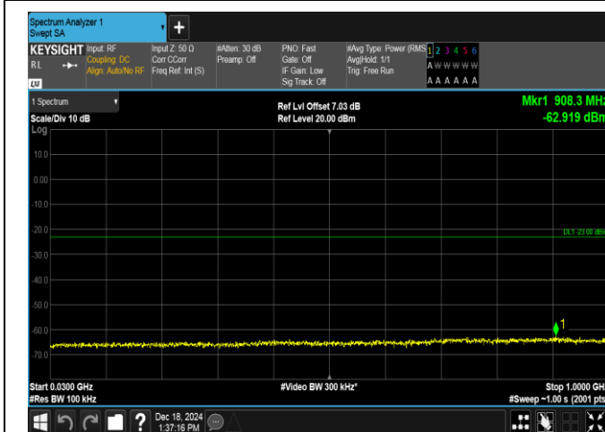
Band4-3MHz-QPSK-20175-1RB#14-30~1000-PASS
