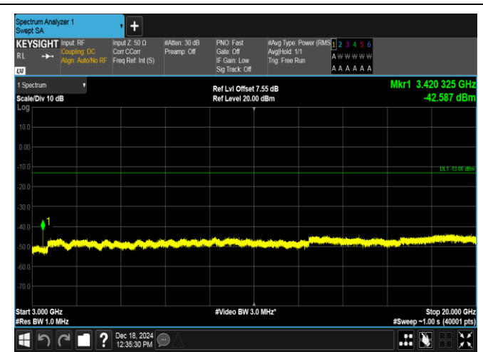
Band4-1.4MHz-16QAM-19957-1RB#0-3000~20000-PASS
