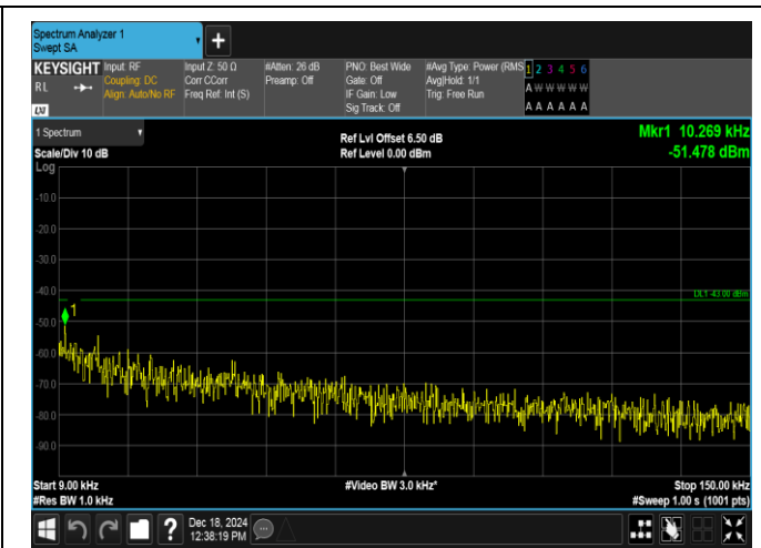
Band4-1.4MHz-16QAM-19957-6RB#0-0.009~0.15-PASS
