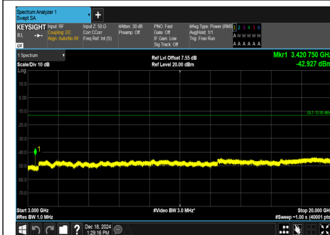
Band4-3MHz-QPSK-19965-1RB#0-3000~20000-PASS
