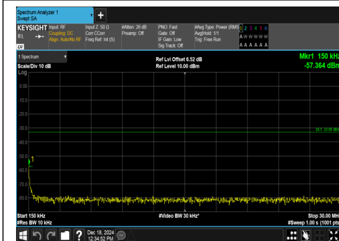
Band4-1.4MHz-16QAM-19957-1RB#0-0.15~30-PASS
