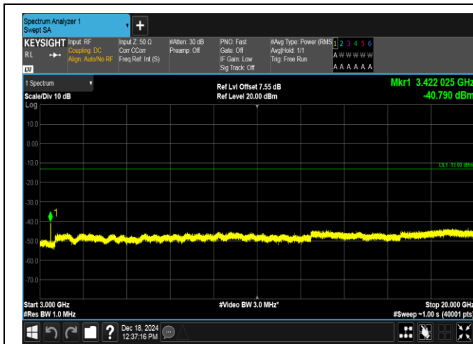
Band4-1.4MHz-16QAM-19957-1RB#5-3000~20000-PASS
