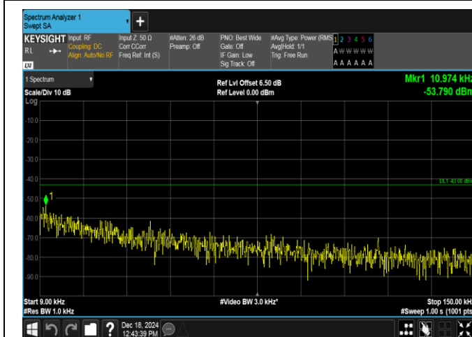
Band4-1.4MHz-16QAM-20175-6RB#0-0.009~0.15-PASS
