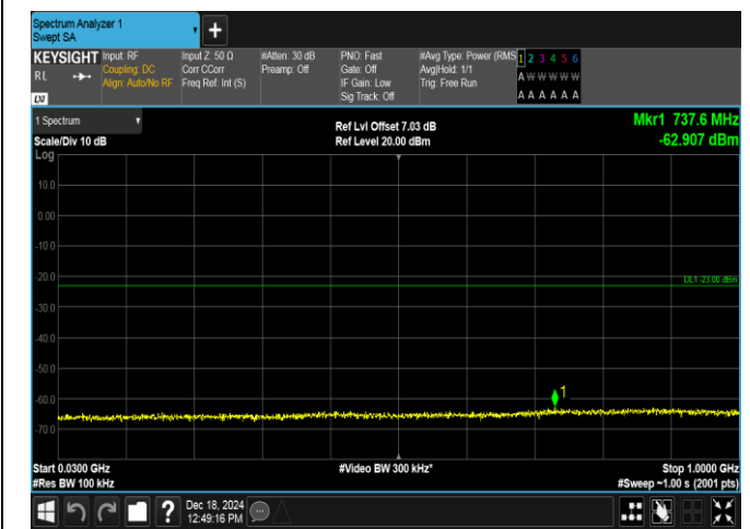
Band4-1.4MHz-16QAM-20393-6RB#0-30~1000-PASS
