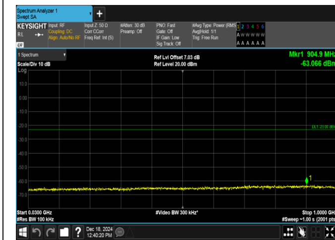
Band4-1.4MHz-16QAM-20175-1RB#0-30~1000-PASS
