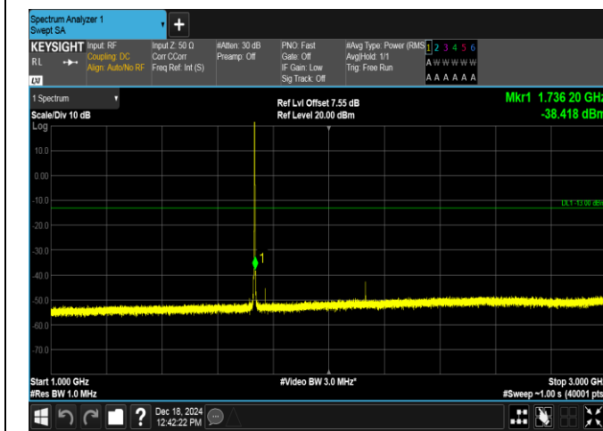
Band4-1.4MHz-16QAM-20175-1RB#5-1000~3000-PASS
