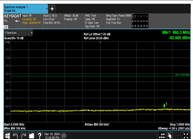
Band4-1.4MHz-16QAM-19957-1RB#0-30~1000-PASS
