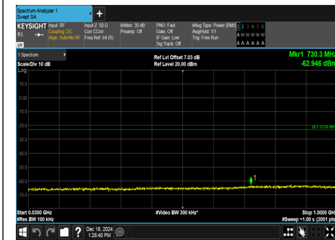
Band4-3MHz-QPSK-19965-1RB#0-30~1000-PASS
