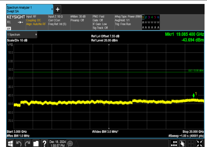
Band4-3MHz-QPSK-20175-15RB#0-3000~20000-PASS
