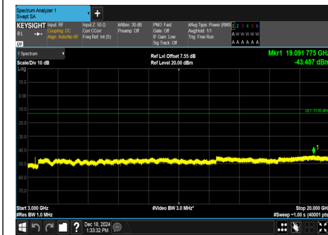
Band4-3MHz-QPSK-19965-15RB#0-3000~20000-PASS
