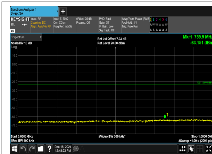
Band4-1.4MHz-QPSK-20393-6RB#0-30~1000-PASS
