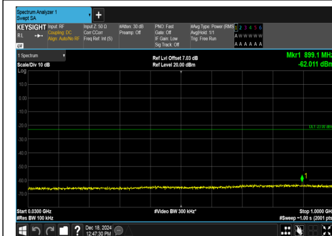
Band4-1.4MHz-16QAM-20393-1RB#5-30~1000-PASS
