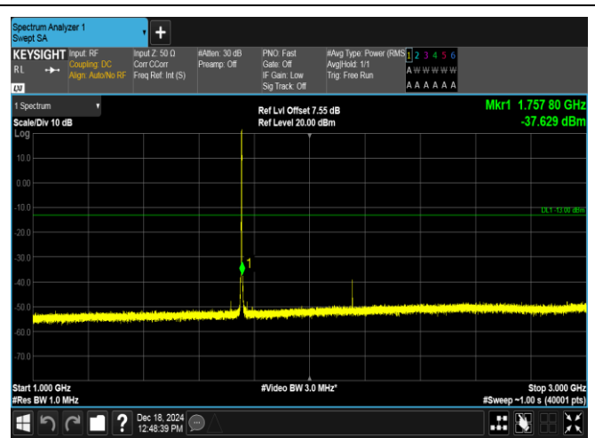
Band4-1.4MHz-QPSK-20393-6RB#0-1000~3000-PASS
