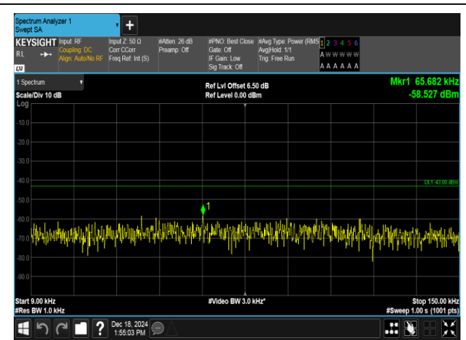
Band4-3MHz-QPSK-20175-15RB#0-0.009~0.15-PASS
