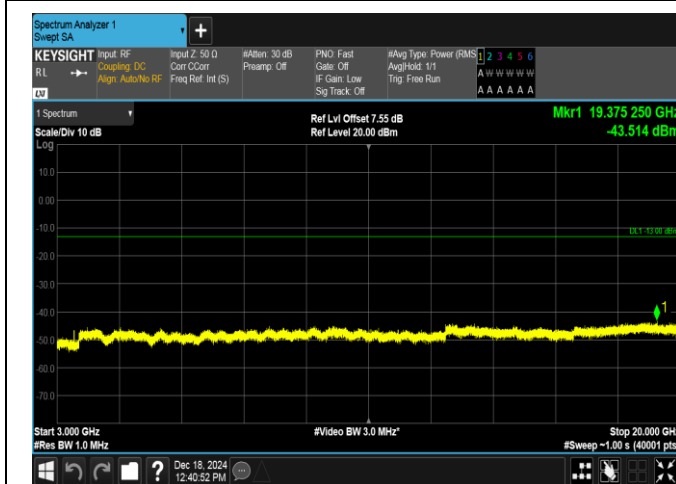
Band4-1.4MHz-16QAM-20175-1RB#0-3000~20000-PASS
