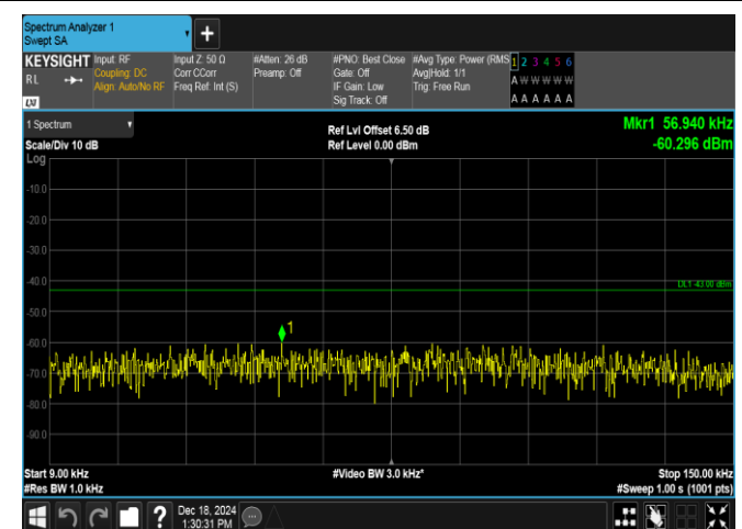
Band4-3MHz-QPSK-19965-1RB#14-0.009~0.15-PASS
