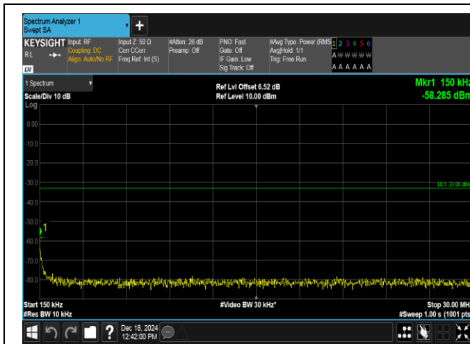
Band4-1.4MHz-16QAM-20175-1RB#5-0.15~30-PASS
