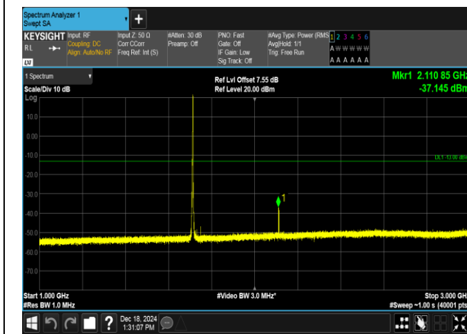
Band4-3MHz-QPSK-19965-1RB#14-1000~3000-PASS
