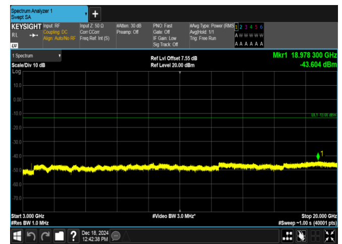
Band4-1.4MHz-16QAM-20175-1RB#5-3000~20000-PASS
