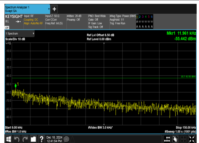
Band4-1.4MHz-16QAM-20175-1RB#5-0.009~0.15-PASS
