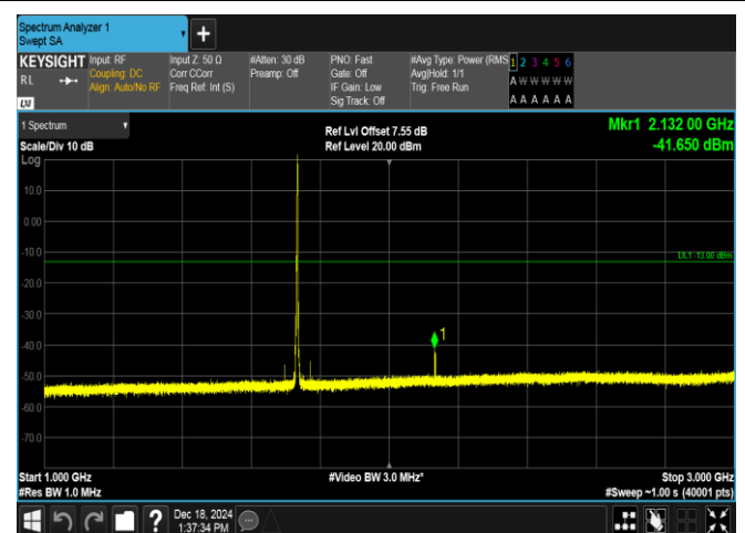
Band4-3MHz-QPSK-20175-1RB#14-1000~3000-PASS
