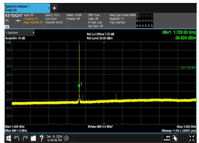
Band4-1.4MHz-16QAM-20175-1RB#0-1000~3000-PASS
