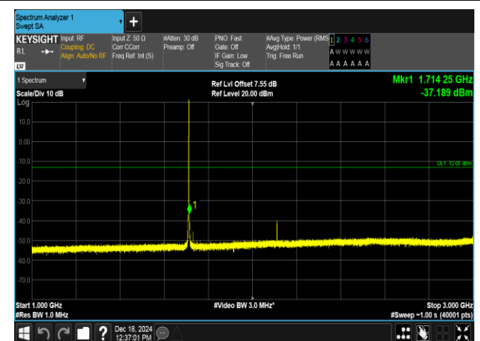
Band4-1.4MHz-16QAM-19957-1RB#5-1000~3000-PASS
