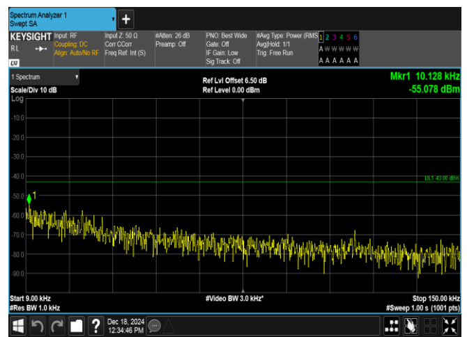
Band4-1.4MHz-16QAM-19957-1RB#0-0.009~0.15-PASS
