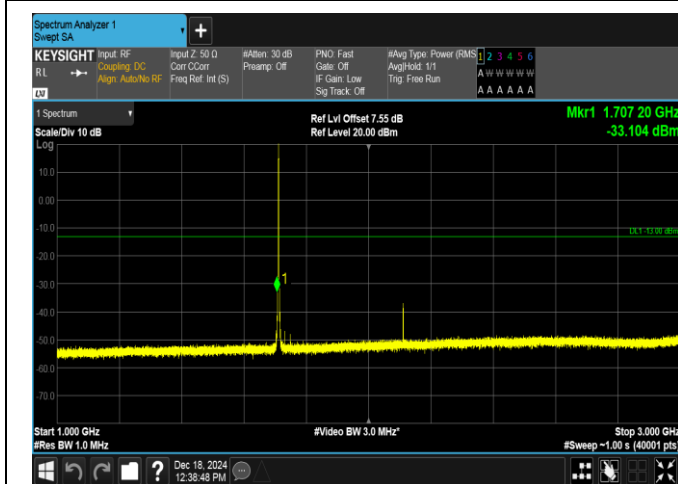
Band4-1.4MHz-16QAM-19957-6RB#0-1000~3000-PASS
