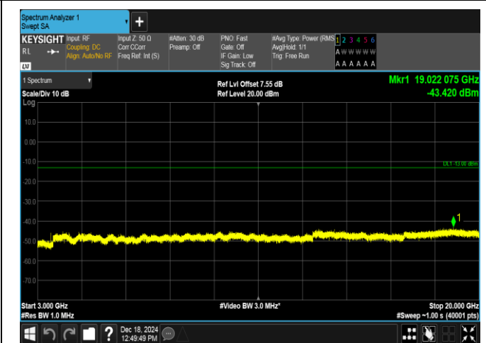
Band4-1.4MHz-16QAM-20393-6RB#0-3000~20000-PASS
