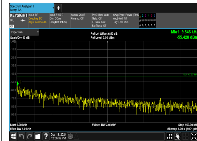
Band4-1.4MHz-16QAM-19957-1RB#5-0.009~0.15-PASS
