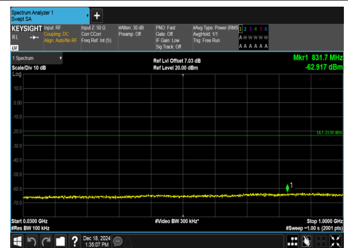
Band4-3MHz-QPSK-20175-1RB#0-30~1000-PASS
