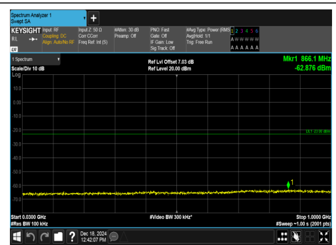
Band4-1.4MHz-16QAM-20175-1RB#5-30~1000-PASS
