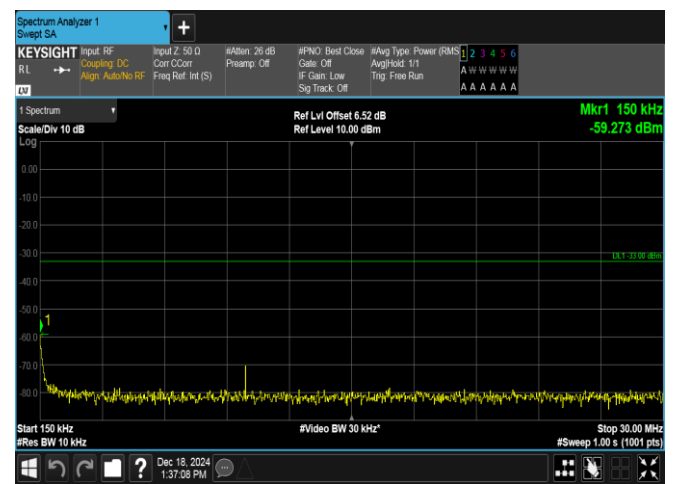
Band4-3MHz-QPSK-20175-1RB#14-0.15~30-PASS
