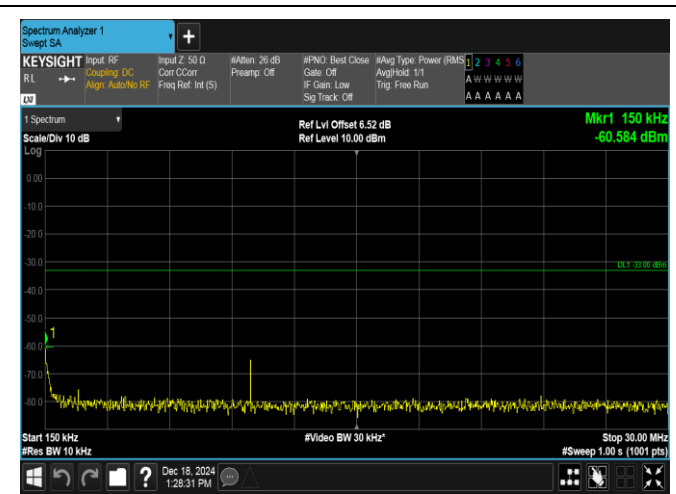
Band4-3MHz-QPSK-19965-1RB#0-0.15~30-PASS
