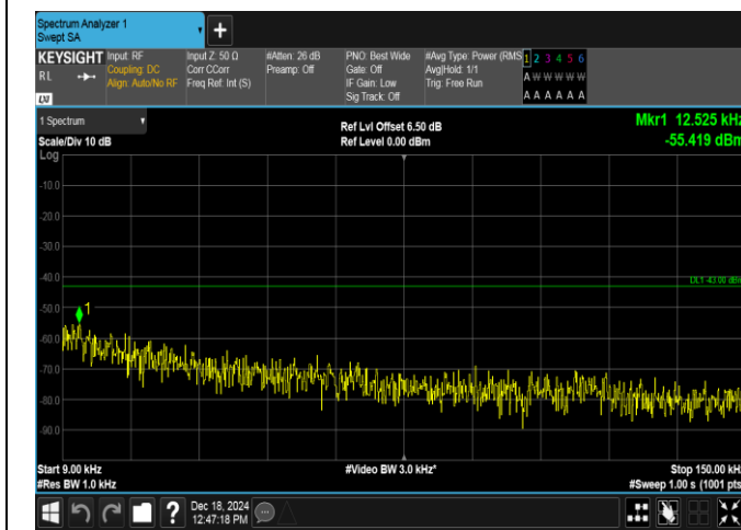
Band4-1.4MHz-16QAM-20393-1RB#5-0.009~0.15-PASS
