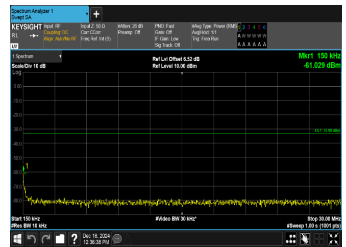
Band4-1.4MHz-16QAM-19957-1RB#5-0.15~30-PASS
