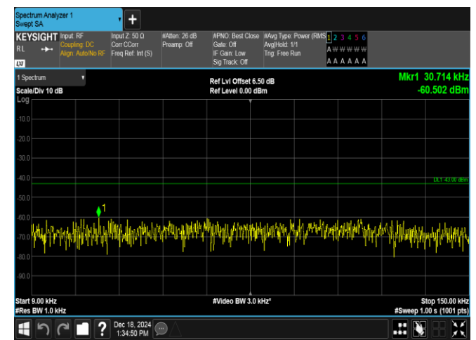
Band4-3MHz-QPSK-20175-1RB#0-0.009~0.15-PASS
