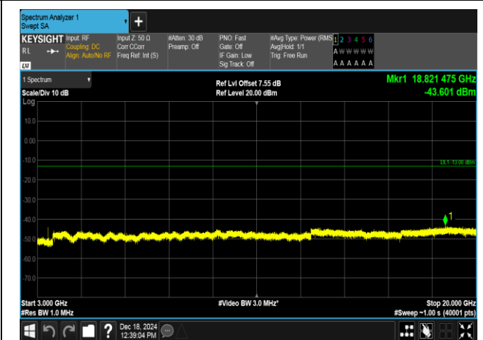
Band4-1.4MHz-16QAM-19957-6RB#0-3000~20000-PASS
