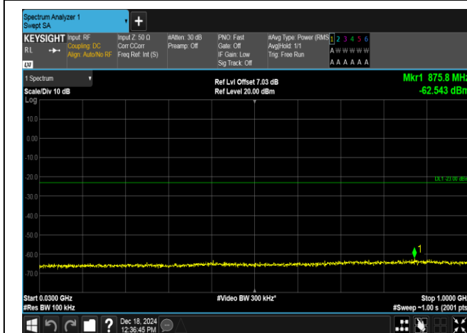
Band4-1.4MHz-16QAM-19957-1RB#5-30~1000-PASS
