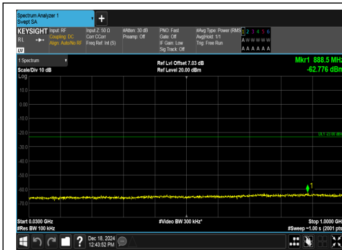
Band4-1.4MHz-16QAM-20175-6RB#0-30~1000-PASS
