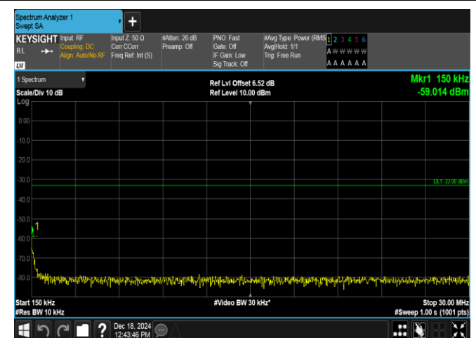
Band4-1.4MHz-16QAM-20175-6RB#0-0.15~30-PASS
