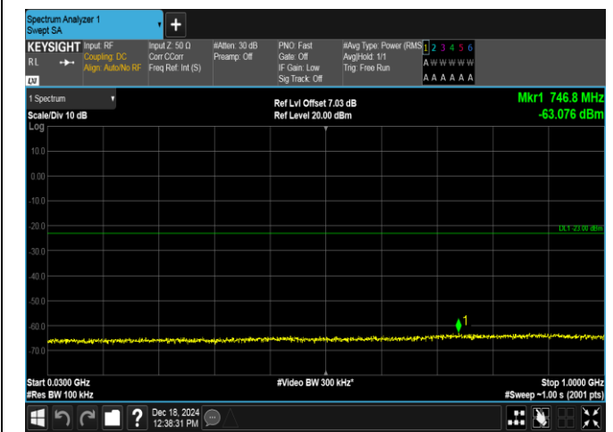
Band4-1.4MHz-16QAM-19957-6RB#0-30~1000-PASS
