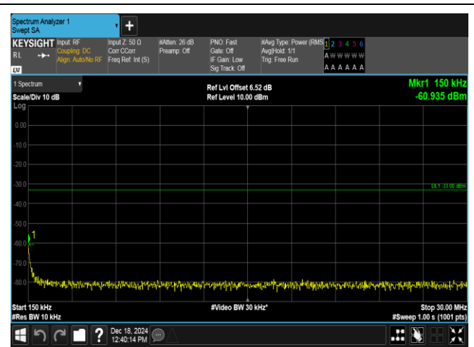
Band4-1.4MHz-16QAM-20175-1RB#0-0.15~30-PASS
