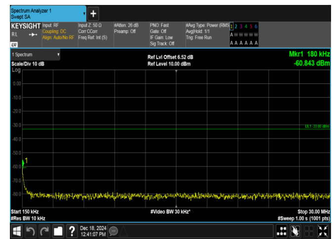
Band4-1.4MHz-QPSK-20175-1RB#5-0.15~30-PASS
