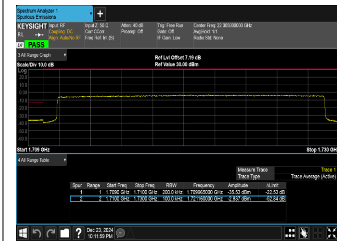
Band4-20MHz-16QAM-20050-100RB#0-PASS
