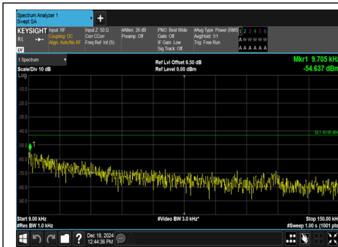
Band4-1.4MHz-QPSK-20393-1RB#0-0.009~0.15-PASS
