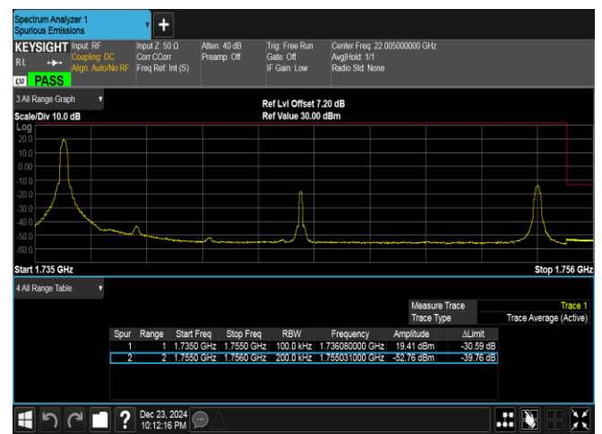
Band4-20MHz-QPSK-20300-1RB#0-PASS
