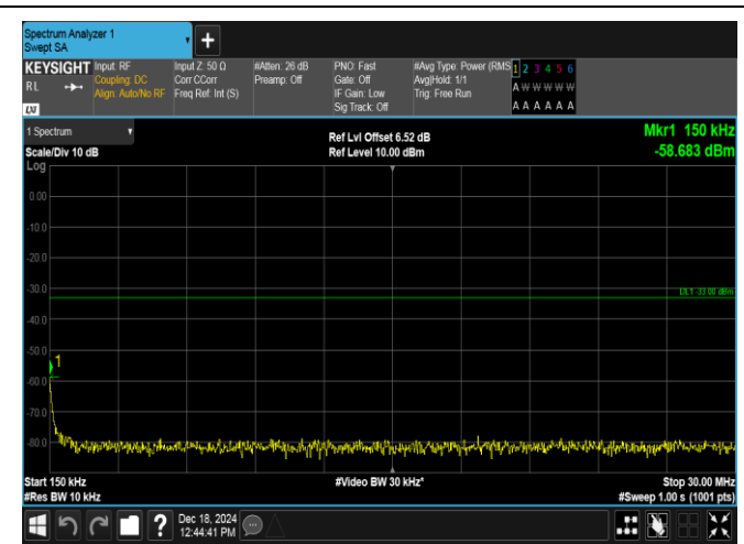
Band4-1.4MHz-QPSK-20393-1RB#0-0.15~30-PASS
