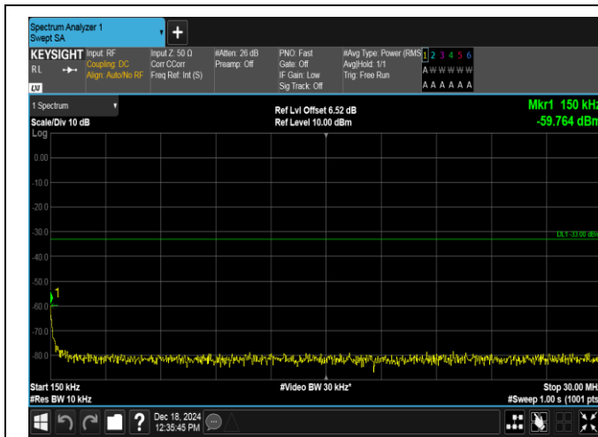
Band4-1.4MHz-QPSK-19957-1RB#5-0.15~30-PASS
