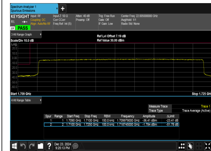
Band4-15MHz-16QAM-20025-75RB#0-PASS
