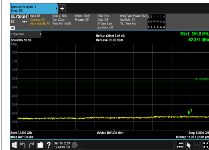
Band4-1.4MHz-QPSK-20393-1RB#0-30~1000-PASS
