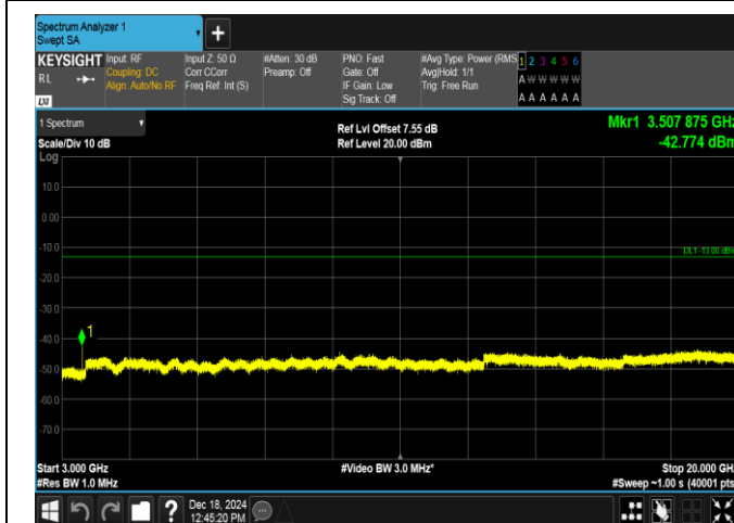
Band4-1.4MHz-QPSK-20393-1RB#0-3000~20000-PASS
