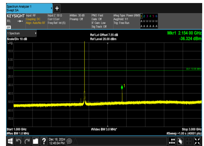
Band4-1.4MHz-QPSK-20393-1RB#0-1000~3000-PASS
