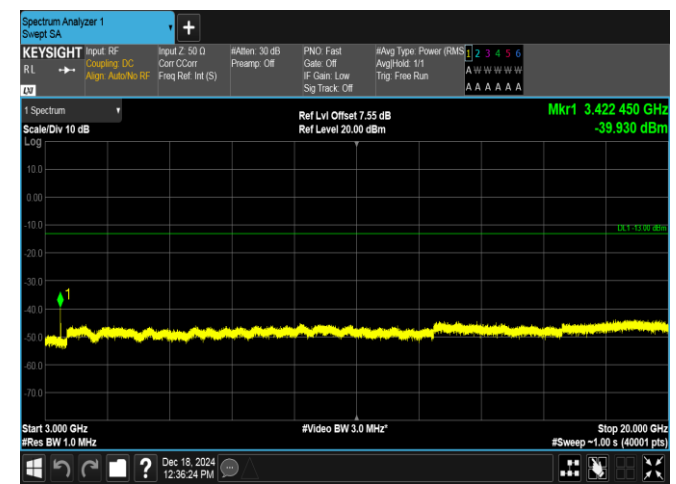
Band4-1.4MHz-QPSK-19957-1RB#5-3000~20000-PASS
