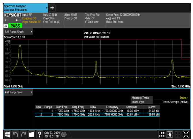
Band4-20MHz-16QAM-20300-1RB#0-PASS
