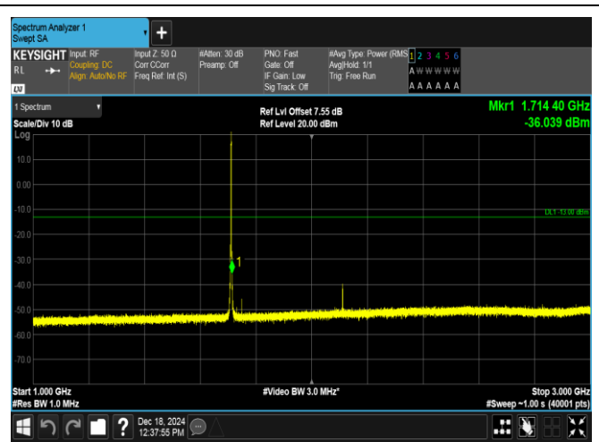
Band4-1.4MHz-QPSK-19957-6RB#0-1000~3000-PASS
