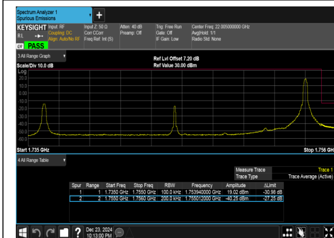
Band4-20MHz-16QAM-20300-1RB#99-PASS
