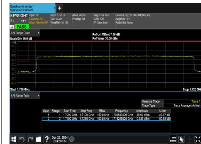
Band4-15MHz-QPSK-20025-75RB#0-PASS
