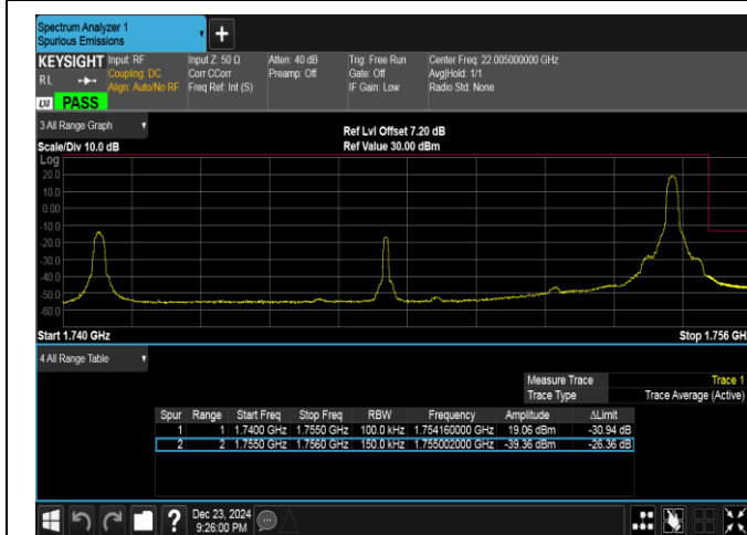
Band4-15MHz-QPSK-20325-1RB#74-PASS
