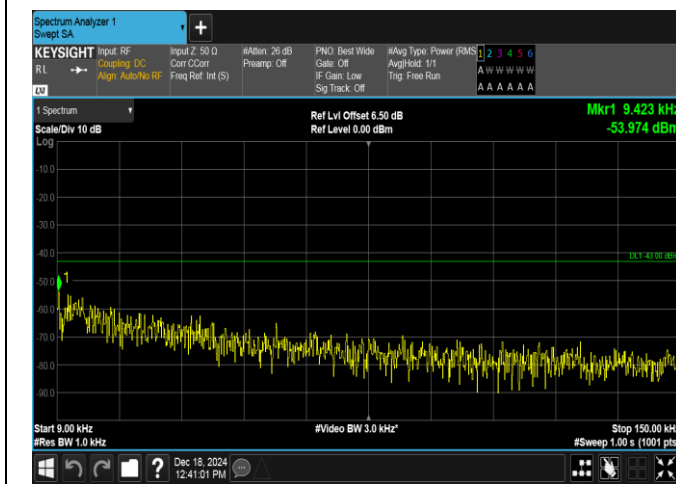
Band4-1.4MHz-QPSK-20175-1RB#5-0.009~0.15-PASS
