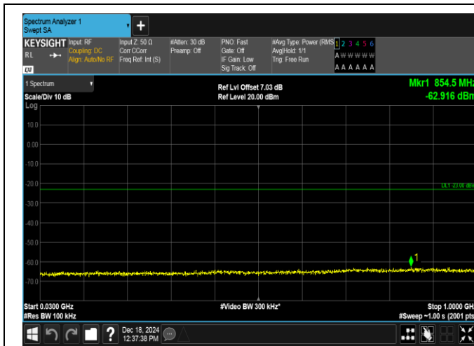
Band4-1.4MHz-QPSK-19957-6RB#0-30~1000-PASS
