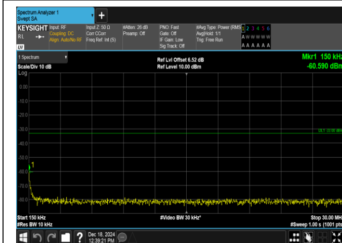
Band4-1.4MHz-QPSK-20175-1RB#0-0.15~30-PASS
