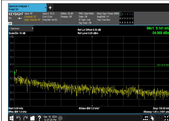
Band4-1.4MHz-QPSK-19957-6RB#0-0.009~0.15-PASS
