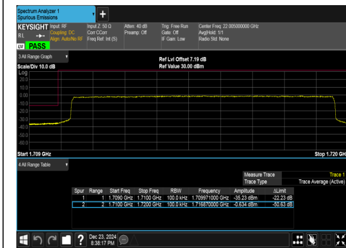
Band4-10MHz-16QAM-20000-50RB#0-PASS
