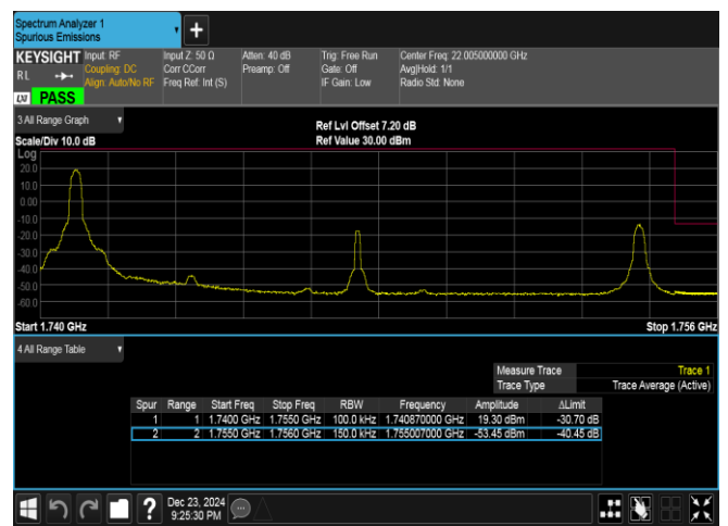
Band4-15MHz-QPSK-20325-1RB#0-PASS
