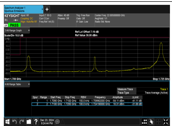
Band4-15MHz-16QAM-20025-1RB#74-PASS
