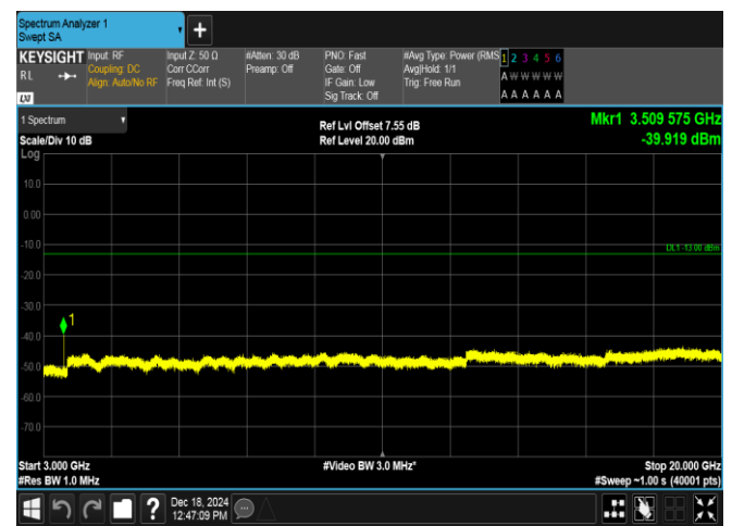
Band4-1.4MHz-QPSK-20393-1RB#5-3000~20000-PASS
