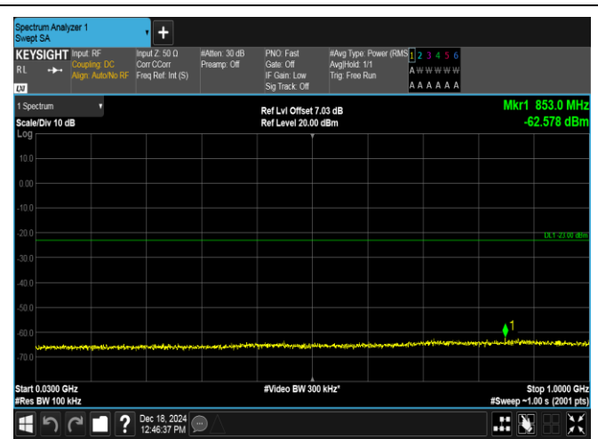
Band4-1.4MHz-QPSK-20393-1RB#5-30~1000-PASS
