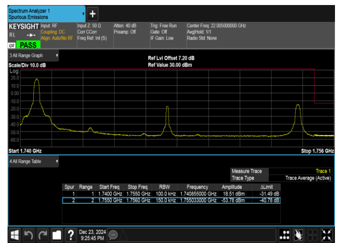
Band4-15MHz-16QAM-20325-1RB#0-PASS
