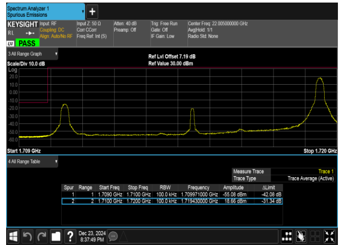
Band4-10MHz-16QAM-20000-1RB#49-PASS
