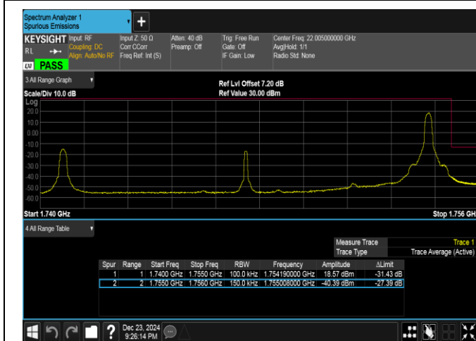
Band4-15MHz-16QAM-20325-1RB#74-PASS
