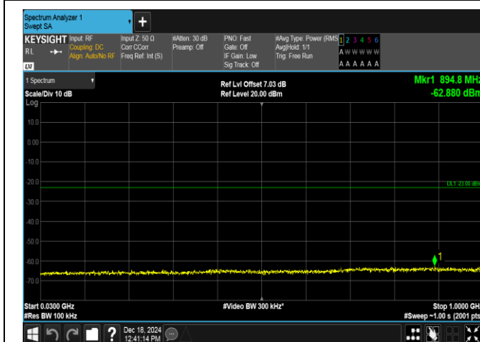
Band4-1.4MHz-QPSK-20175-1RB#5-30~1000-PASS
