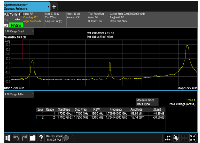
Band4-15MHz-QPSK-20025-1RB#74-PASS
