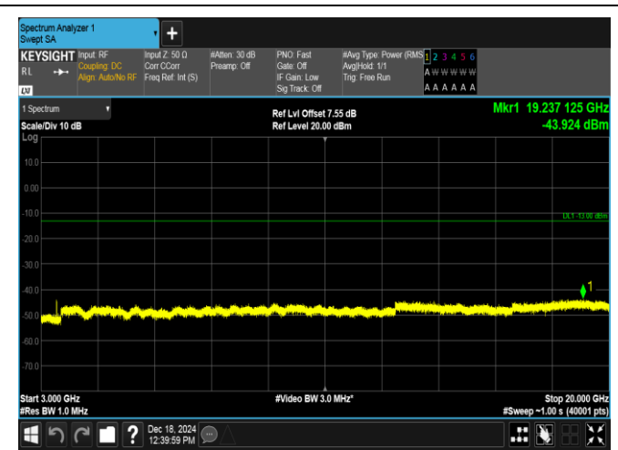
Band4-1.4MHz-QPSK-20175-1RB#0-3000~20000-PASS
