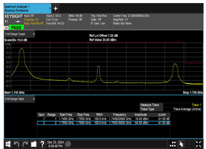
Band4-10MHz-16QAM-20350-1RB#0-PASS
