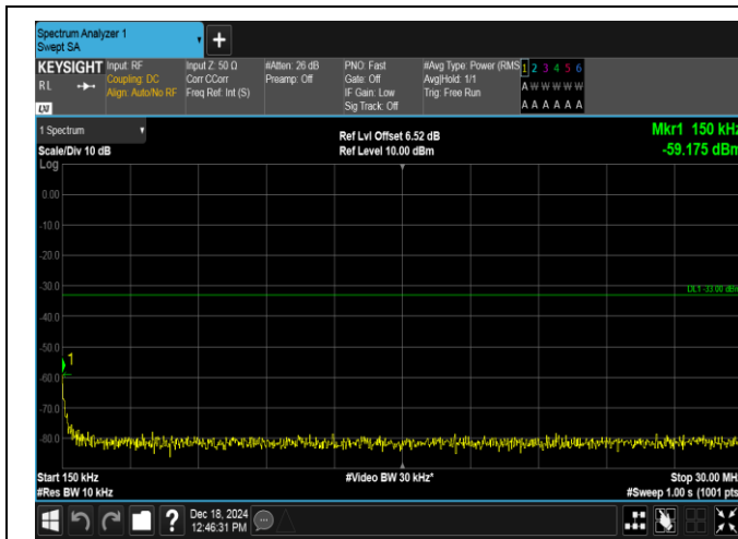
Band4-1.4MHz-QPSK-20393-1RB#5-0.15~30-PASS
