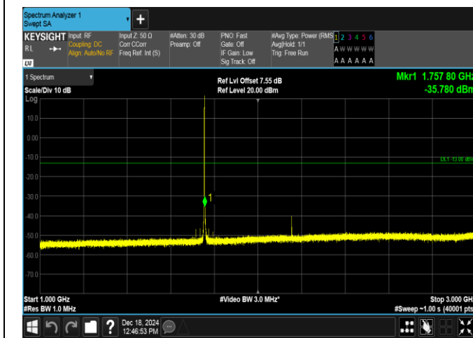
Band4-1.4MHz-QPSK-20393-1RB#5-1000~3000-PASS
