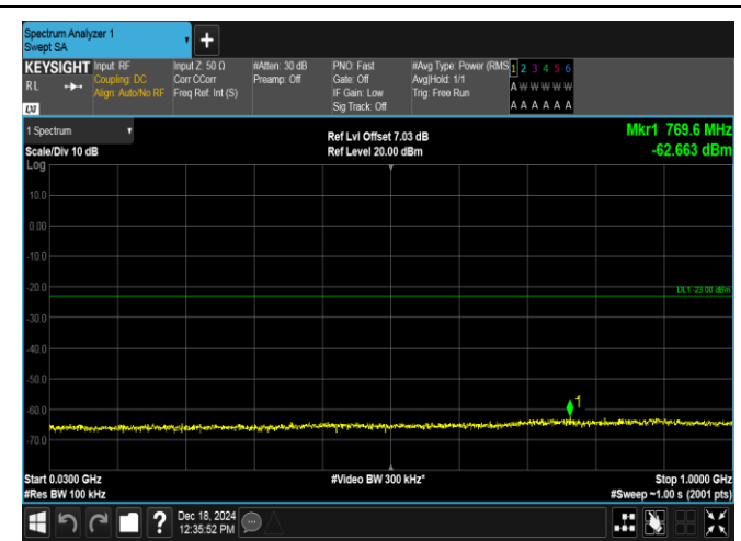
Band4-1.4MHz-QPSK-19957-1RB#5-30~1000-PASS
