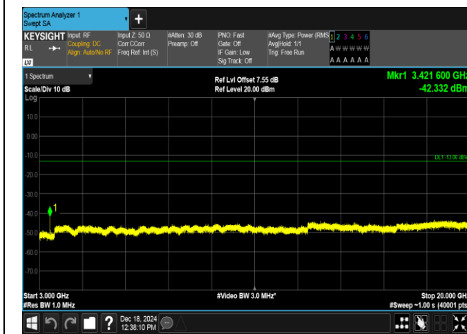
Band4-1.4MHz-QPSK-19957-6RB#0-3000~20000-PASS
