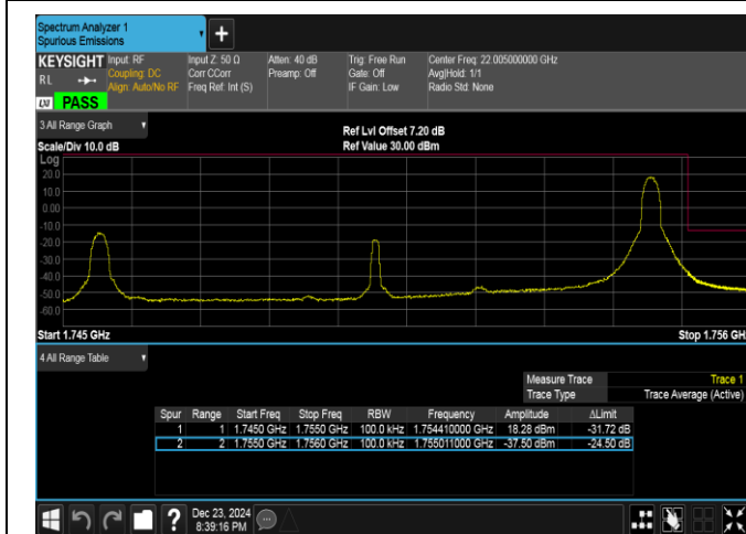
Band4-10MHz-16QAM-20350-1RB#49-PASS
