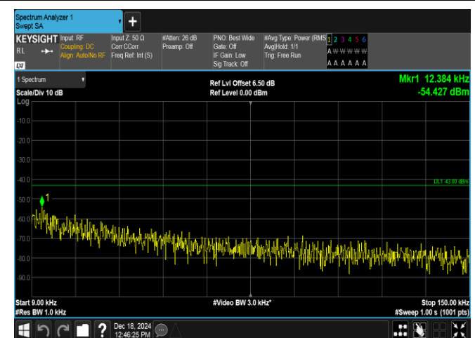
Band4-1.4MHz-QPSK-20393-1RB#5-0.009~0.15-PASS
