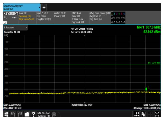
Band4-1.4MHz-QPSK-20175-1RB#0-30~1000-PASS
