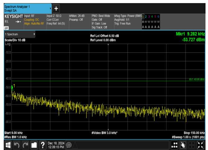
Band4-1.4MHz-QPSK-20175-1RB#0-0.009~0.15-PASS
