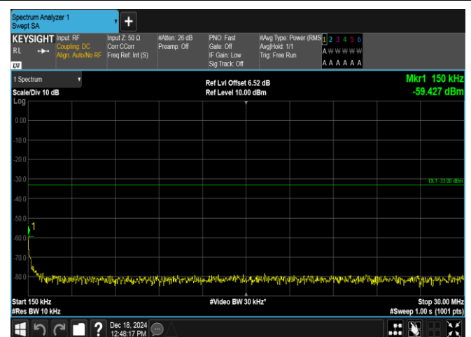
Band4-1.4MHz-QPSK-20393-6RB#0-0.15~30-PASS
