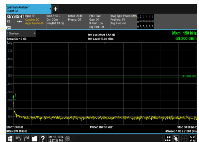
Band4-1.4MHz-QPSK-19957-6RB#0-0.15~30-PASS
