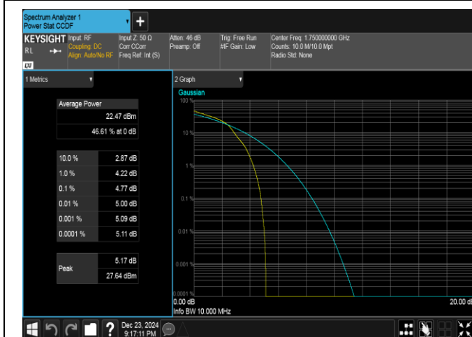
Band4-10MHz-16QAM-20350-1RB#0-PASS
