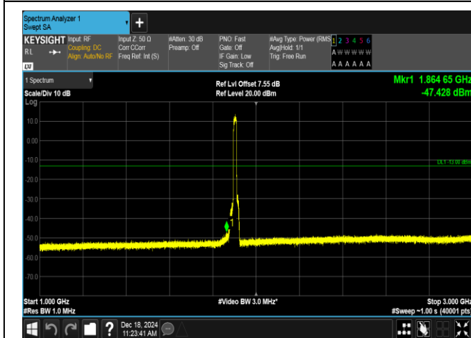
Band2-15MHz-16QAM-19125-75RB#0-1000~3000-PASS
