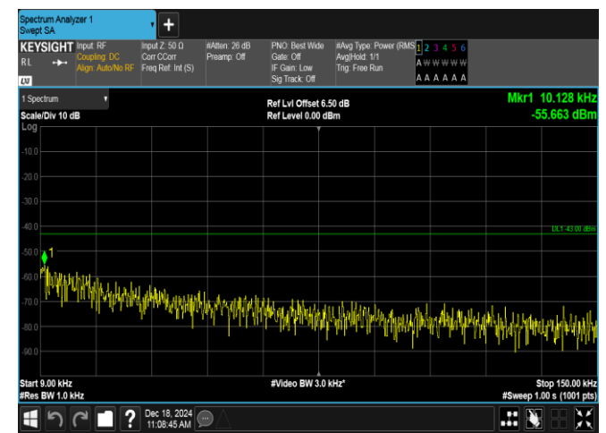
Band2-15MHz-16QAM-18675-1RB#0-0.009~0.15-PASS
