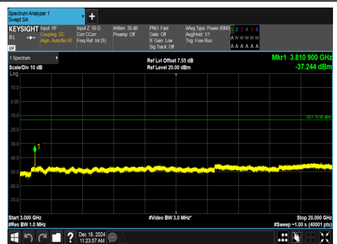
Band2-15MHz-16QAM-19125-75RB#0-3000~20000-PASS
