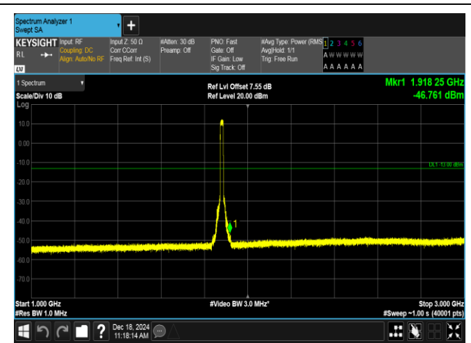
Band2-15MHz-16QAM-18900-75RB#0-1000~3000-PASS
