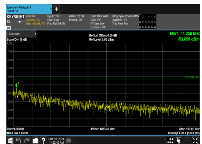
Band2-20MHz-QPSK-18700-1RB#99-0.009~0.15-PASS
