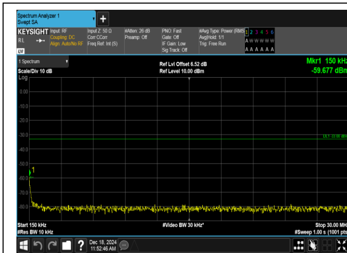
Band2-20MHz-QPSK-18700-1RB#99-0.15~30-PASS
