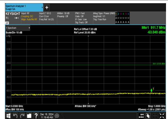
Band2-15MHz-16QAM-19125-1RB#0-30~1000-PASS
