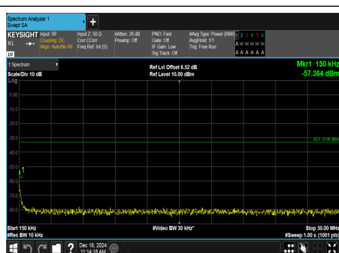
Band2-15MHz-16QAM-18900-1RB#0-0.15~30-PASS
