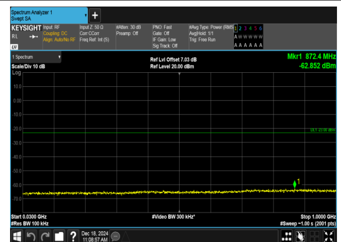
Band2-15MHz-16QAM-18675-1RB#0-30~1000-PASS
