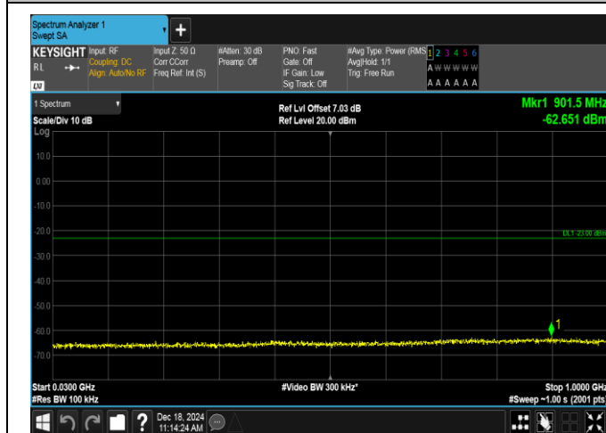
Band2-15MHz-16QAM-18900-1RB#0-30~1000-PASS
