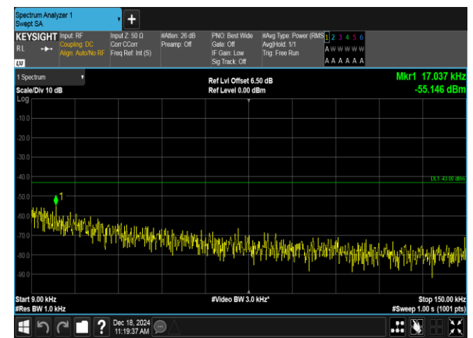
Band2-15MHz-16QAM-19125-1RB#0-0.009~0.15-PASS
