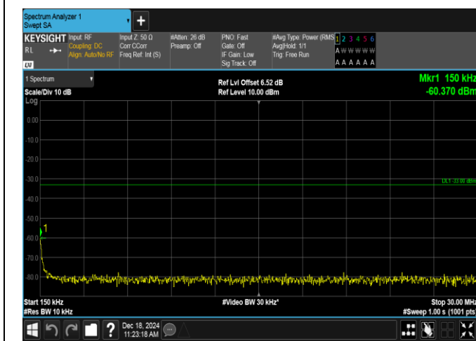
Band2-15MHz-16QAM-19125-75RB#0-0.15~30-PASS
