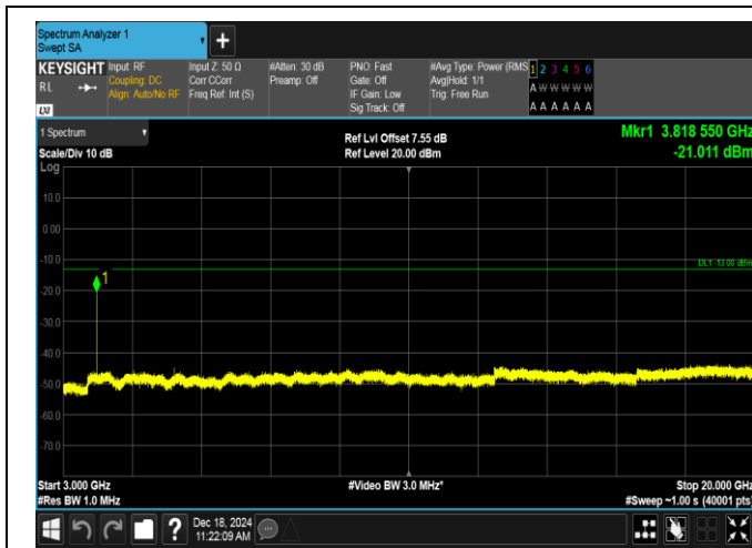
Band2-15MHz-16QAM-19125-1RB#74-3000~20000-PASS
