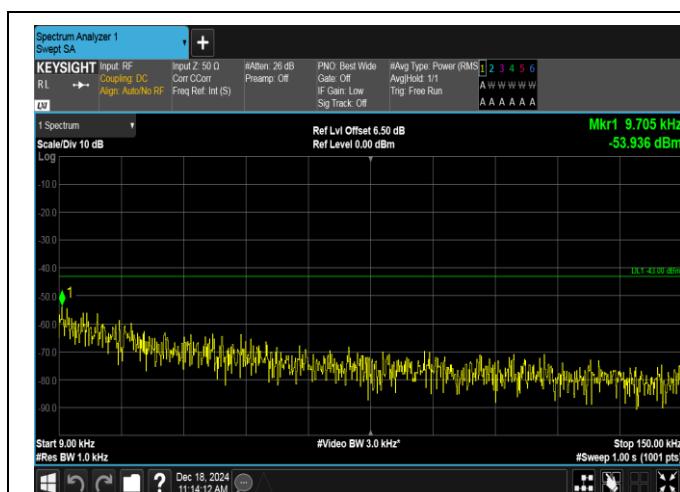
Band2-15MHz-16QAM-18900-1RB#0-0.009~0.15-PASS
