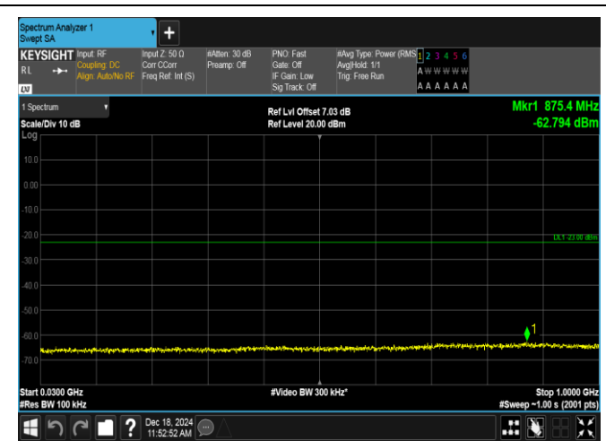
Band2-20MHz-QPSK-18700-1RB#99-30~1000-PASS
