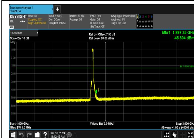
Band2-15MHz-16QAM-18675-75RB#0-1000~3000-PASS
