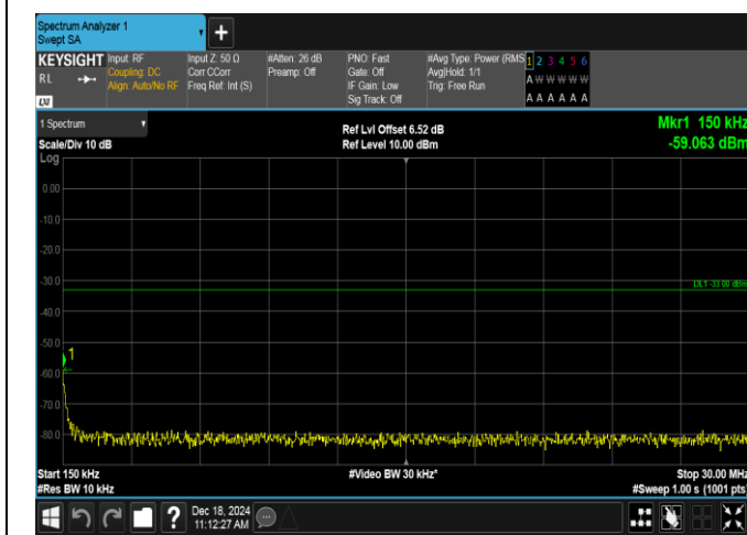
Band2-15MHz-16QAM-18675-75RB#0-0.15~30-PASS
