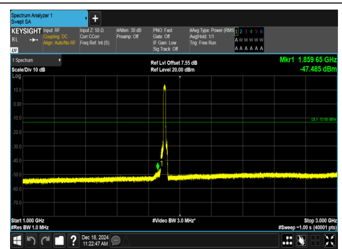
Band2-15MHz-QPSK-19125-75RB#0-1000~3000-PASS
