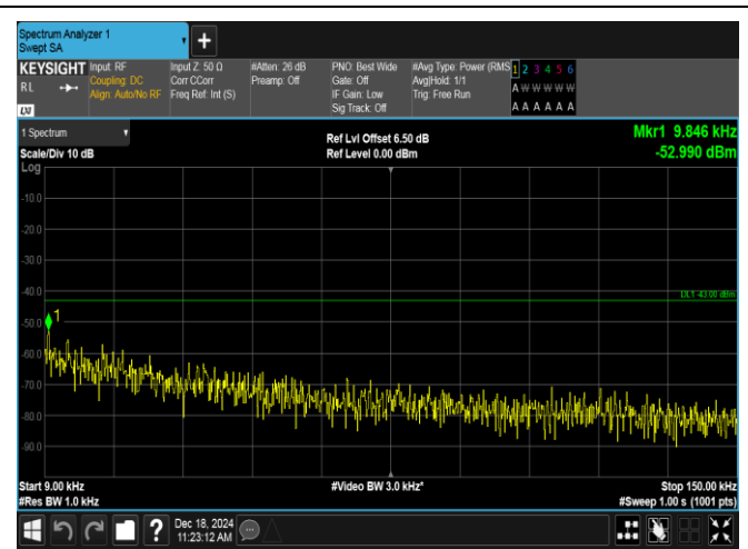
Band2-15MHz-16QAM-19125-75RB#0-0.009~0.15-PASS
