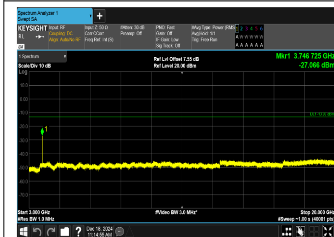
Band2-15MHz-16QAM-18900-1RB#0-3000~20000-PASS
