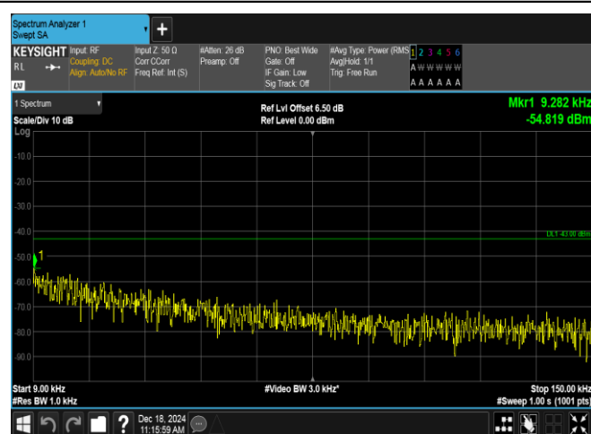
Band2-15MHz-16QAM-18900-1RB#74-0.009~0.15-PASS
