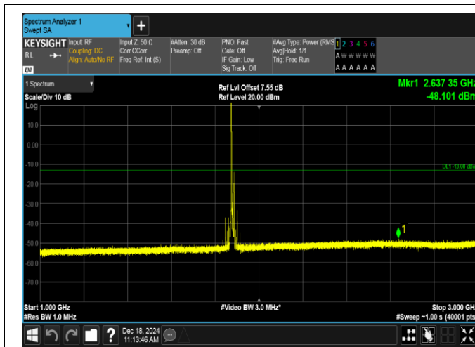
Band2-15MHz-QPSK-18900-1RB#0-1000~3000-PASS
