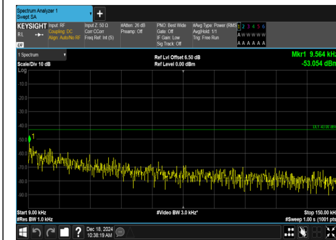
Band2-10MHz-16QAM-19150-1RB#49-0.009~0.15-PASS
