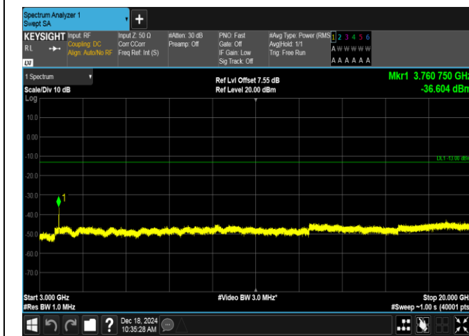
Band2-10MHz-16QAM-18900-50RB#0-3000~20000-PASS
