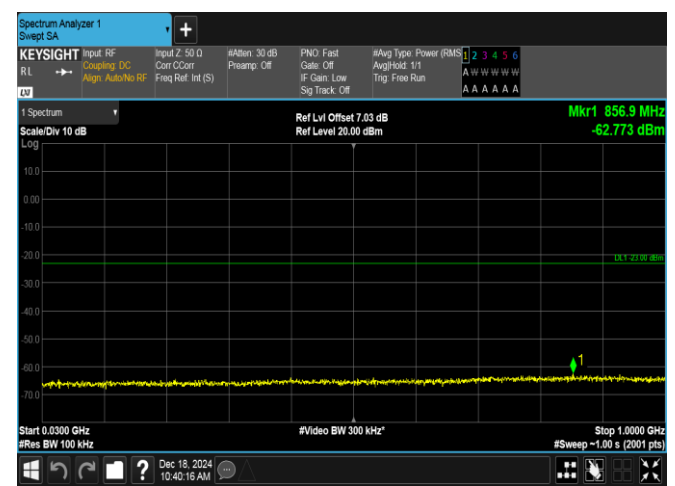
Band2-10MHz-16QAM-19150-50RB#0-30~1000-PASS
