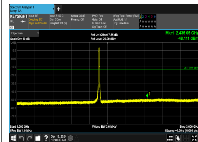
Band2-10MHz-16QAM-19150-50RB#0-1000~3000-PASS
