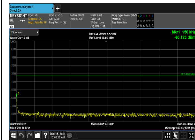
Band2-10MHz-16QAM-19150-50RB#0-0.15~30-PASS
