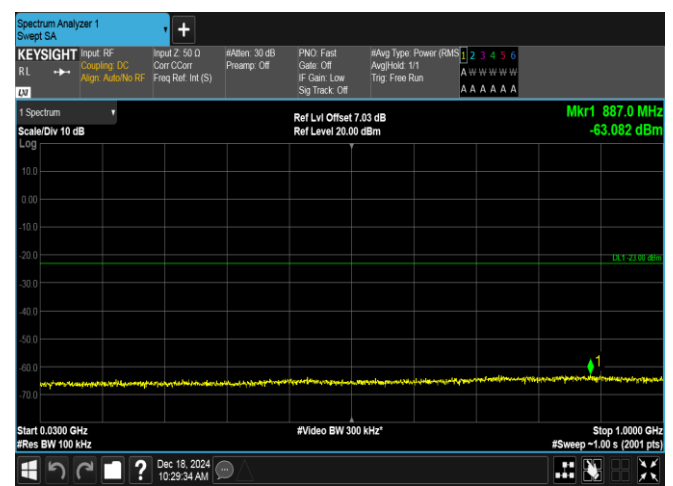
Band2-10MHz-16QAM-18650-50RB#0-30~1000-PASS
