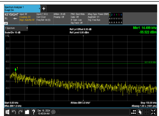
Band2-10MHz-16QAM-19150-50RB#0-0.009~0.15-PASS
