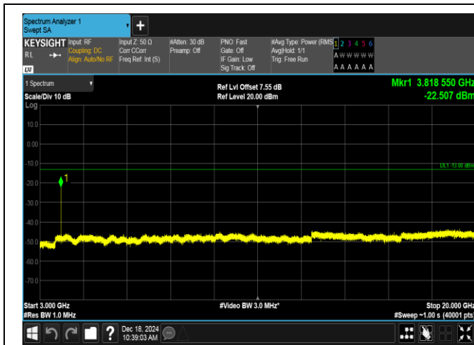
Band2-10MHz-16QAM-19150-1RB#49-3000~20000-PASS
