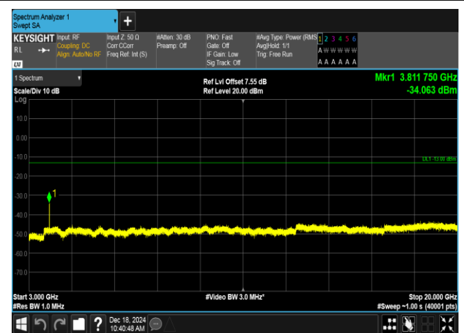
Band2-10MHz-16QAM-19150-50RB#0-3000~20000-PASS
