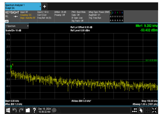
Band2-10MHz-16QAM-19150-1RB#0-0.009~0.15-PASS
