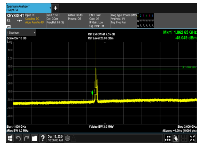
Band2-10MHz-QPSK-19150-1RB#0-1000~3000-PASS
