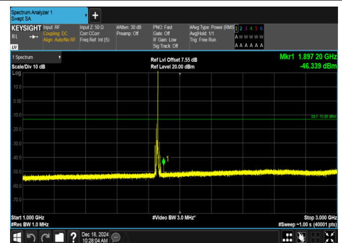
Band2-10MHz-16QAM-18650-1RB#49-1000~3000-PASS
