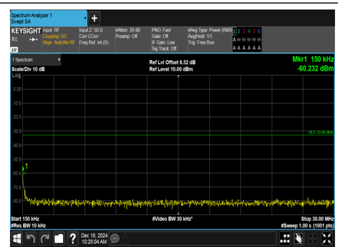
Band2-10MHz-QPSK-18650-1RB#0-0.15~30-PASS
