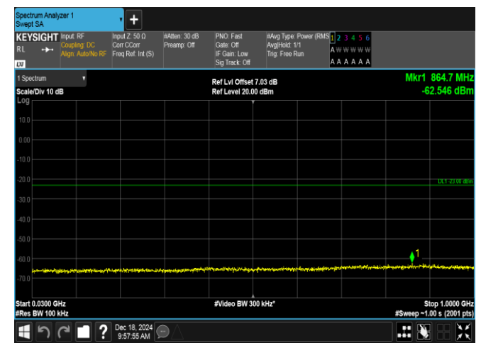
Band2-5MHz-16QAM-19175-25RB#0-30~1000-PASS
