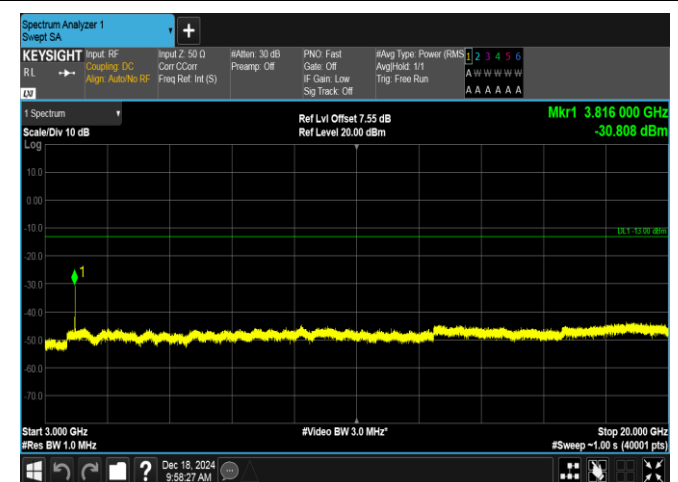
Band2-5MHz-16QAM-19175-25RB#0-3000~20000-PASS
