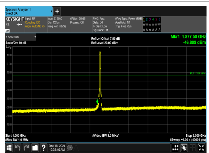
Band2-10MHz-QPSK-19150-50RB#0-1000~3000-PASS
