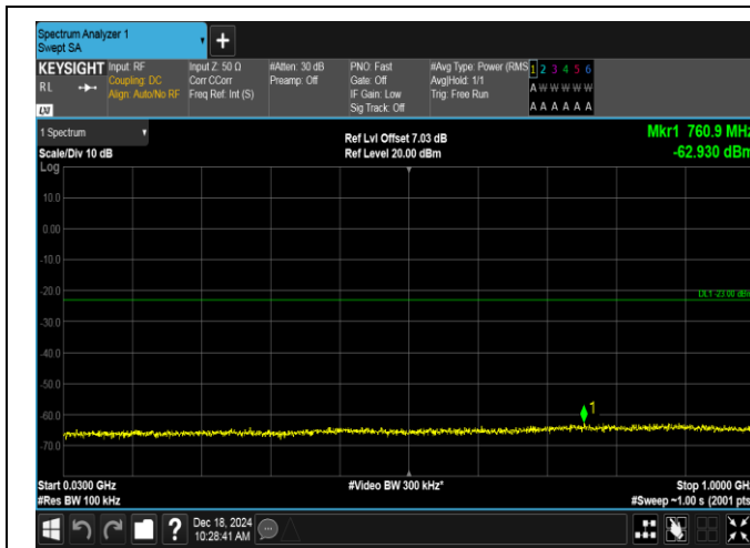
Band2-10MHz-QPSK-18650-50RB#0-30~1000-PASS
