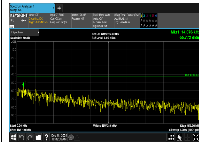
Band2-10MHz-QPSK-18900-1RB#49-0.009~0.15-PASS
