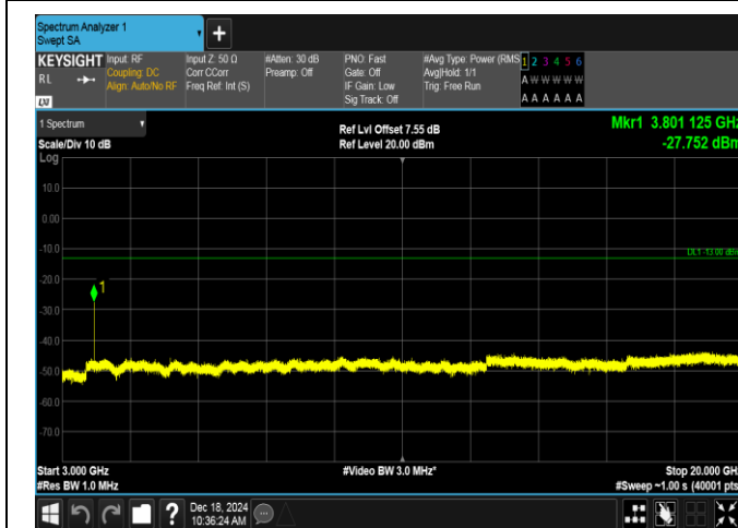
Band2-10MHz-QPSK-19150-1RB#0-3000~20000-PASS
