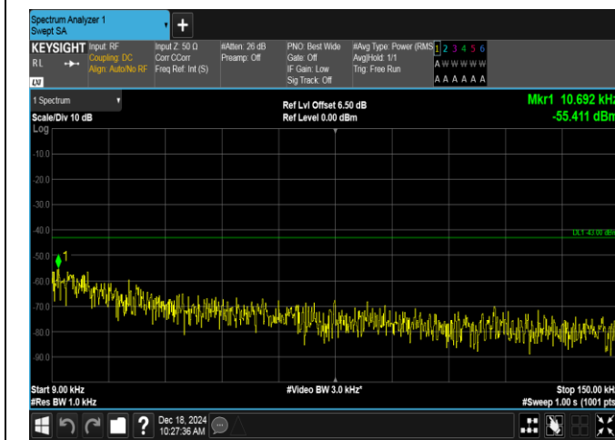
Band2-10MHz-16QAM-18650-1RB#49-0.009~0.15-PASS
