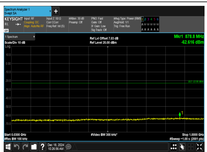
Band2-10MHz-QPSK-18650-1RB#49-30~1000-PASS
