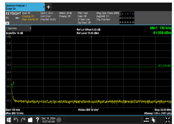
Band2-10MHz-16QAM-18650-1RB#49-0.15~30-PASS
