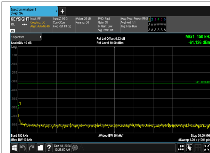
Band2-10MHz-QPSK-18650-1RB#49-0.15~30-PASS
