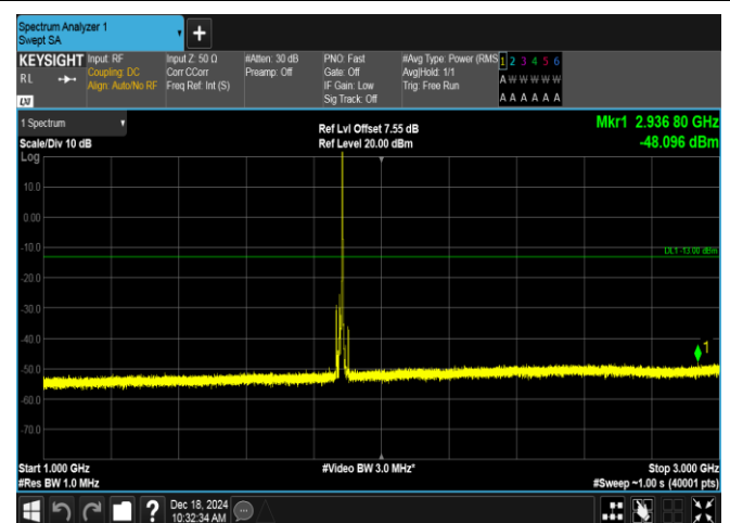
Band2-10MHz-QPSK-18900-1RB#49-1000~3000-PASS
