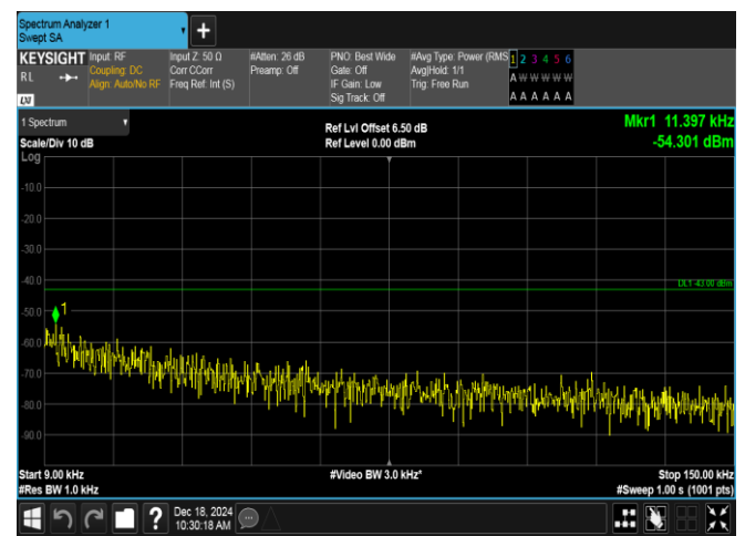
Band2-10MHz-QPSK-18900-1RB#0-0.009~0.15-PASS
