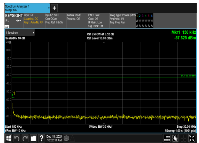
Band2-10MHz-QPSK-18900-1RB#49-0.15~30-PASS
