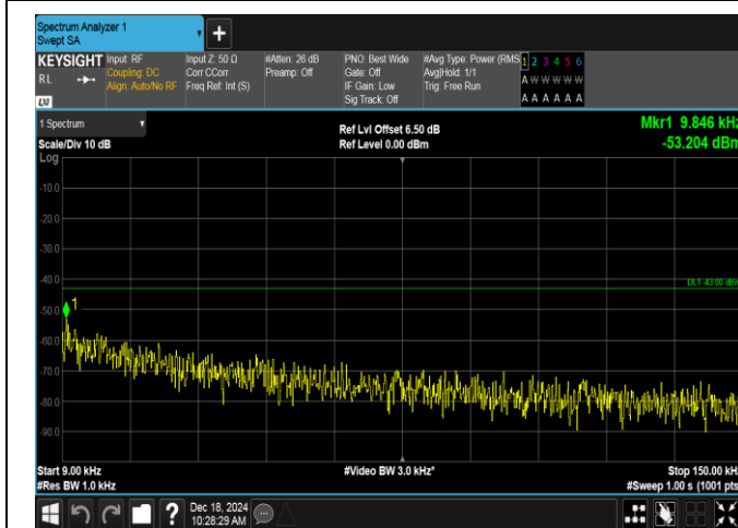
Band2-10MHz-QPSK-18650-50RB#0-0.009~0.15-PASS
