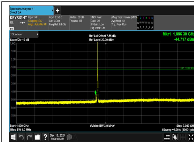
Band2-5MHz-16QAM-19175-1RB#0-1000~3000-PASS
