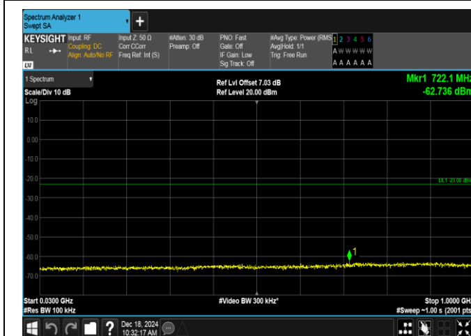
Band2-10MHz-QPSK-18900-1RB#49-30~1000-PASS
