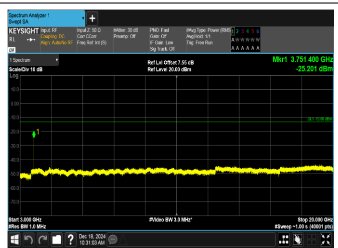
Band2-10MHz-QPSK-18900-1RB#0-3000~20000-PASS
