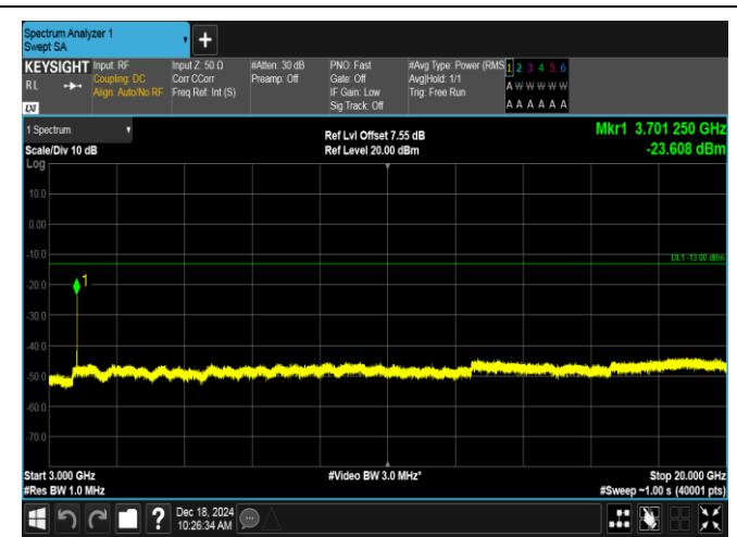
Band2-10MHz-16QAM-18650-1RB#0-3000~20000-PASS
