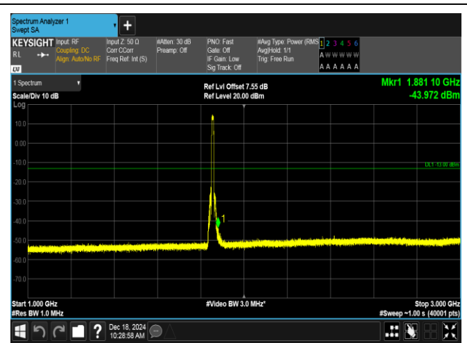
Band2-10MHz-QPSK-18650-50RB#0-1000~3000-PASS
