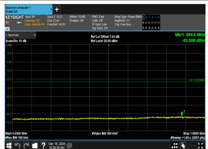
Band2-10MHz-QPSK-18900-1RB#0-30~1000-PASS
