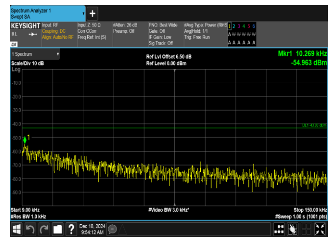
Band2-5MHz-16QAM-19175-1RB#0-0.009~0.15-PASS
