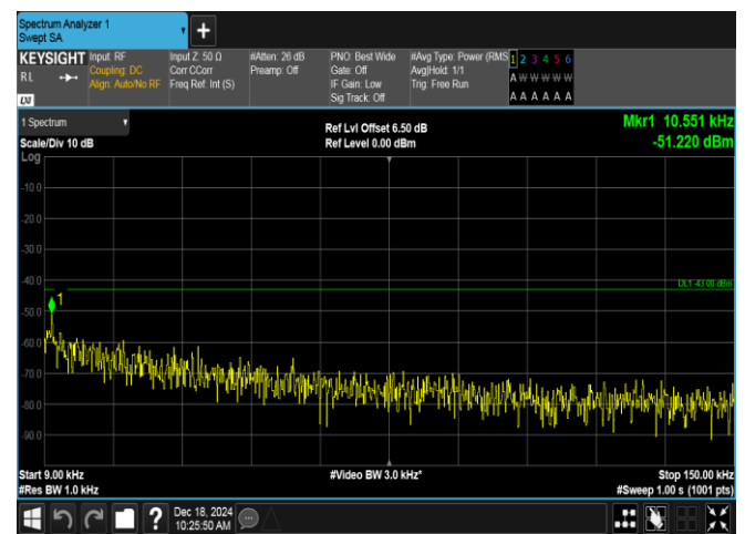
Band2-10MHz-16QAM-18650-1RB#0-0.009~0.15-PASS
