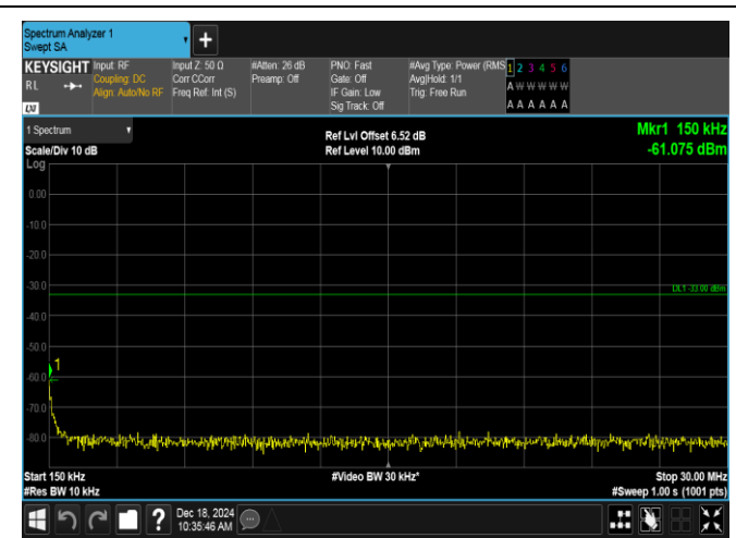
Band2-10MHz-QPSK-19150-1RB#0-0.15~30-PASS
