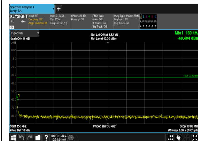
Band2-10MHz-QPSK-18900-1RB#0-0.15~30-PASS
