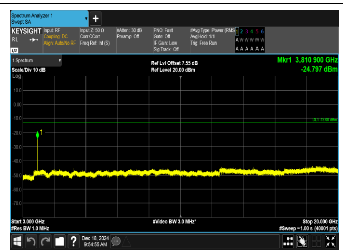
Band2-5MHz-16QAM-19175-1RB#0-3000~20000-PASS
