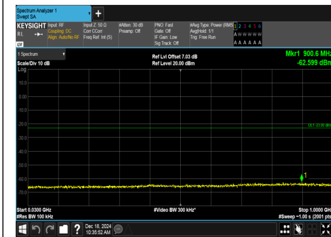
Band2-10MHz-QPSK-19150-1RB#0-30~1000-PASS
