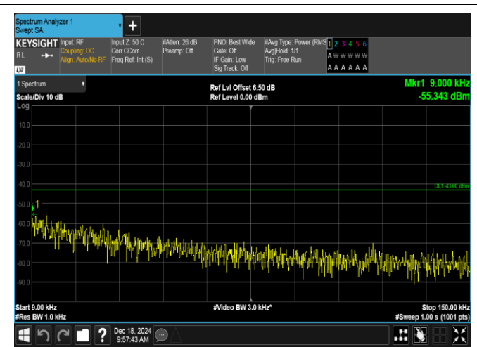
Band2-5MHz-16QAM-19175-25RB#0-0.009~0.15-PASS
