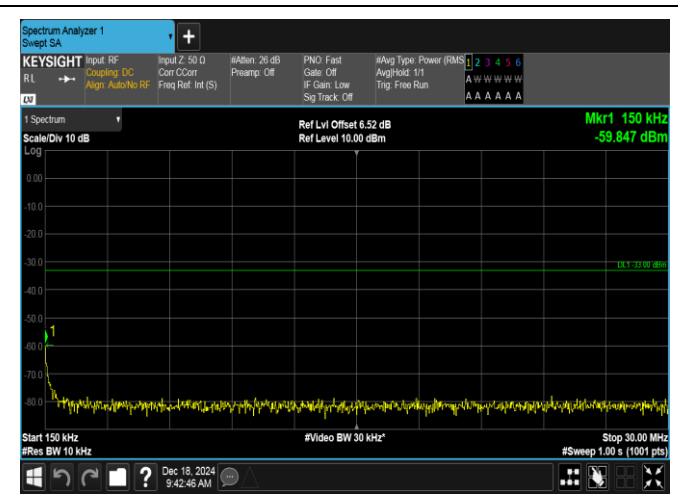
Band2-5MHz-QPSK-18625-1RB#0-0.15~30-PASS
