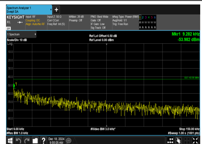
Band2-5MHz-QPSK-19175-1RB#24-0.009~0.15-PASS
