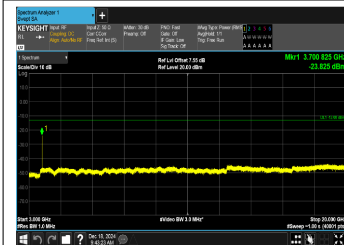
Band2-5MHz-QPSK-18625-1RB#0-3000~20000-PASS
