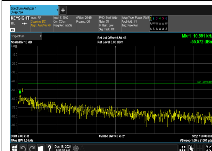
Band2-5MHz-QPSK-19175-25RB#0-0.009~0.15-PASS
