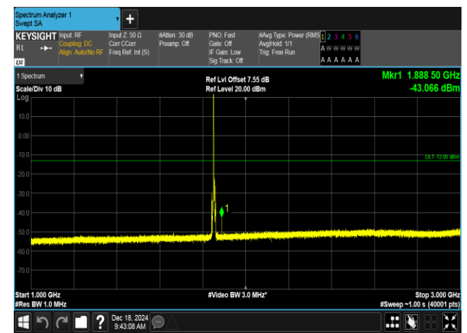
Band2-5MHz-QPSK-18625-1RB#0-1000~3000-PASS
