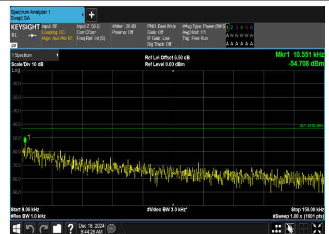
Band2-5MHz-QPSK-18625-1RB#24-0.009~0.15-PASS
