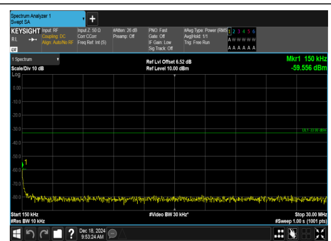
Band2-5MHz-QPSK-19175-1RB#0-0.15~30-PASS
