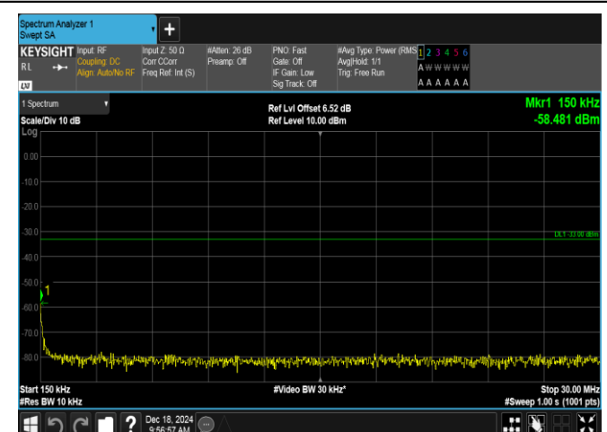
Band2-5MHz-QPSK-19175-25RB#0-0.15~30-PASS
