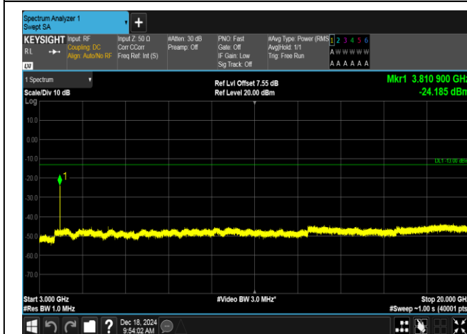
Band2-5MHz-QPSK-19175-1RB#0-3000~20000-PASS
