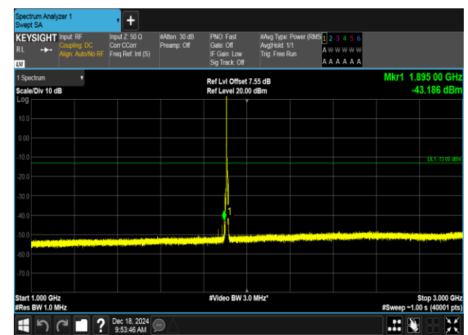
Band2-5MHz-QPSK-19175-1RB#0-1000~3000-PASS
