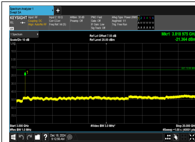
Band2-3MHz-16QAM-19185-1RB#14-3000~20000-PASS
