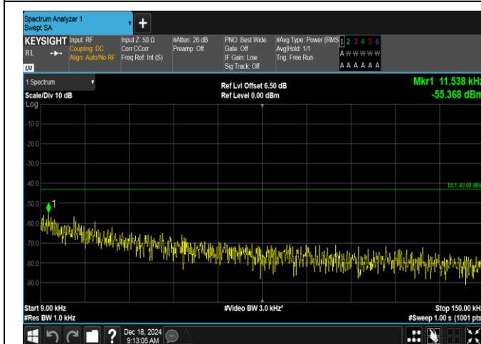
Band2-3MHz-QPSK-19185-15RB#0-0.009~0.15-PASS
