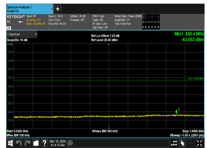
Band2-3MHz-16QAM-19185-15RB#0-30~1000-PASS
