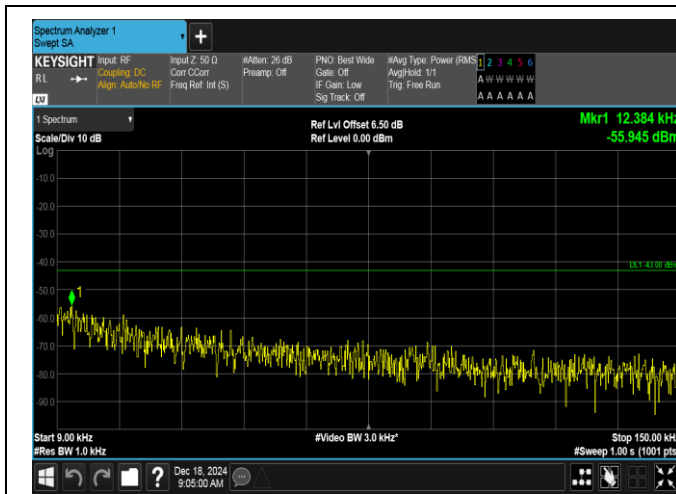
Band2-3MHz-16QAM-18900-1RB#0-0.009~0.15-PASS
