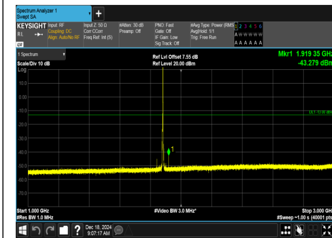
Band2-3MHz-16QAM-18900-1RB#14-1000~3000-PASS
