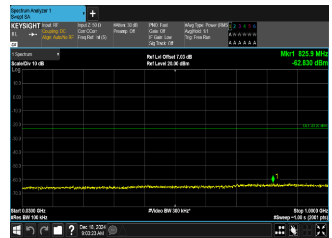
Band2-3MHz-16QAM-18615-15RB#0-30~1000-PASS
