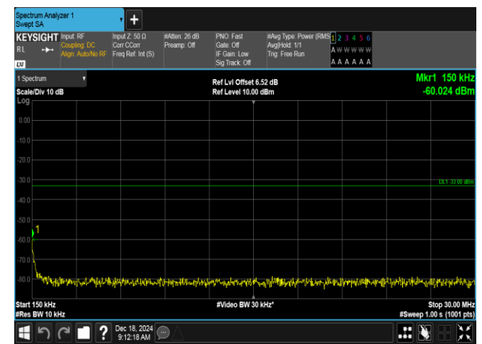
Band2-3MHz-16QAM-19185-1RB#14-0.15~30-PASS
