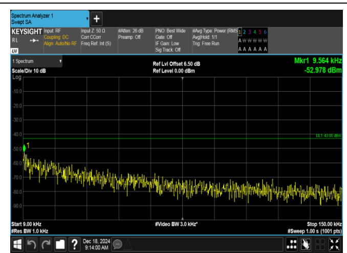
Band2-3MHz-16QAM-19185-15RB#0-0.009~0.15-PASS
