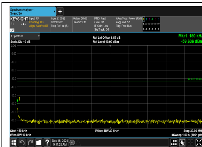
Band2-3MHz-QPSK-19185-1RB#14-0.15~30-PASS
