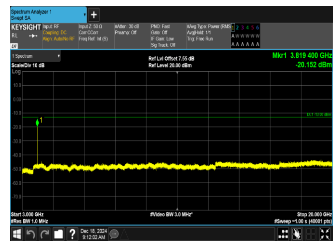
Band2-3MHz-QPSK-19185-1RB#14-3000~20000-PASS
