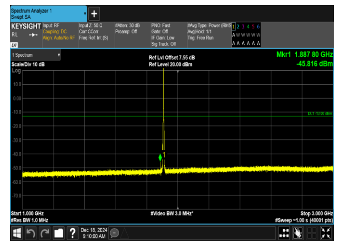
Band2-3MHz-QPSK-19185-1RB#0-1000~3000-PASS
