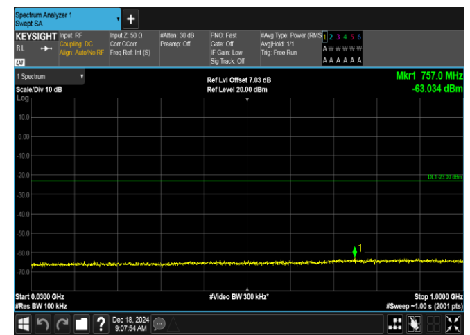
Band2-3MHz-QPSK-18900-15RB#0-30~1000-PASS
