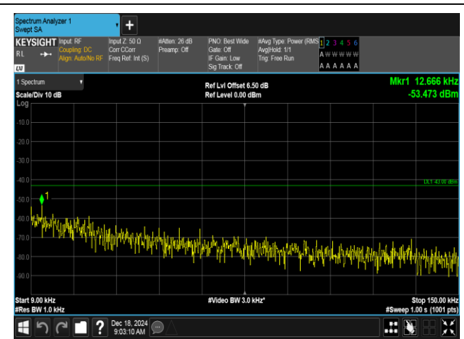
Band2-3MHz-16QAM-18615-15RB#0-0.009~0.15-PASS
