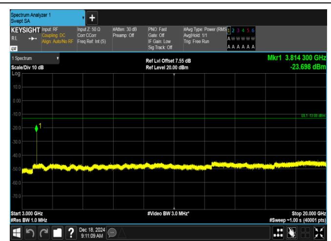
Band2-3MHz-16QAM-19185-1RB#0-3000~20000-PASS
