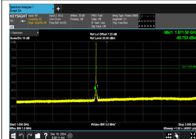
Band2-3MHz-QPSK-18900-15RB#0-1000~3000-PASS
