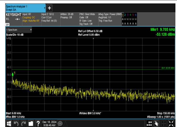
Band2-3MHz-16QAM-18900-1RB#14-0.009~0.15-PASS
