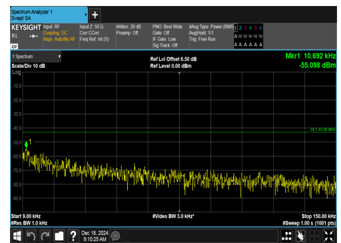
Band2-3MHz-16QAM-19185-1RB#0-0.009~0.15-PASS
