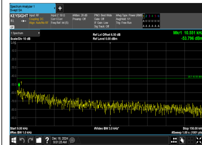
Band2-3MHz-16QAM-18615-1RB#14-0.009~0.15-PASS
