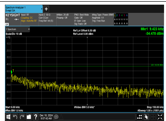
Band2-3MHz-QPSK-18900-15RB#0-0.009~0.15-PASS
