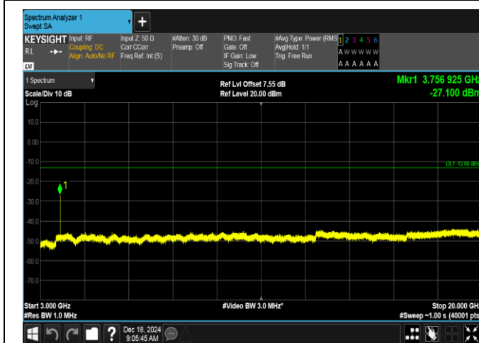
Band2-3MHz-16QAM-18900-1RB#0-3000~20000-PASS
