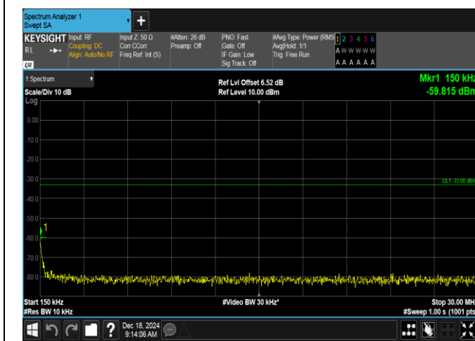
Band2-3MHz-16QAM-19185-15RB#0-0.15~30-PASS
