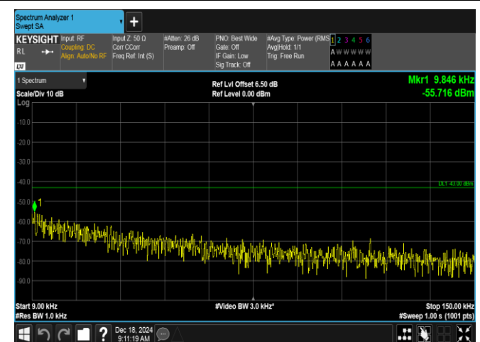
Band2-3MHz-QPSK-19185-1RB#14-0.009~0.15-PASS
