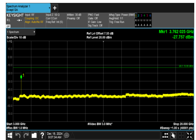
Band2-3MHz-16QAM-18900-1RB#14-3000~20000-PASS
