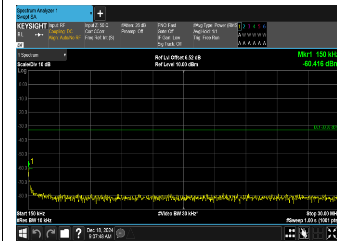
Band2-3MHz-QPSK-18900-15RB#0-0.15~30-PASS
