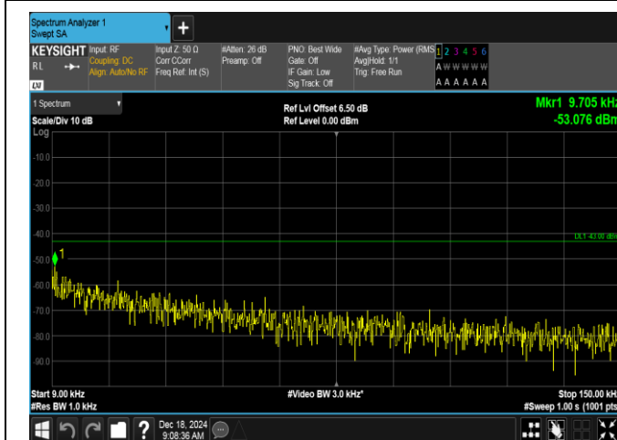
Band2-3MHz-16QAM-18900-15RB#0-0.009~0.15-PASS
