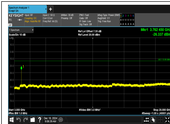
Band2-3MHz-QPSK-18900-1RB#14-3000~20000-PASS
