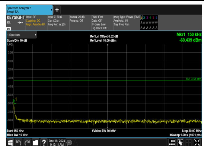
Band2-3MHz-QPSK-19185-15RB#0-0.15~30-PASS
