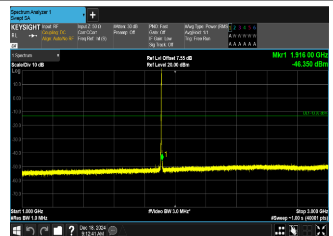
Band2-3MHz-16QAM-19185-1RB#14-1000~3000-PASS
