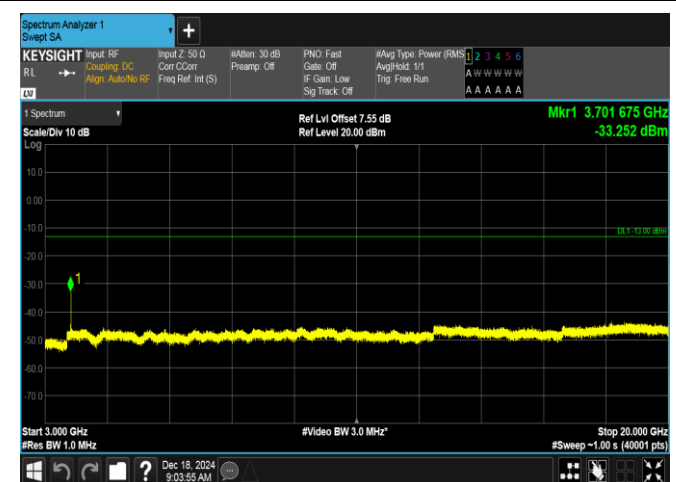
Band2-3MHz-16QAM-18615-15RB#0-3000~20000-PASS
