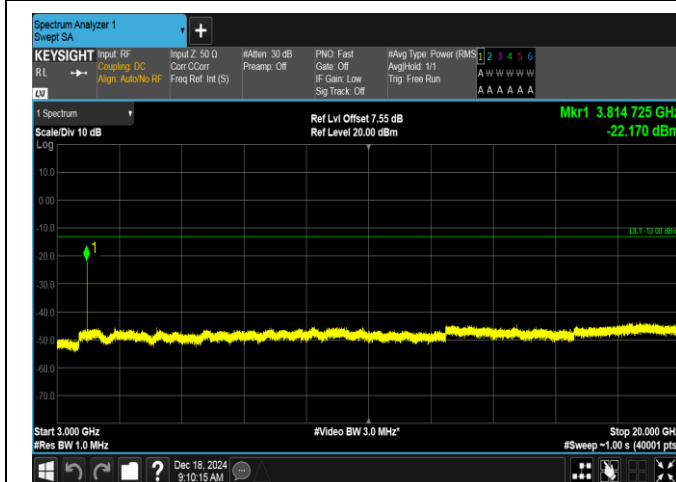
Band2-3MHz-QPSK-19185-1RB#0-3000~20000-PASS
