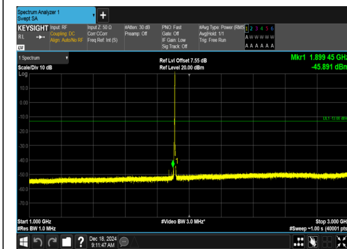
Band2-3MHz-QPSK-19185-1RB#14-1000~3000-PASS
