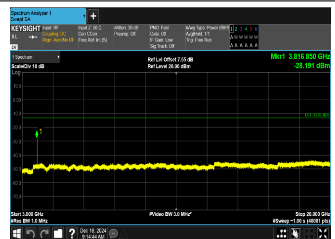
Band2-3MHz-16QAM-19185-15RB#0-3000~20000-PASS
