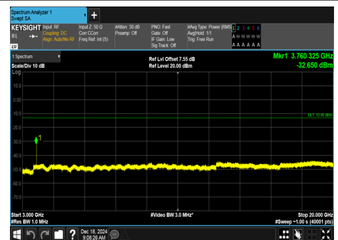
Band2-3MHz-QPSK-18900-15RB#0-3000~20000-PASS
