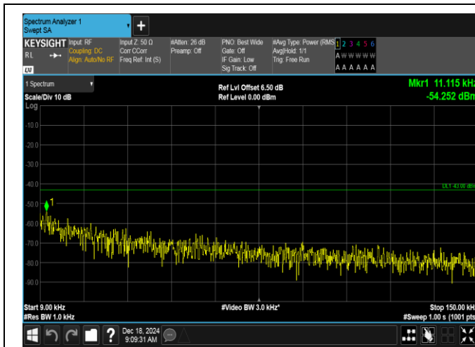
Band2-3MHz-QPSK-19185-1RB#0-0.009~0.15-PASS
