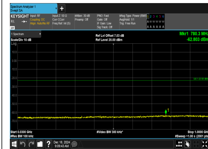
Band2-3MHz-QPSK-19185-1RB#0-30~1000-PASS
