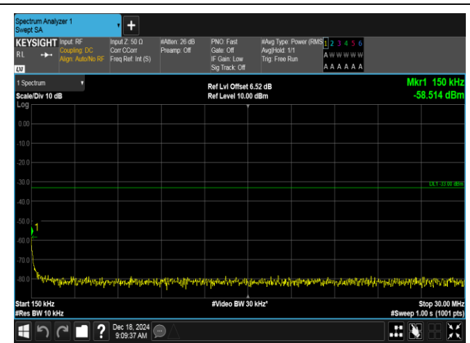
Band2-3MHz-QPSK-19185-1RB#0-0.15~30-PASS
