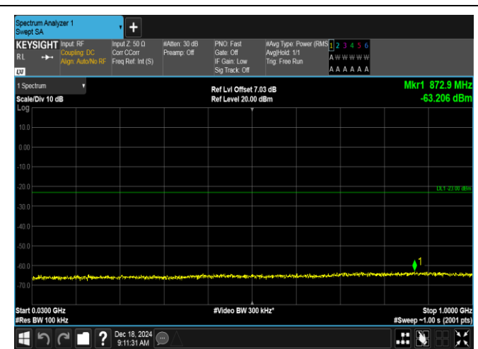
Band2-3MHz-QPSK-19185-1RB#14-30~1000-PASS
