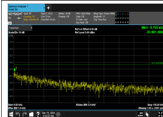
Band2-1.4MHz-16QAM-18900-6RB#0-0.009~0.15-PASS
