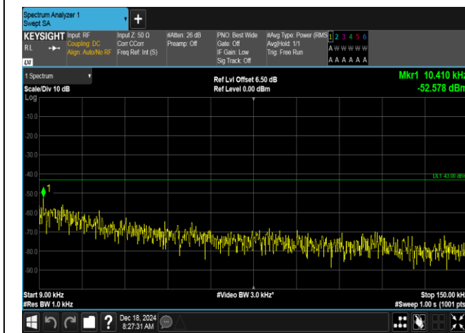
Band2-1.4MHz-16QAM-19193-1RB#5-0.009~0.15-PASS
