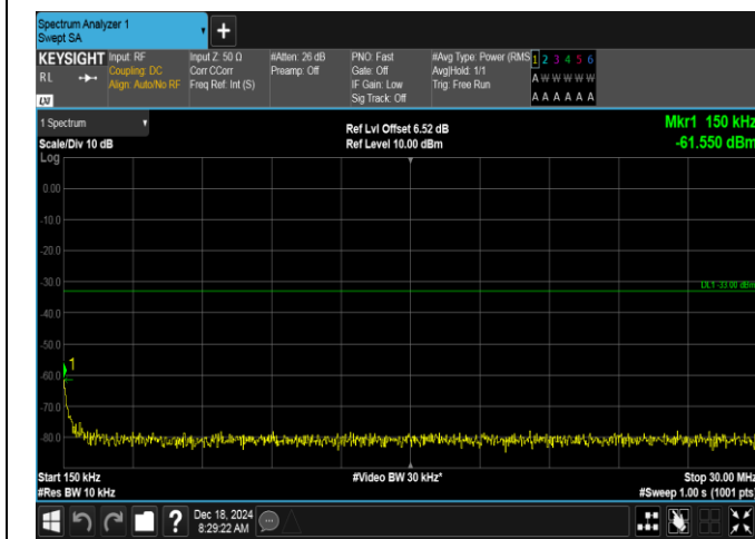
Band2-1.4MHz-16QAM-19193-6RB#0-0.15~30-PASS
