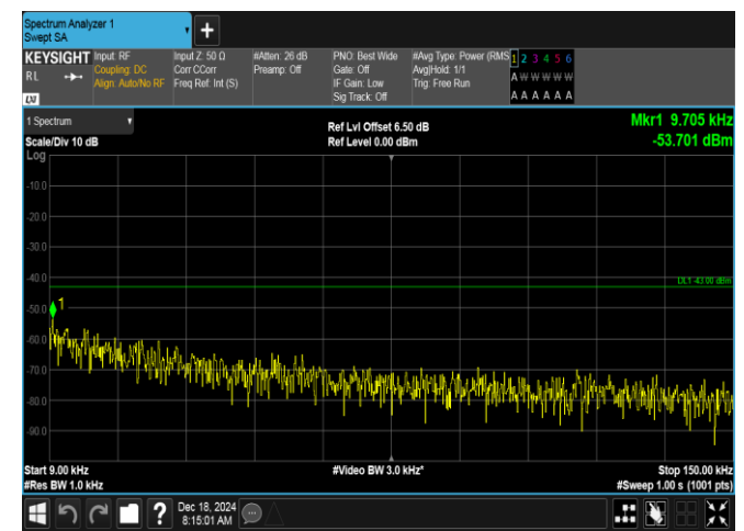
Band2-1.4MHz-16QAM-18607-1RB#0-0.009~0.15-PASS
