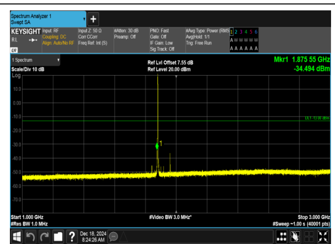
Band2-1.4MHz-16QAM-18900-6RB#0-1000~3000-PASS
