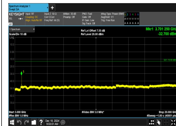
Band2-3MHz-QPSK-18615-15RB#0-3000~20000-PASS
