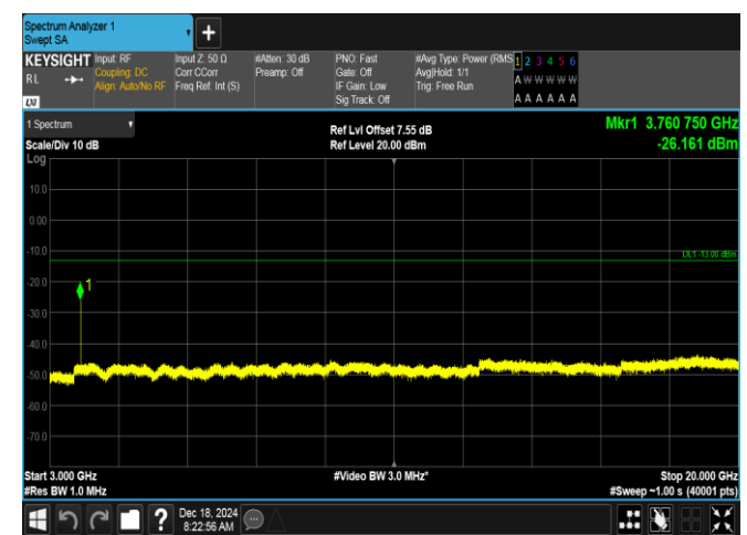
Band2-1.4MHz-16QAM-18900-1RB#5-3000~20000-PASS
