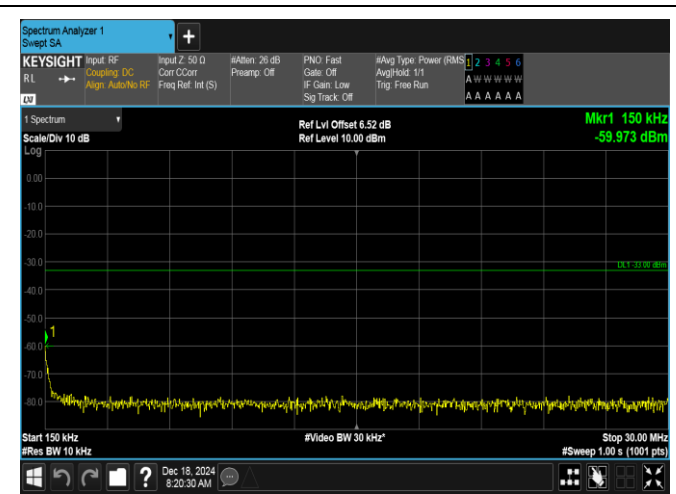
Band2-1.4MHz-16QAM-18900-1RB#0-0.15~30-PASS
