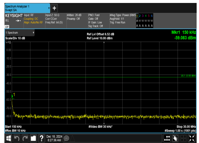
Band2-1.4MHz-16QAM-19193-1RB#5-0.15~30-PASS
