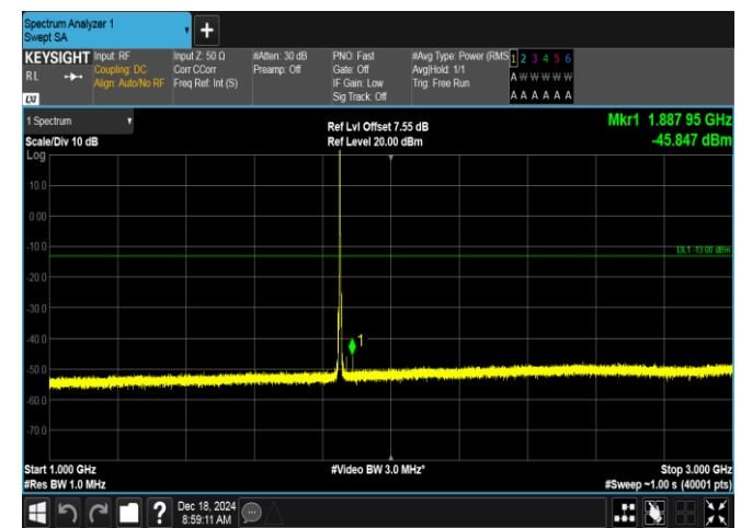
Band2-3MHz-QPSK-18615-1RB#0-1000~3000-PASS
