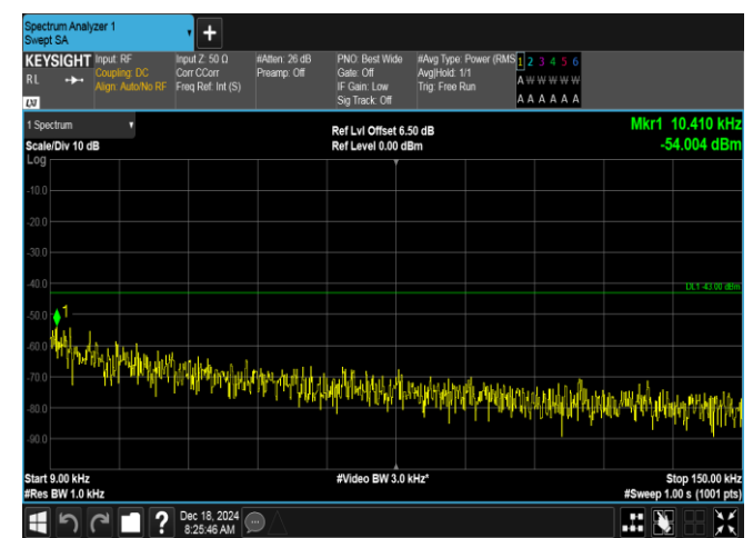
Band2-1.4MHz-16QAM-19193-1RB#0-0.009~0.15-PASS
