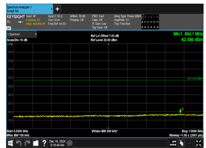
Band2-1.4MHz-16QAM-18607-6RB#0-30~1000-PASS
