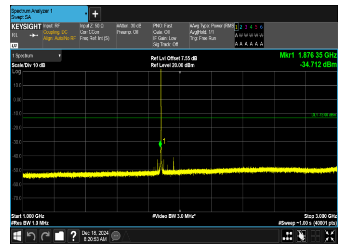
Band2-1.4MHz-16QAM-18900-1RB#0-1000~3000-PASS
