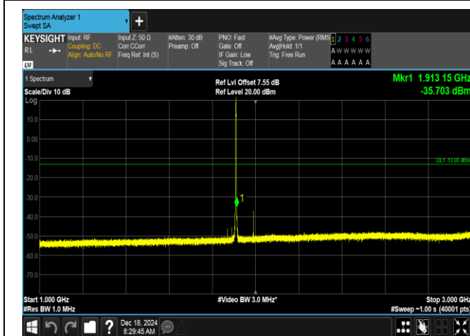
Band2-1.4MHz-16QAM-19193-6RB#0-1000~3000-PASS
