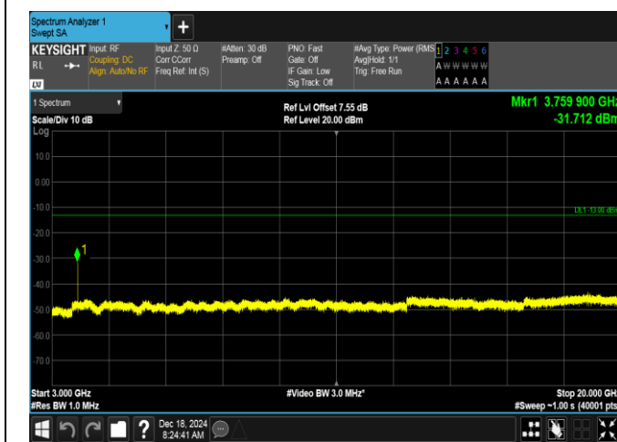
Band2-1.4MHz-16QAM-18900-6RB#0-3000~20000-PASS
