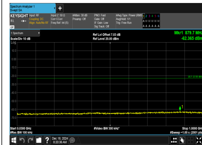
Band2-1.4MHz-16QAM-18900-1RB#0-30~1000-PASS
