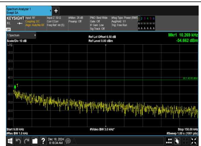
Band2-1.4MHz-16QAM-18607-6RB#0-0.009~0.15-PASS
