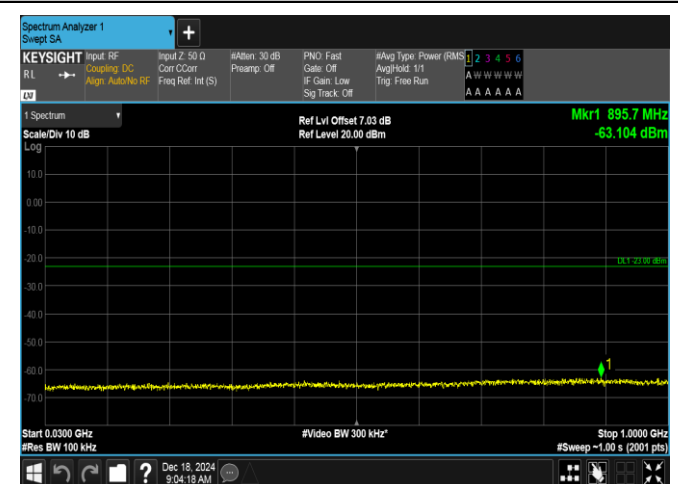
Band2-3MHz-QPSK-18900-1RB#0-30~1000-PASS
