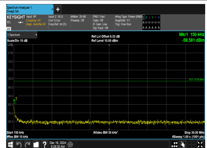
Band2-1.4MHz-QPSK-19193-6RB#0-0.15~30-PASS
