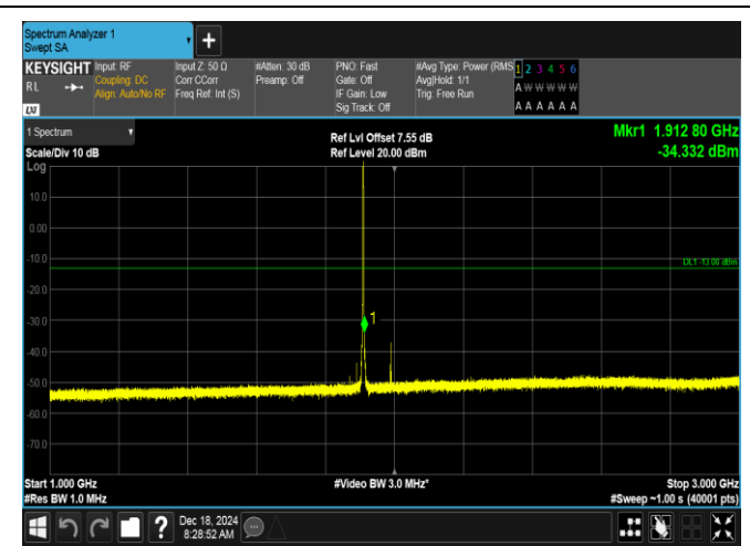
Band2-1.4MHz-QPSK-19193-6RB#0-1000~3000-PASS
