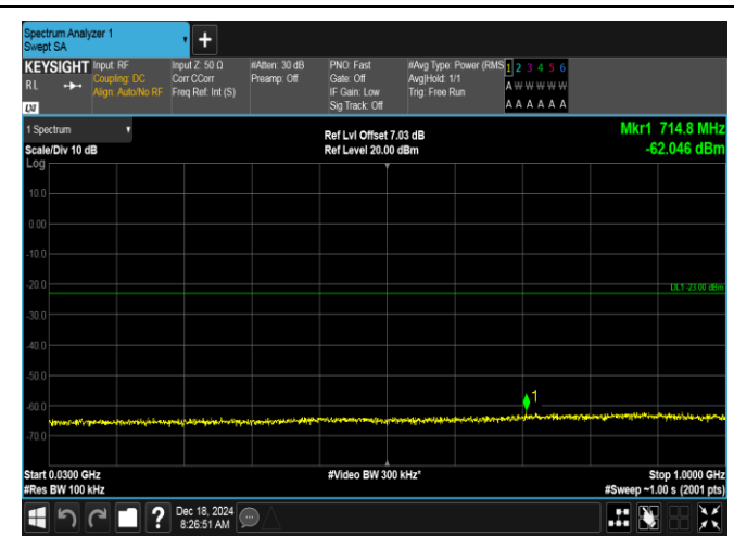
Band2-1.4MHz-QPSK-19193-1RB#5-30~1000-PASS
