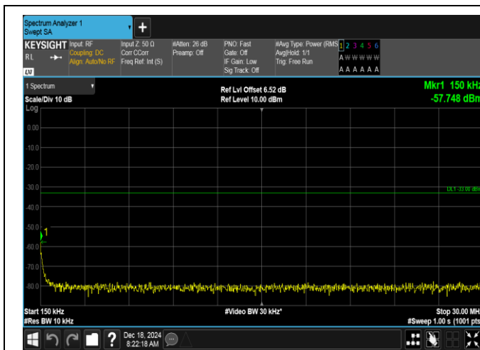
Band2-1.4MHz-16QAM-18900-1RB#5-0.15~30-PASS
