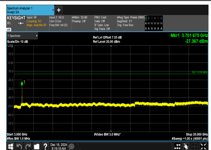
Band2-1.4MHz-16QAM-18607-6RB#0-3000~20000-PASS
