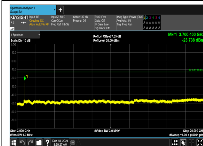
Band2-3MHz-QPSK-18615-1RB#0-3000~20000-PASS
