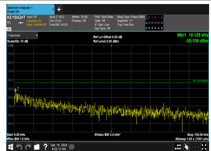
Band2-1.4MHz-16QAM-18900-1RB#5-0.009~0.15-PASS
