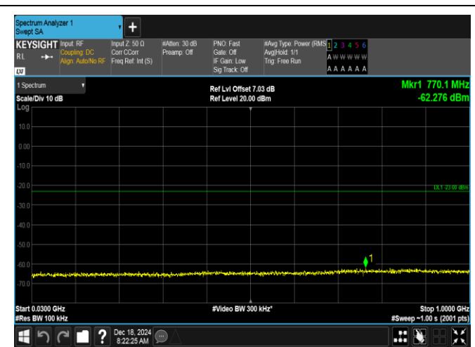
Band2-1.4MHz-16QAM-18900-1RB#5-30~1000-PASS
