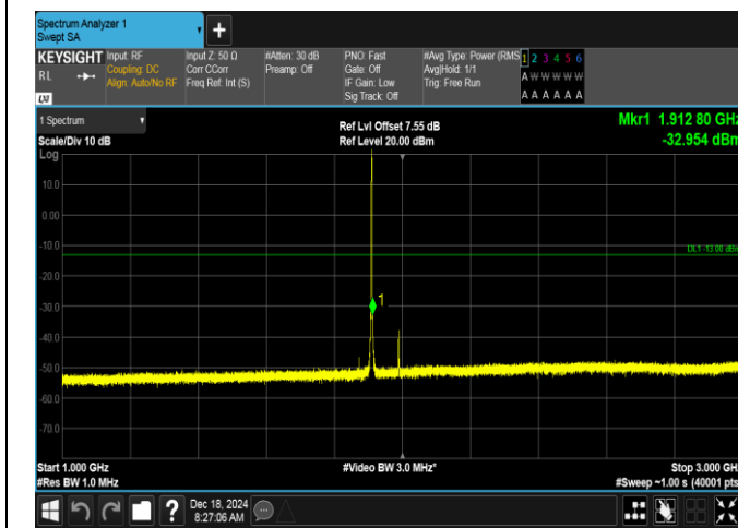
Band2-1.4MHz-QPSK-19193-1RB#5-1000~3000-PASS
