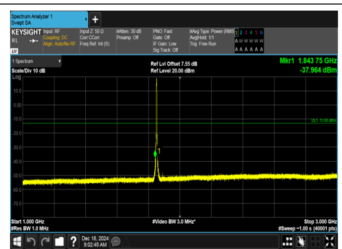
Band2-3MHz-QPSK-18615-15RB#0-1000~3000-PASS
