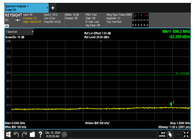
Band2-1.4MHz-16QAM-19193-6RB#0-30~1000-PASS
