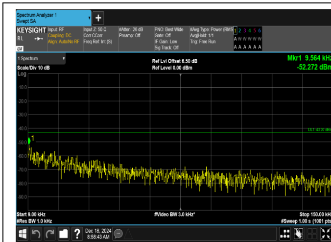
Band2-3MHz-QPSK-18615-1RB#0-0.009~0.15-PASS
