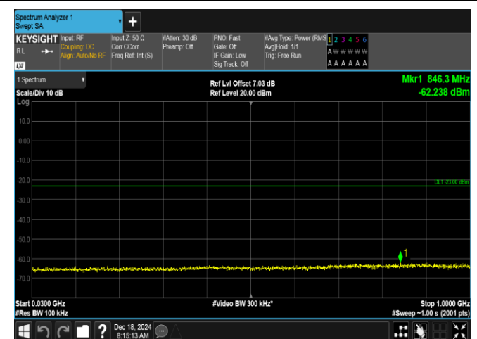
Band2-1.4MHz-16QAM-18607-1RB#0-30~1000-PASS
