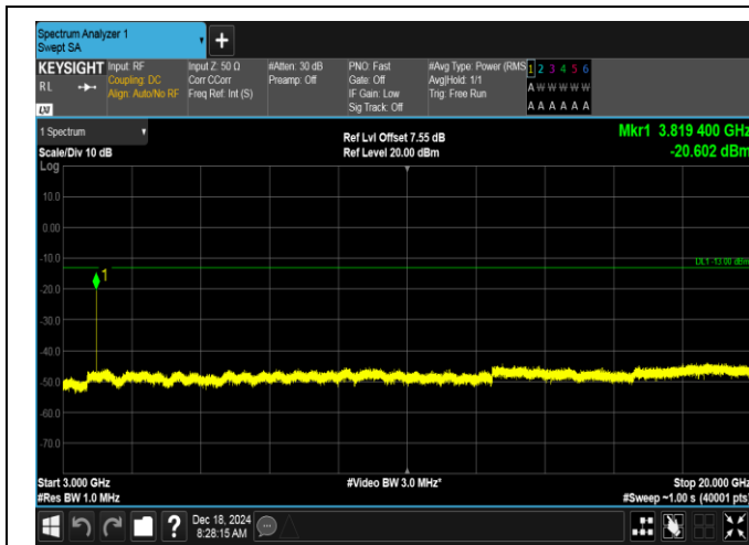
Band2-1.4MHz-16QAM-19193-1RB#5-3000~20000-PASS
