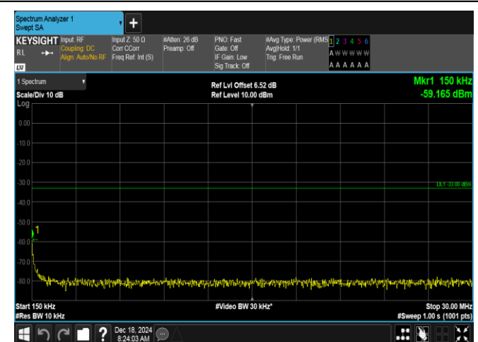
Band2-1.4MHz-16QAM-18900-6RB#0-0.15~30-PASS
