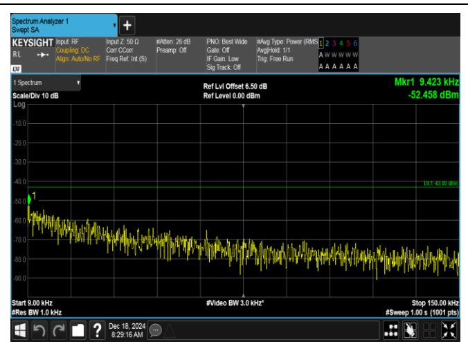
Band2-1.4MHz-16QAM-19193-6RB#0-0.009~0.15-PASS
