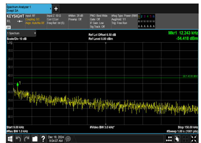
Band2-3MHz-QPSK-18900-1RB#0-0.009~0.15-PASS
