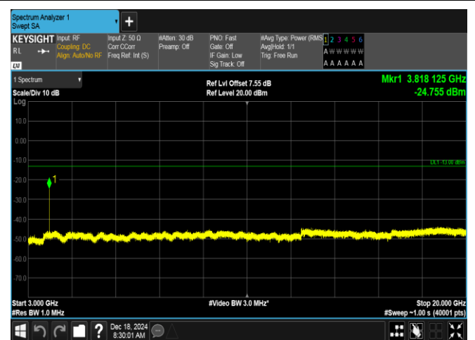
Band2-1.4MHz-16QAM-19193-6RB#0-3000~20000-PASS
