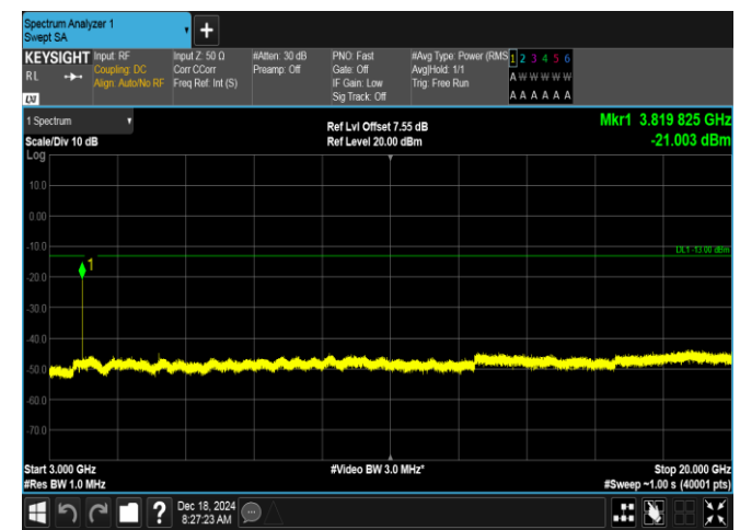
Band2-1.4MHz-QPSK-19193-1RB#5-3000~20000-PASS
