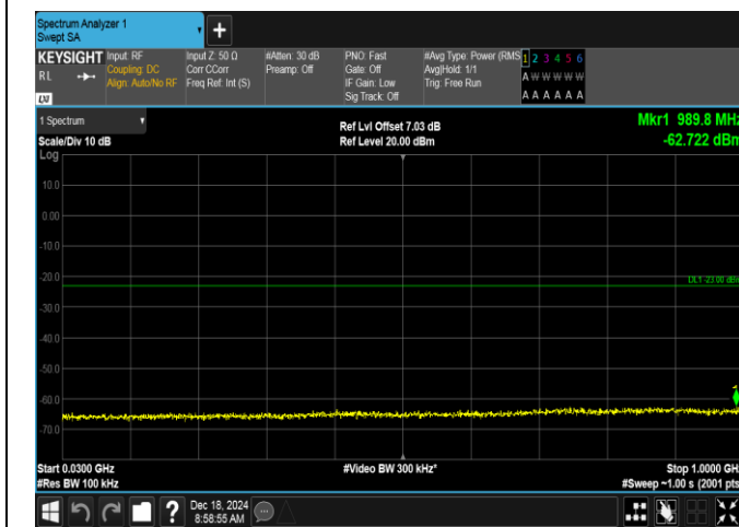
Band2-3MHz-QPSK-18615-1RB#0-30~1000-PASS
