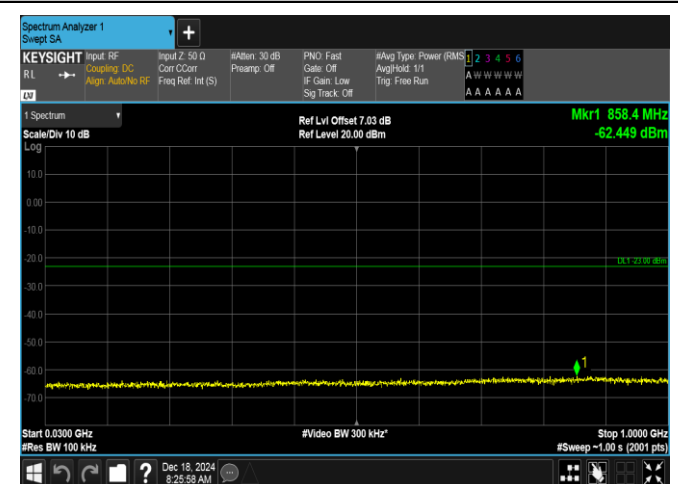
Band2-1.4MHz-16QAM-19193-1RB#0-30~1000-PASS
