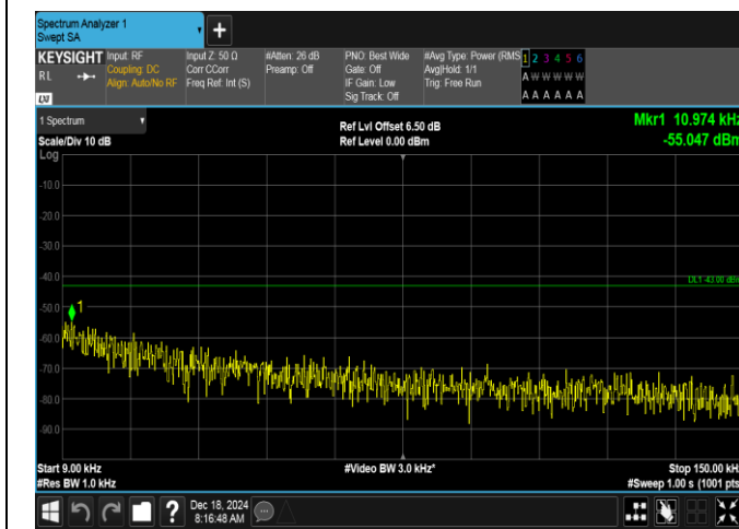
Band2-1.4MHz-16QAM-18607-1RB#5-0.009~0.15-PASS
