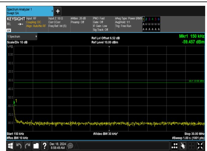
Band2-3MHz-QPSK-18615-1RB#0-0.15~30-PASS
