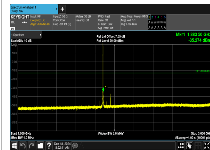
Band2-1.4MHz-16QAM-18900-1RB#5-1000~3000-PASS
