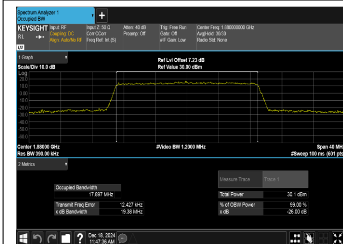
Band2-20MHz-16QAM-18900-100RB#0-PASS
