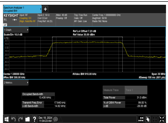
Band2-15MHz-QPSK-18900-75RB#0-PASS
