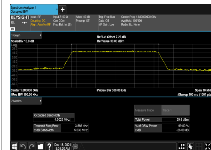
Band2-5MHz-16QAM-18900-25RB#0-PASS
