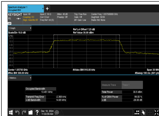
Band2-15MHz-QPSK-18675-75RB#0-PASS
