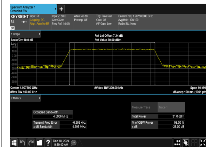
Band2-5MHz-QPSK-19175-25RB#0-PASS
