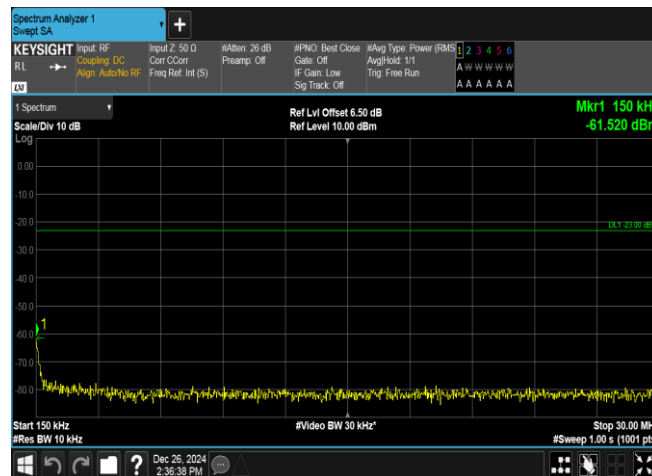
Band5-4233-1-0.15~30MHz-PASS
