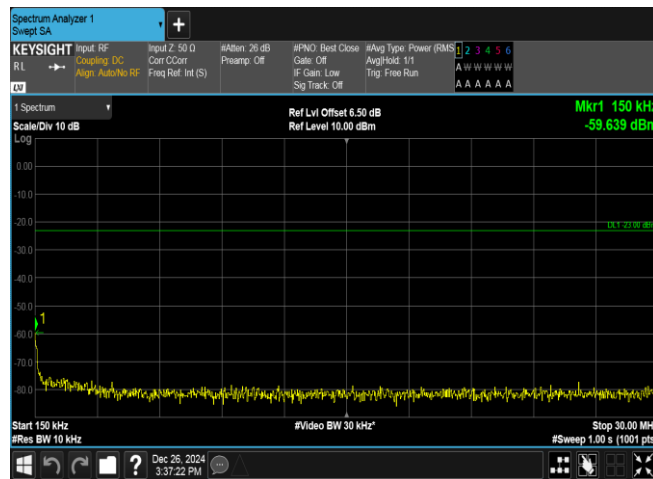
Band5-4132-1-0.15~30MHz-PASS
