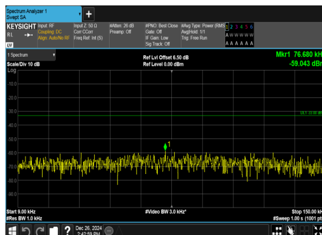
Band5-4233-4-0.009~0.15MHz-PASS
