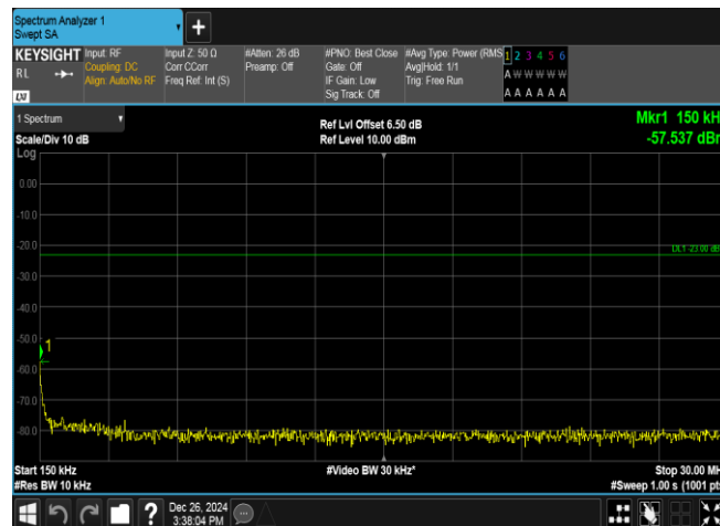
Band5-4182-1-0.15~30MHz-PASS
