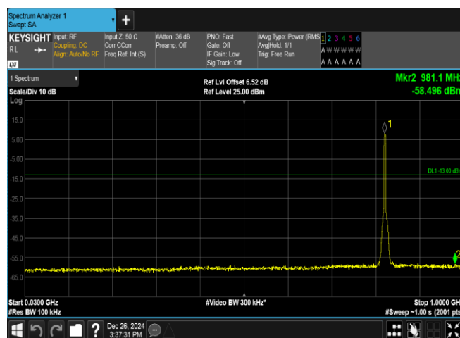
Band5-4132-1-30~1000MHz-PASS
