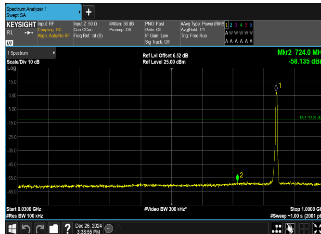
Band5-4233-1-30~1000MHz-PASS
