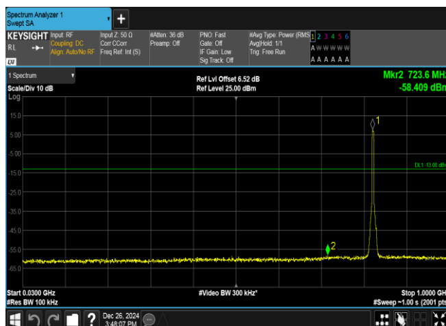
Band5-4132-5-30~1000MHz-PASS
