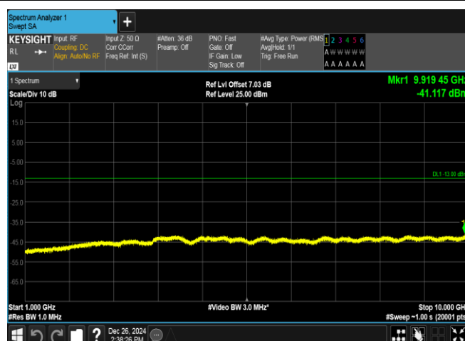
Band5-4182-2-1000~10000MHz-PASS
