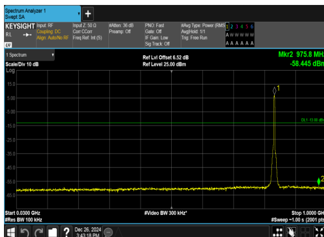
Band5-4182-3-30~1000MHz-PASS
