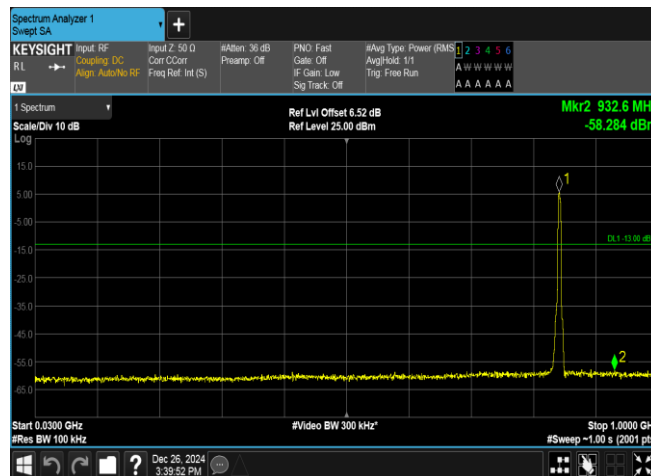
Band5-4132-2-30~1000MHz-PASS
