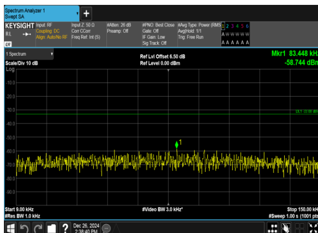
Band5-4233-2-0.009~0.15MHz-PASS
