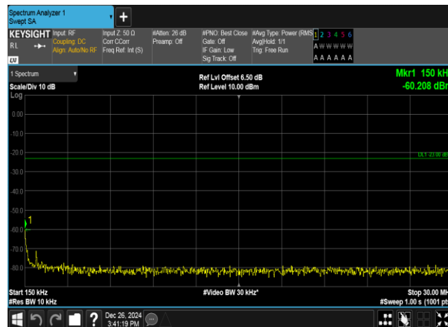
Band5-4233-2-0.15~30MHz-PASS
