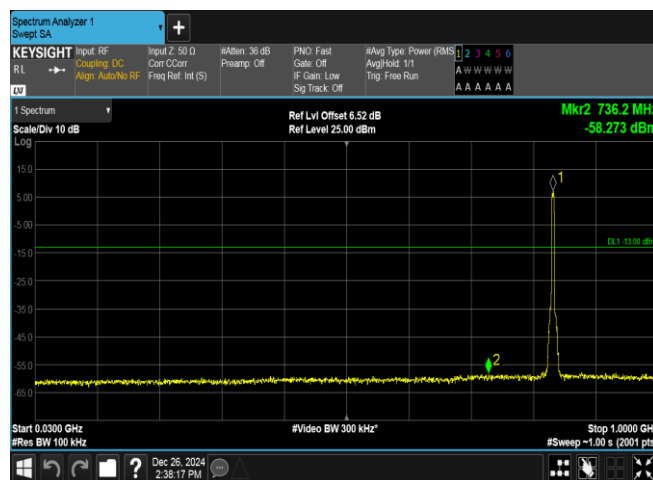
Band5-4182-2-30~1000MHz-PASS
