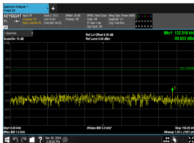
Band5-4182-2-0.009~0.15MHz-PASS
