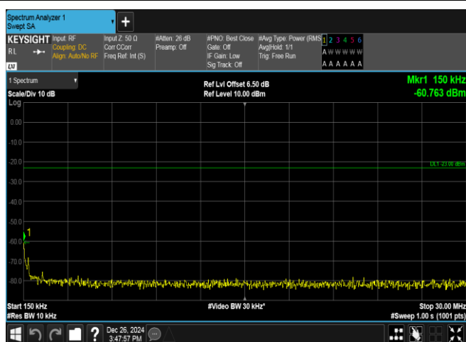
Band5-4132-5-0.15~30MHz-PASS
