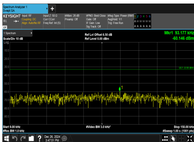
Band5-4132-5-0.009~0.15MHz-PASS
