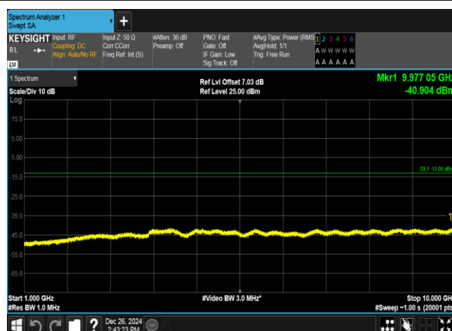
Band5-4233-4-1000~10000MHz-PASS
