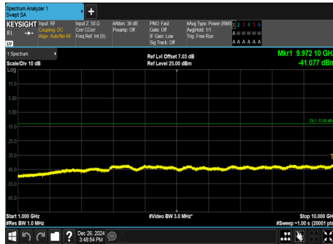
Band5-4182-5-1000~10000MHz-PASS
