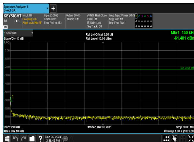
Band5-4233-1-0.15~30MHz-PASS
