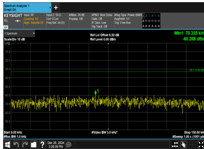
Band5-4233-1-0.009~0.15MHz-PASS
