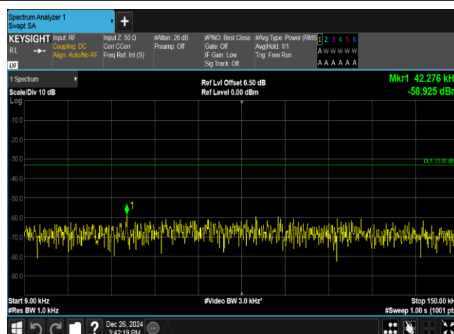
Band5-4132-3-0.009~0.15MHz-PASS
