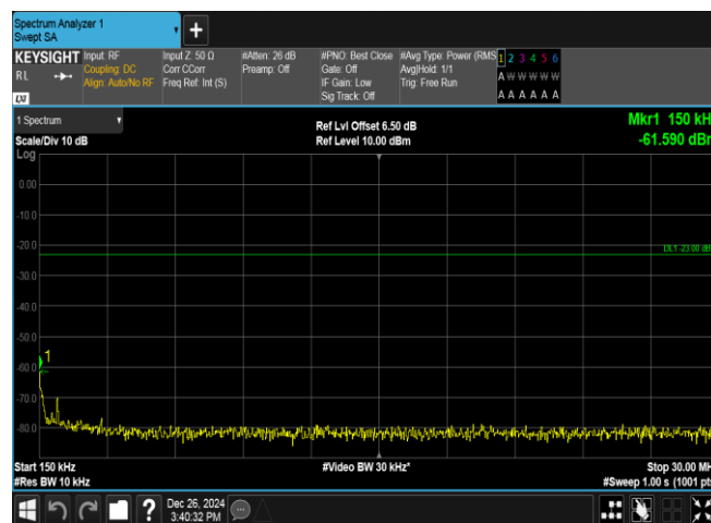
Band5-4182-2-0.15~30MHz-PASS
