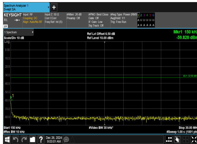
Band2-9538-1-0.15~30MHz-PASS
