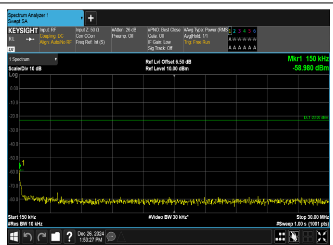
Band5-4132-0.15~30MHz-PASS
