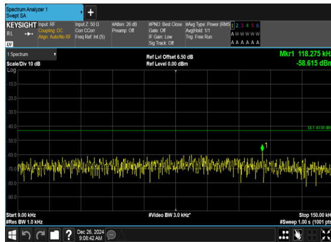
Band2-9400-4-0.009~0.15MHz-PASS
