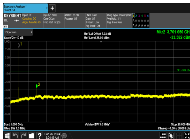
Band2-9400-2-1000~20000MHz-PASS
