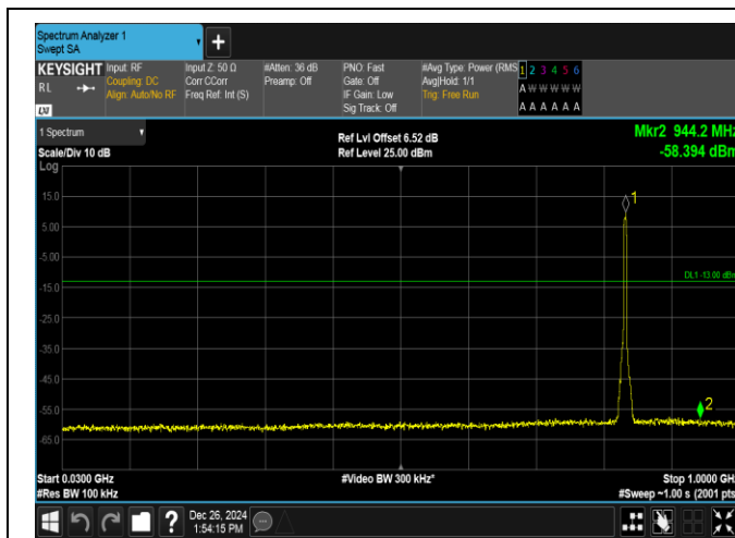
Band5-4182-30~1000MHz-PASS
