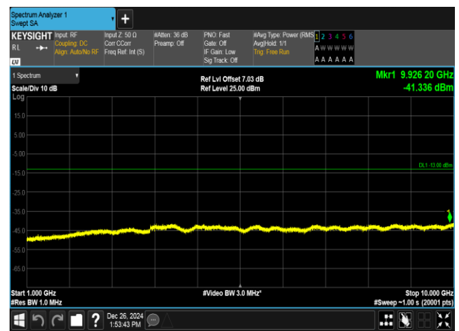
Band5-4132-1000~10000MHz-PASS
