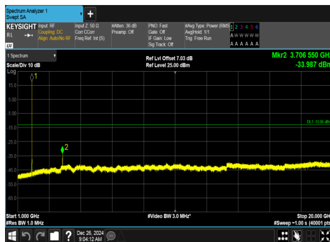
Band2-9262-2-1000~20000MHz-PASS
