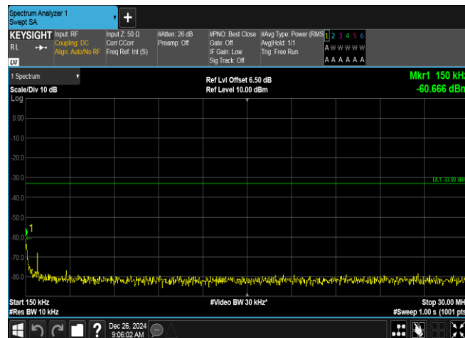
Band2-9262-3-0.15~30MHz-PASS
