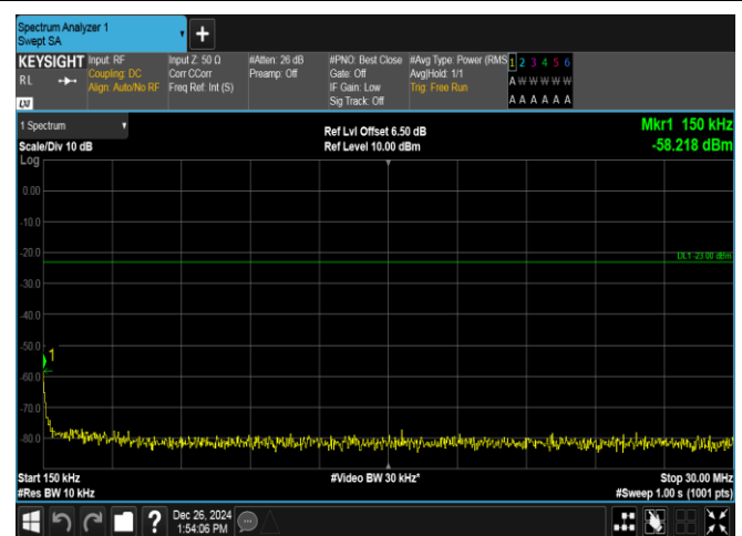
Band5-4182-0.15~30MHz-PASS
