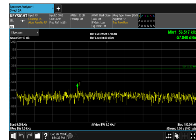
Band5-4233-0.009~0.15MHz-PASS
