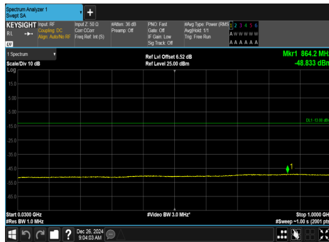
Band2-9262-2-30~1000MHz-PASS
