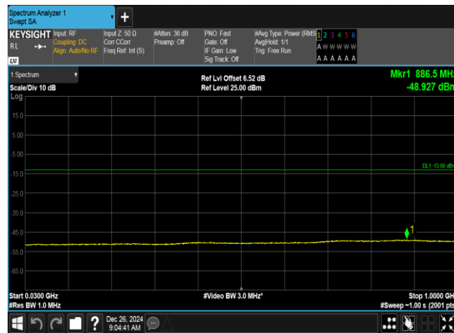
Band2-9400-2-30~1000MHz-PASS
