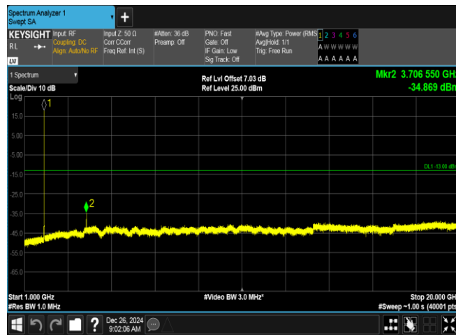
Band2-9262-1-1000~20000MHz-PASS
