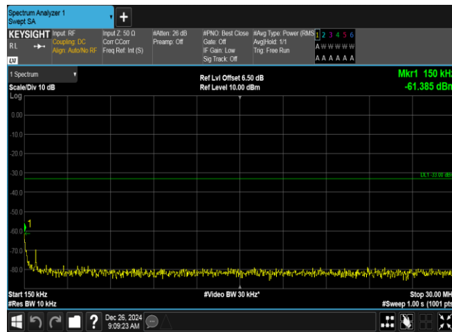
Band2-9538-4-0.15~30MHz-PASS
