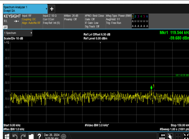
Band2-9262-3-0.009~0.15MHz-PASS
