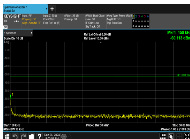
Band2-9262-2-0.15~30MHz-PASS
