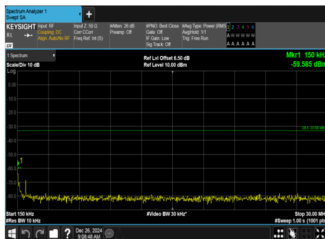
Band2-9400-4-0.15~30MHz-PASS
